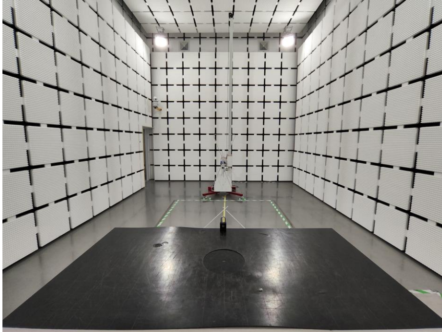
Radiated Spurious Emission bellow 1GHz
