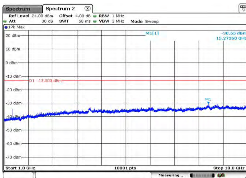
B13_CH23205_5M_1RB0_QPSK_Above 1G
