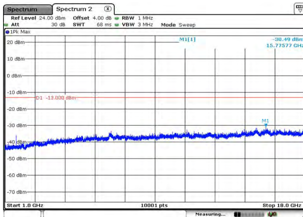
B26_CH26697_1.4M_1RB0_QPSK_Above 1G
