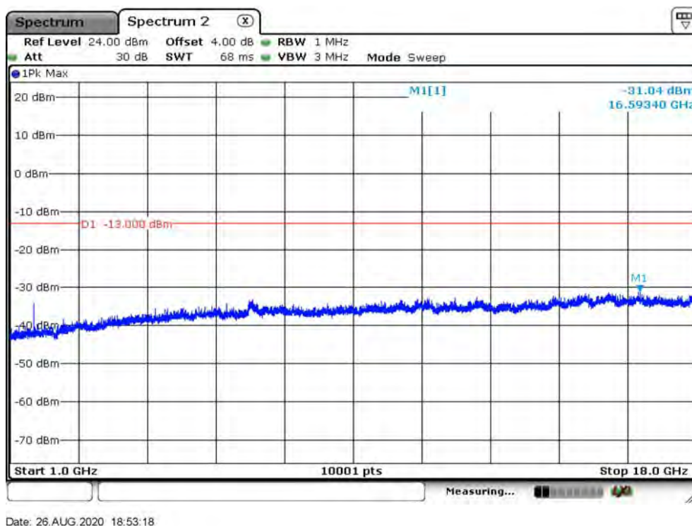
B14_CH23305_5M_1RB0_QPSK_Above 1G
