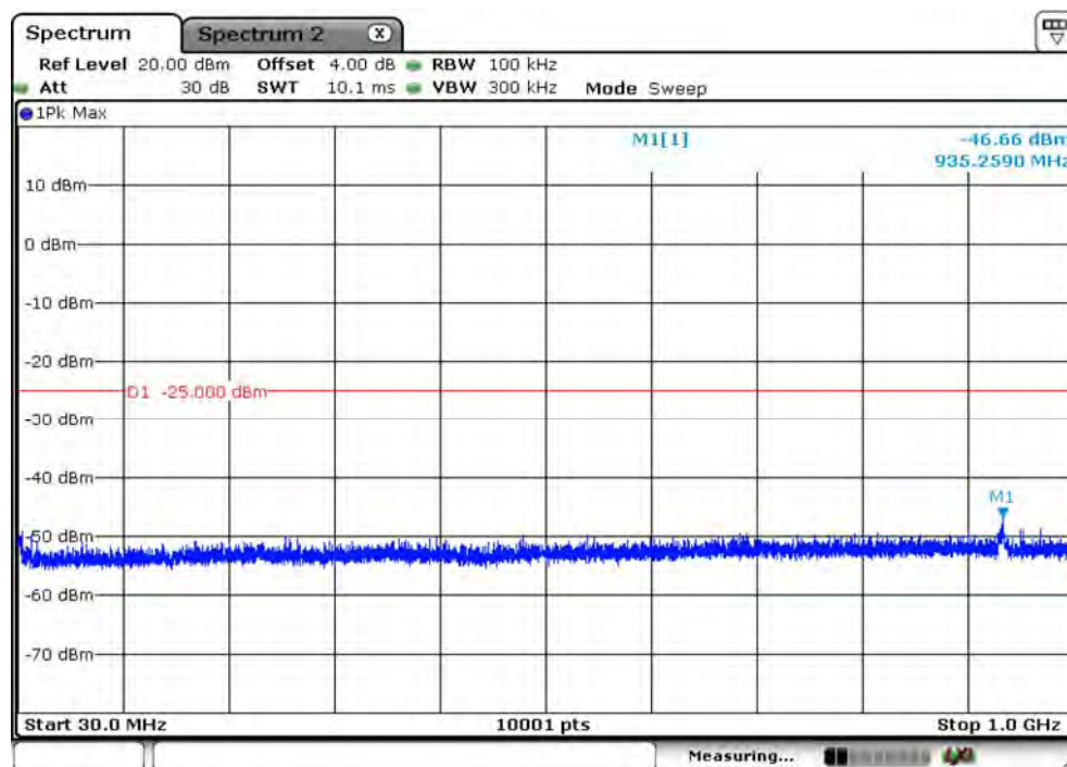
B41_CH39675_5M_1RB12__QPSK_Below 1G
