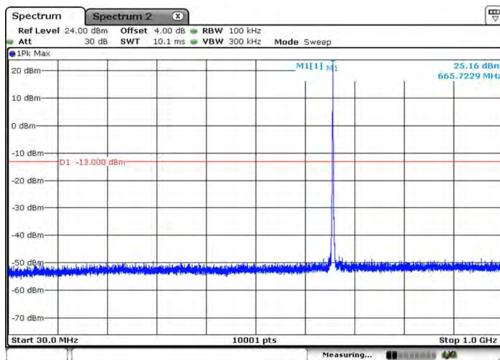
B71_CH133147_5M_1RB12_QPSK_Below 1G
