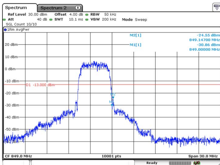
WCDMA_Band 5_RMC_846.6
