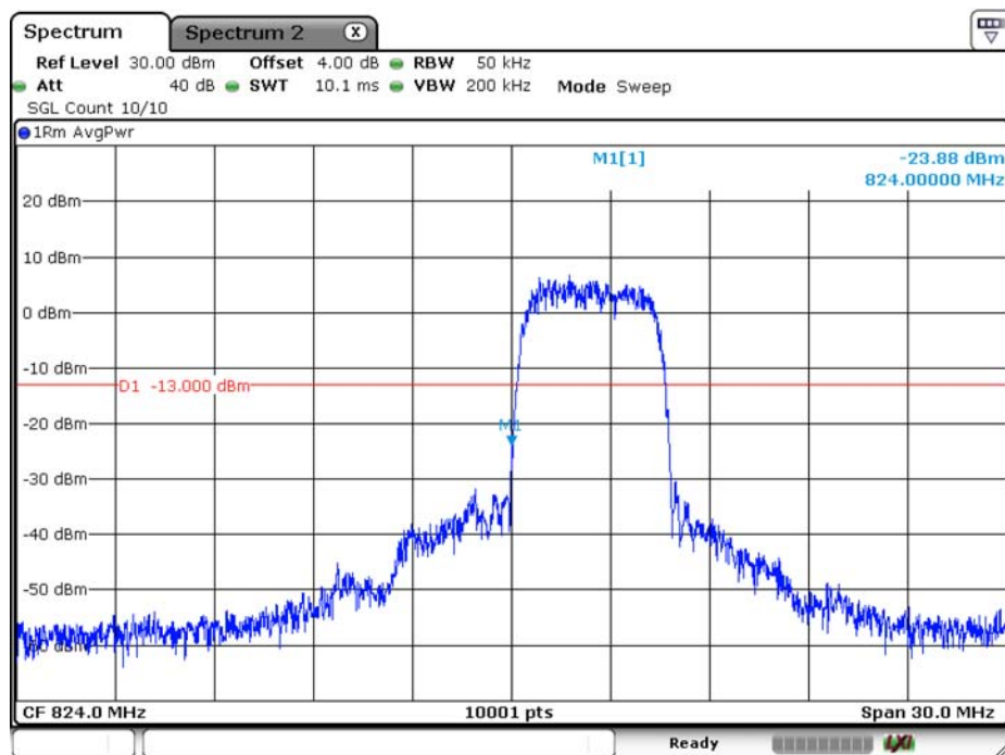
WCDMA_Band 5_RMC_826.4
