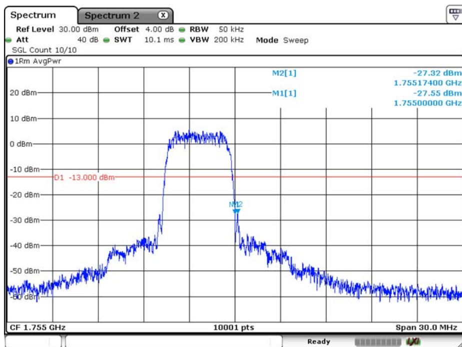
WCDMA_Band 4_RMC_1752.6
