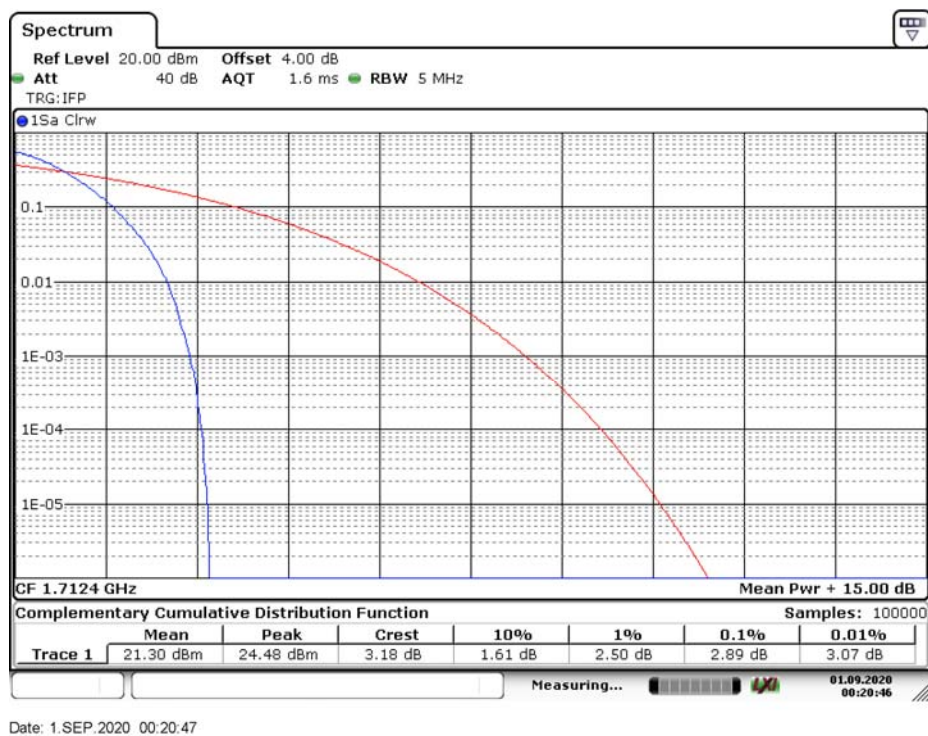
WCDMA_Band 4_RMC_1712.4MHz
