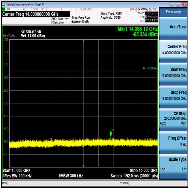
BLE_2M-Ant1-2402-13000~15000-PASS
