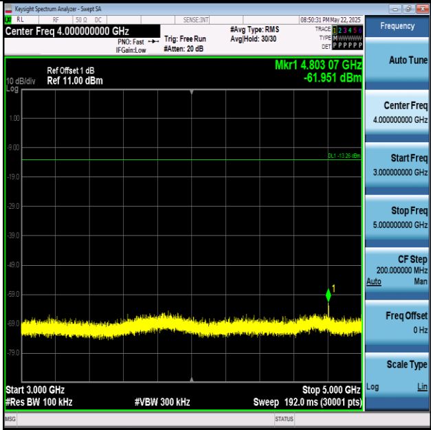
BLE_2M-Ant1-2402-3000~5000-PASS
