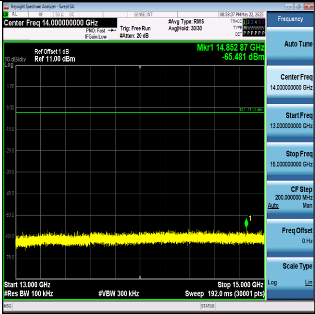
BLE_2M-Ant1-2440-13000~15000-PASS
