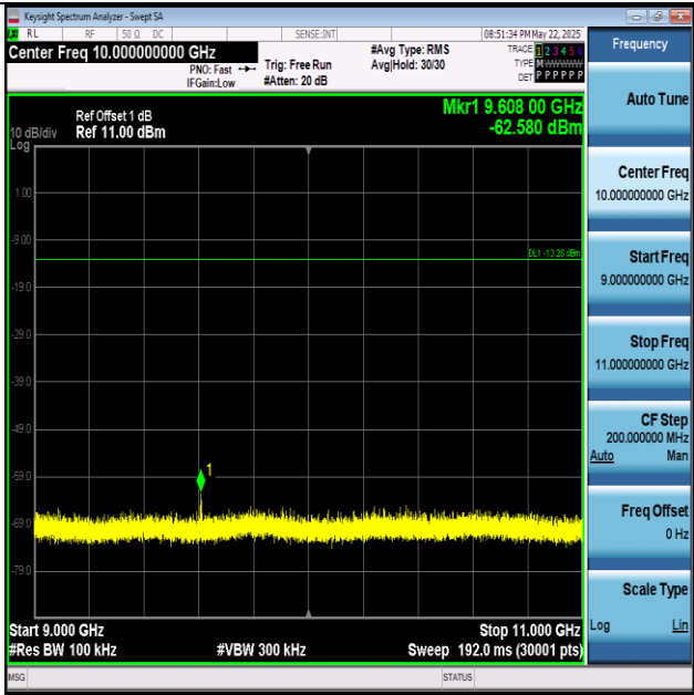
BLE_2M-Ant1-2402-9000~11000-PASS
