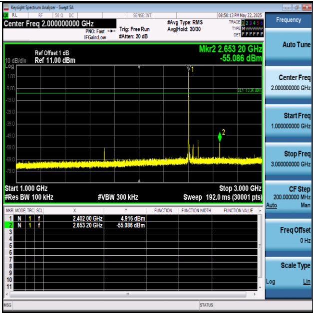
BLE_2M-Ant1-2402-1000~3000-PASS
