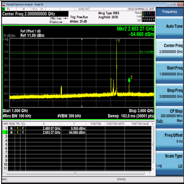
BLE_2M-Ant1-2480-1000~3000-PASS
