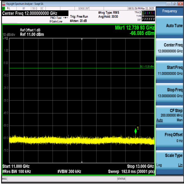
BLE_2M-Ant1-2402-11000~13000-PASS
