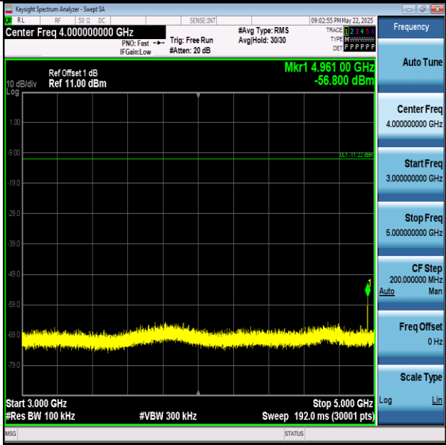
BLE_2M-Ant1-2480-3000~5000-PASS
