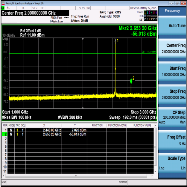
BLE_2M-Ant1-2440-1000~3000-PASS
