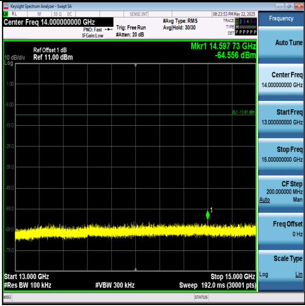
BLE_1M-Ant1-2402-13000~15000-PASS
