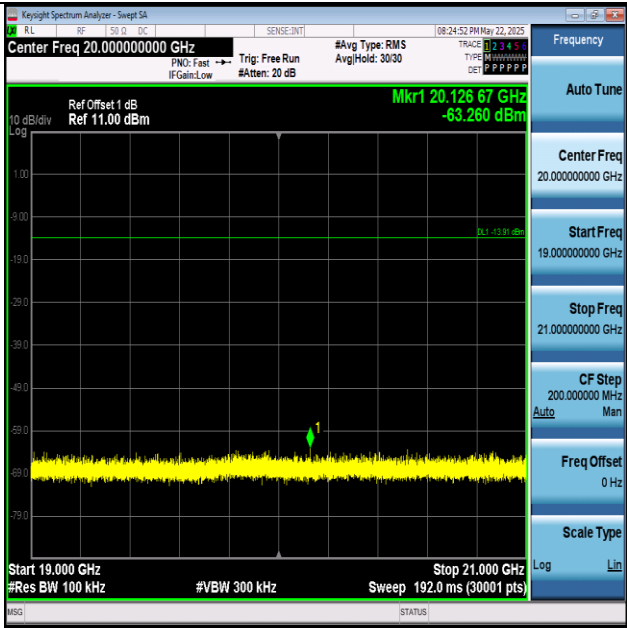
BLE_1M-Ant1-2402-19000~21000-PASS
