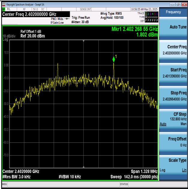
BLE_500K-Ant1-2402-PASS
