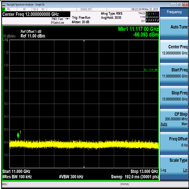
BLE_1M-Ant1-2402-11000~13000-PASS
