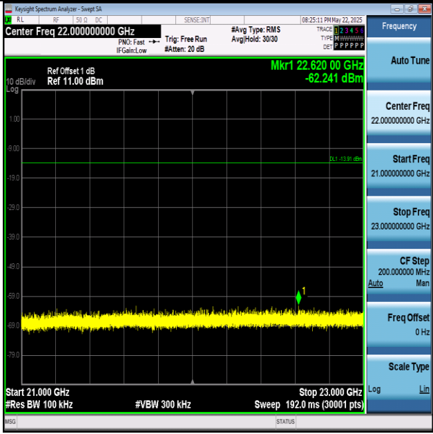
BLE_1M-Ant1-2402-21000~23000-PASS
