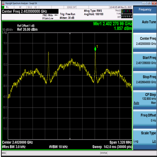
BLE_125K-Ant1-2402-PASS
