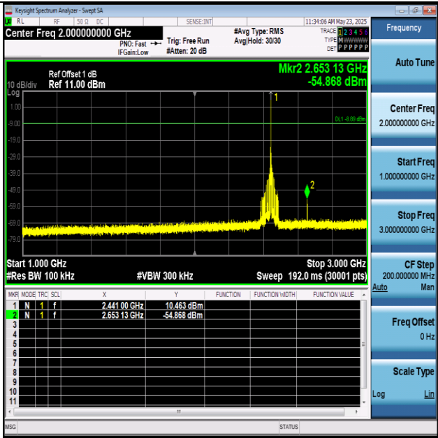
DH5-Ant1-2441-1000~3000-PASS
