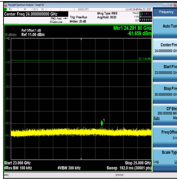
DH5-Ant1-2480-23000~25000-PASS
