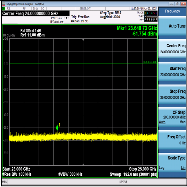
DH5-Ant1-2441-23000~25000-PASS
