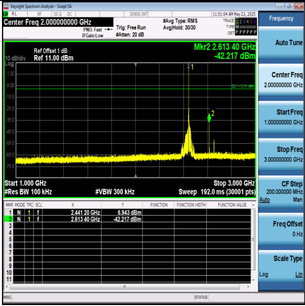
2DH5-Ant1-2441-1000~3000-PASS
