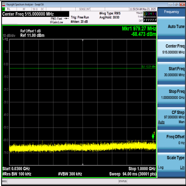
2DH5-Ant1-2441-30~1000-PASS
