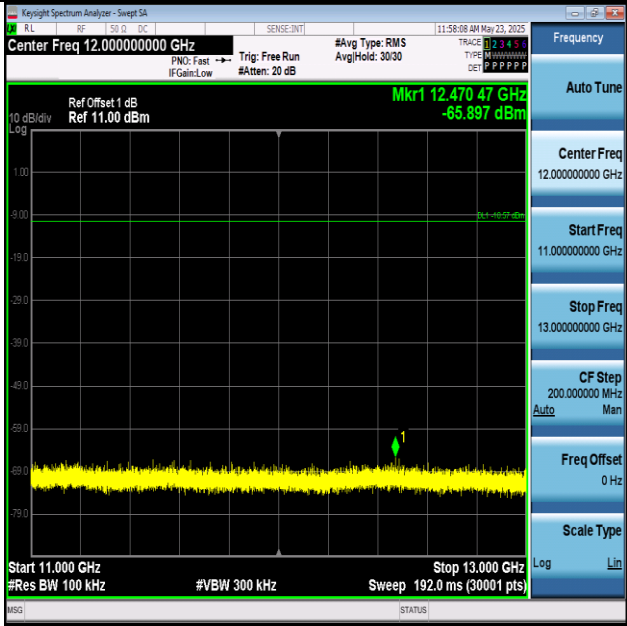
2DH5-Ant1-2480-11000~13000-PASS
