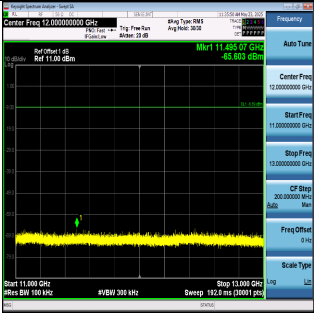
DH5-Ant1-2441-11000~13000-PASS
