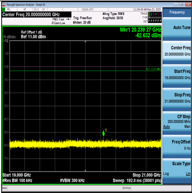
2DH5-Ant1-2441-19000~21000-PASS
