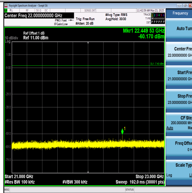
DH5-Ant1-2480-21000~23000-PASS
