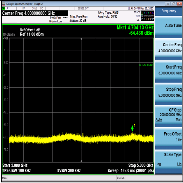
2DH5-Ant1-2402-3000~5000-PASS
