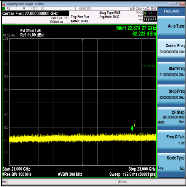
2DH5-Ant1-2441-21000~23000-PASS
