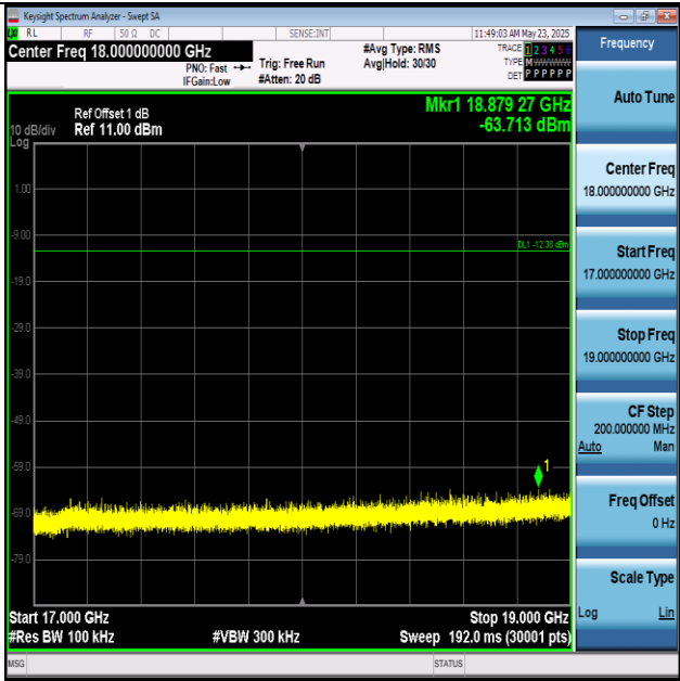
2DH5-Ant1-2402-17000~19000-PASS
