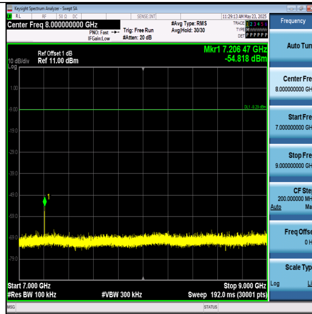
DH5-Ant1-2402-7000~9000-PASS
