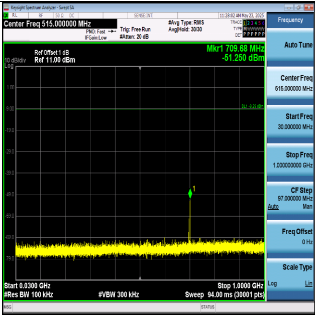
DH5-Ant1-2402-30~1000-PASS
