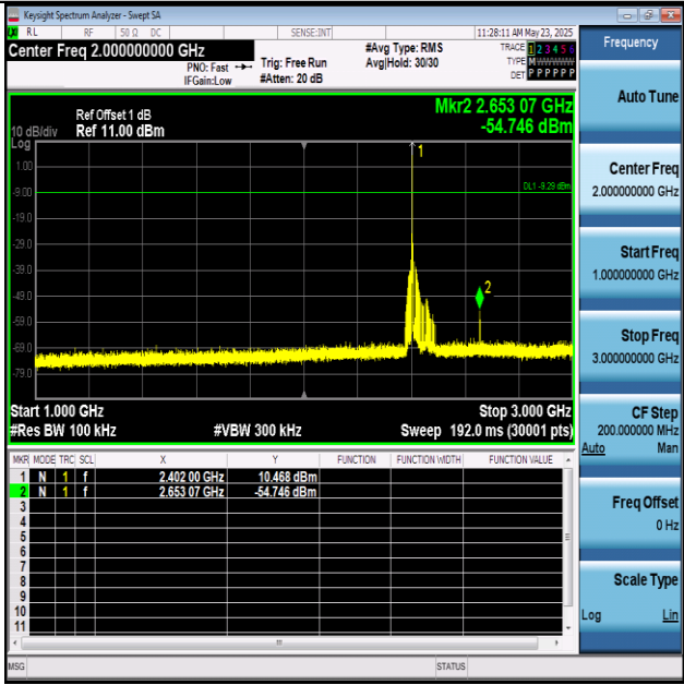
DH5-Ant1-2402-1000~3000-PASS
