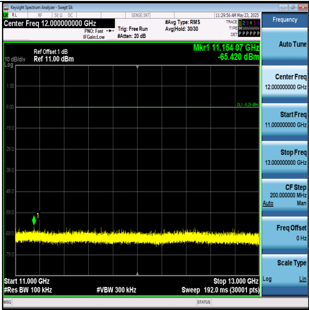
DH5-Ant1-2402-11000~13000-PASS
