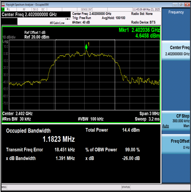
2DH5-Ant1-2402
