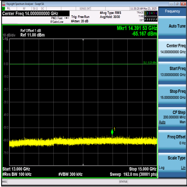
DH5-Ant1-2402-13000~15000-PASS
