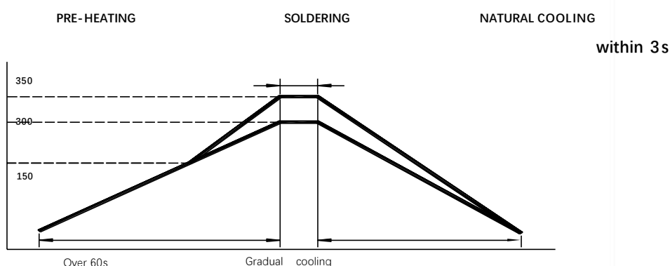
Iron Soldering
