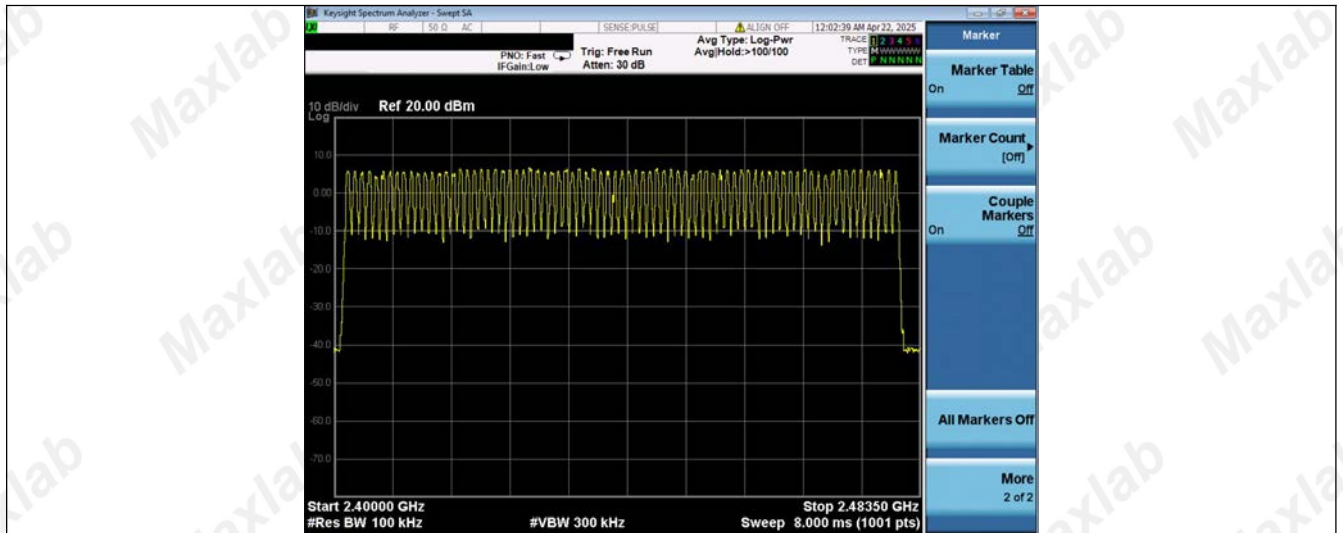
GFSK Modulation
