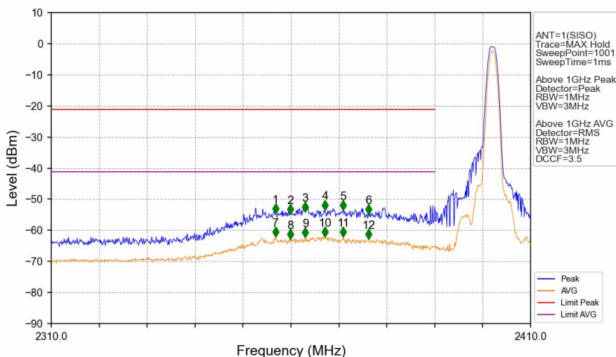
1M_LCH_2402MHz_Ant1_NTNV
