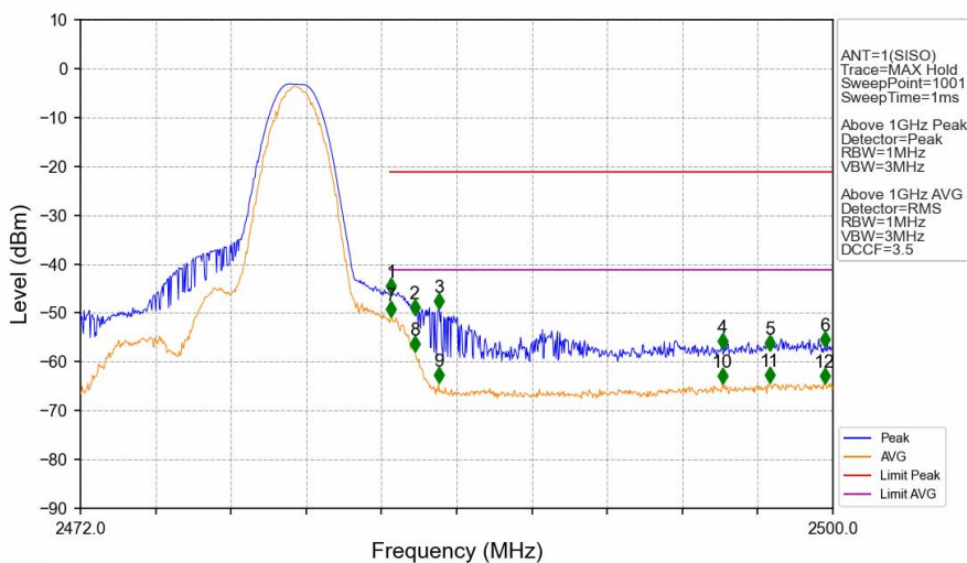
1M_HCH_2480MHz_Ant1_NTNV
