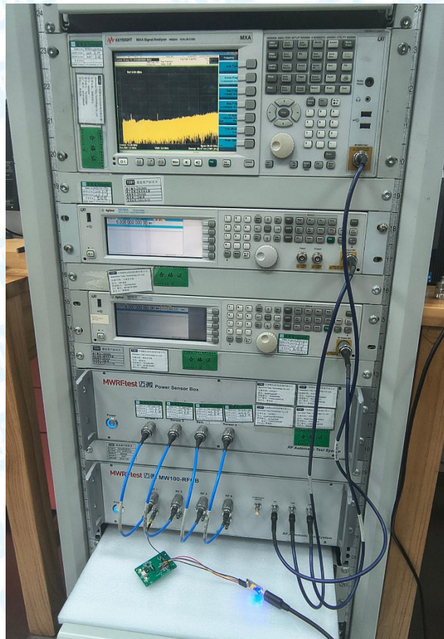
Photo of Setup for Conducted Measurement
