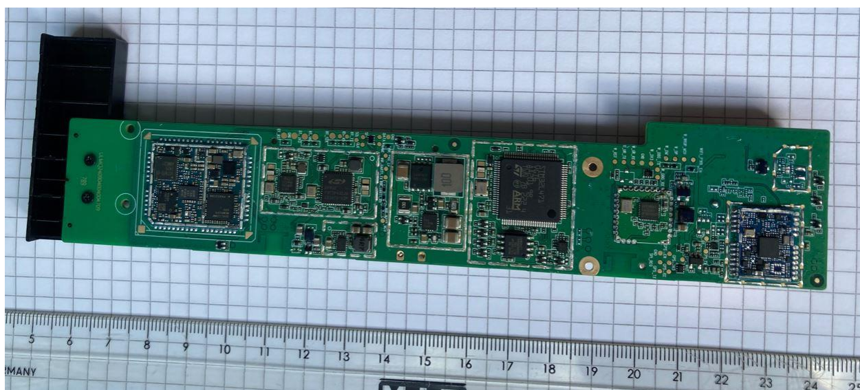
Figure 2: PCB Front without Shields
