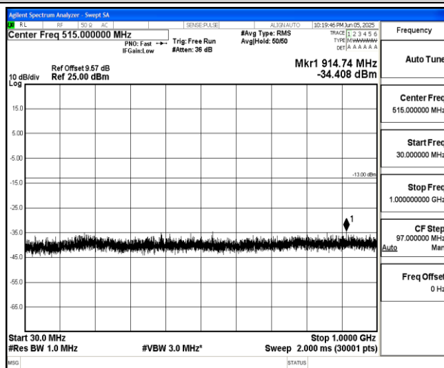
Band66-20MHz-16QAM-132322-1-0-Low-30-1000--34.41-PASS
