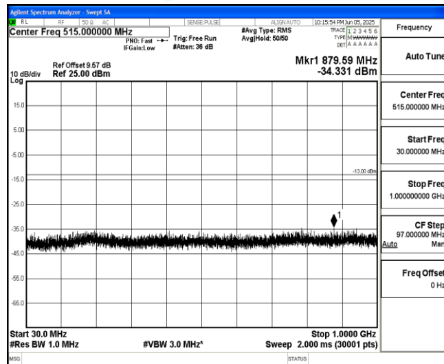
Band66-20MHz-16QAM-132072-1-0-Low-30-1000--34.33-PASS
