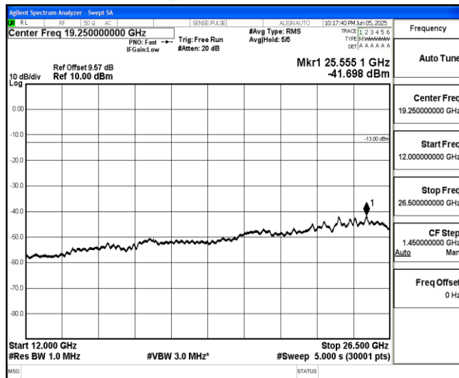
Band66-20MHz-16QAM-132072-1-0-Low-12000-26500--41.7-PASS
