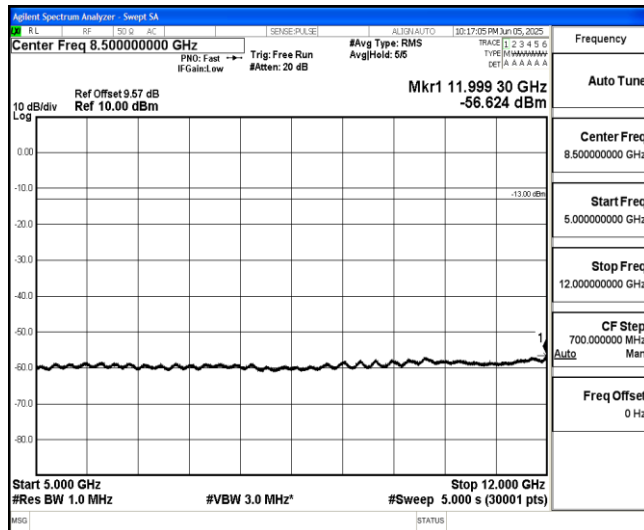
Band66-20MHz-16QAM-132072-1-0-Low-5000-12000--56.62-PASS
