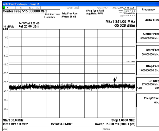
Band66-15MHz-QPSK-132597-1-0-High-30-1000--35.03-PASS
