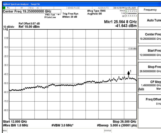
Band66-1.4MHz-QPSK-132665-1-0-High-12000-26500--41.64-PASS
