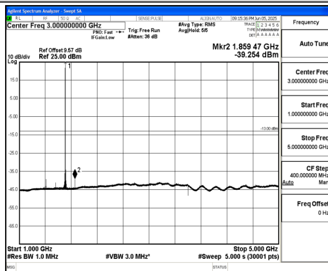
Band66-5MHz-16QAM-131997-1-0-Low-1000-5000--39.25-PASS
