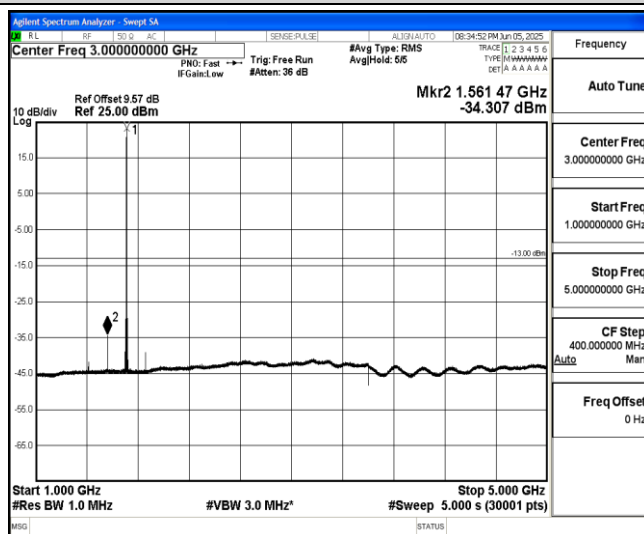
Band66-1.4MHz-16QAM-131979-1-0-Low-1000-5000--34.31-PASS
