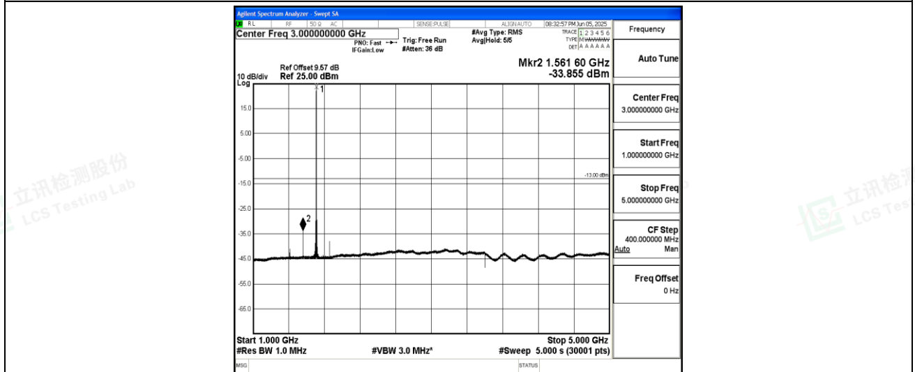
Band66-1.4MHz-QPSK-131979-1-0-Low-1000-5000--33.86-PASS
