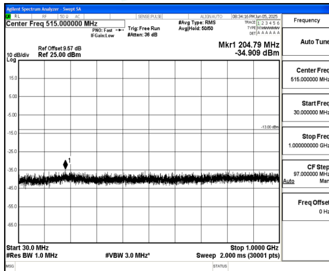
Band66-1.4MHz-16QAM-131979-1-0-Low-30-1000--34.91-PASS
