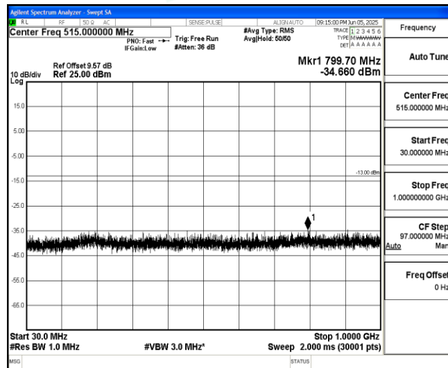
Band66-5MHz-16QAM-131997-1-0-Low-30-1000--34.66-PASS
