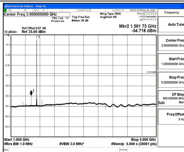
Band66-3MHz-16QAM-131987-1-0-Low-1000-5000--34.72-PASS
