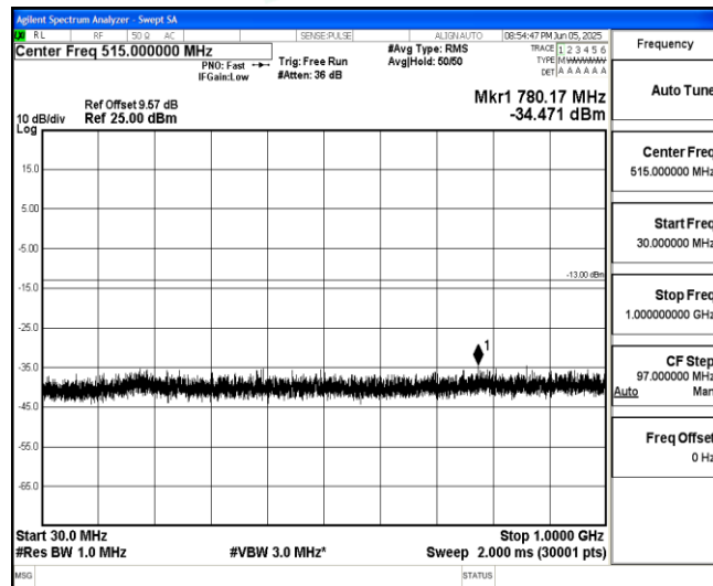
Band66-3MHz-16QAM-131987-1-0-Low-30-1000--34.47-PASS
