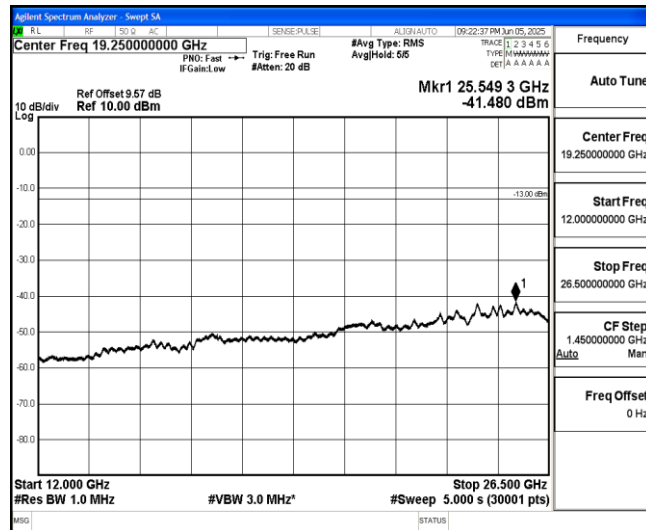
Band66-5MHz-QPSK-132647-1-0-High-12000-26500--41.48-PASS
