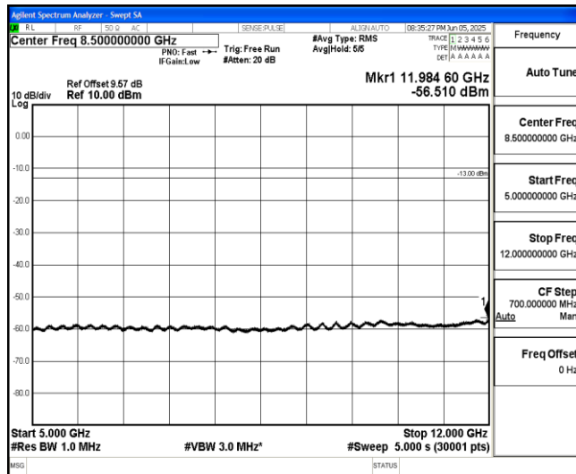
Band66-1.4MHz-16QAM-131979-1-0-Low-5000-12000--56.51-PASS
