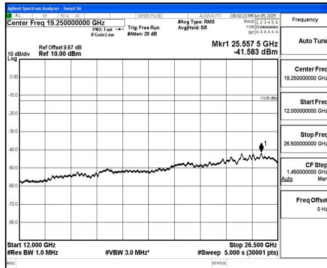
Band66-3MHz-QPSK-132657-1-0-High-12000-26500--41.58-PASS
