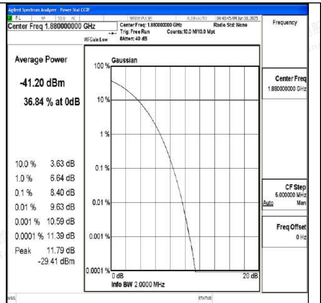
Channel 661 / 1880 MHz
