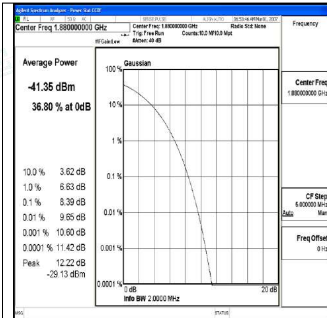
Channel 661 / 1880 MHz
