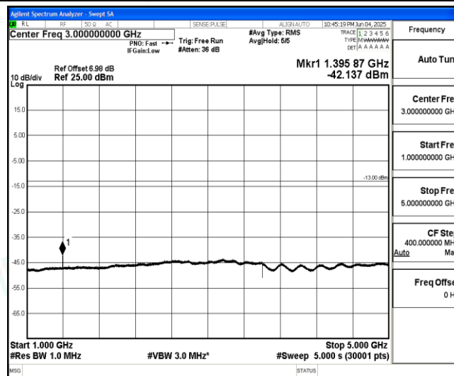
Band71-Stand-Alone-NaN-BPSK-133471-1@11-15kHz-1000-5000-1000~5000MHz@-42.14dBm--13-PASS
