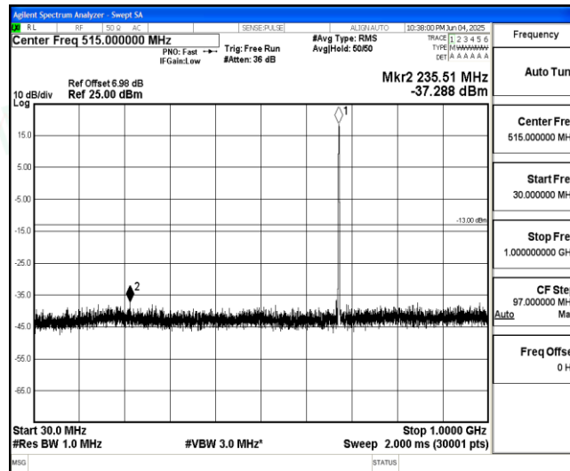
Band71-Stand-Alone-NaN-BPSK-133297-1@0-15kHz-30-1000-30~1000MHz@-37.29dBm--13-PASS
