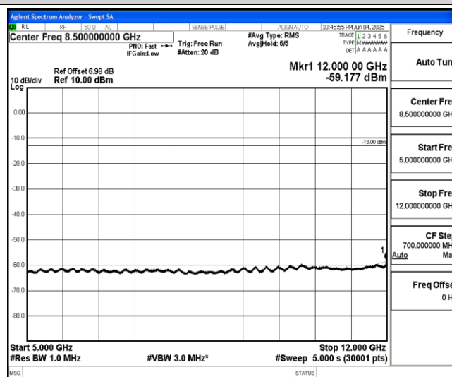
Band71-Stand-Alone-NaN-BPSK-133471-1@11-15kHz-5000-12000-5000~12000MHz@-59.18dBm--13-PASS
