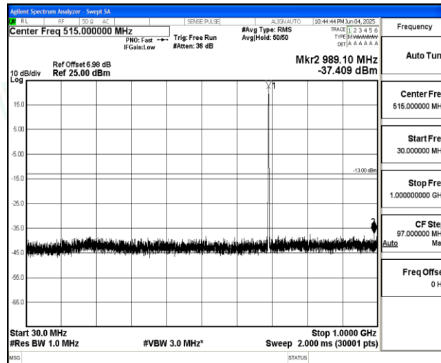
Band71-Stand-Alone-NaN-BPSK-133471-1@11-15kHz-30-1000-30~1000MHz@-37.41dBm--13-PASS
