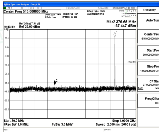
Band5-Stand-Alone-NaN-BPSK-20525-1@0-15kHz-30-1000-30~1000MHz@-37.45dBm--13-PASS
