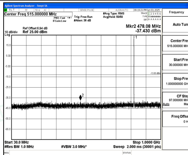
Band5-Stand-Alone-NaN-QPSK-20401-12@0-15kHz-30-1000-30~1000MHz@-37.43dBm--13-PASS
