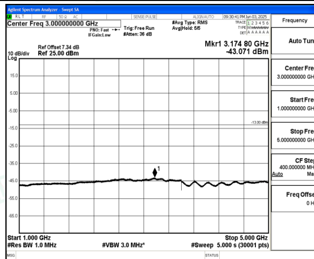
Band5-Stand-Alone-NaN-BPSK-20525-1@0-15kHz-1000-5000-1000~5000MHz@-43.07dBm--13-PASS
