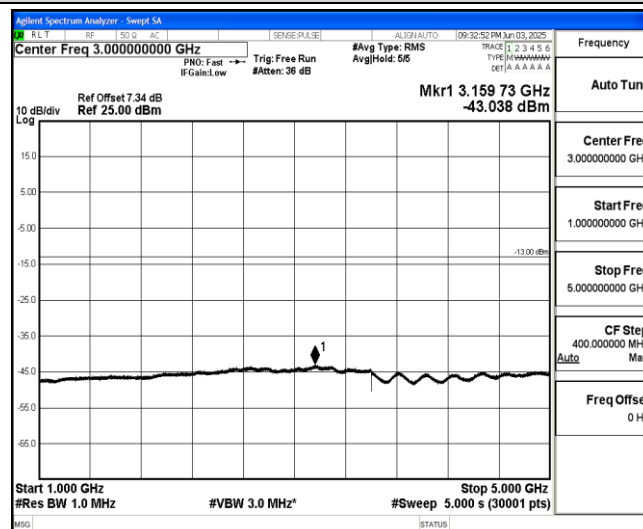
Band5-Stand-Alone-NaN-BPSK-20525-1@11-15kHz-1000-5000-1000~5000MHz@-43.04dBm--13-PASS
