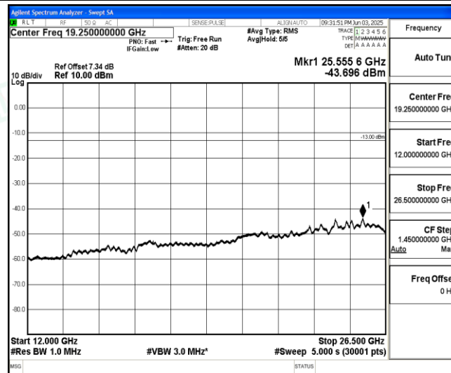
Band5-Stand-Alone-NaN-BPSK-20525-1@0-15kHz-12000-26500-12000~26500MHz@-43.7dBm--13-PASS
