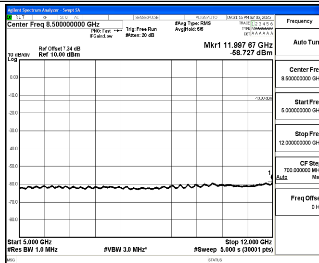
Band5-Stand-Alone-NaN-BPSK-20525-1@0-15kHz-5000-12000-5000~12000MHz@-58.73dBm--13-PASS
