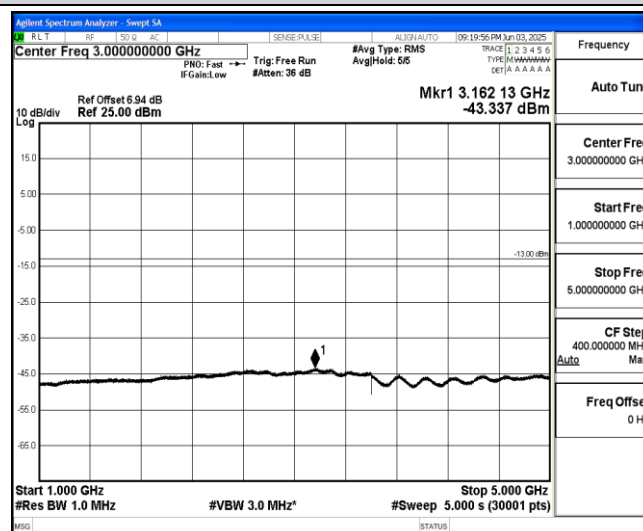
Band5-Stand-Alone-NaN-QPSK-20401-12@0-15kHz-1000-5000-1000~5000MHz@-43.34dBm--13-PASS
