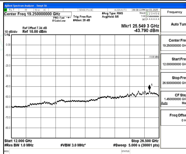
Band5-Stand-Alone-NaN-BPSK-20649-1@11-15kHz-12000-26500-12000~26500MHz@-43.79dBm--13-PASS
