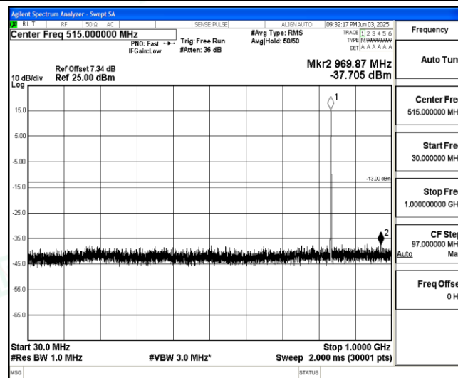
Band5-Stand-Alone-NaN-BPSK-20525-1@11-15kHz-30-1000-30~1000MHz@-37.71dBm--13-PASS
