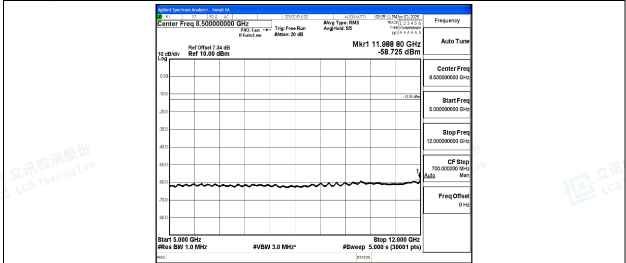
Band26-15MHz-QPSK-26915-1-0-Low-5000-12000--58.73-PASS
