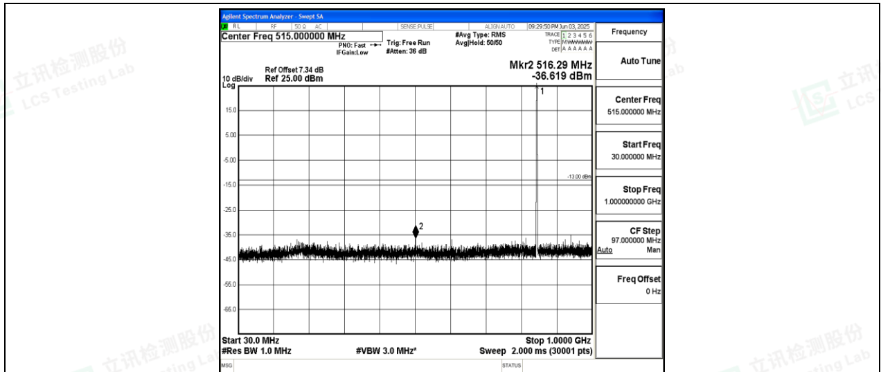
Band26-15MHz-16QAM-26965-1-0-High-30-1000--36.62-PASS
