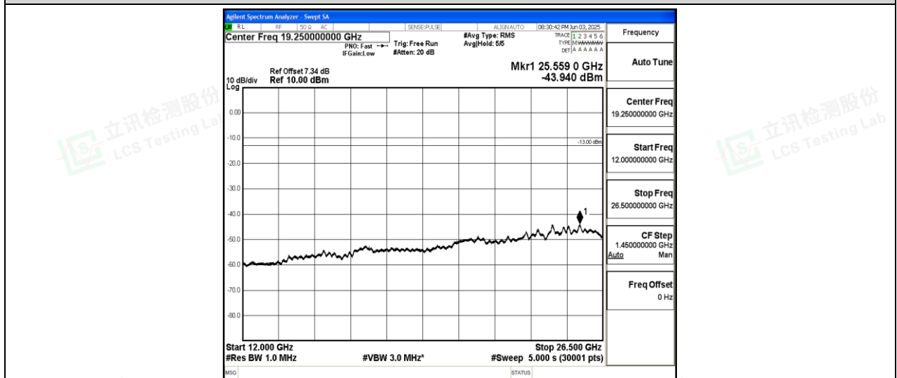
Band26-5MHz-16QAM-26915-1-0-Low-12000-26500--43.94-PASS
