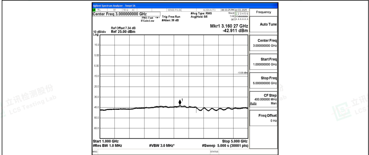
Band26-5MHz-16QAM-27015-1-0-High-1000-5000--42.91-PASS
