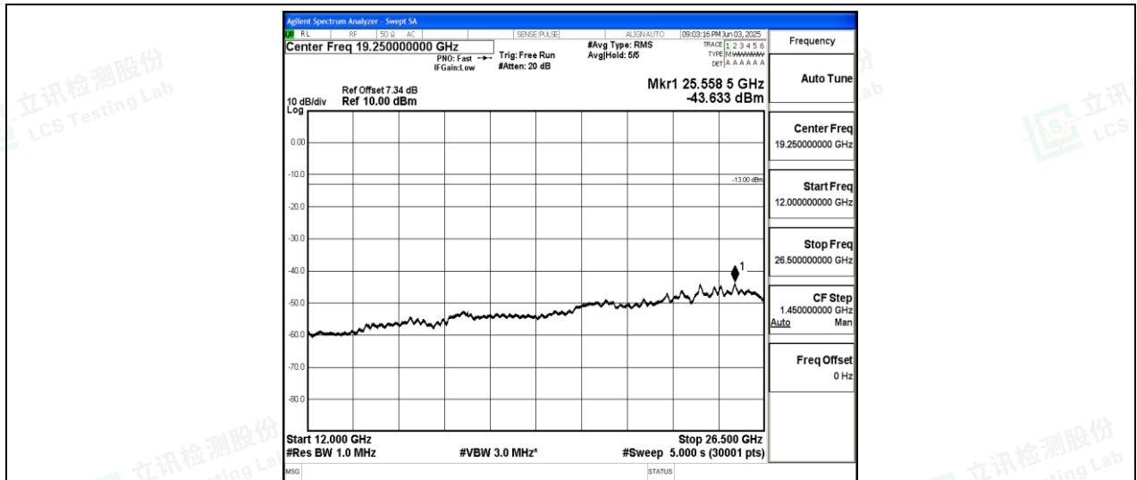
Band26-10MHz-16QAM-26990-1-0-High-12000-26500--43.63-PASS
