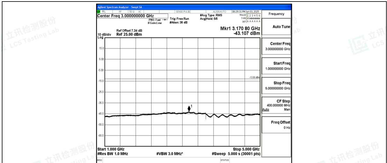
Band26-5MHz-16QAM-26915-1-0-Low-1000-5000--43.11-PASS
