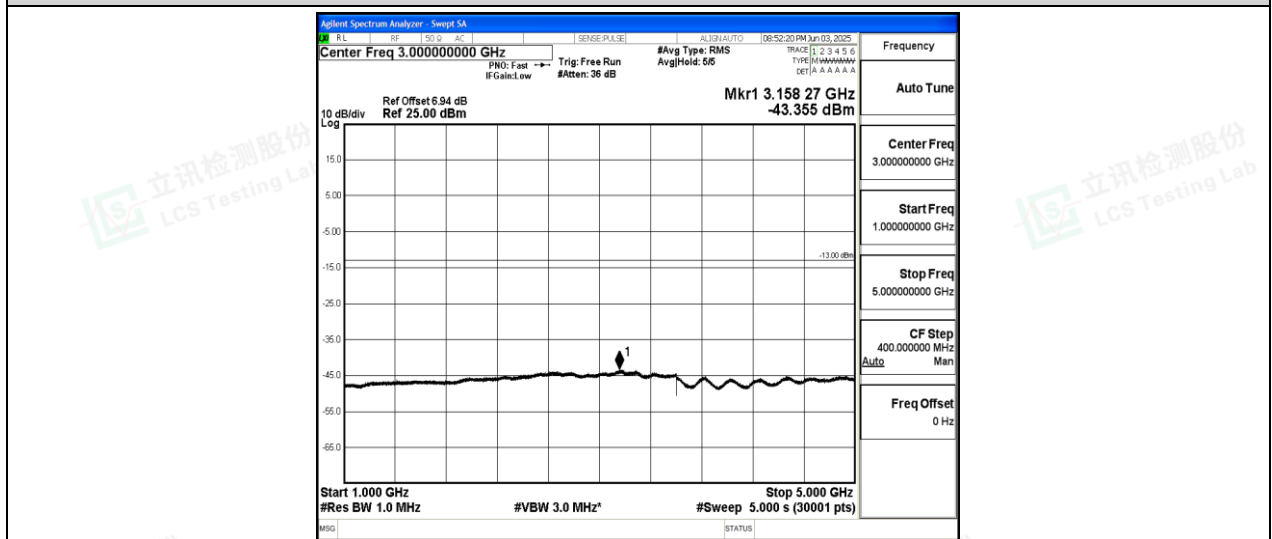
Band26-10MHz-QPSK-26840-1-0-Low-1000-5000--43.36-PASS
