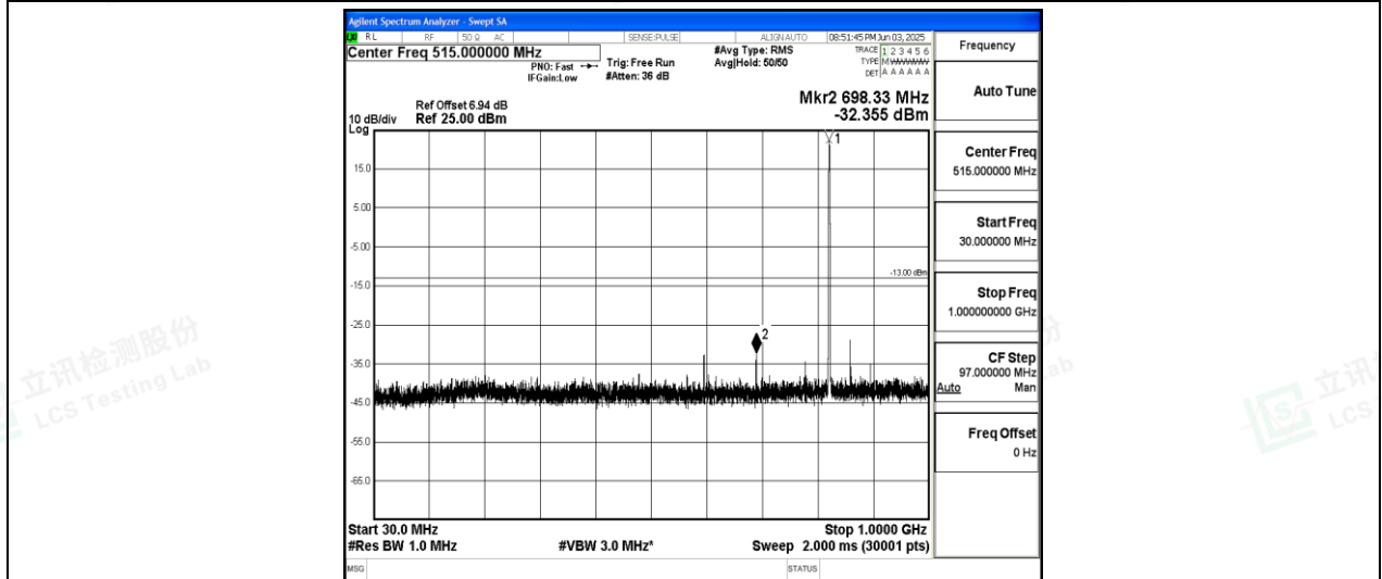
Band26-10MHz-QPSK-26840-1-0-Low-30-1000--32.36-PASS
