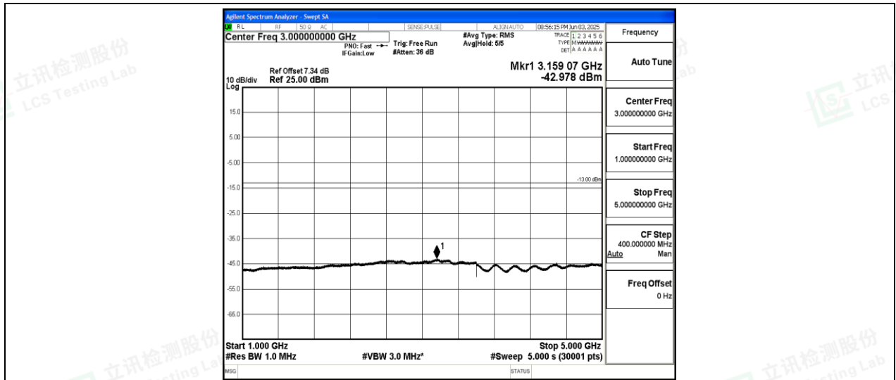
Band26-10MHz-QPSK-26915-1-0-Low-1000-5000--42.98-PASS
