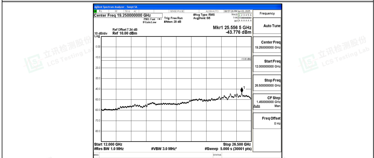
Band26-10MHz-QPSK-26915-1-0-Low-12000-26500--43.78-PASS
