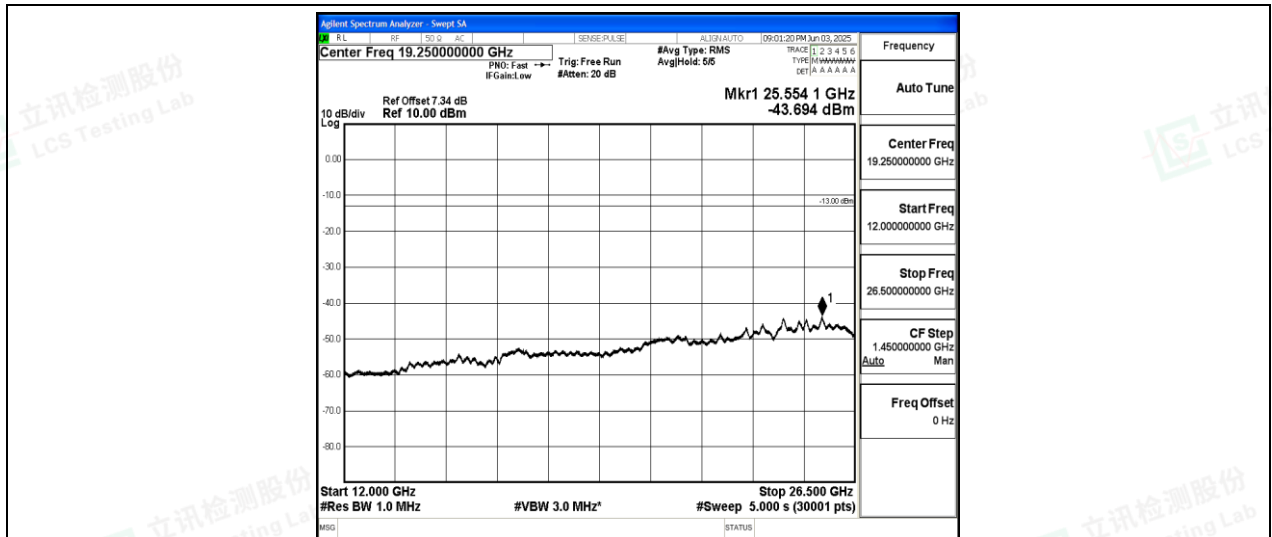
Band26-10MHz-QPSK-26990-1-0-High-12000-26500--43.69-PASS
