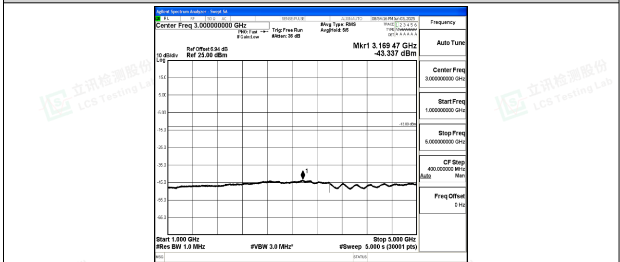
Band26-10MHz-16QAM-26840-1-0-Low-1000-5000--43.34-PASS
