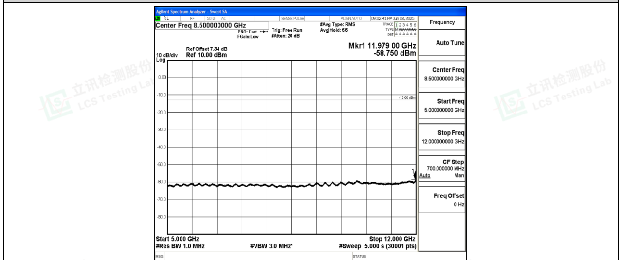
Band26-10MHz-16QAM-26990-1-0-High-5000-12000--58.75-PASS
