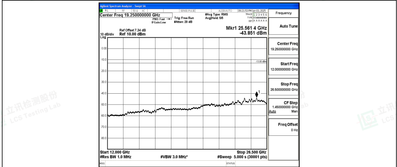
Band26-15MHz-QPSK-26865-1-0-Low-12000-26500--43.85-PASS
