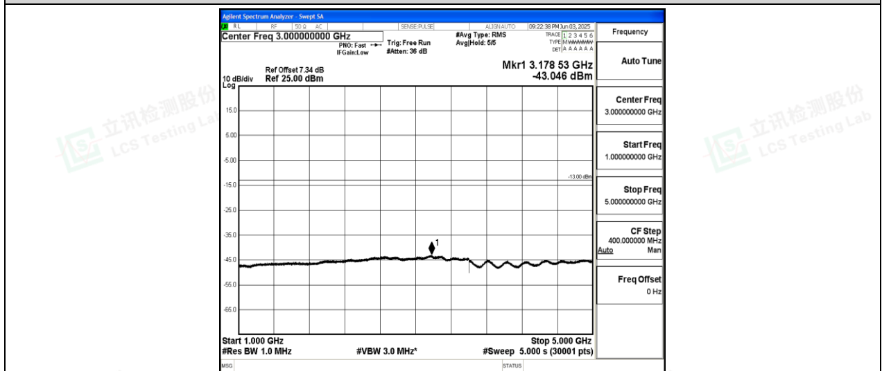
Band26-15MHz-16QAM-26865-1-0-Low-1000-5000--43.05-PASS
