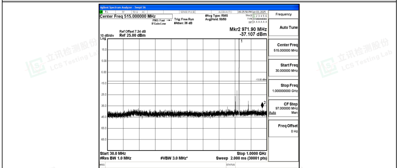
Band26-15MHz-16QAM-26915-1-0-Low-30-1000--37.11-PASS
