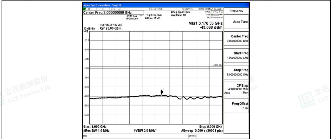
Band26-10MHz-QPSK-26990-1-0-High-1000-5000--43.07-PASS
