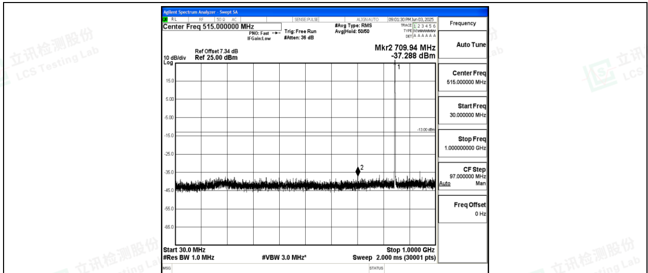
Band26-10MHz-16QAM-26990-1-0-High-30-1000--37.29-PASS
