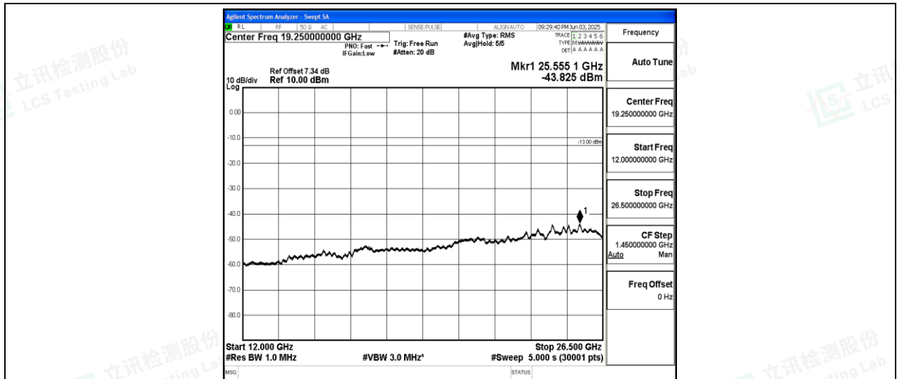
Band26-15MHz-QPSK-26965-1-0-High-12000-26500--43.83-PASS
