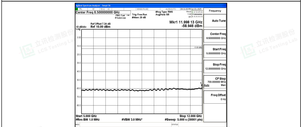
Band26-15MHz-16QAM-26965-1-0-High-5000-12000--58.95-PASS
