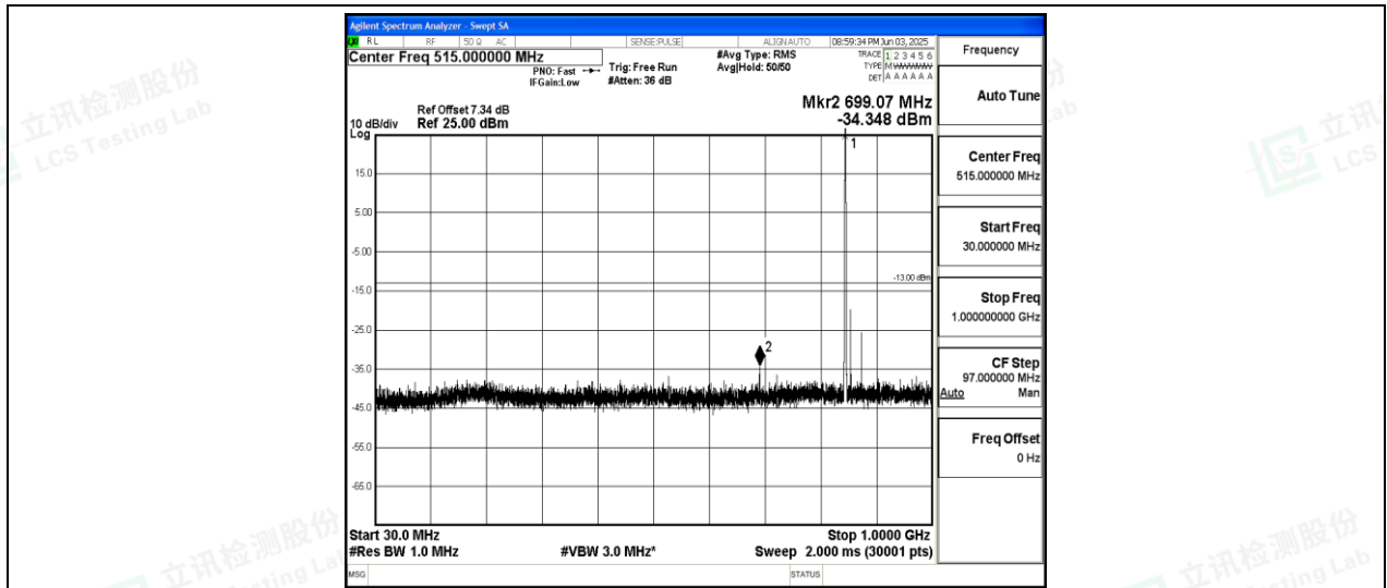
Band26-10MHz-QPSK-26990-1-0-High-30-1000--34.35-PASS
