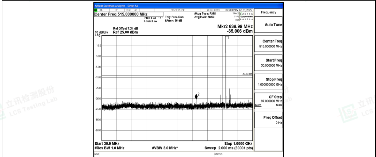
Band26-15MHz-QPSK-26865-1-0-Low-30-1000--35.81-PASS
