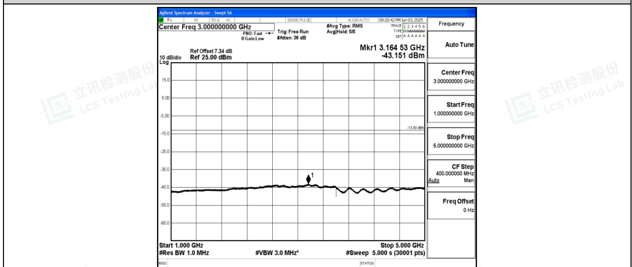
Band26-15MHz-QPSK-26865-1-0-Low-1000-5000--43.15-PASS
