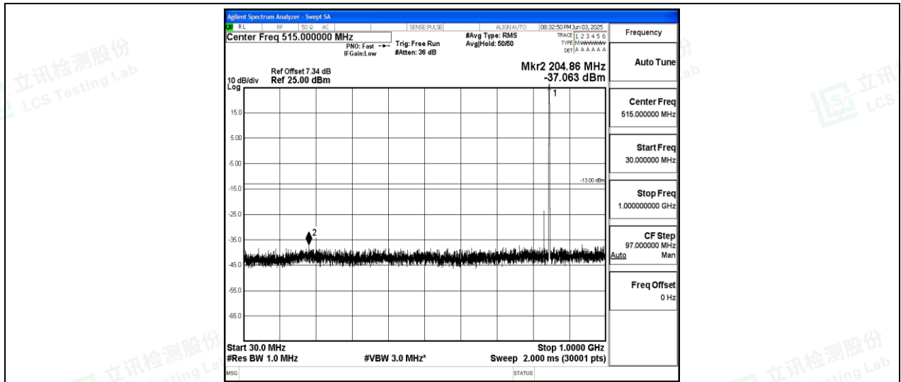
Band26-5MHz-16QAM-27015-1-0-High-30-1000--37.06-PASS
