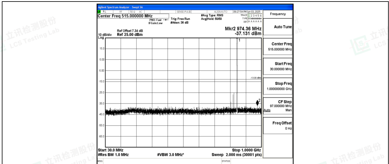
Band26-15MHz-QPSK-26965-1-0-High-30-1000--37.13-PASS
