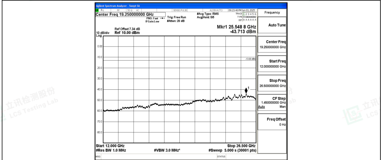
Band26-15MHz-16QAM-26865-1-0-Low-12000-26500--43.71-PASS
