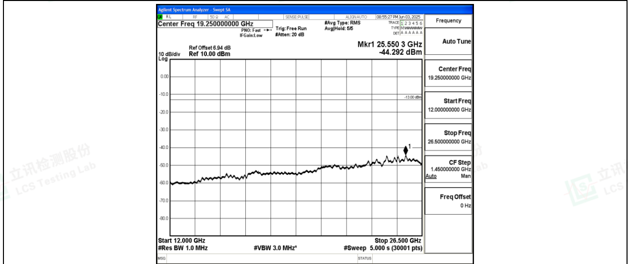
Band26-10MHz-16QAM-26840-1-0-Low-12000-26500--44.29-PASS
