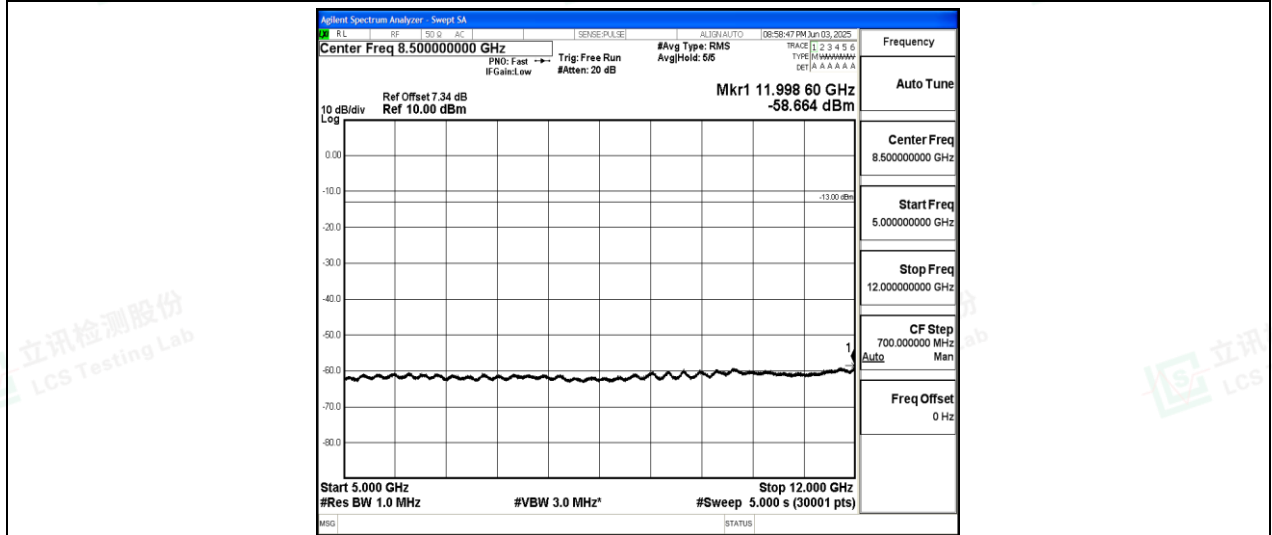
Band26-10MHz-16QAM-26915-1-0-Low-5000-12000--58.66-PASS
