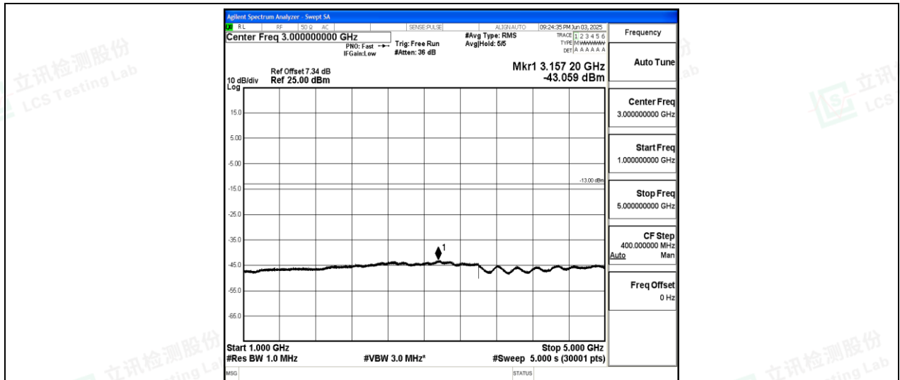
Band26-15MHz-QPSK-26915-1-0-Low-1000-5000--43.06-PASS
