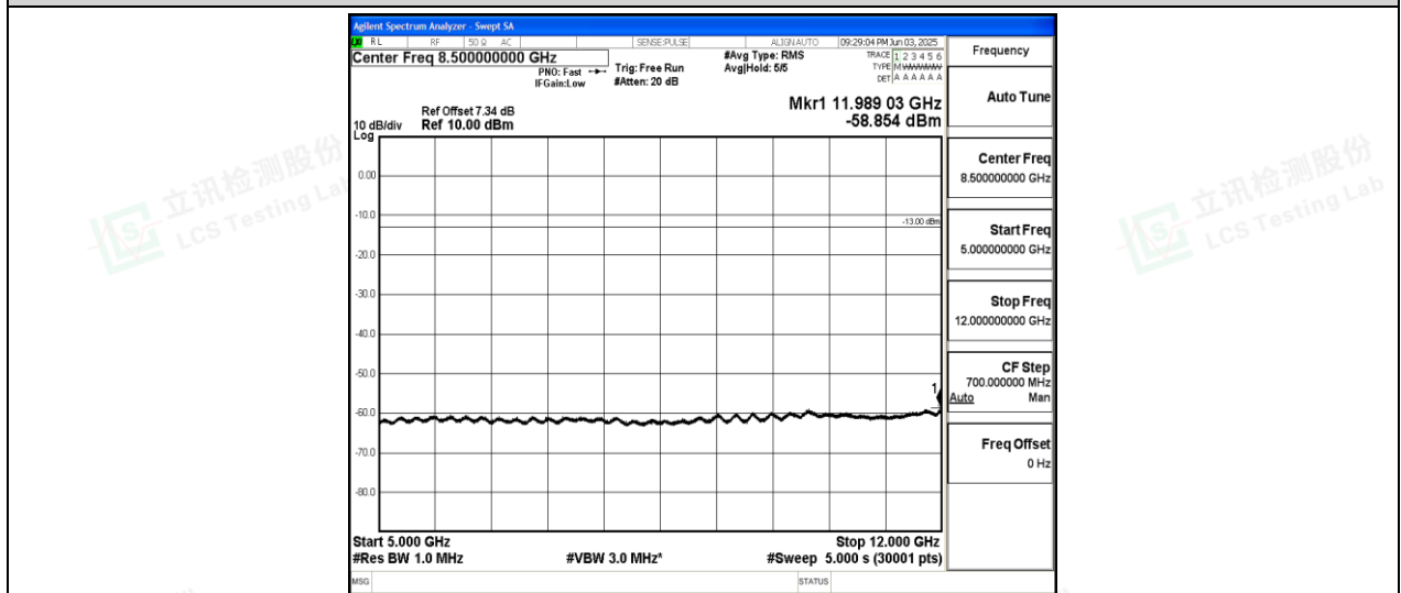
Band26-15MHz-QPSK-26965-1-0-High-5000-12000--58.85-PASS
