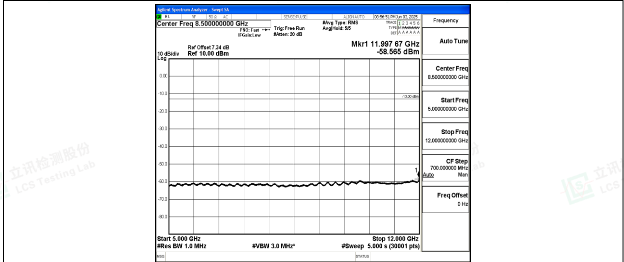
Band26-10MHz-QPSK-26915-1-0-Low-5000-12000--58.57-PASS
