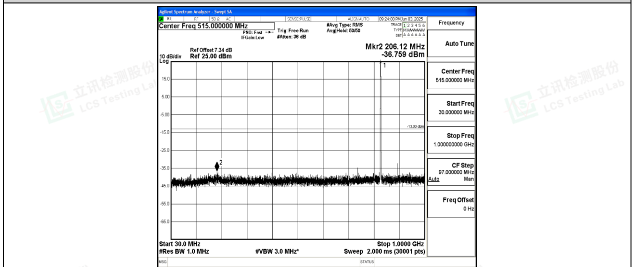
Band26-15MHz-QPSK-26915-1-0-Low-30-1000--36.76-PASS
