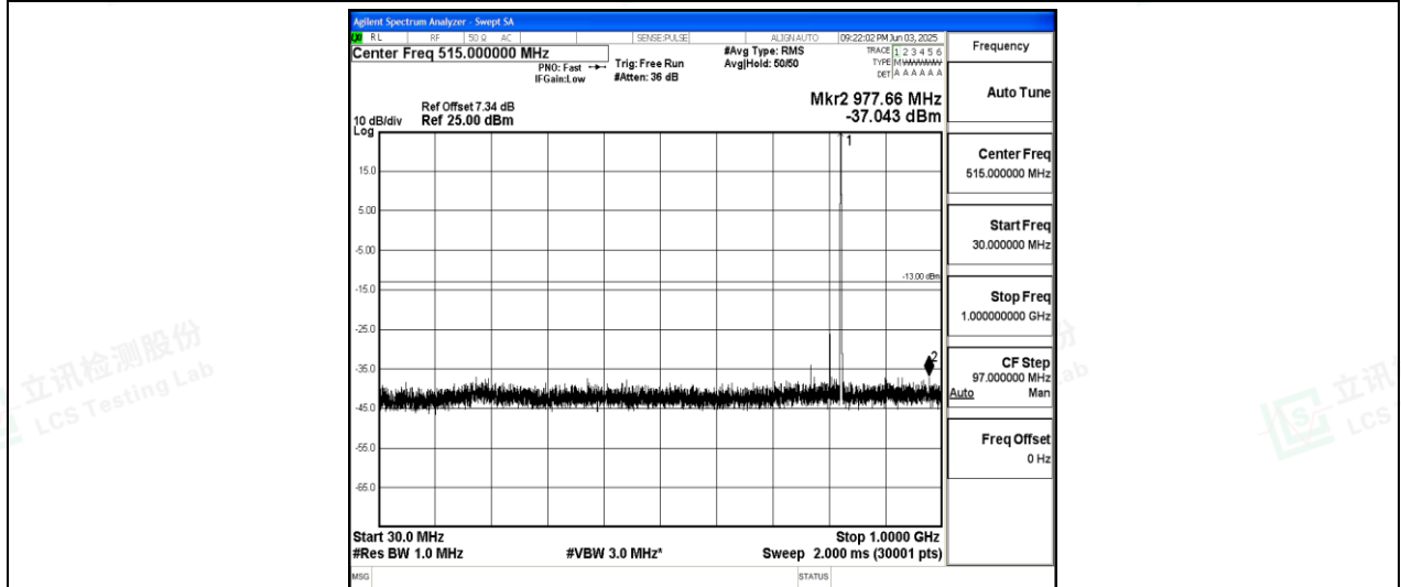
Band26-15MHz-16QAM-26865-1-0-Low-30-1000--37.04-PASS
