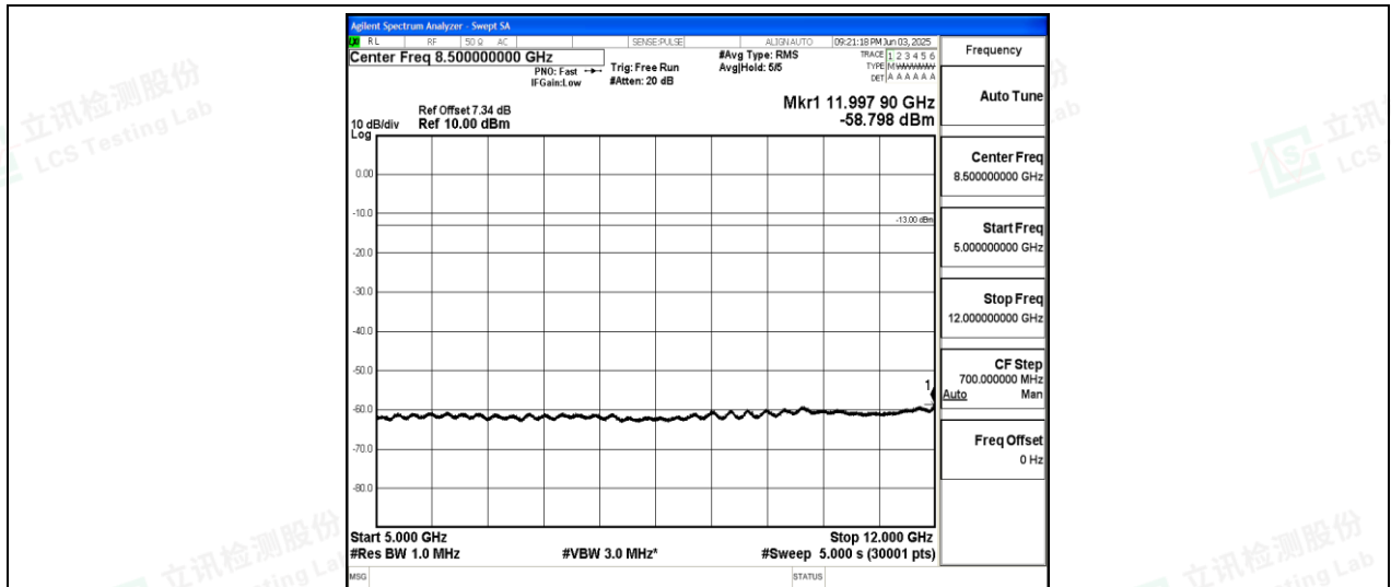
Band26-15MHz-QPSK-26865-1-0-Low-5000-12000--58.8-PASS
