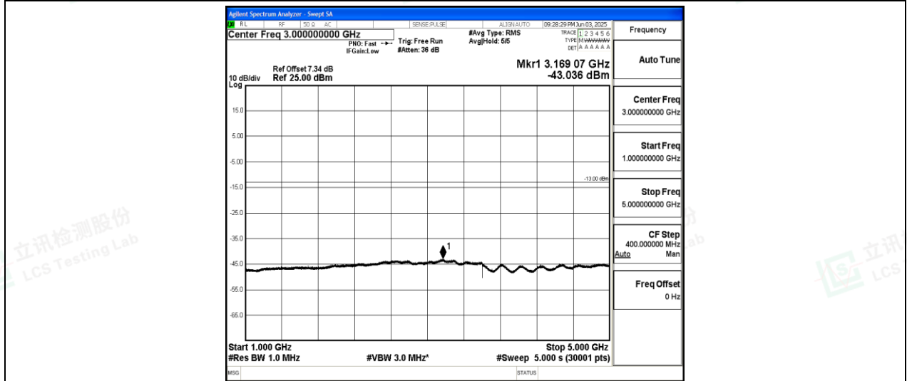
Band26-15MHz-QPSK-26965-1-0-High-1000-5000--43.04-PASS
