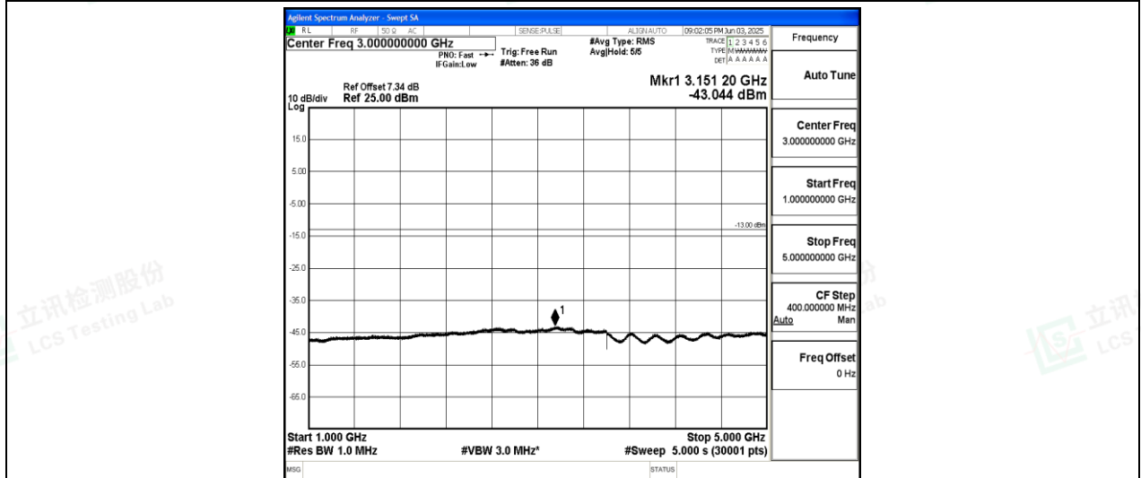
Band26-10MHz-16QAM-26990-1-0-High-1000-5000--43.04-PASS
