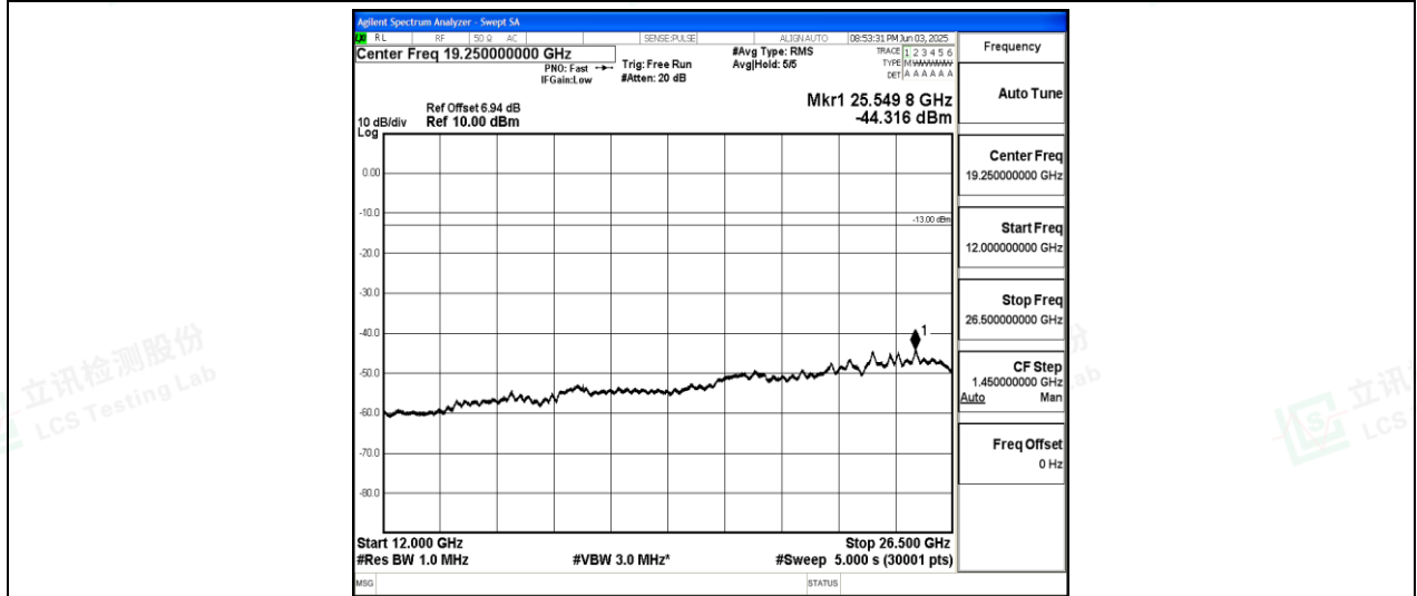
Band26-10MHz-QPSK-26840-1-0-Low-12000-26500--44.32-PASS
