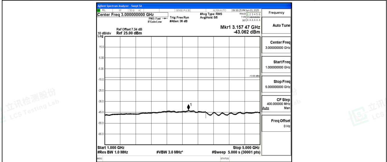
Band26-15MHz-16QAM-26965-1-0-High-1000-5000--43.06-PASS
