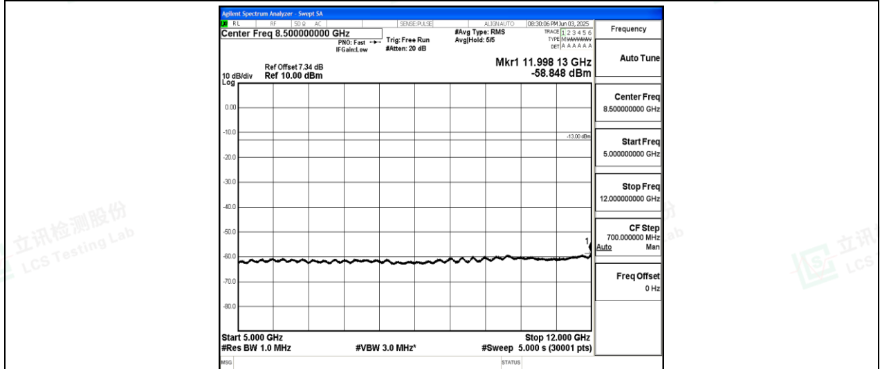
Band26-5MHz-16QAM-26915-1-0-Low-5000-12000--58.85-PASS
