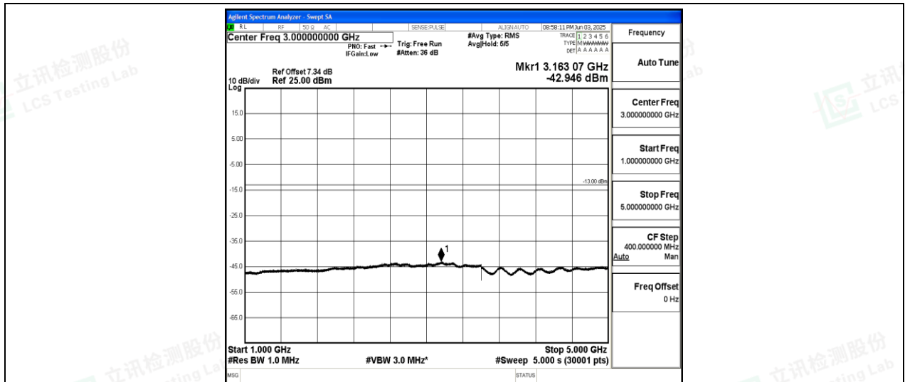
Band26-10MHz-16QAM-26915-1-0-Low-1000-5000--42.95-PASS
