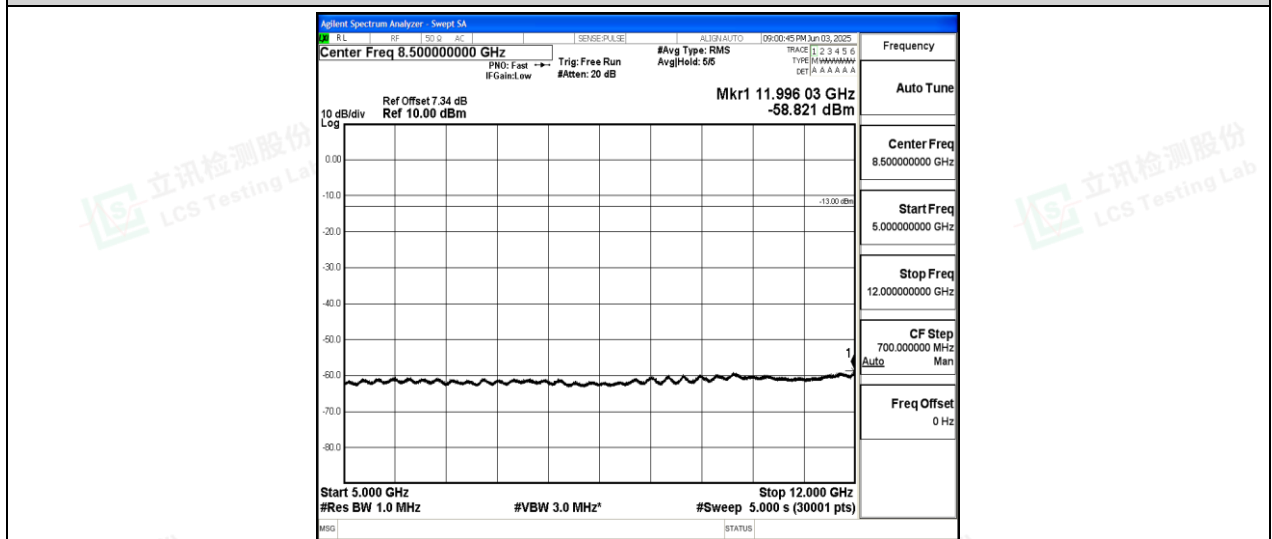
Band26-10MHz-QPSK-26990-1-0-High-5000-12000--58.82-PASS
