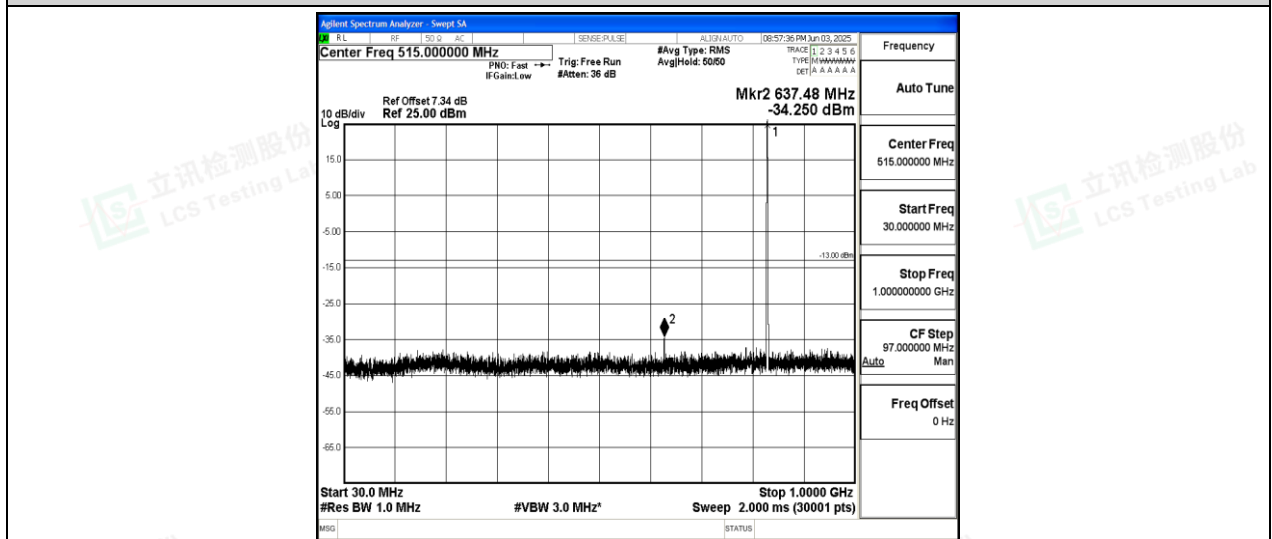
Band26-10MHz-16QAM-26915-1-0-Low-30-1000--34.25-PASS
