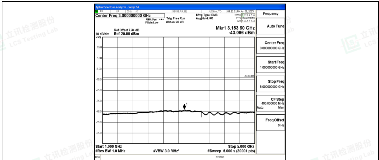
Band26-15MHz-16QAM-26915-1-0-Low-1000-5000--43.09-PASS
