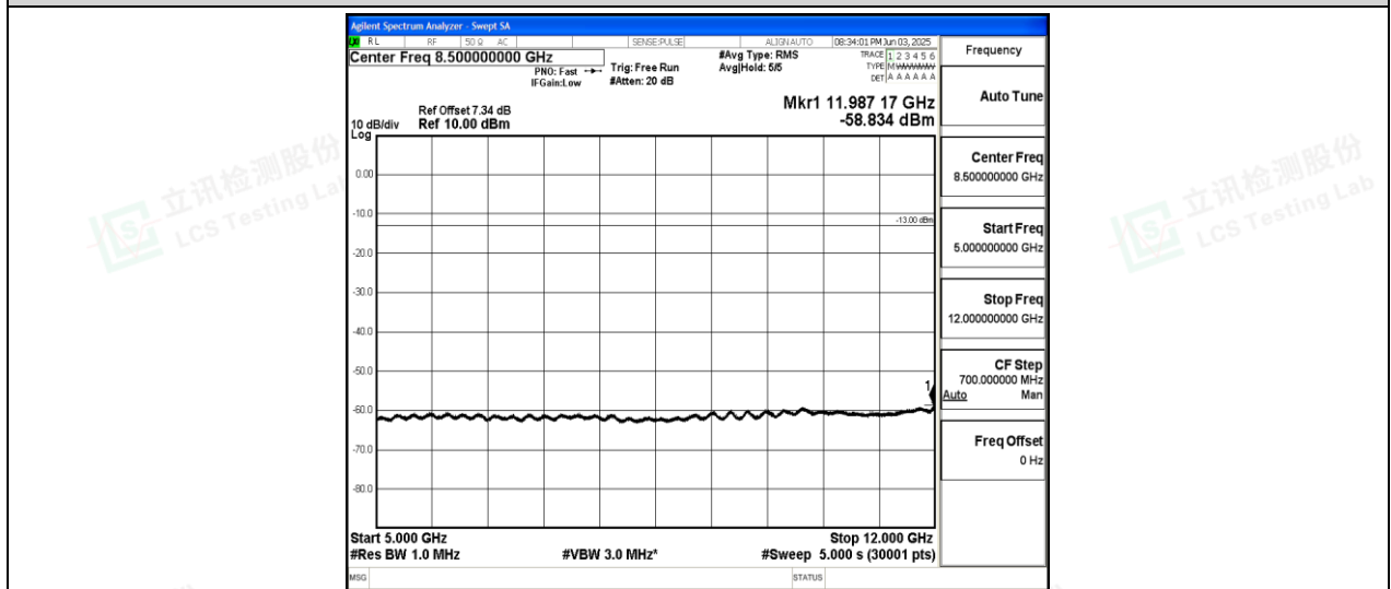
Band26-5MHz-16QAM-27015-1-0-High-5000-12000--58.83-PASS
