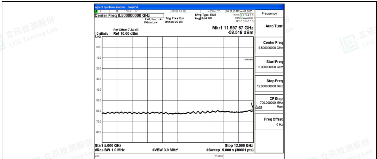
Band26-15MHz-16QAM-26865-1-0-Low-5000-12000--58.52-PASS
