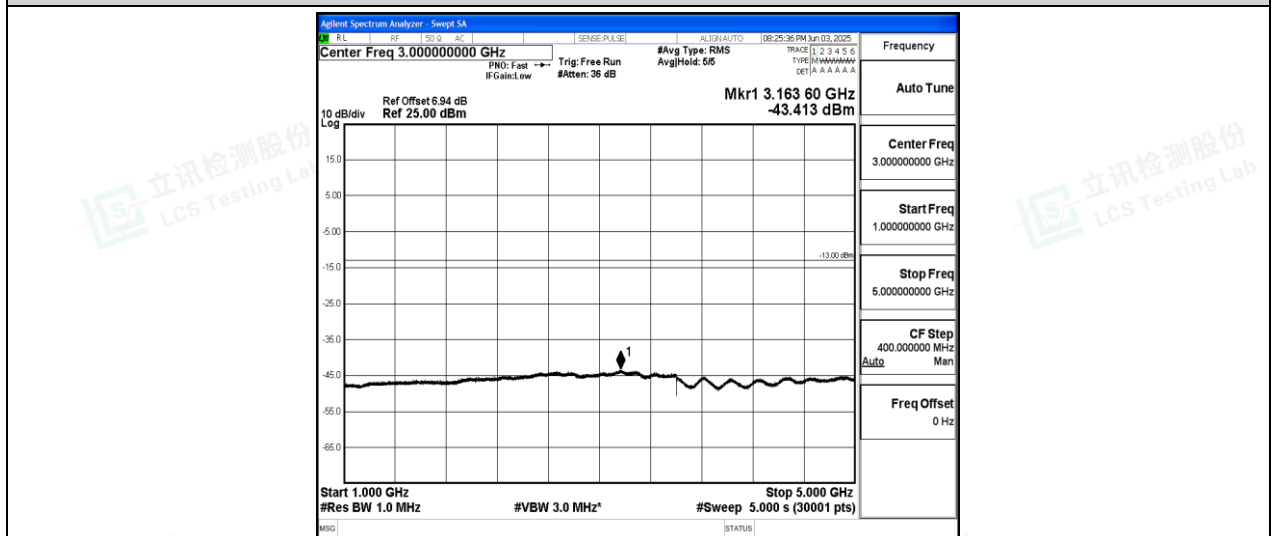
Band26-5MHz-16QAM-26815-1-0-Low-1000-5000--43.41-PASS
