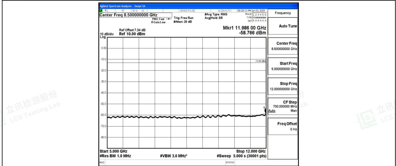
Band26-5MHz-QPSK-26915-1-0-Low-5000-12000--58.77-PASS
