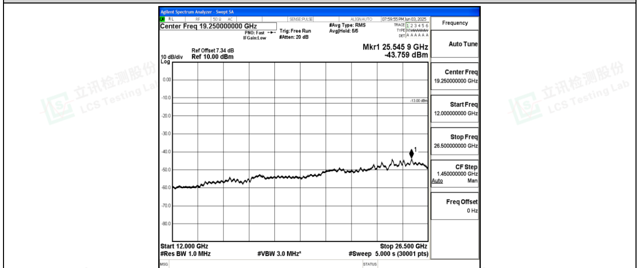
Band26-3MHz-16QAM-26915-1-0-Low-12000-26500--43.76-PASS
