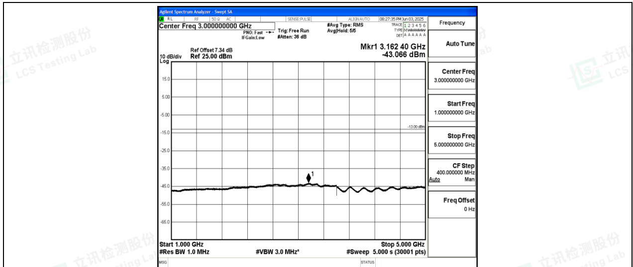
Band26-5MHz-QPSK-26915-1-0-Low-1000-5000--43.07-PASS
