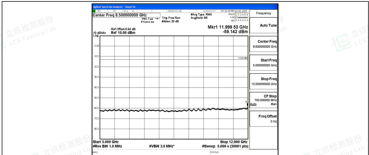
Band26-1.4MHz-QPSK-26797-1-0-Low-5000-12000--59.14-PASS
