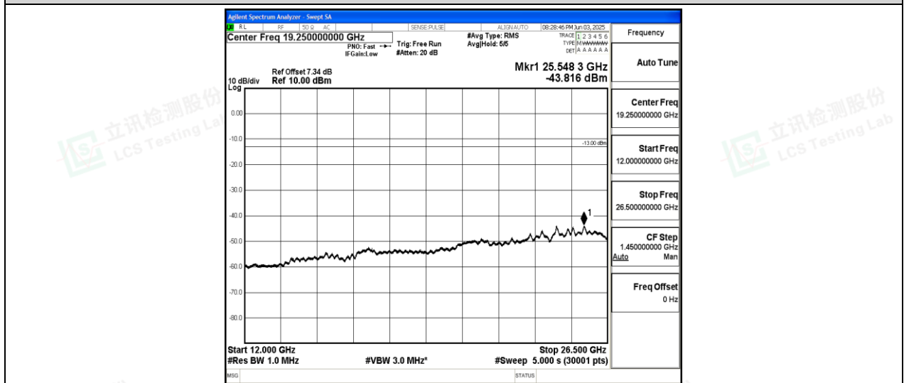
Band26-5MHz-QPSK-26915-1-0-Low-12000-26500--43.82-PASS
