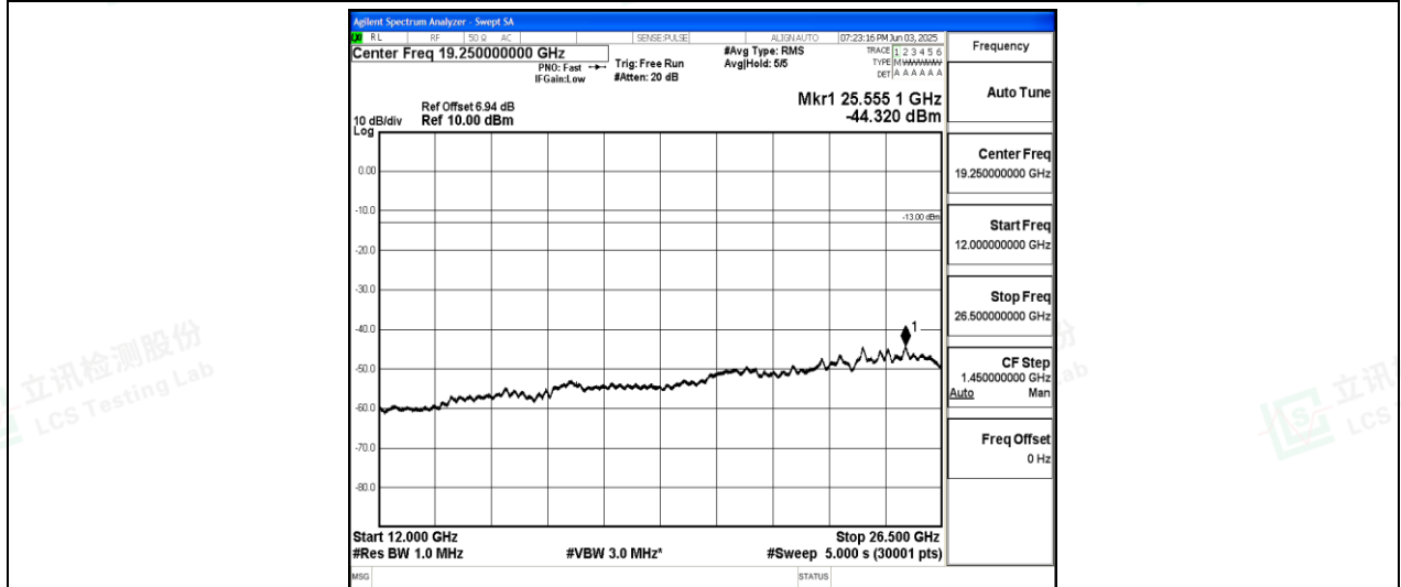
Band26-1.4MHz-QPSK-26797-1-0-Low-12000-26500--44.32-PASS
