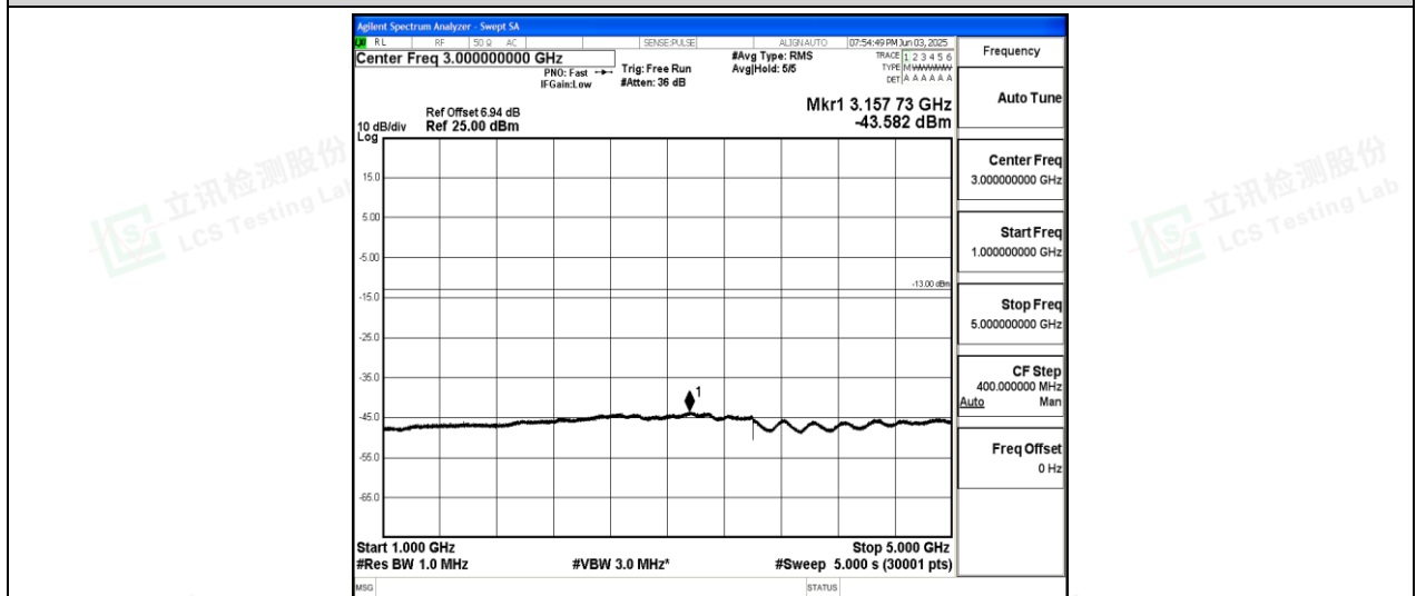
Band26-3MHz-16QAM-26805-1-0-Low-1000-5000--43.58-PASS
