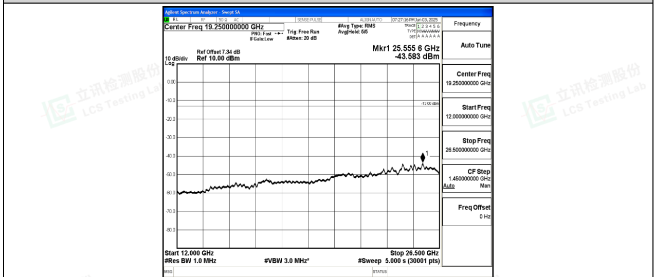
Band26-1.4MHz-QPSK-26915-1-0-Low-12000-26500--43.58-PASS
