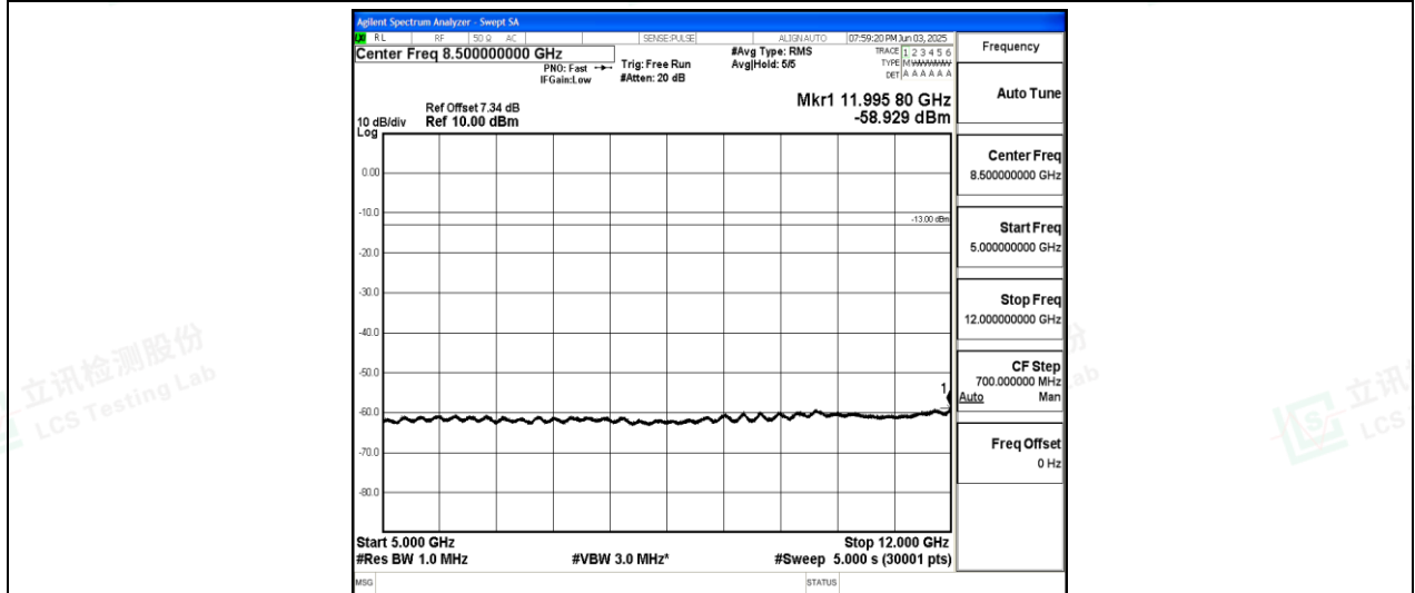
Band26-3MHz-16QAM-26915-1-0-Low-5000-12000--58.93-PASS
