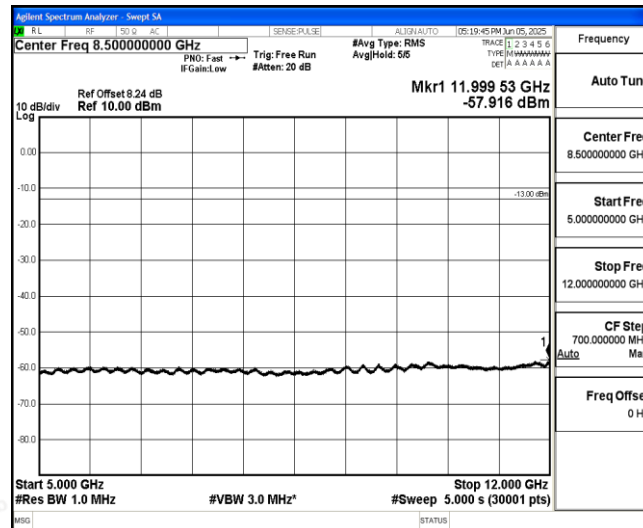
Band26-5MHz-QPSK-26715-1-0-Low-5000-12000--57.92-PASS
