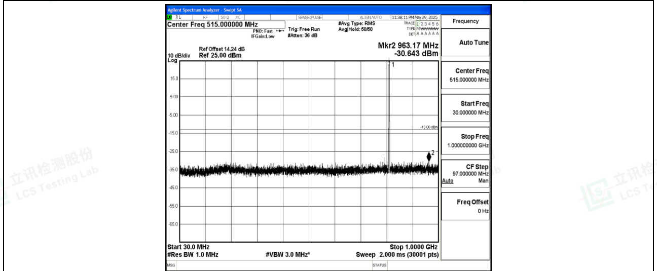
Band26-3MHz-16QAM-26705-1-0-Low-30-1000--30.64-PASS
