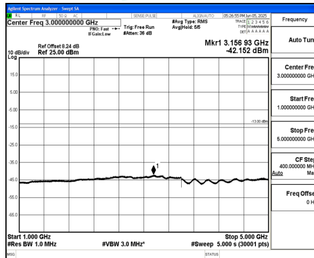
Band26-5MHz-QPSK-26785-1-0-High-1000-5000--42.15-PASS
