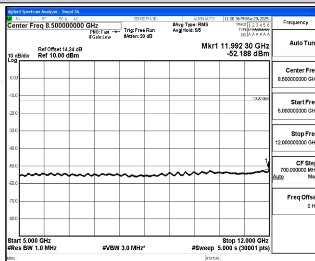
Band26-1.4MHz-16QAM-26783-1-0-High-5000-12000--52.19-PASS
