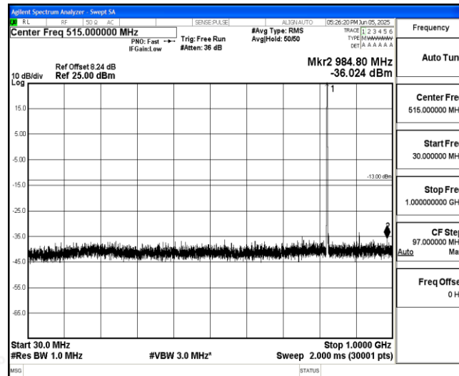
Band26-5MHz-QPSK-26785-1-0-High-30-1000--36.02-PASS
