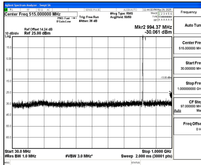
Band26-3MHz-QPSK-26775-1-0-High-30-1000--30.06-PASS
