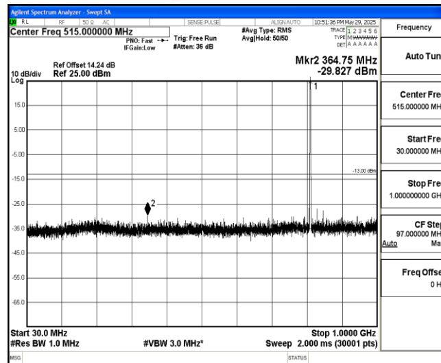
Band26-1.4MHz-16QAM-26697-1-0-Low-30-1000--29.83-PASS
