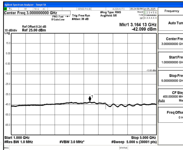
Band26-5MHz-16QAM-26740-1-0-Low-1000-5000--42.1-PASS
