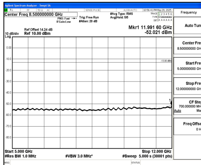
Band26-1.4MHz-16QAM-26740-1-0-Low-5000-12000--52.02-PASS
