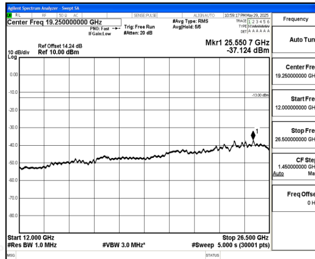
Band26-1.4MHz-QPSK-26783-1-0-High-12000-26500--37.12-PASS
