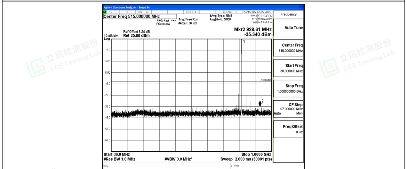
Band26-5MHz-16QAM-26740-1-0-Low-30-1000--35.34-PASS
