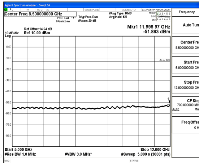
Band26-3MHz-QPSK-26705-1-0-Low-5000-12000--51.86-PASS
