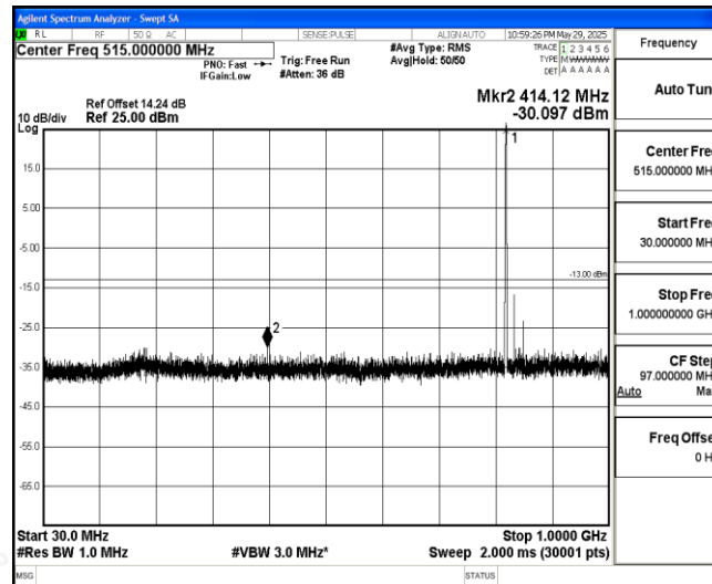
Band26-1.4MHz-16QAM-26783-1-0-High-30-1000--30.1-PASS
