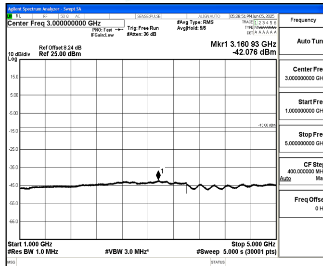
Band26-5MHz-16QAM-26785-1-0-High-1000-5000--42.08-PASS
