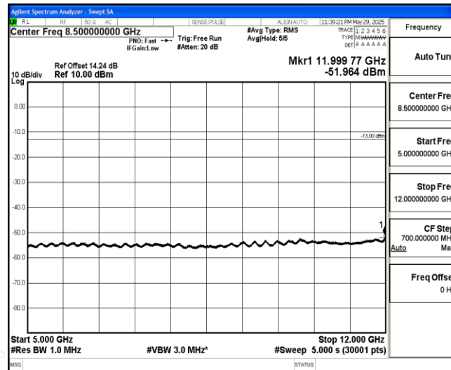
Band26-3MHz-16QAM-26705-1-0-Low-5000-12000--51.96-PASS
