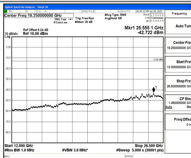
Band26-10MHz-16QAM-26740-1-0-Low-12000-26500--42.72-PASS
