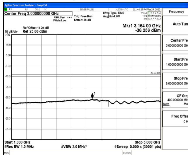
Band26-3MHz-16QAM-26775-1-0-High-1000-5000--36.26-PASS
