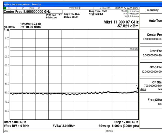
Band26-5MHz-16QAM-26740-1-0-Low-5000-12000--57.82-PASS
