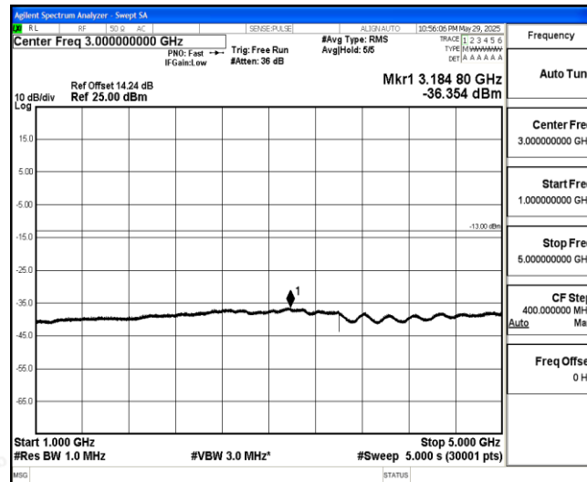
Band26-1.4MHz-16QAM-26740-1-0-Low-1000-5000--36.35-PASS
