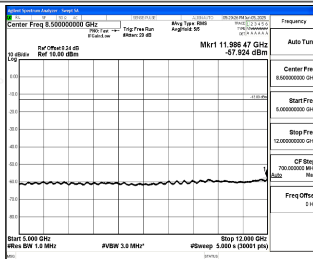
Band26-5MHz-16QAM-26785-1-0-High-5000-12000--57.92-PASS
