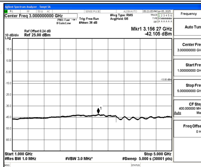
Band26-5MHz-16QAM-26715-1-0-Low-1000-5000--42.11-PASS
