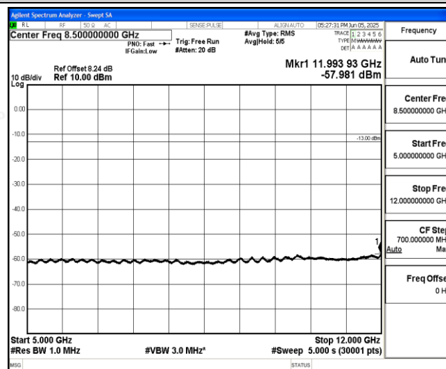
Band26-5MHz-QPSK-26785-1-0-High-5000-12000--57.98-PASS
