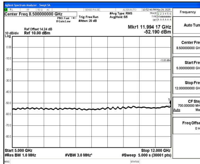
Band26-1.4MHz-16QAM-26697-1-0-Low-5000-12000--52.19-PASS
