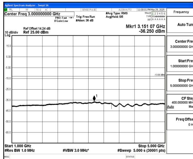
Band26-1.4MHz-16QAM-26783-1-0-High-1000-5000--36.25-PASS
