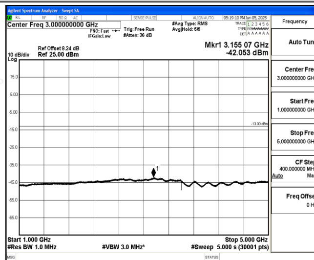
Band26-5MHz-QPSK-26715-1-0-Low-1000-5000--42.05-PASS
