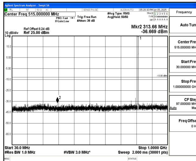
Band26-5MHz-16QAM-26715-1-0-Low-30-1000--36.67-PASS
