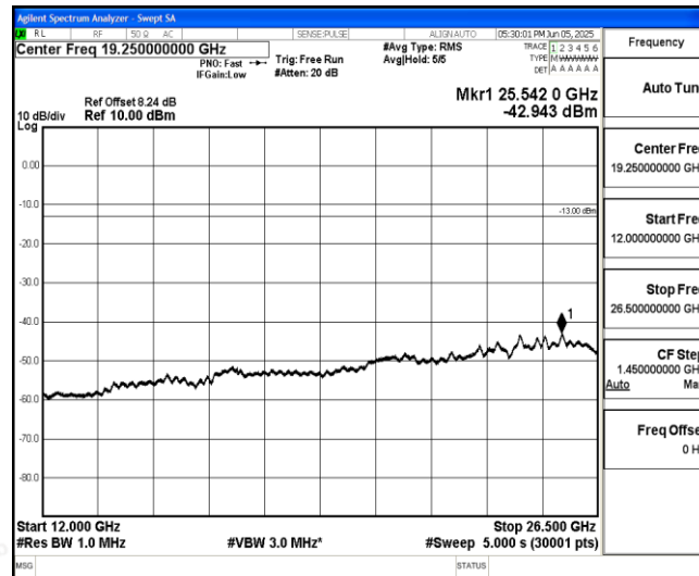
Band26-5MHz-16QAM-26785-1-0-High-12000-26500--42.94-PASS
