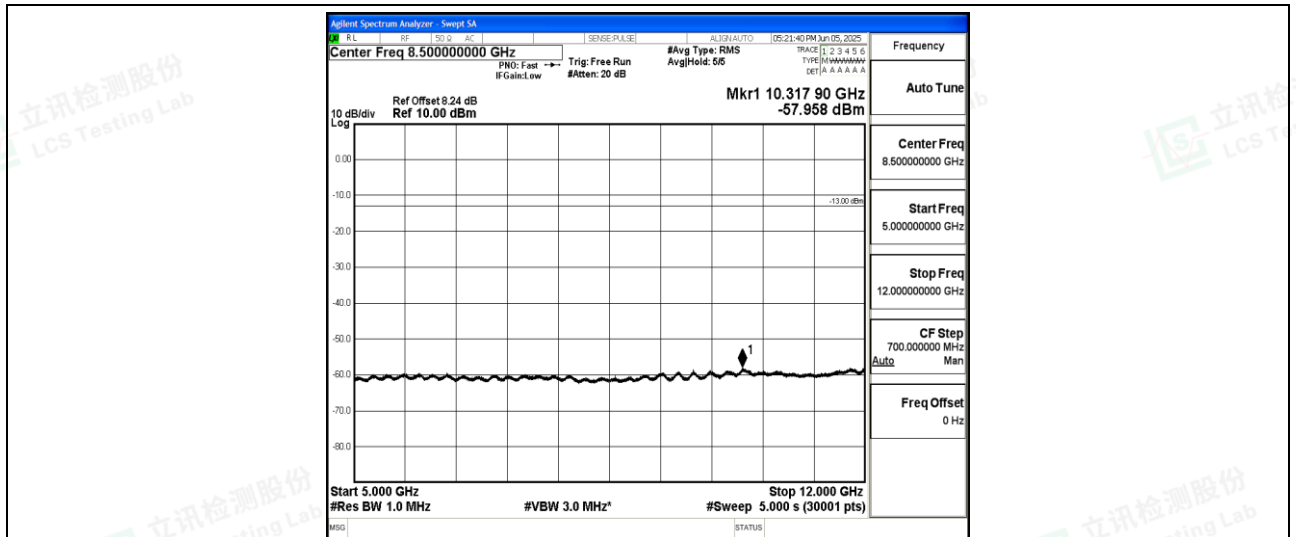
Band26-5MHz-16QAM-26715-1-0-Low-5000-12000--57.96-PASS
