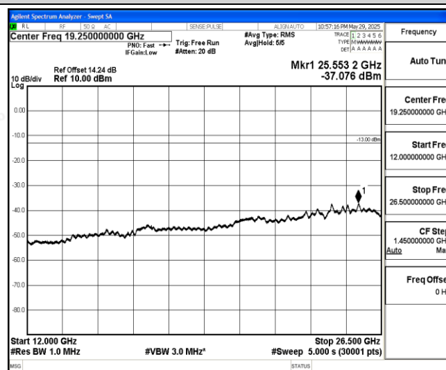
Band26-1.4MHz-16QAM-26740-1-0-Low-12000-26500--37.08-PASS
