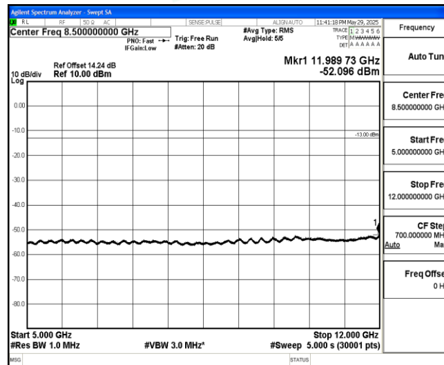
Band26-3MHz-QPSK-26740-1-0-Low-5000-12000--52.1-PASS
