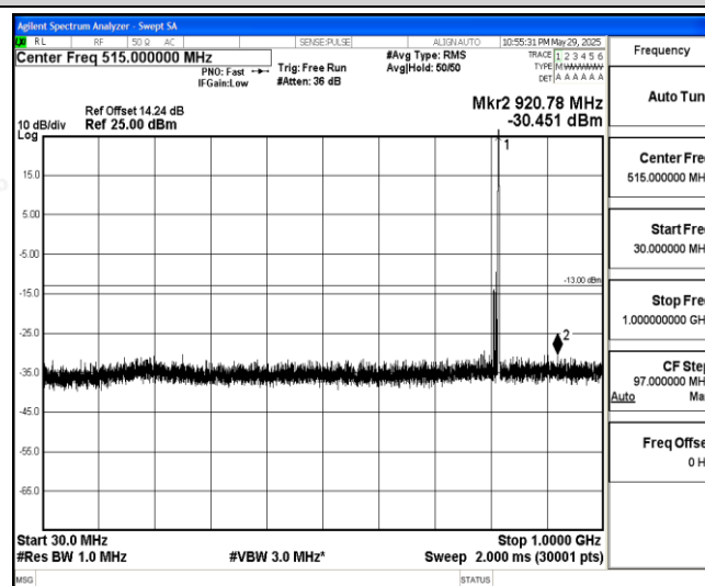
Band26-1.4MHz-16QAM-26740-1-0-Low-30-1000--30.45-PASS
