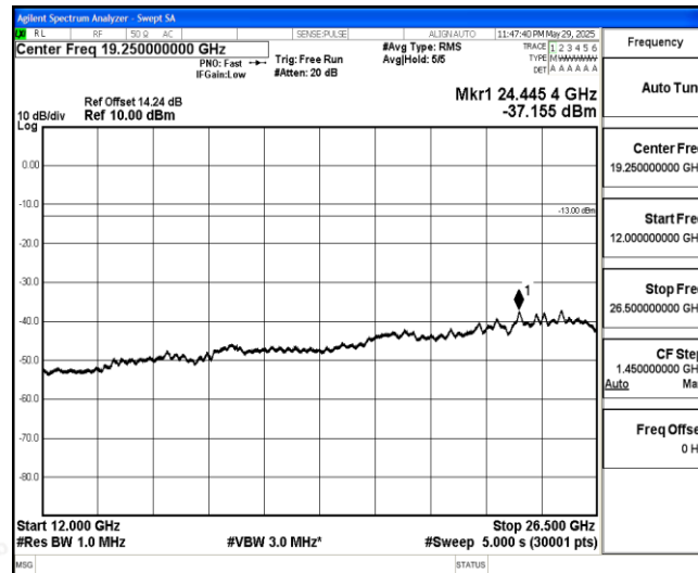
Band26-3MHz-16QAM-26775-1-0-High-12000-26500--37.16-PASS
