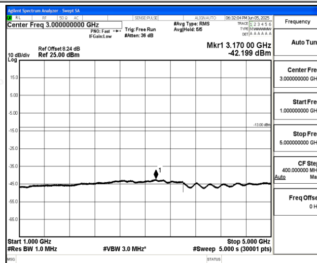
Band26-10MHz-QPSK-26740-1-0-Low-1000-5000--42.2-PASS
