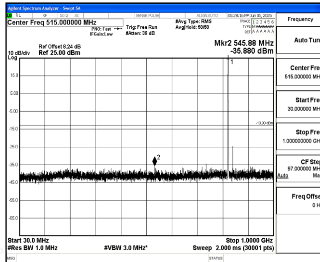
Band26-5MHz-16QAM-26785-1-0-High-30-1000--35.88-PASS
