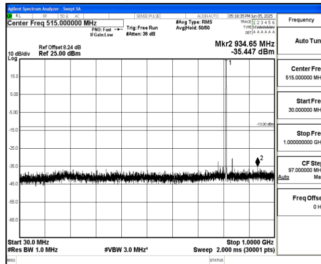
Band26-5MHz-QPSK-26715-1-0-Low-30-1000--35.45-PASS
