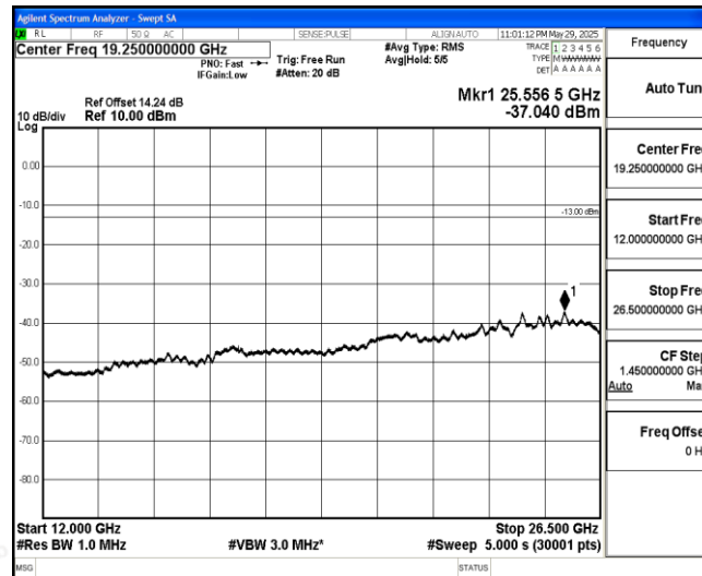
Band26-1.4MHz-16QAM-26783-1-0-High-12000-26500--37.04-PASS
