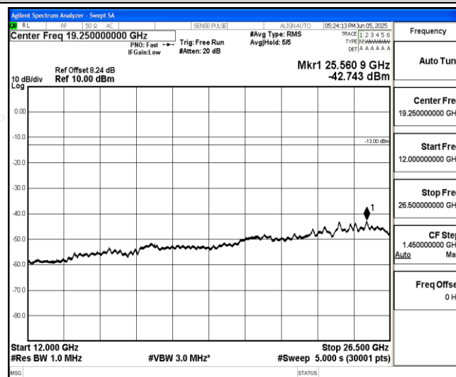
Band26-5MHz-QPSK-26740-1-0-Low-12000-26500--42.74-PASS
