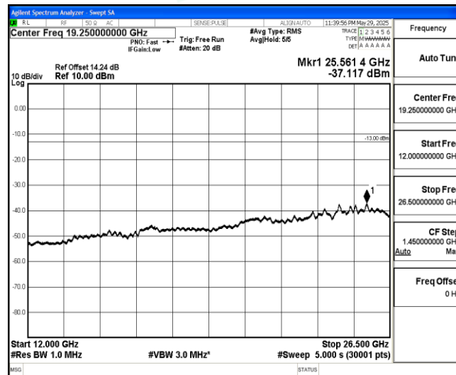
Band26-3MHz-16QAM-26705-1-0-Low-12000-26500--37.12-PASS
