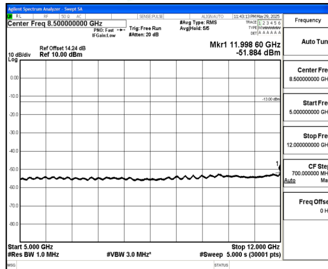
Band26-3MHz-16QAM-26740-1-0-Low-5000-12000--51.88-PASS
