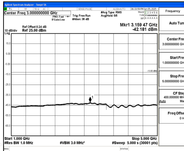
Band26-10MHz-16QAM-26740-1-0-Low-1000-5000--42.18-PASS
