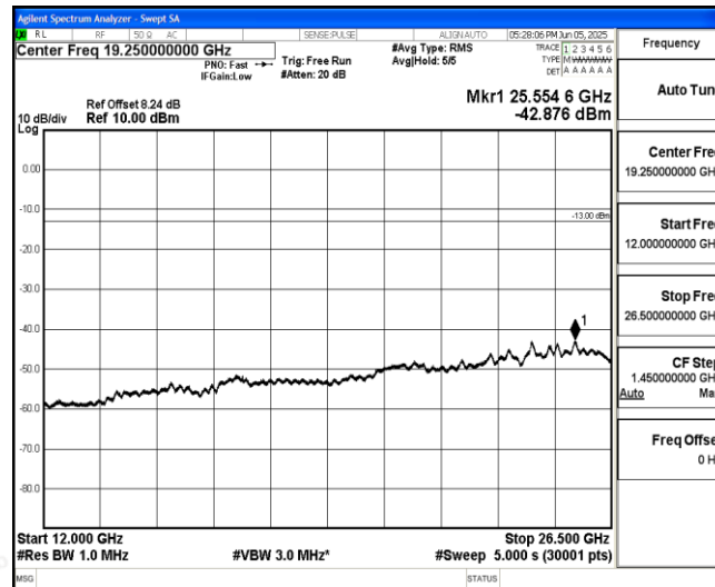
Band26-5MHz-QPSK-26785-1-0-High-12000-26500--42.88-PASS
