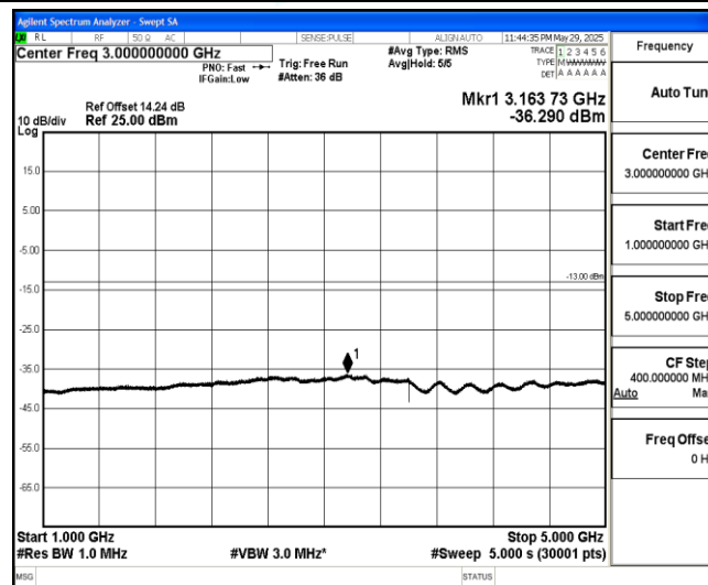
Band26-3MHz-QPSK-26775-1-0-High-1000-5000--36.29-PASS
