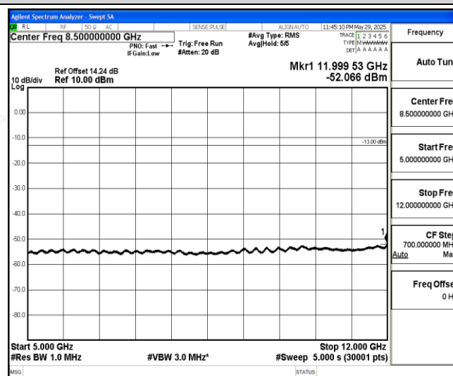
Band26-3MHz-QPSK-26775-1-0-High-5000-12000--52.07-PASS
