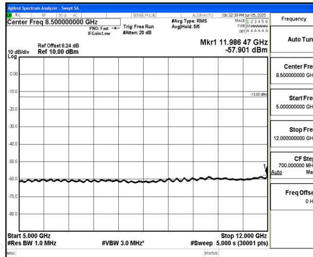
Band26-10MHz-QPSK-26740-1-0-Low-5000-12000--57.9-PASS
