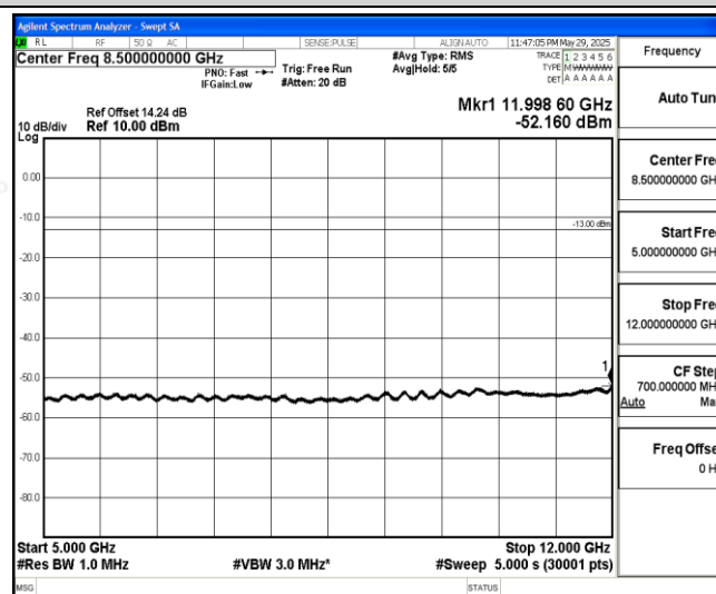
Band26-3MHz-16QAM-26775-1-0-High-5000-12000--52.16-PASS
