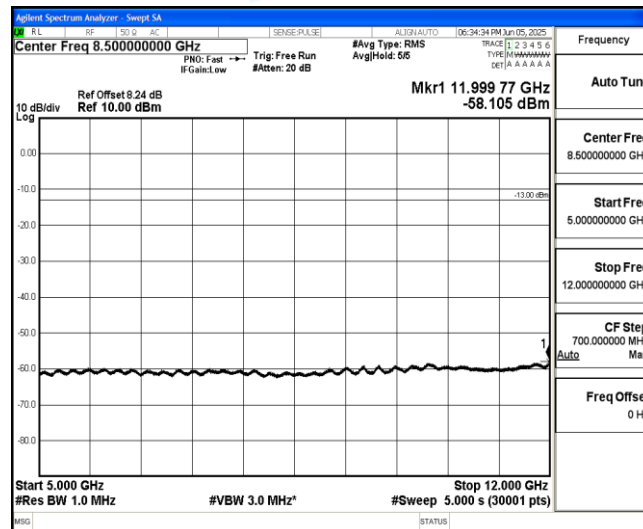
Band26-10MHz-16QAM-26740-1-0-Low-5000-12000--58.11-PASS
