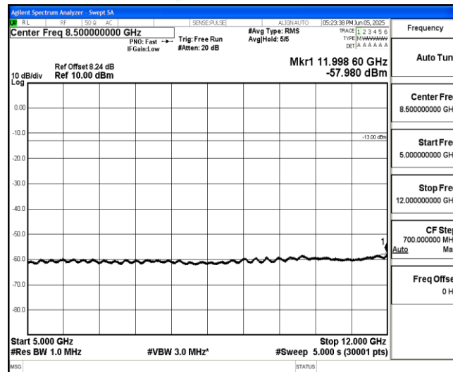
Band26-5MHz-QPSK-26740-1-0-Low-5000-12000--57.98-PASS
