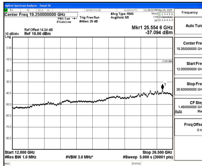
Band26-3MHz-QPSK-26705-1-0-Low-12000-26500--37.09-PASS
