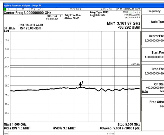
Band26-1.4MHz-16QAM-26697-1-0-Low-1000-5000--36.29-PASS
