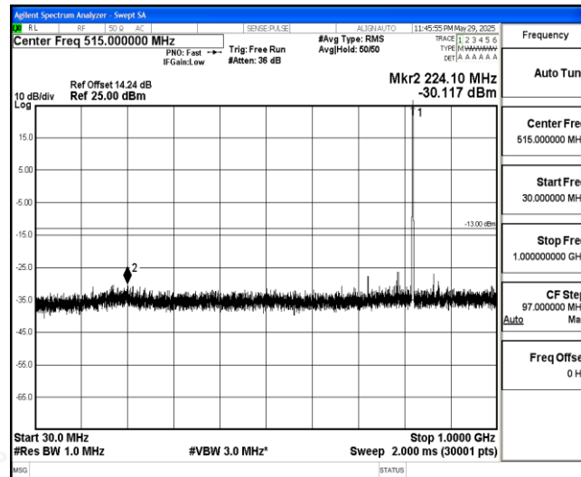
Band26-3MHz-16QAM-26775-1-0-High-30-1000--30.12-PASS
