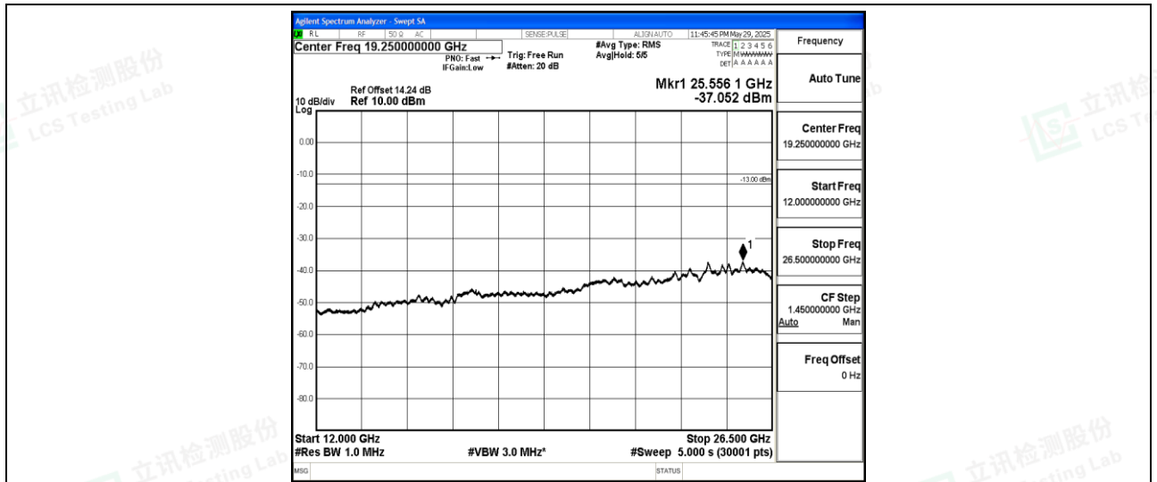
Band26-3MHz-QPSK-26775-1-0-High-12000-26500--37.05-PASS
