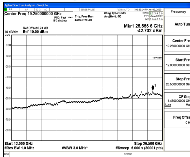
Band26-10MHz-QPSK-26740-1-0-Low-12000-26500--42.7-PASS
