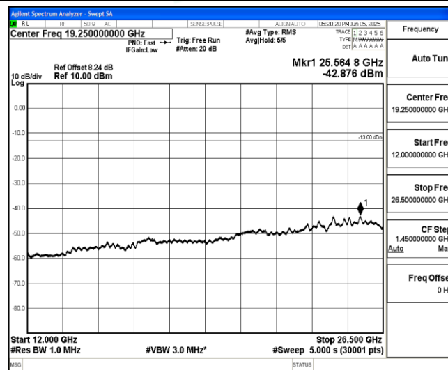
Band26-5MHz-QPSK-26715-1-0-Low-12000-26500--42.88-PASS
