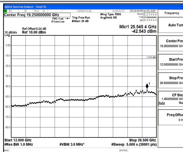
Band26-5MHz-16QAM-26740-1-0-Low-12000-26500--42.54-PASS
