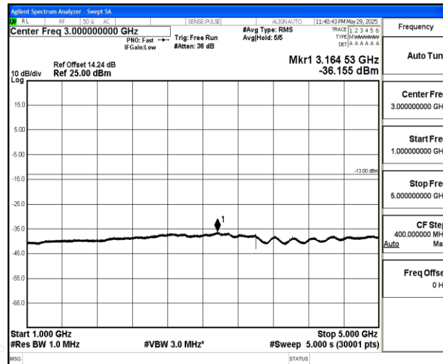
Band26-3MHz-QPSK-26740-1-0-Low-1000-5000--36.16-PASS
