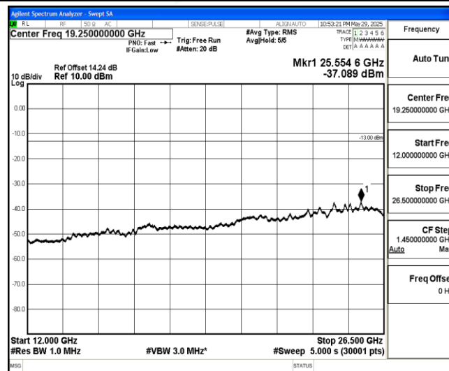
Band26-1.4MHz-16QAM-26697-1-0-Low-12000-26500--37.09-PASS
