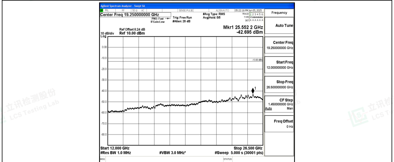
Band26-5MHz-16QAM-26715-1-0-Low-12000-26500--42.7-PASS
