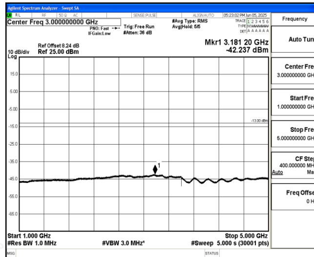
Band26-5MHz-QPSK-26740-1-0-Low-1000-5000--42.24-PASS
