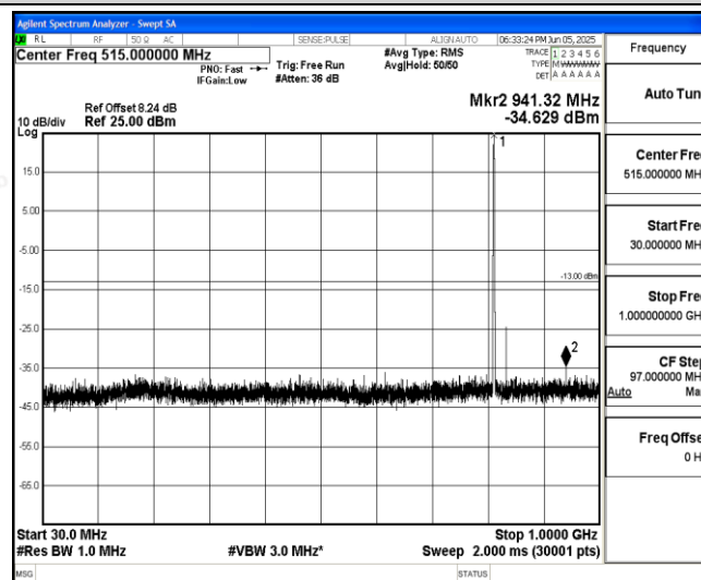
Band26-10MHz-16QAM-26740-1-0-Low-30-1000--34.63-PASS
