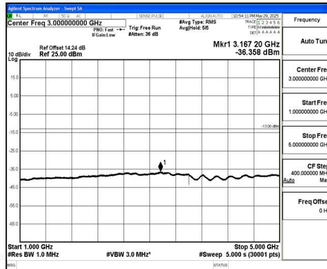
Band26-1.4MHz-QPSK-26740-1-0-Low-1000-5000--36.36-PASS
