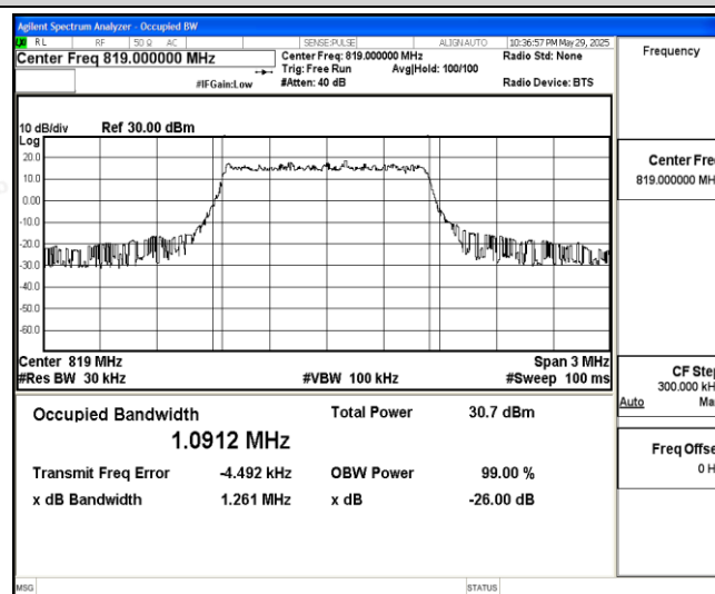
Band26-1.4MHz-16QAM-26740-6-0-Low-1.0912-1.261-PASS
