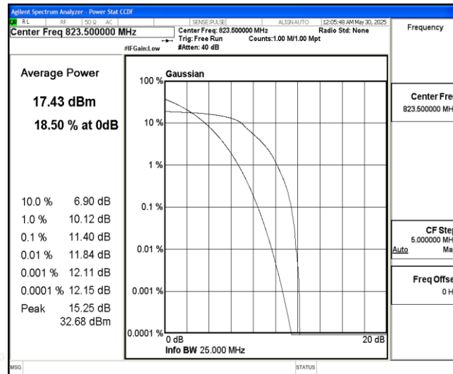
Band26-5MHz-16QAM-26785-6-0-High-11.40-&lt;=13-PASS
