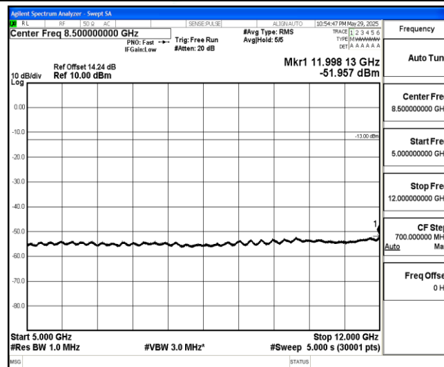
Band26-1.4MHz-QPSK-26740-1-0-Low-5000-12000--51.96-PASS
