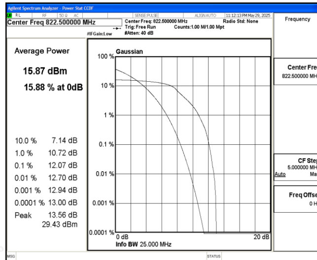
Band26-3MHz-16QAM-26775-6-0-High-12.07-&lt;=13-PASS
