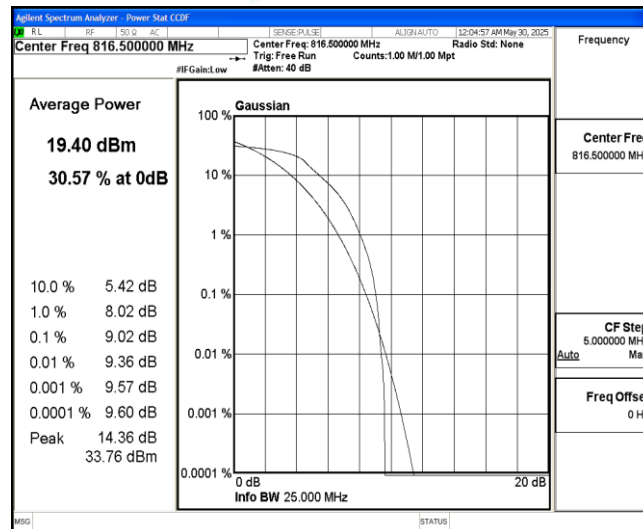
Band26-5MHz-QPSK-26715-6-0-Low-9.02-&lt;=13-PASS
