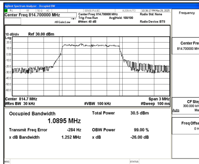
Band26-1.4MHz-16QAM-26697-6-0-Low-1.0895-1.252-PASS
