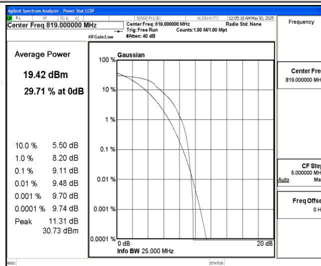
Band26-5MHz-QPSK-26740-6-0-Low-9.11-&lt;=13-PASS
