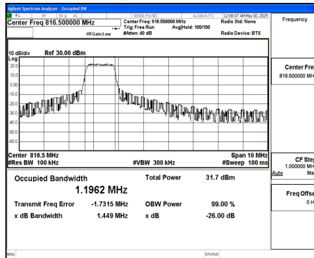
Band26-5MHz-QPSK-26715-6-0-Low-1.1962-1.449-PASS
