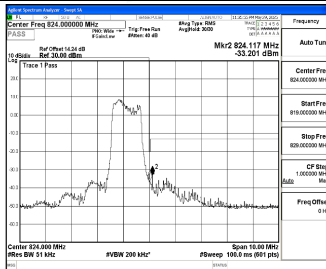
Band26-3MHz-QPSK-26775-6-0-High--36.41,-33.20-PASS
