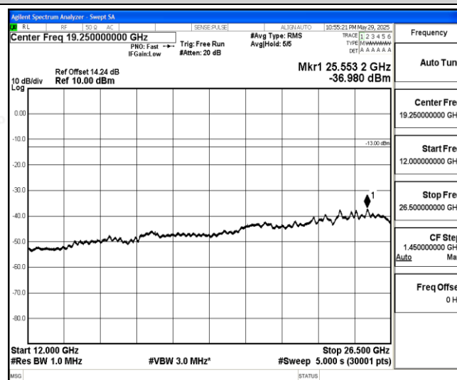
Band26-1.4MHz-QPSK-26740-1-0-Low-12000-26500--36.98-PASS
