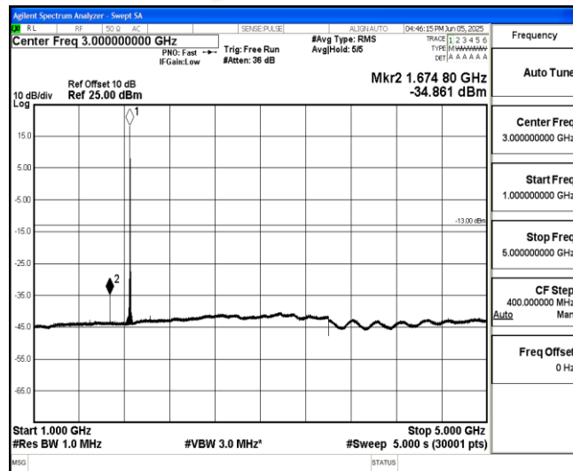
Band25-20MHz-16QAM-26140-1-0-Low-1000-5000--34.86-PASS
