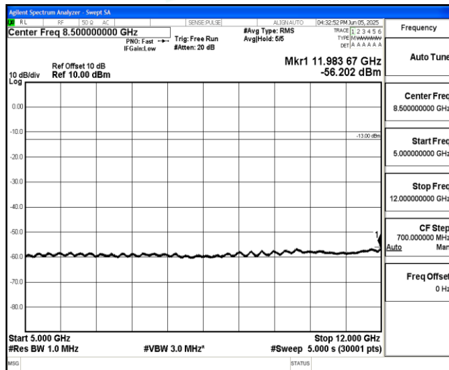
Band25-15MHz-16QAM-26615-1-0-High-5000-12000--56.2-PASS
