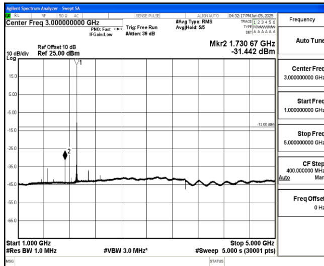
Band25-15MHz-16QAM-26615-1-0-High-1000-5000--31.44-PASS
