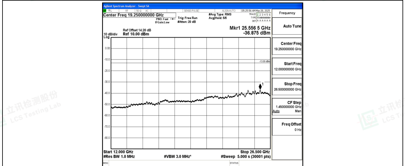
Band12-5MHz-16QAM-23095-1-0-Low-12000-26500--36.88-PASS
