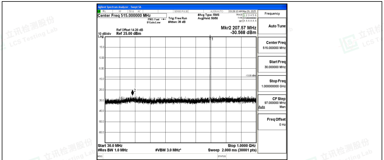
Band12-10MHz-QPSK-23095-1-0-Low-30-1000--30.57-PASS
