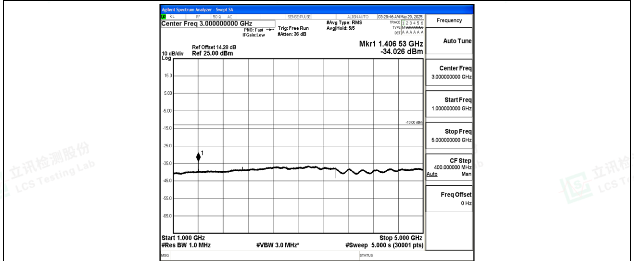
Band12-10MHz-QPSK-23095-1-0-Low-1000-5000--34.03-PASS
