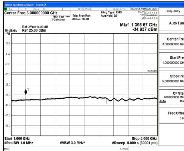
Band12-5MHz-16QAM-23035-1-0-Low-1000-5000--34.94-PASS
