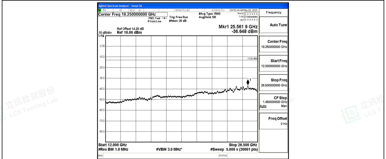
Band12-3MHz-QPSK-23025-1-0-Low-12000-26500--36.65-PASS
