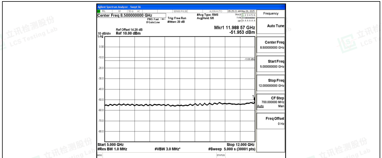
Band12-5MHz-16QAM-23095-1-0-Low-5000-12000--51.95-PASS
