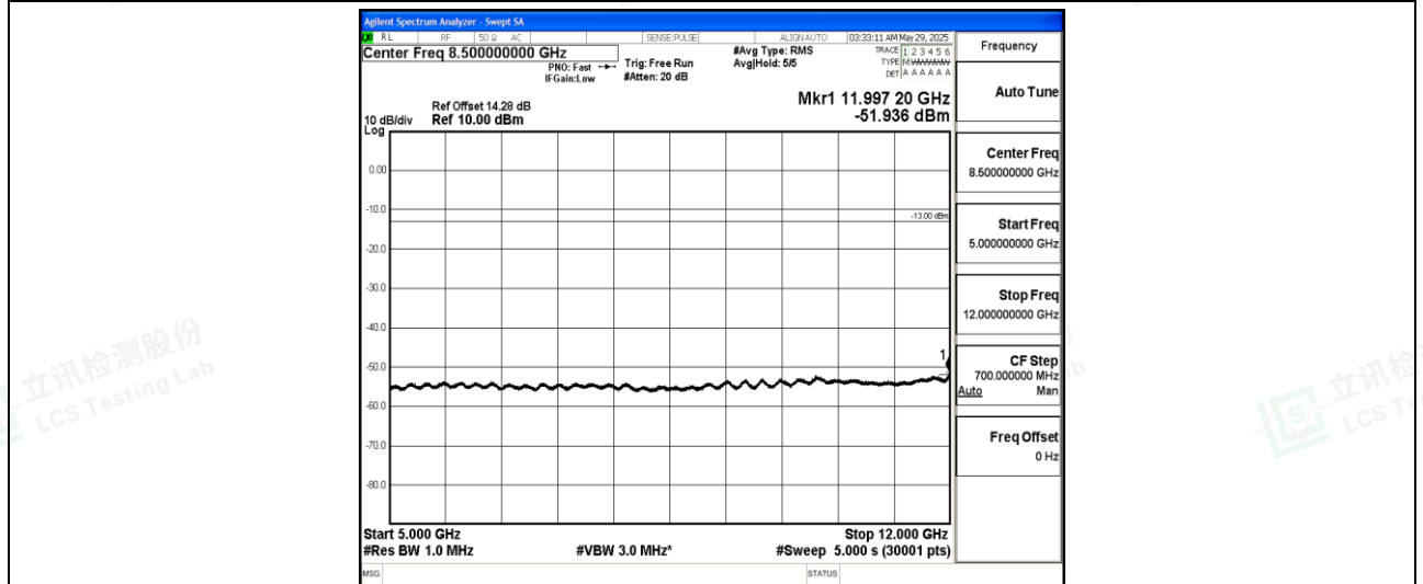
Band12-10MHz-QPSK-23130-1-0-High-5000-12000--51.94-PASS
