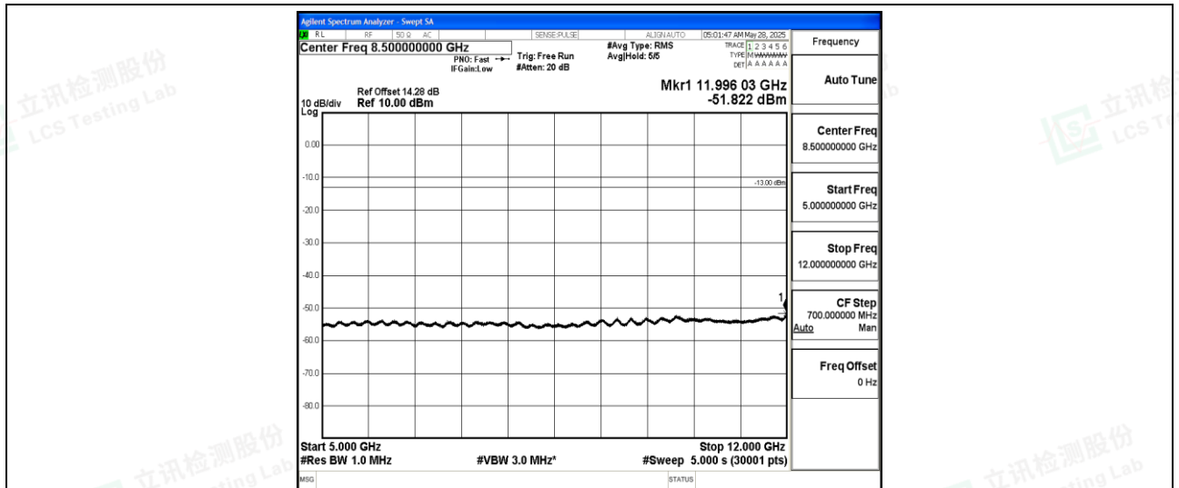
Band12-3MHz-16QAM-23165-1-0-High-5000-12000--51.82-PASS
