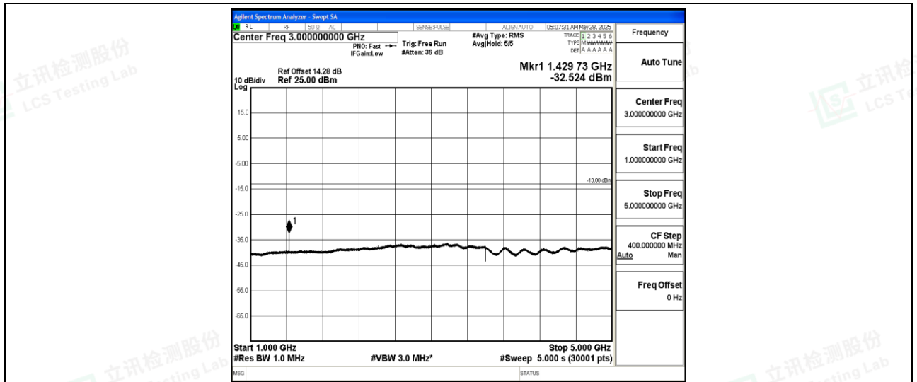
Band12-1.4MHz-16QAM-23173-1-0-High-1000-5000--32.52-PASS
