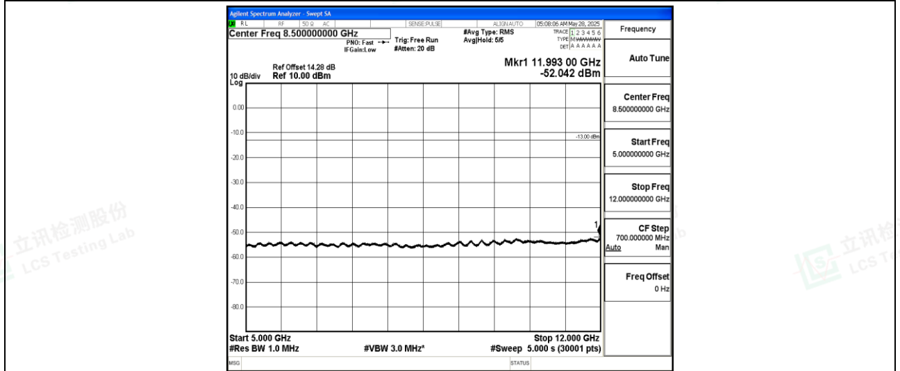
Band12-1.4MHz-16QAM-23173-1-0-High-5000-12000--52.04-PASS
