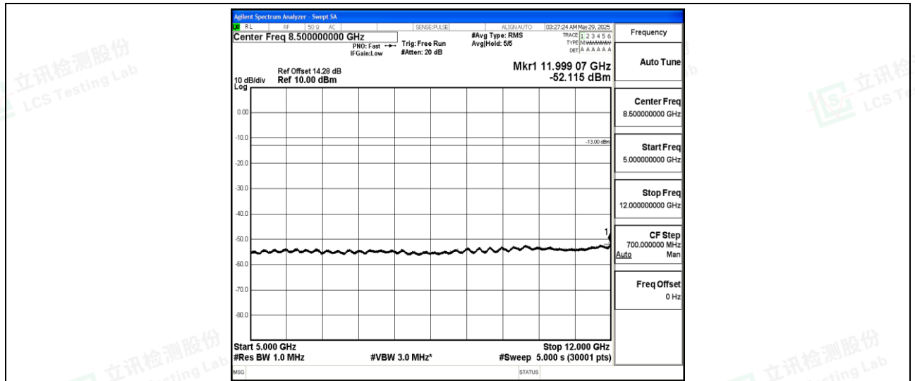
Band12-10MHz-16QAM-23060-1-0-Low-5000-12000--52.12-PASS
