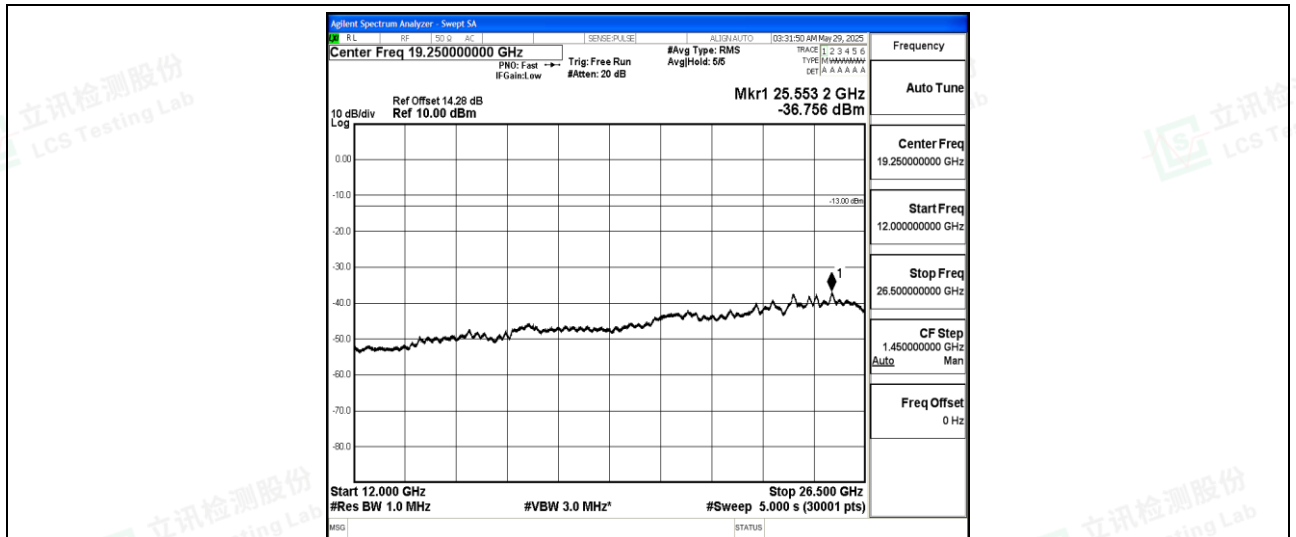
Band12-10MHz-16QAM-23095-1-0-Low-12000-26500--36.76-PASS
