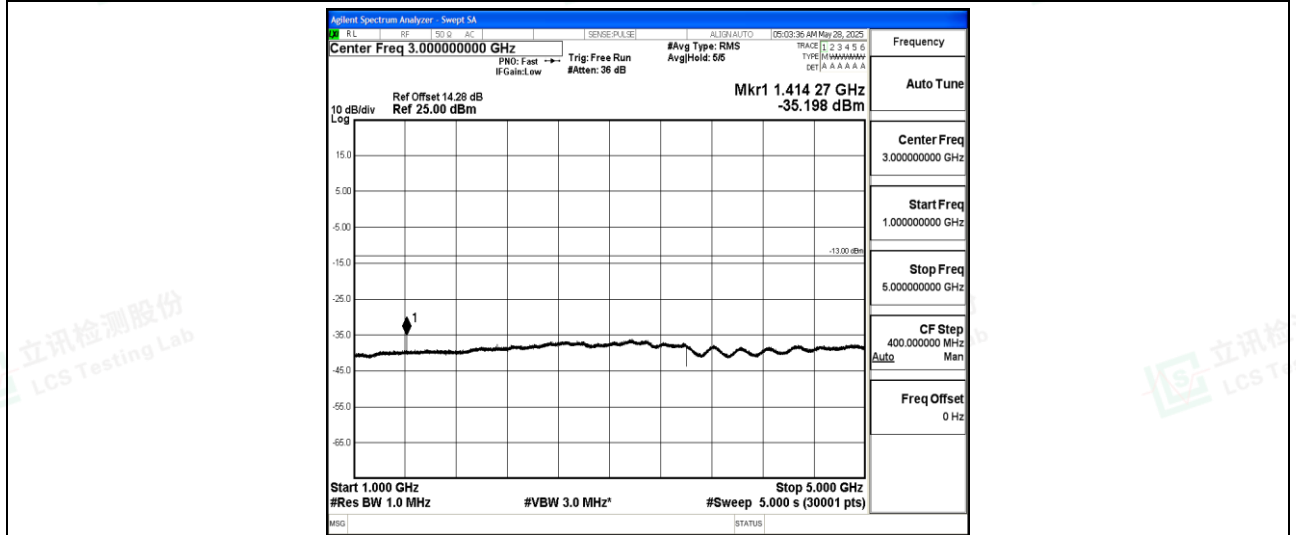
Band12-1.4MHz-16QAM-23095-1-0-Low-1000-5000--35.2-PASS
