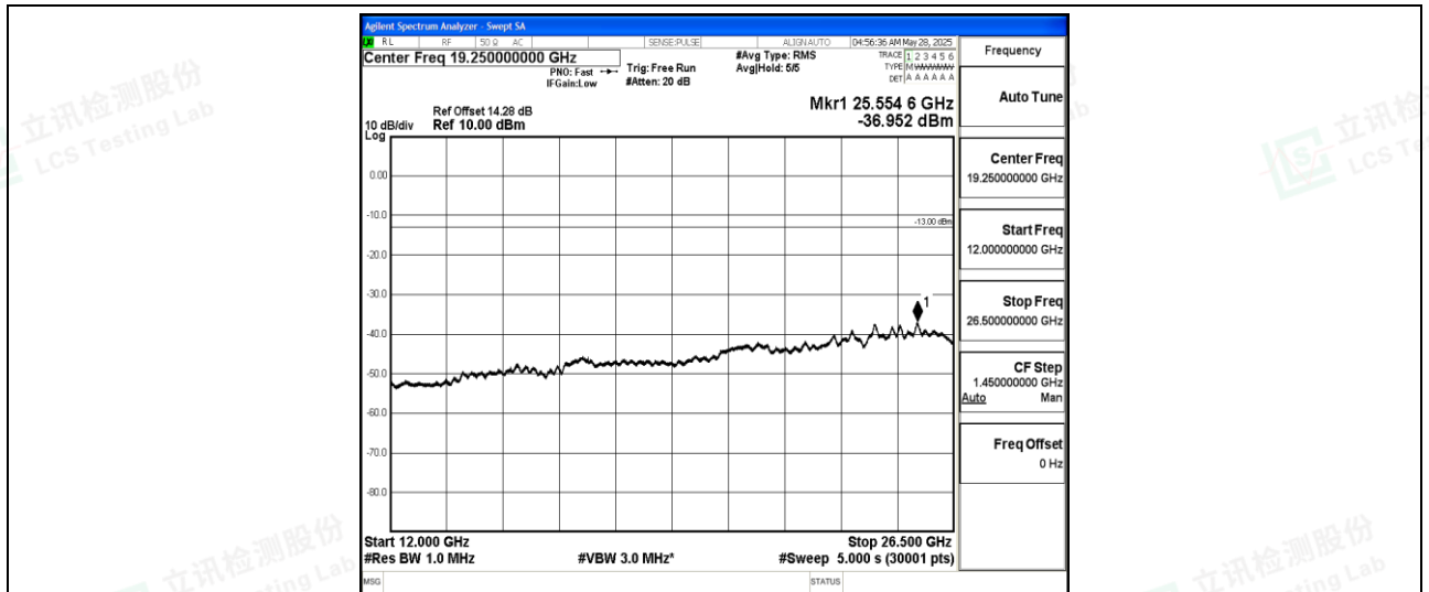
Band12-3MHz-QPSK-23095-1-0-Low-12000-26500--36.95-PASS
