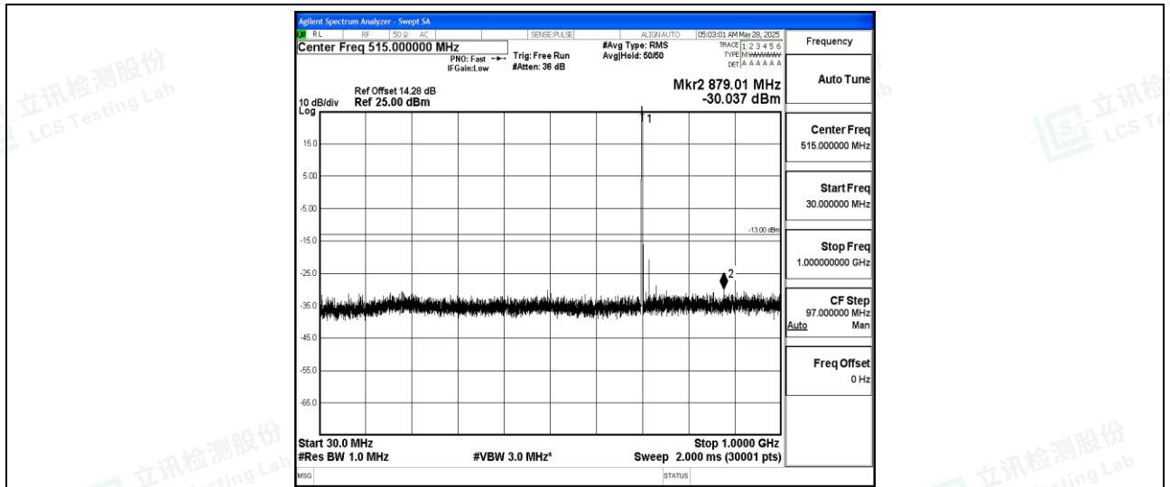
Band12-1.4MHz-16QAM-23095-1-0-Low-30-1000--30.04-PASS
