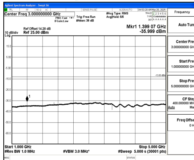
Band12-3MHz-16QAM-23025-1-0-Low-1000-5000--36-PASS
