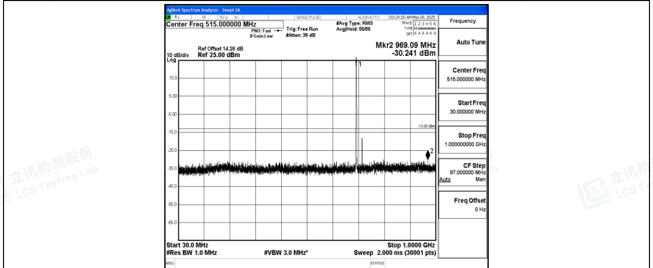
Band12-10MHz-QPSK-23060-1-0-Low-30-1000--30.24-PASS
