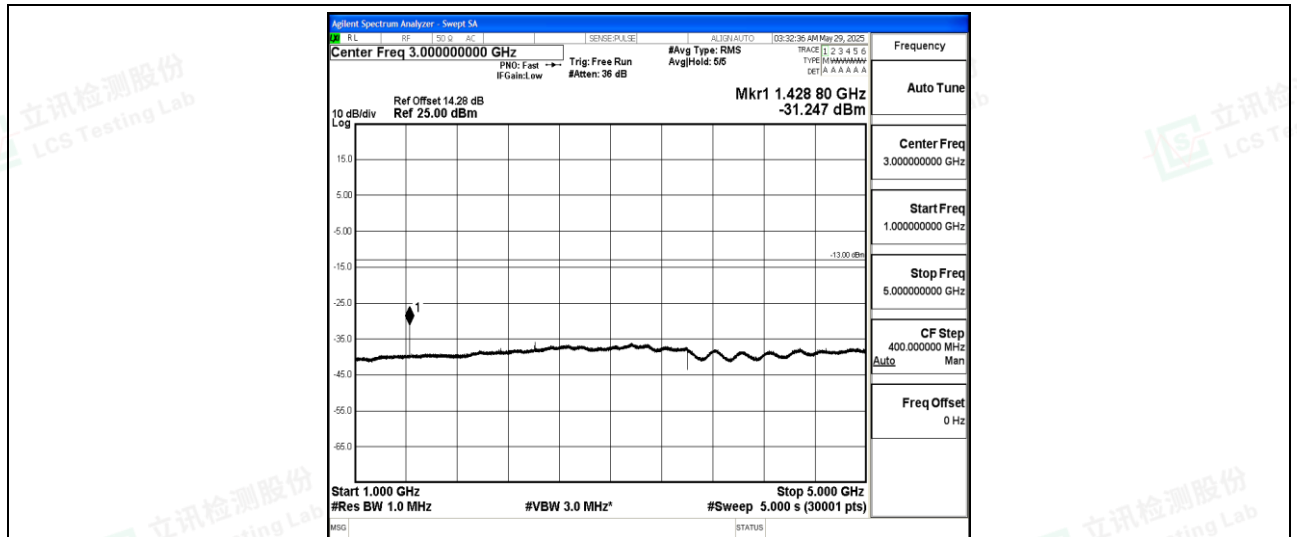
Band12-10MHz-QPSK-23130-1-0-High-1000-5000--31.25-PASS
