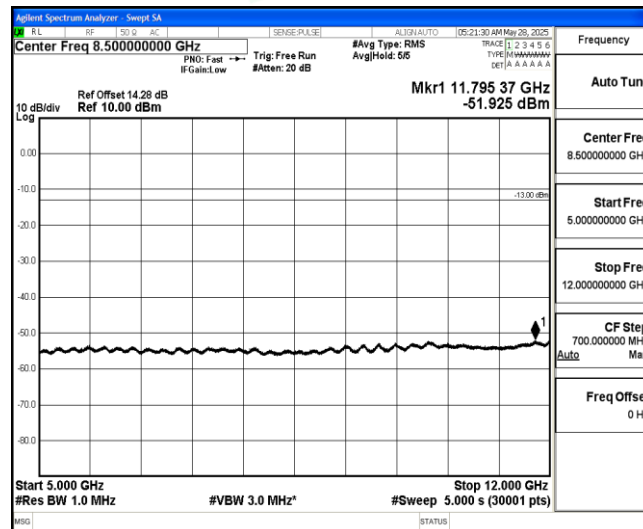
Band12-5MHz-16QAM-23035-1-0-Low-5000-12000--51.93-PASS
