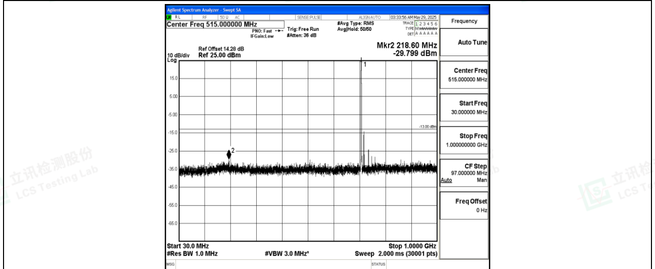
Band12-10MHz-16QAM-23130-1-0-High-30-1000--29.8-PASS
