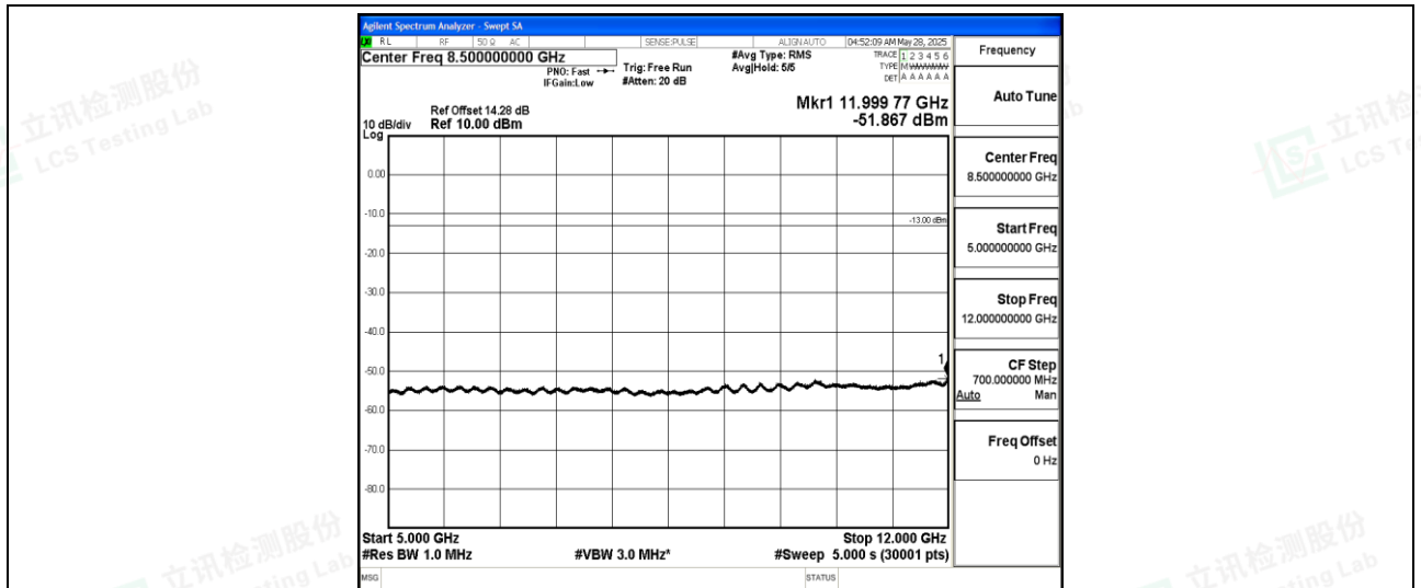
Band12-3MHz-QPSK-23025-1-0-Low-5000-12000--51.87-PASS
