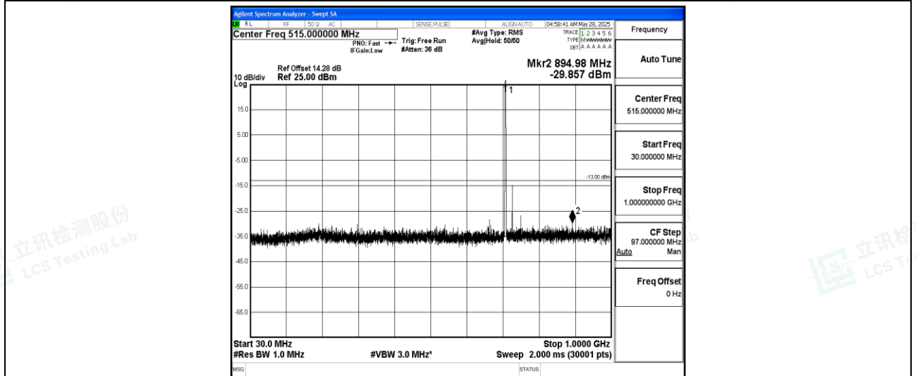
Band12-3MHz-QPSK-23165-1-0-High-30-1000--29.86-PASS
