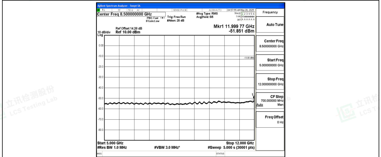
Band12-3MHz-16QAM-23095-1-0-Low-5000-12000--51.85-PASS
