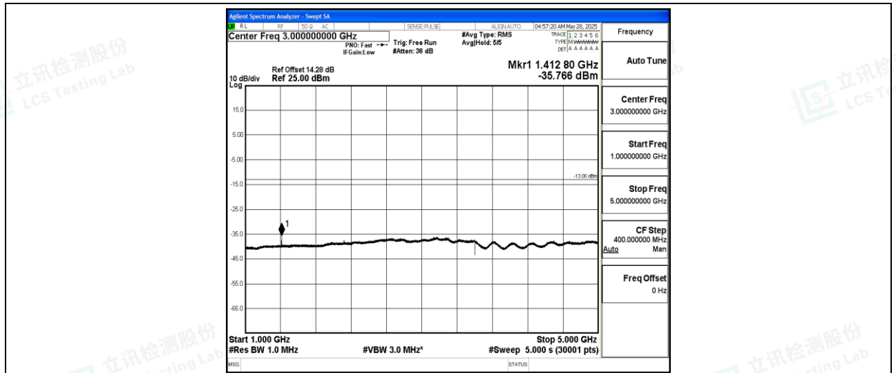
Band12-3MHz-16QAM-23095-1-0-Low-1000-5000--35.77-PASS
