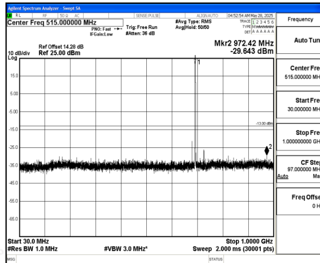
Band12-3MHz-16QAM-23025-1-0-Low-30-1000--29.64-PASS
