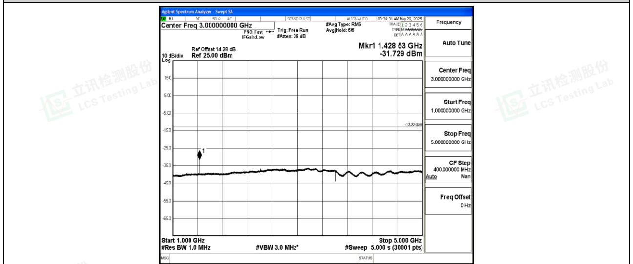
Band12-10MHz-16QAM-23130-1-0-High-30-1000--29.8-PASS
