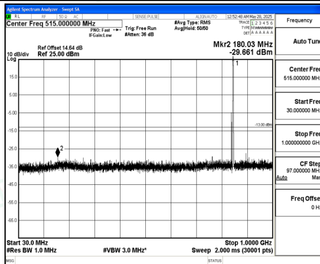
Band5-1.4MHz-16QAM-20643-1-0-High-30-1000--29.66-PASS
