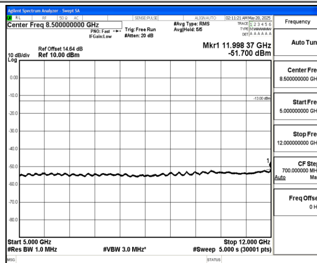
Band5-5MHz-16QAM-20525-1-0-Low-5000-12000--51.7-PASS
