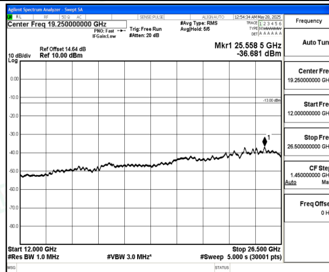
Band5-1.4MHz-16QAM-20643-1-0-High-12000-26500--36.68-PASS
