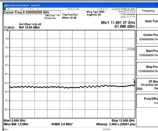
Band5-3MHz-QPSK-20525-1-0-Low-5000-12000--51.69-PASS
