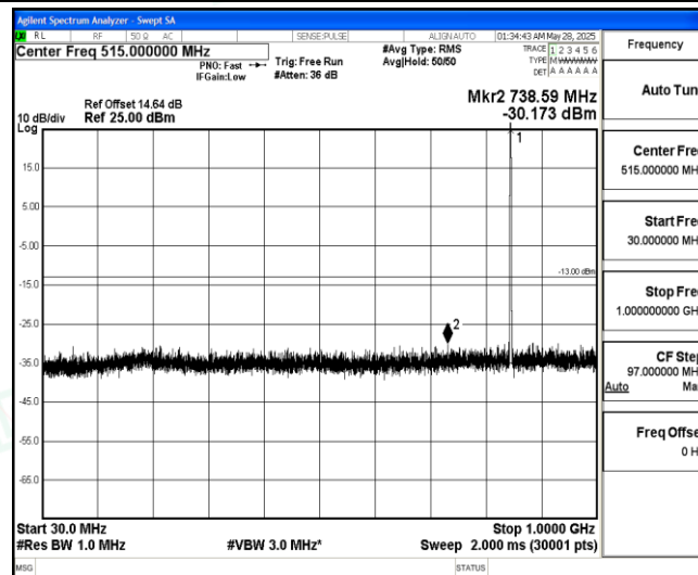
Band5-3MHz-QPSK-20635-1-0-High-30-1000--30.17-PASS
