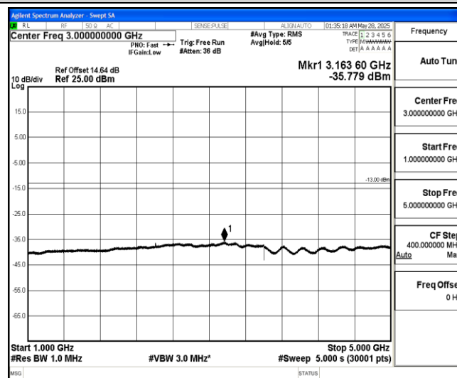
Band5-3MHz-QPSK-20635-1-0-High-1000-5000--35.78-PASS
