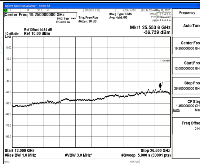
Band5-3MHz-16QAM-20525-1-0-Low-12000-26500--36.74-PASS
