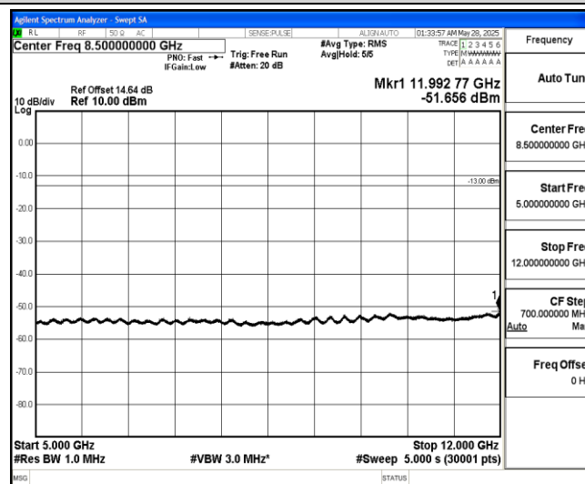
Band5-3MHz-16QAM-20525-1-0-Low-5000-12000--51.66-PASS
