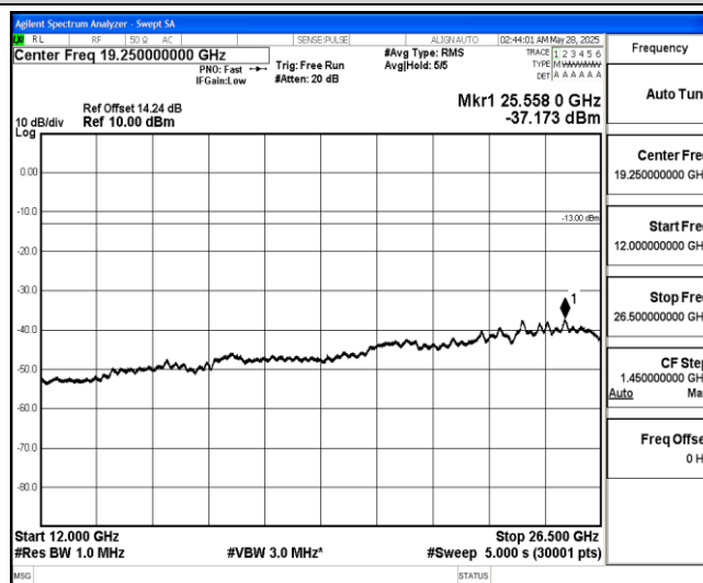
Band5-10MHz-16QAM-20450-1-0-Low-12000-26500--37.17-PASS
