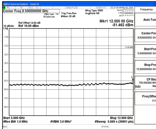
Band5-3MHz-16QAM-20635-1-0-High-5000-12000--51.46-PASS
