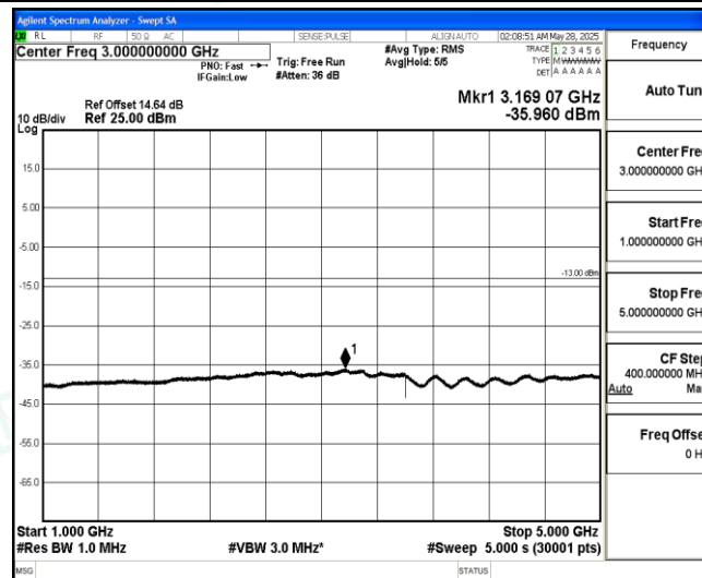
Band5-5MHz-QPSK-20525-1-0-Low-1000-5000--35.96-PASS
