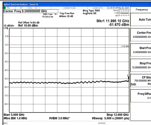
Band5-3MHz-QPSK-20635-1-0-High-5000-12000--51.67-PASS
