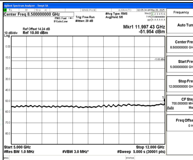
Band5-5MHz-QPSK-20425-1-0-Low-5000-12000--51.95-PASS
