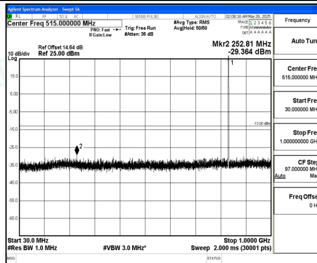
Band5-5MHz-QPSK-20525-1-0-Low-30-1000--29.36-PASS
