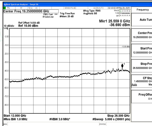
Band5-5MHz-QPSK-20525-1-0-Low-12000-26500--36.69-PASS
