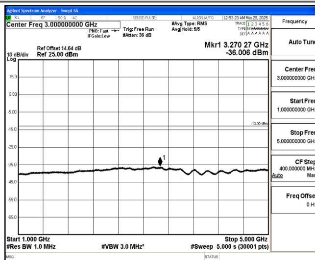
Band5-1.4MHz-16QAM-20643-1-0-High-1000-5000--36.01-PASS
