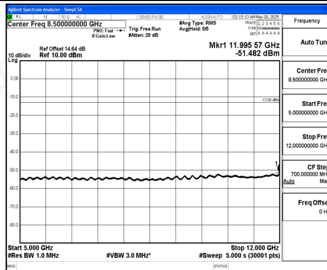
Band5-5MHz-16QAM-20625-1-0-High-5000-12000--51.48-PASS
