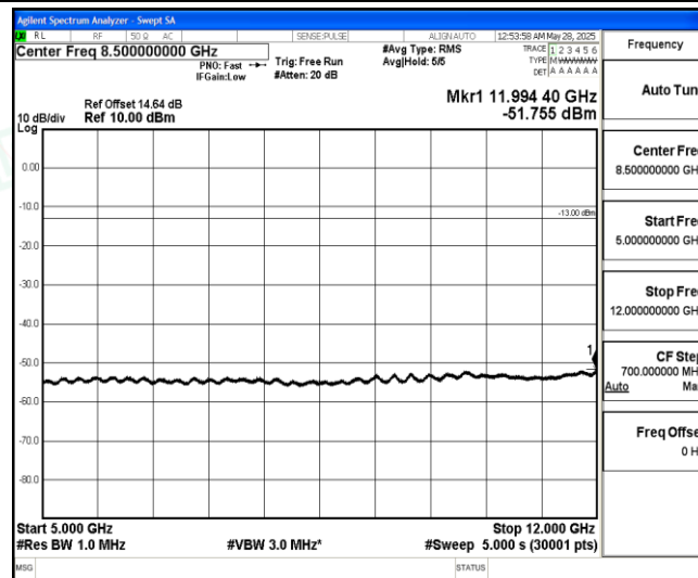
Band5-1.4MHz-16QAM-20643-1-0-High-5000-12000--51.76-PASS
