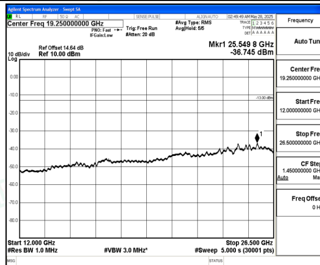
Band5-10MHz-QPSK-20600-1-0-High-12000-26500--36.75-PASS
