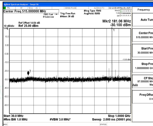
Band5-5MHz-QPSK-20625-1-0-High-30-1000--30.1-PASS
