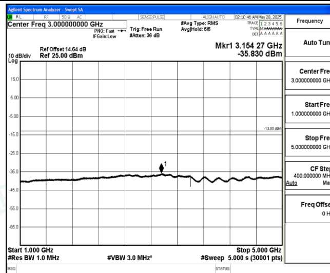
Band5-5MHz-16QAM-20525-1-0-Low-1000-5000--35.83-PASS
