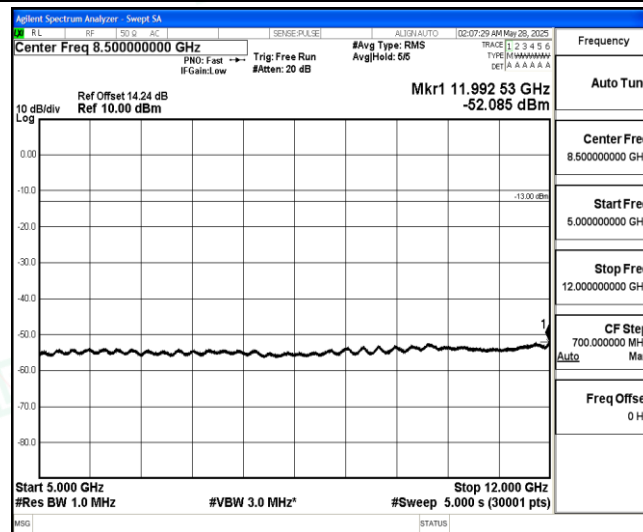
Band5-5MHz-16QAM-20425-1-0-Low-5000-12000--52.09-PASS
