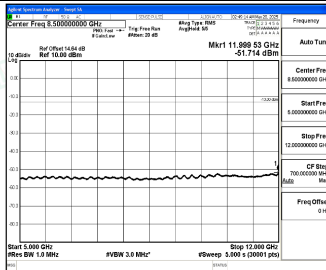
Band5-10MHz-QPSK-20600-1-0-High-5000-12000--51.71-PASS
