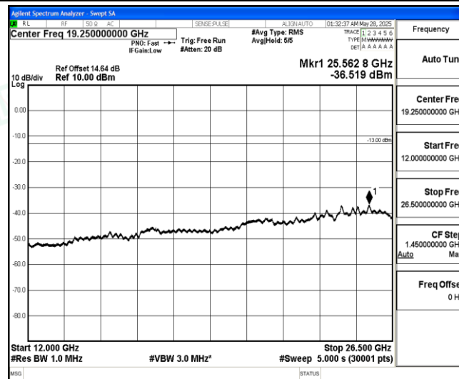
Band5-3MHz-QPSK-20525-1-0-Low-12000-26500--36.52-PASS
