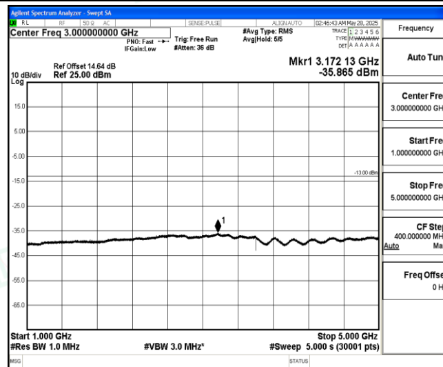
Band5-10MHz-16QAM-20525-1-0-Low-1000-5000--35.87-PASS
