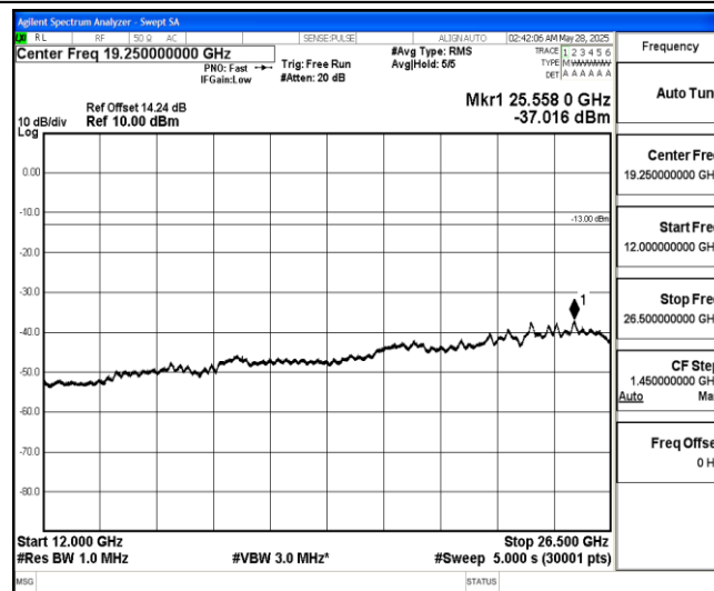
Band5-10MHz-QPSK-20450-1-0-Low-12000-26500--37.02-PASS
