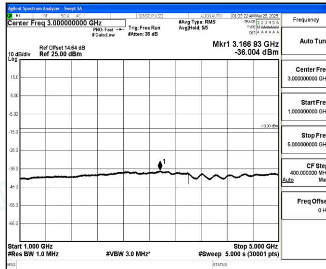
Band5-3MHz-16QAM-20525-1-0-Low-1000-5000--36-PASS
