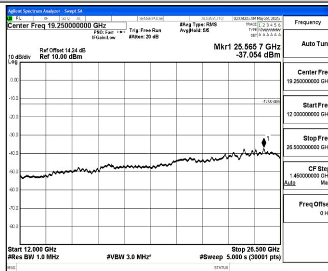
Band5-5MHz-16QAM-20425-1-0-Low-12000-26500--37.05-PASS
