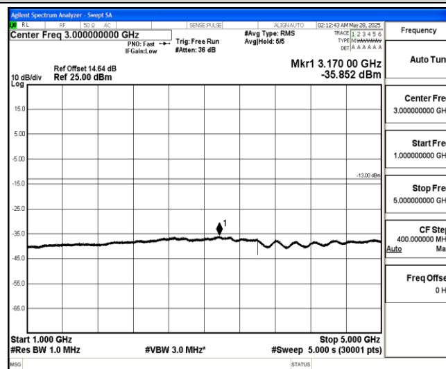
Band5-5MHz-QPSK-20625-1-0-High-1000-5000--35.85-PASS
