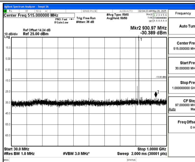
Band5-5MHz-QPSK-20425-1-0-Low-30-1000--30.39-PASS
