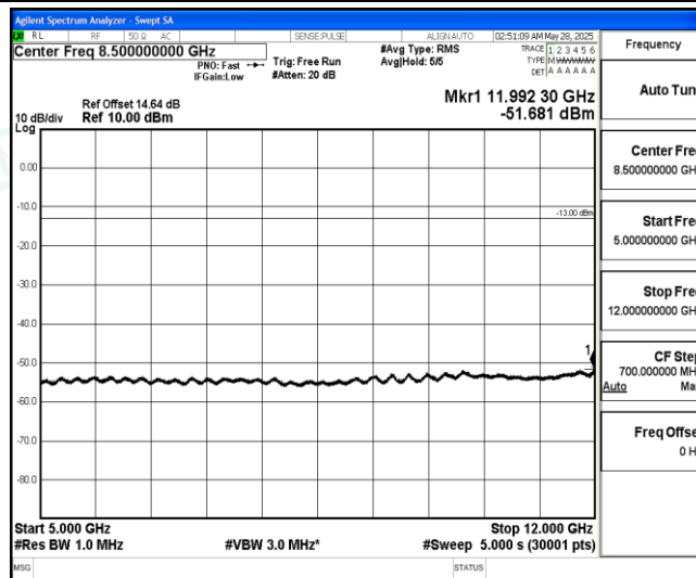
Band5-10MHz-16QAM-20600-1-0-High-5000-12000--51.68-PASS
