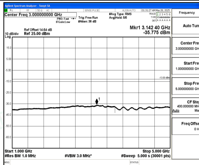
Band5-3MHz-QPSK-20525-1-0-Low-1000-5000--35.78-PASS
