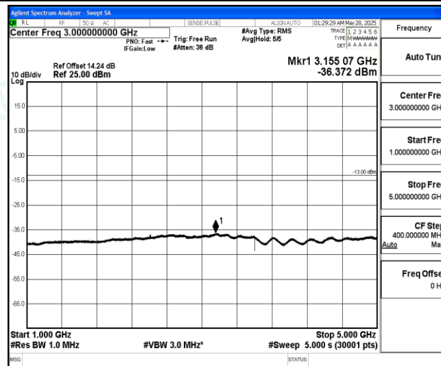
Band5-3MHz-16QAM-20415-1-0-Low-1000-5000--36.37-PASS
