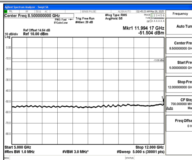
Band5-10MHz-QPSK-20525-1-0-Low-5000-12000--51.5-PASS
