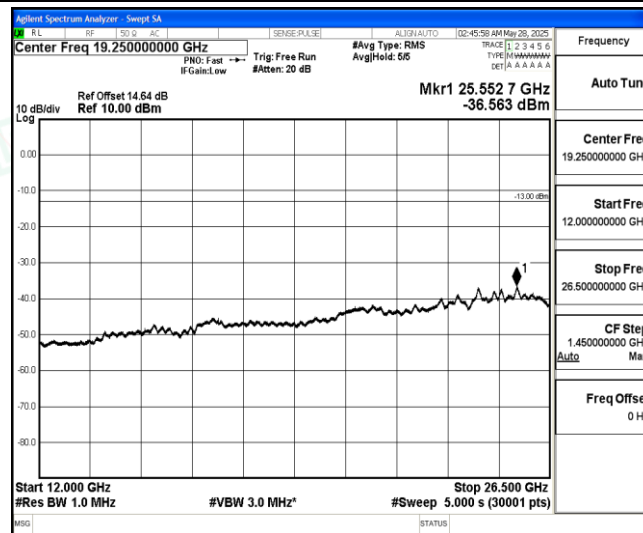
Band5-10MHz-QPSK-20525-1-0-Low-12000-26500--36.56-PASS
