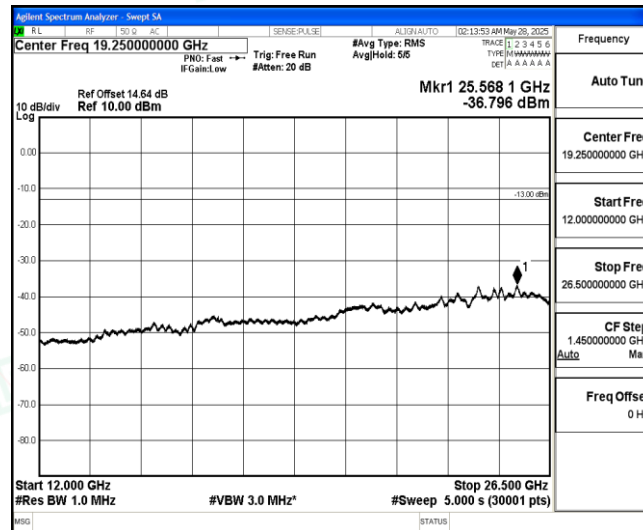
Band5-5MHz-QPSK-20625-1-0-High-12000-26500--36.8-PASS
