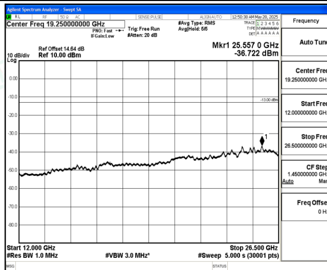
Band5-1.4MHz-16QAM-20525-1-0-Low-12000-26500--36.72-PASS
