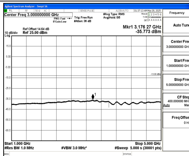
Band5-3MHz-16QAM-20635-1-0-High-1000-5000--35.77-PASS
