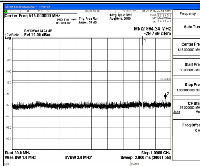
Band5-10MHz-16QAM-20450-1-0-Low-30-1000--29.77-PASS
