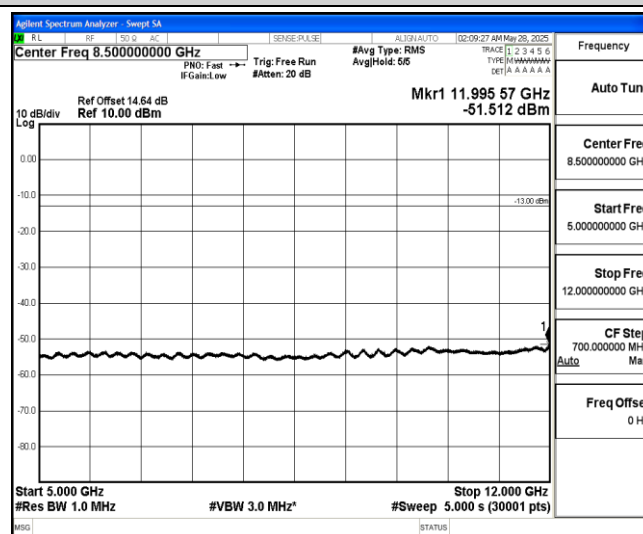
Band5-5MHz-QPSK-20525-1-0-Low-5000-12000--51.51-PASS
