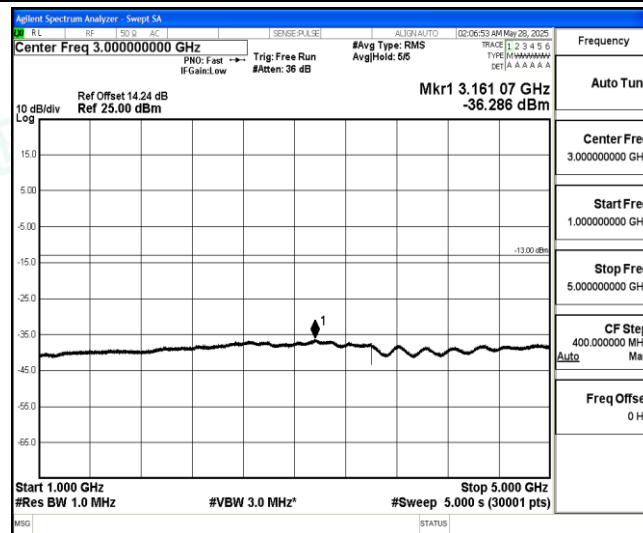
Band5-5MHz-16QAM-20425-1-0-Low-1000-5000--36.29-PASS
