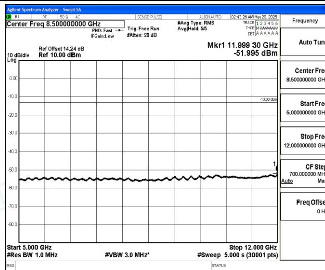
Band5-10MHz-16QAM-20450-1-0-Low-5000-12000--52-PASS
