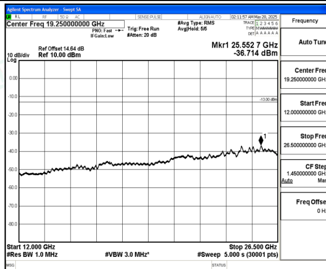
Band5-5MHz-16QAM-20525-1-0-Low-12000-26500--36.71-PASS
