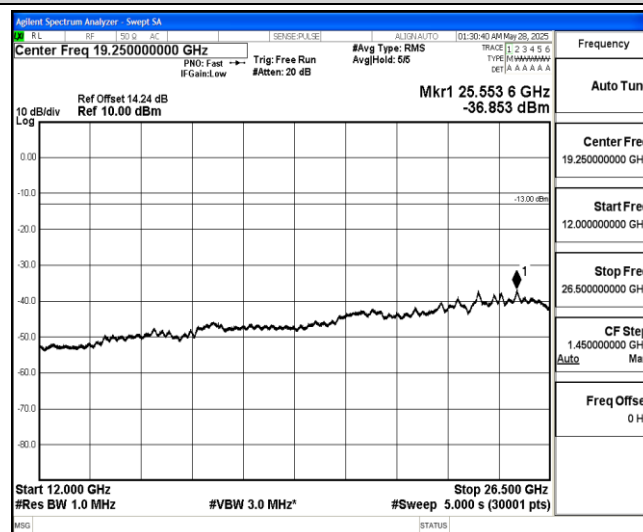
Band5-3MHz-16QAM-20415-1-0-Low-12000-26500--36.85-PASS
