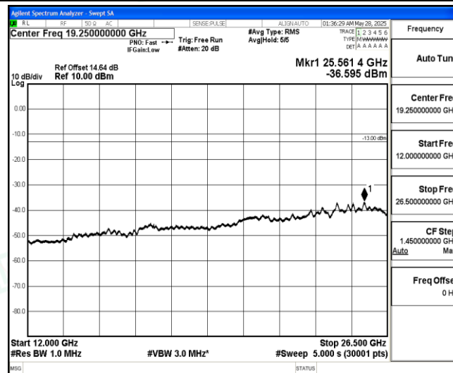
Band5-3MHz-QPSK-20635-1-0-High-12000-26500--36.6-PASS
