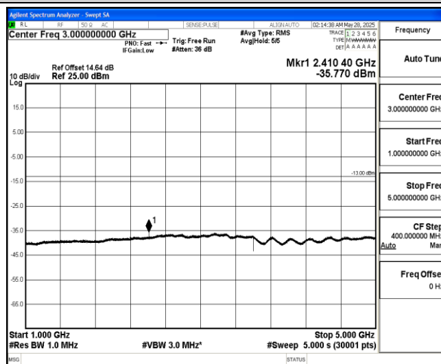
Band5-5MHz-16QAM-20625-1-0-High-1000-5000--35.77-PASS
