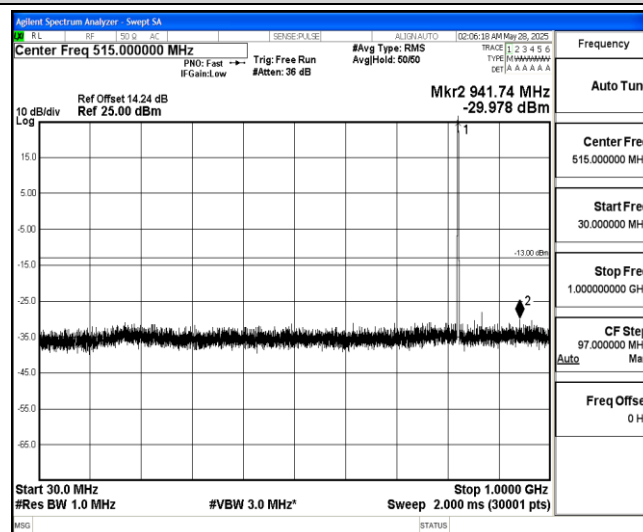
Band5-5MHz-16QAM-20425-1-0-Low-30-1000--29.98-PASS
