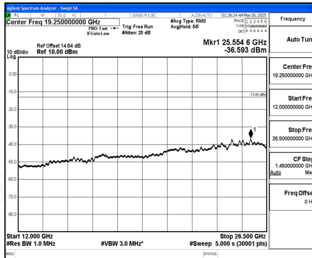
Band5-3MHz-16QAM-20635-1-0-High-12000-26500--36.59-PASS
