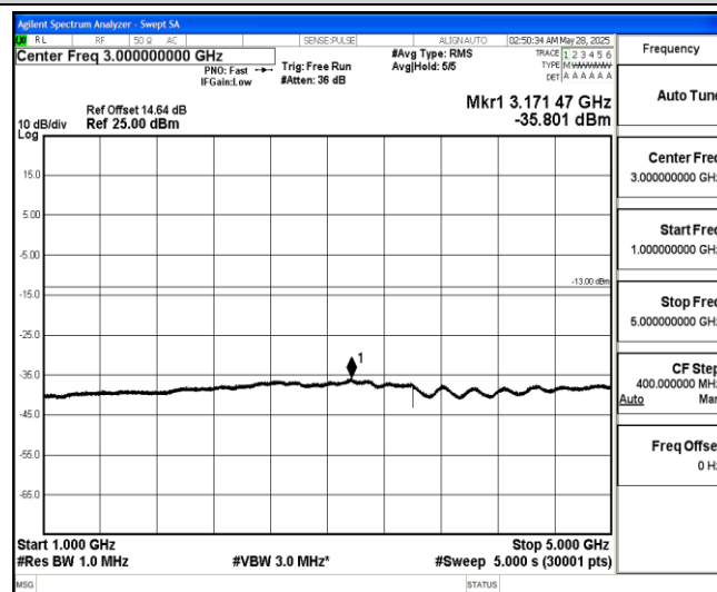
Band5-10MHz-16QAM-20600-1-0-High-1000-5000--35.8-PASS
