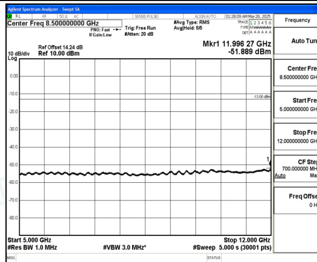
Band5-3MHz-QPSK-20415-1-0-Low-5000-12000--51.89-PASS
