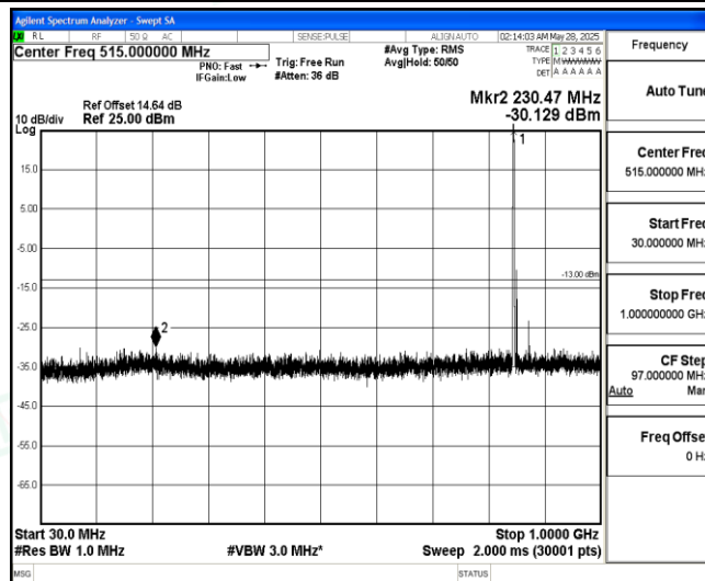
Band5-5MHz-16QAM-20625-1-0-High-30-1000--30.13-PASS
