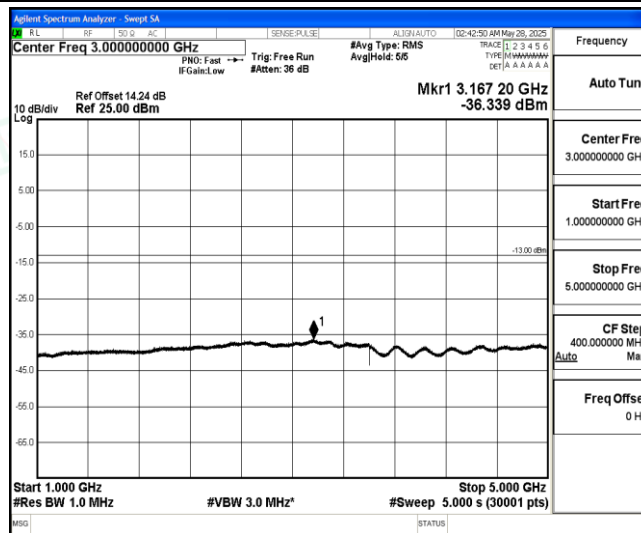
Band5-10MHz-16QAM-20450-1-0-Low-1000-5000--36.34-PASS
