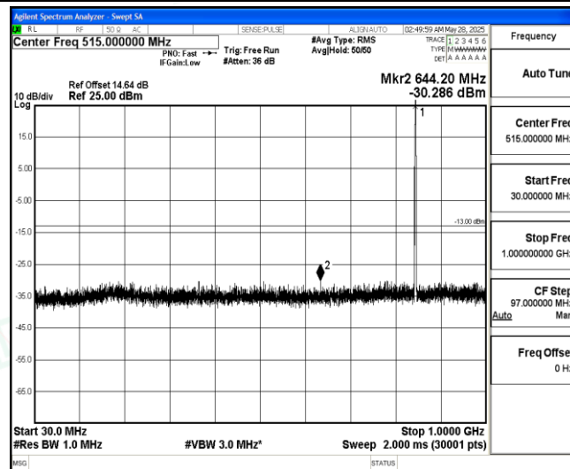
Band5-10MHz-16QAM-20600-1-0-High-30-1000--30.29-PASS
