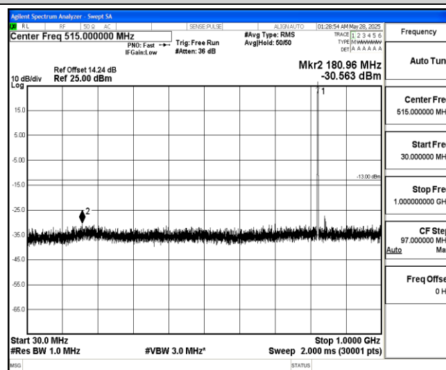
Band5-3MHz-16QAM-20415-1-0-Low-30-1000--30.56-PASS
