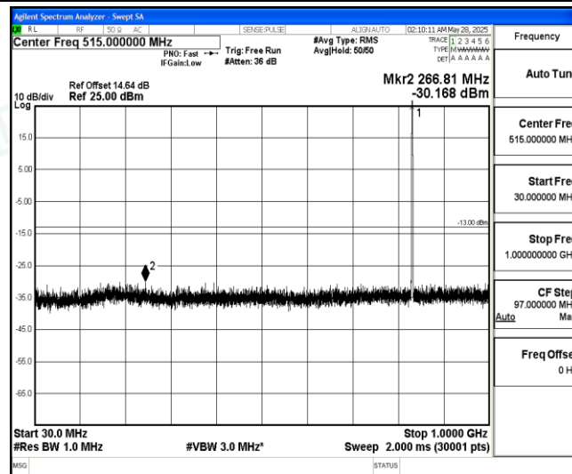
Band5-5MHz-16QAM-20525-1-0-Low-30-1000--30.17-PASS
