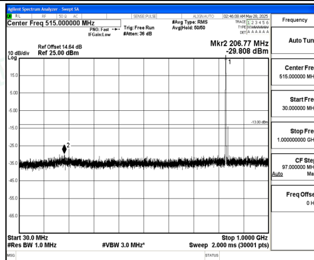
Band5-10MHz-16QAM-20525-1-0-Low-30-1000--29.81-PASS
