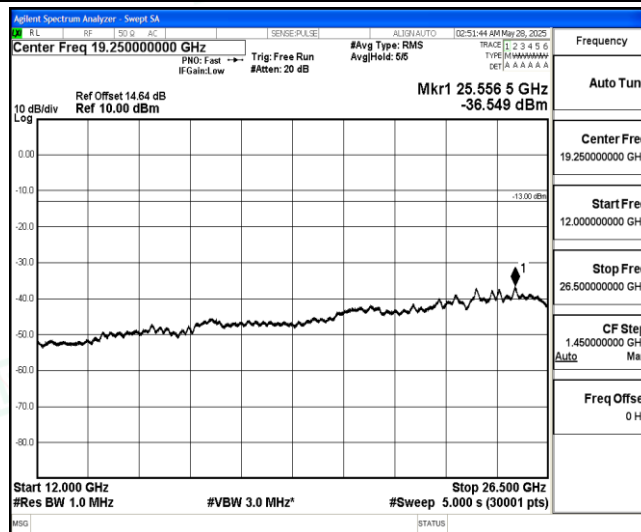
Band5-10MHz-16QAM-20600-1-0-High-12000-26500--36.55-PASS
