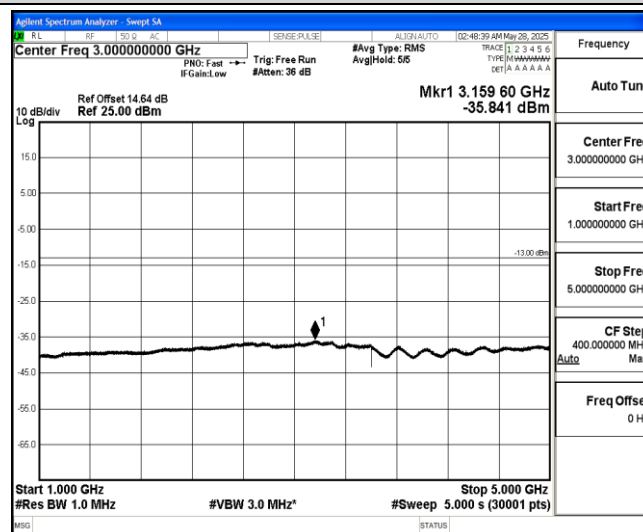
Band5-10MHz-QPSK-20600-1-0-High-1000-5000--35.84-PASS
