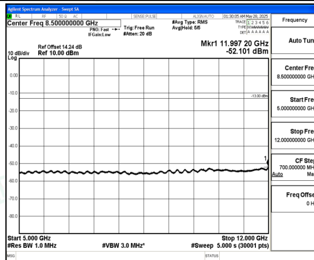
Band5-3MHz-16QAM-20415-1-0-Low-5000-12000--52.1-PASS
