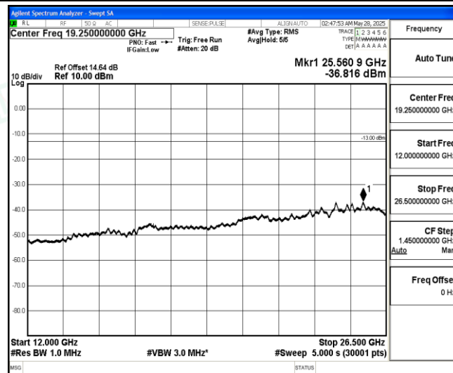
Band5-10MHz-16QAM-20525-1-0-Low-12000-26500--36.82-PASS
