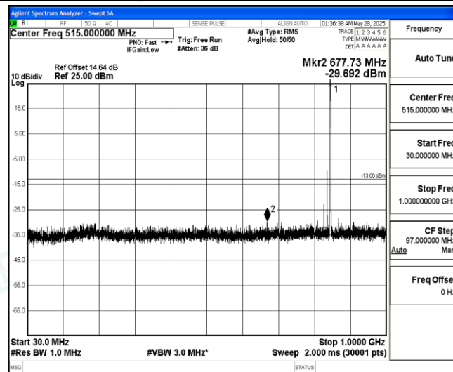
Band5-3MHz-16QAM-20635-1-0-High-30-1000--29.69-PASS
