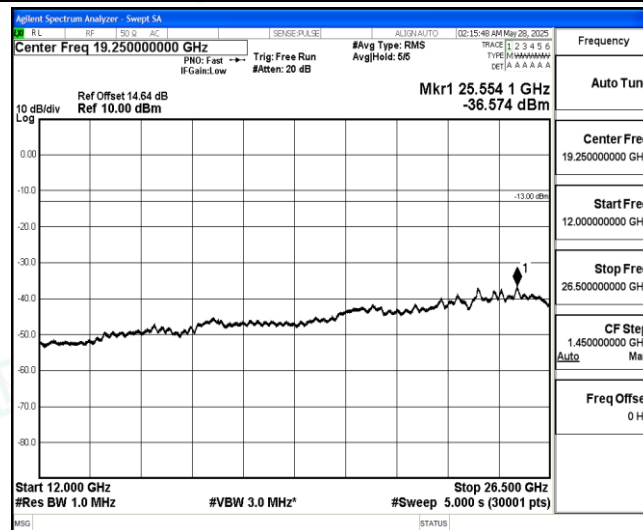
Band5-5MHz-16QAM-20625-1-0-High-12000-26500--36.57-PASS
