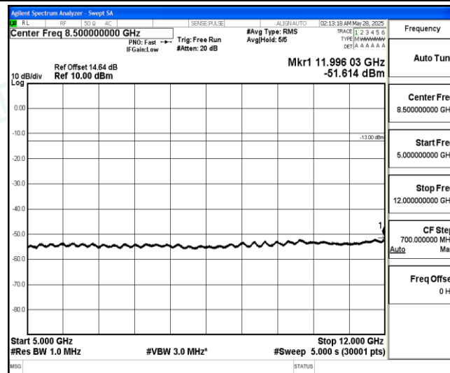
Band5-5MHz-QPSK-20625-1-0-High-5000-12000--51.61-PASS
