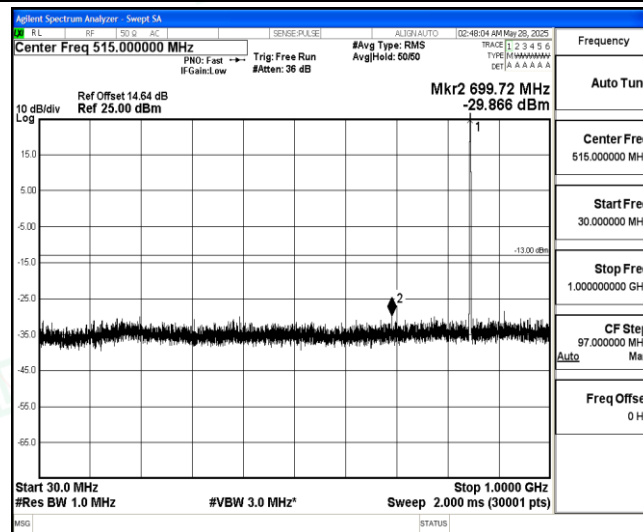
Band5-10MHz-QPSK-20600-1-0-High-30-1000--29.87-PASS
