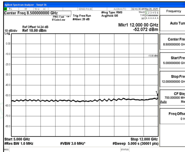
Band5-10MHz-QPSK-20450-1-0-Low-5000-12000--52.07-PASS
