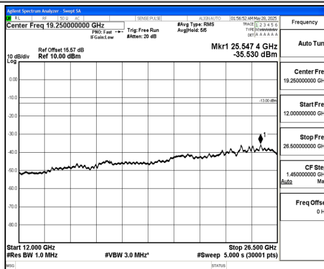
Band4-10MHz-16QAM-20000-1-0-Low-12000-26500--35.53-PASS
