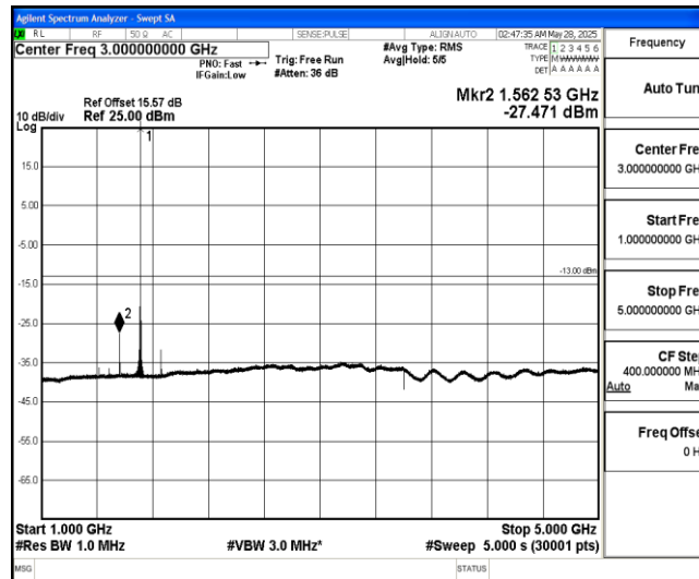
Band4-20MHz-16QAM-20050-1-0-Low-1000-5000--27.47-PASS
