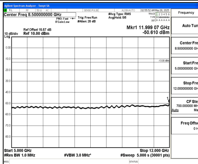
Band4-20MHz-16QAM-20300-1-0-High-5000-12000--50.61-PASS
