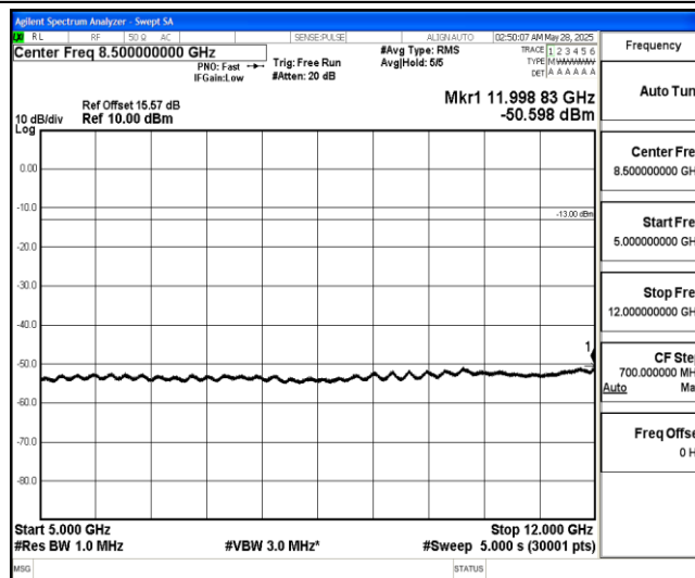
Band4-20MHz-QPSK-20175-1-0-Low-5000-12000--50.6-PASS
