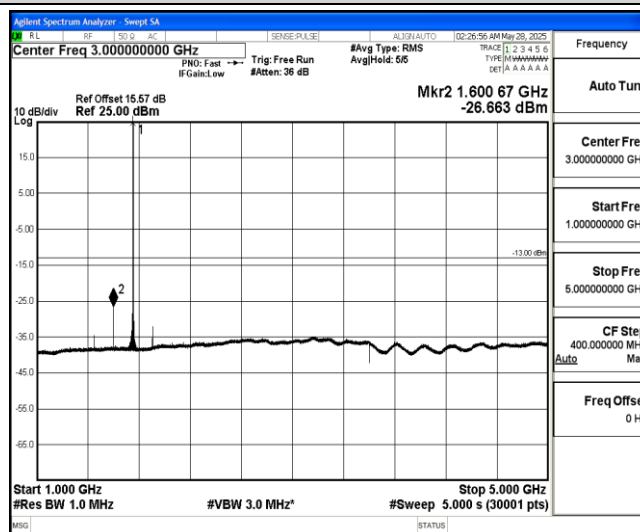
Band4-15MHz-QPSK-20325-1-0-High-1000-5000--26.66-PASS
