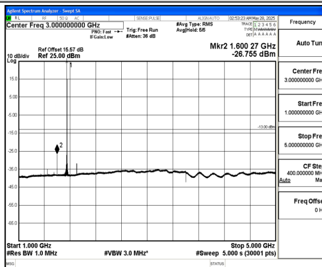
Band4-20MHz-QPSK-20300-1-0-High-1000-5000--26.76-PASS
