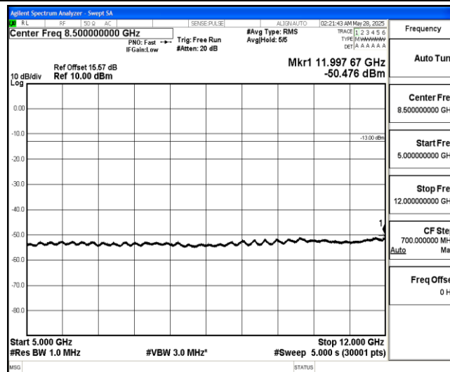
Band4-15MHz-16QAM-20025-1-0-Low-5000-12000--50.48-PASS
