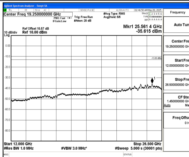
Band4-20MHz-QPSK-20050-1-0-Low-12000-26500--35.62-PASS
