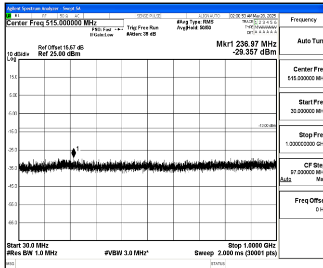
Band4-10MHz-QPSK-20350-1-0-High-30-1000--29.36-PASS
