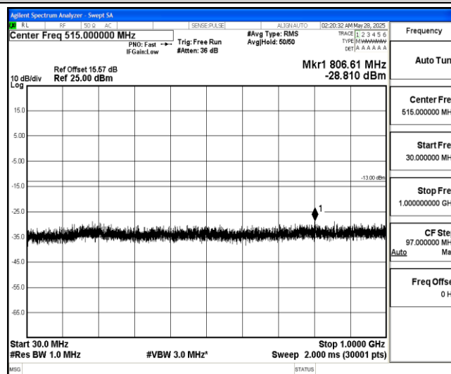
Band4-15MHz-16QAM-20025-1-0-Low-30-1000--28.81-PASS
