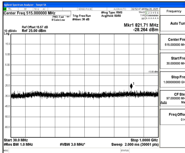
Band4-20MHz-QPSK-20300-1-0-High-30-1000--28.26-PASS
