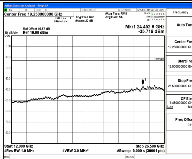
Band4-20MHz-QPSK-20300-1-0-High-12000-26500--35.72-PASS
