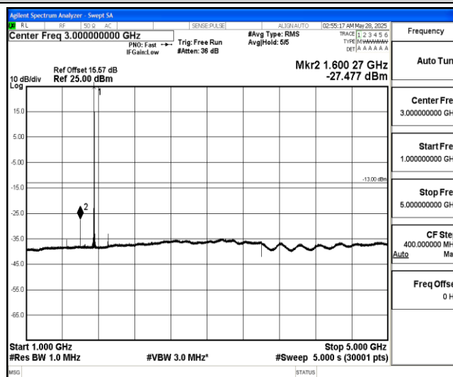
Band4-20MHz-16QAM-20300-1-0-High-1000-5000--27.48-PASS
