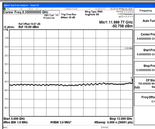
Band4-15MHz-16QAM-20175-1-0-Low-5000-12000--50.76-PASS
