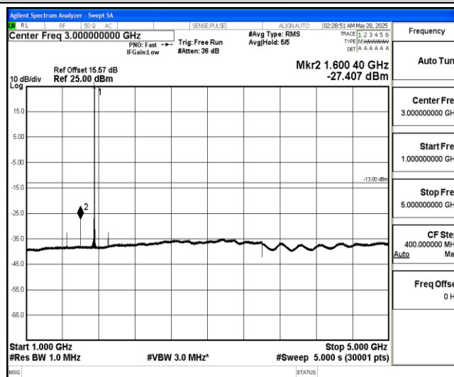
Band4-15MHz-16QAM-20325-1-0-High-1000-5000--27.41-PASS
