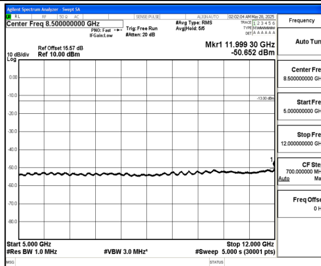
Band4-10MHz-QPSK-20350-1-0-High-5000-12000--50.65-PASS
