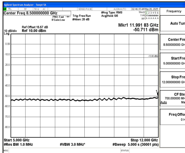
Band4-20MHz-QPSK-20050-1-0-Low-5000-12000--50.71-PASS
