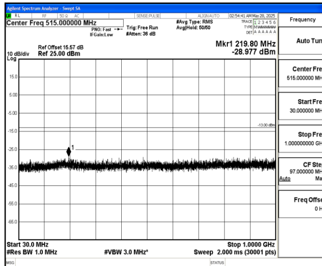
Band4-20MHz-16QAM-20300-1-0-High-30-1000--28.98-PASS
