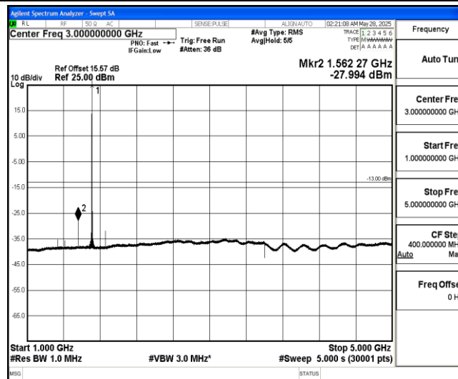
Band4-15MHz-16QAM-20025-1-0-Low-1000-5000--27.99-PASS
