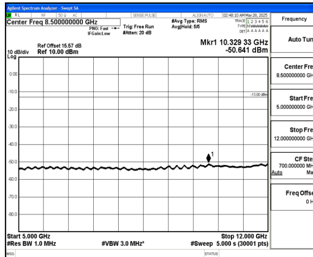
Band4-20MHz-16QAM-20050-1-0-Low-5000-12000--50.64-PASS
