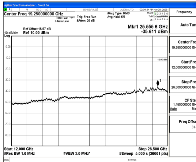
Band4-10MHz-16QAM-20350-1-0-High-12000-26500--35.61-PASS
