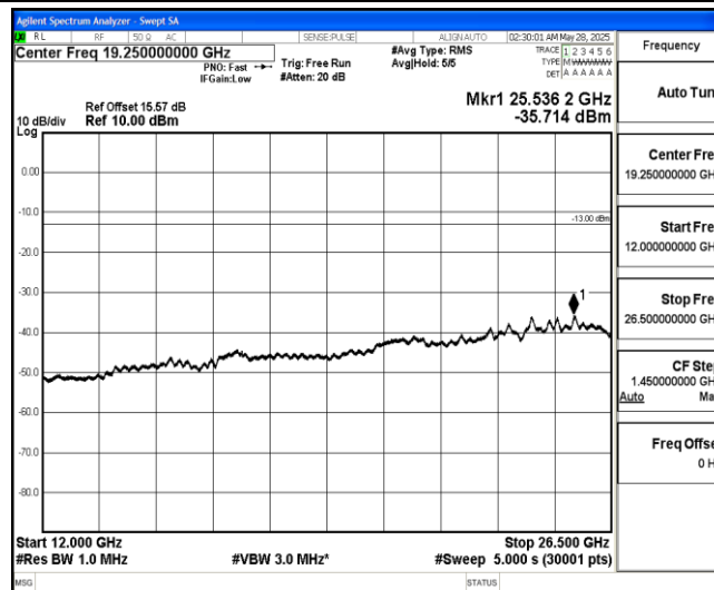
Band4-15MHz-16QAM-20325-1-0-High-12000-26500--35.71-PASS
