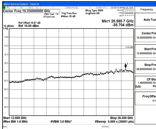
Band4-10MHz-16QAM-20175-1-0-Low-12000-26500--35.7-PASS
