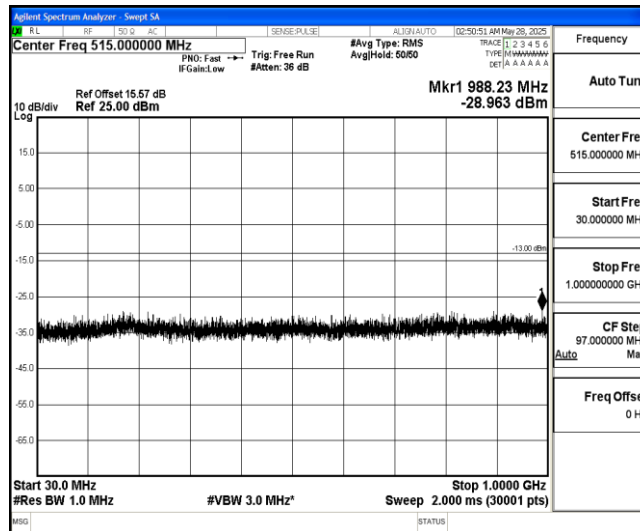
Band4-20MHz-16QAM-20175-1-0-Low-30-1000--28.96-PASS
