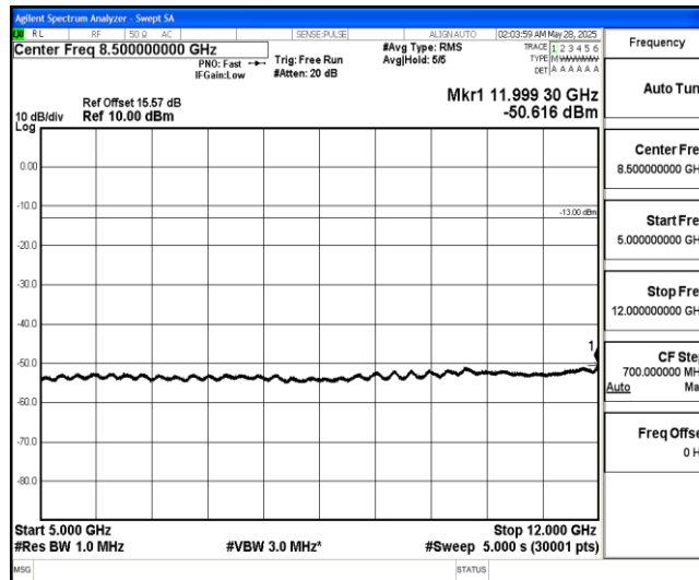
Band4-10MHz-16QAM-20350-1-0-High-5000-12000--50.62-PASS
