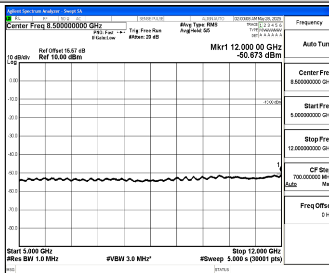
Band4-10MHz-16QAM-20175-1-0-Low-5000-12000--50.67-PASS
