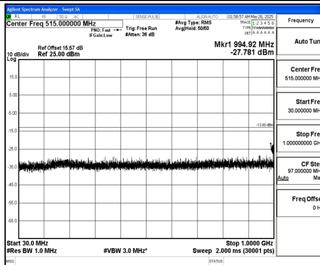
Band4-10MHz-16QAM-20175-1-0-Low-30-1000--27.78-PASS
