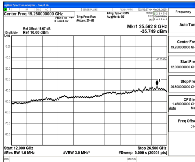
Band4-20MHz-16QAM-20175-1-0-Low-12000-26500--35.75-PASS
