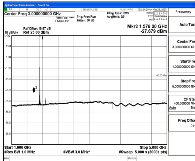
Band4-15MHz-16QAM-20175-1-0-Low-1000-5000--27.68-PASS
