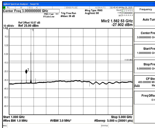
Band4-20MHz-QPSK-20050-1-0-Low-1000-5000--27.9-PASS
