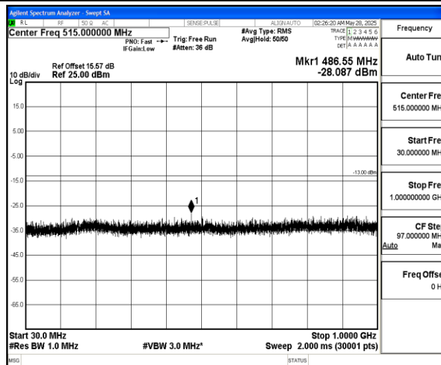
Band4-15MHz-QPSK-20325-1-0-High-30-1000--28.09-PASS
