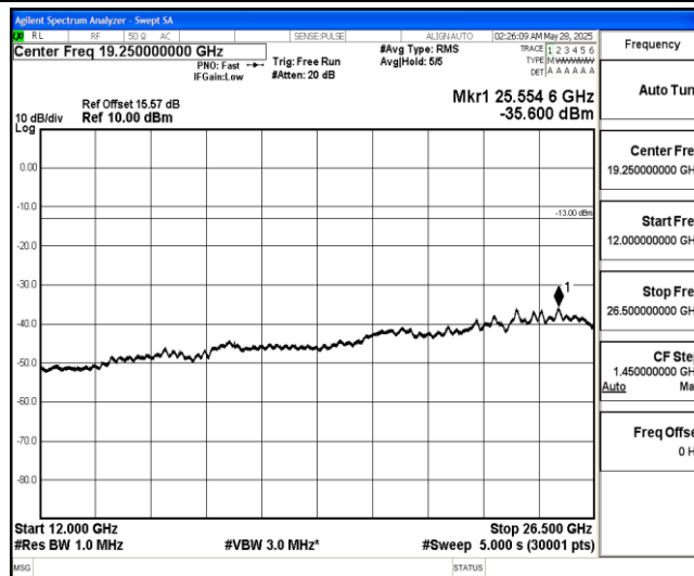
Band4-15MHz-16QAM-20175-1-0-Low-12000-26500--35.6-PASS
