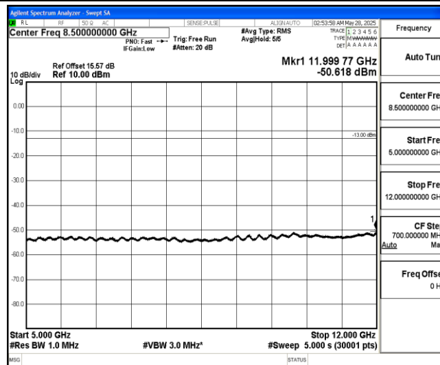
Band4-20MHz-QPSK-20300-1-0-High-5000-12000--50.62-PASS
