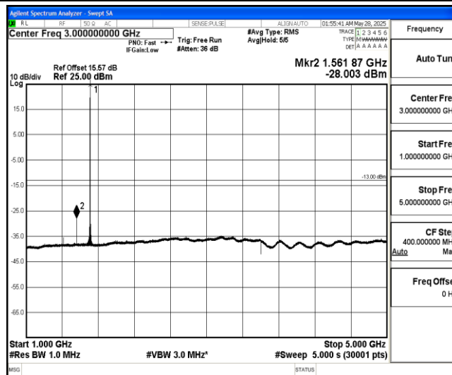
Band4-10MHz-16QAM-20000-1-0-Low-1000-5000--28-PASS
