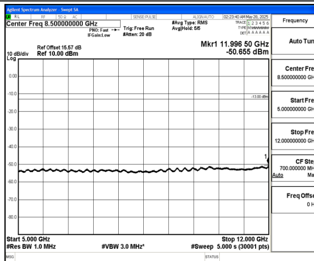
Band4-15MHz-QPSK-20175-1-0-Low-5000-12000--50.66-PASS
