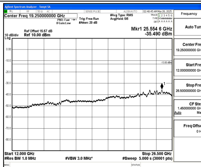
Band4-20MHz-16QAM-20050-1-0-Low-12000-26500--35.49-PASS
