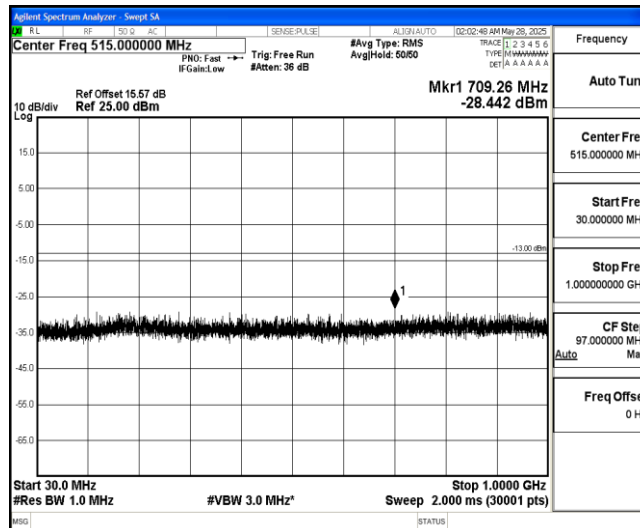
Band4-10MHz-16QAM-20350-1-0-High-30-1000--28.44-PASS
