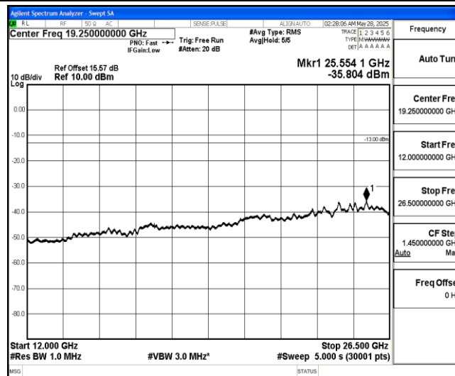
Band4-15MHz-QPSK-20325-1-0-High-12000-26500--35.8-PASS
