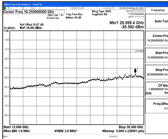
Band4-10MHz-QPSK-20175-1-0-Low-12000-26500--35.39-PASS
