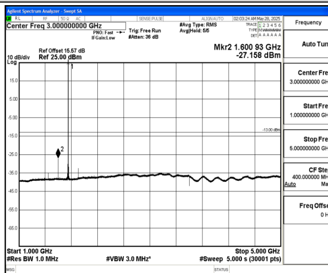
Band4-10MHz-16QAM-20350-1-0-High-1000-5000--27.16-PASS
