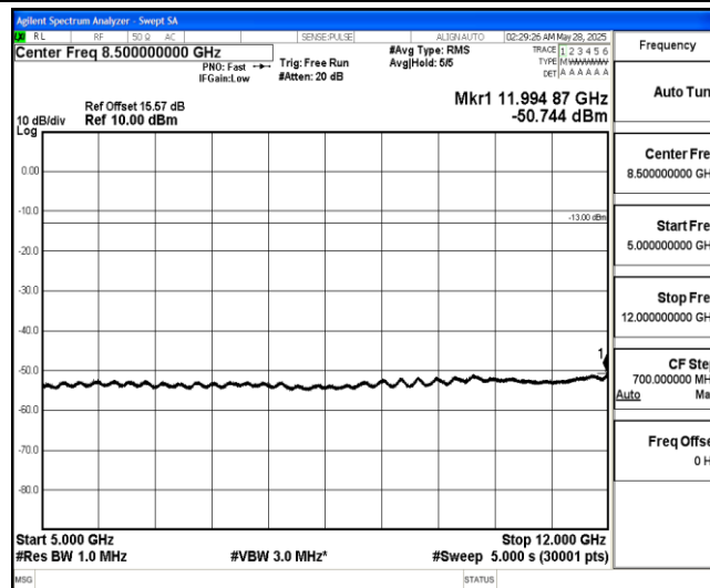
Band4-15MHz-16QAM-20325-1-0-High-5000-12000--50.74-PASS
