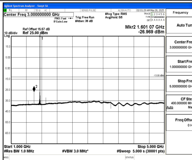
Band4-10MHz-QPSK-20350-1-0-High-1000-5000--26.97-PASS
