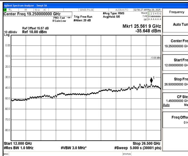
Band4-20MHz-16QAM-20300-1-0-High-12000-26500--35.65-PASS
