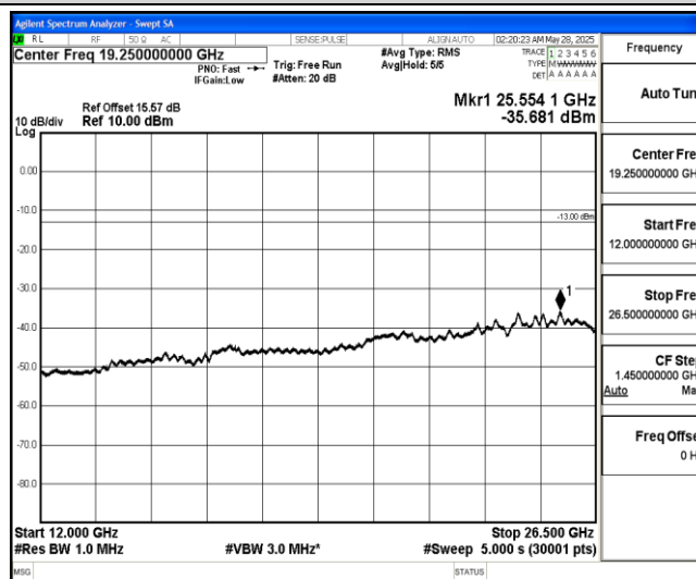
Band4-15MHz-QPSK-20025-1-0-Low-12000-26500--35.68-PASS
