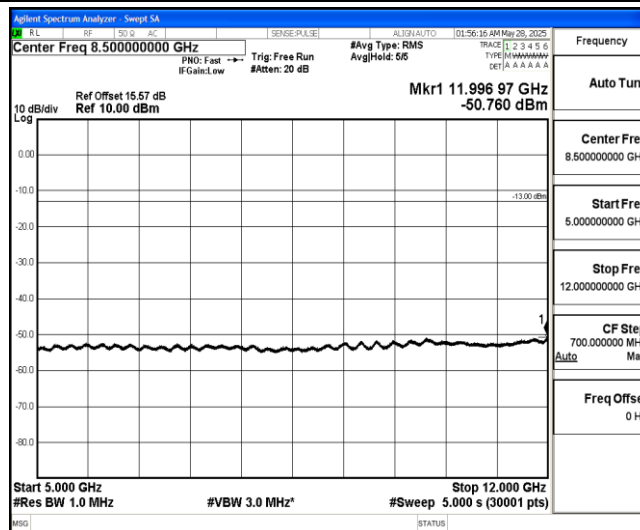
Band4-10MHz-16QAM-20000-1-0-Low-5000-12000--50.76-PASS
