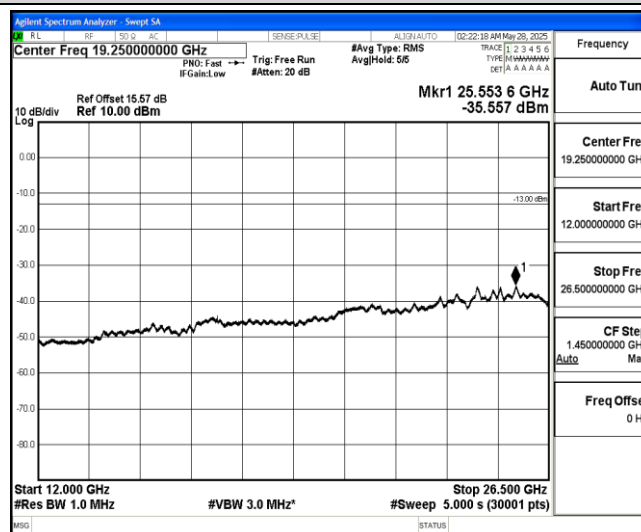
Band4-15MHz-16QAM-20025-1-0-Low-12000-26500--35.56-PASS
