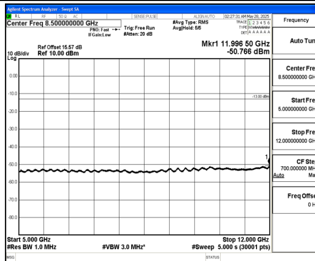
Band4-15MHz-QPSK-20325-1-0-High-5000-12000--50.77-PASS
