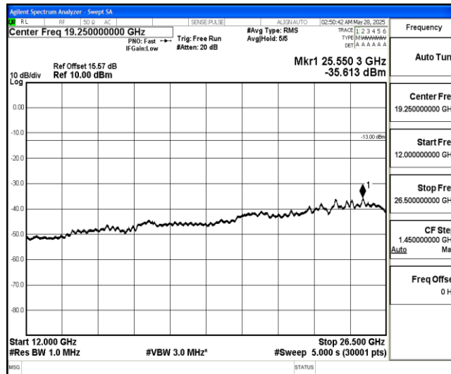
Band4-20MHz-QPSK-20175-1-0-Low-12000-26500--35.61-PASS
