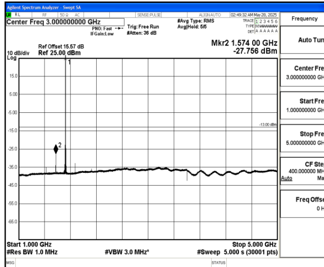
Band4-20MHz-QPSK-20175-1-0-Low-1000-5000--27.76-PASS
