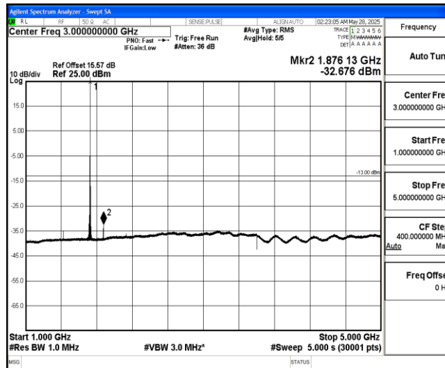
Band4-15MHz-QPSK-20175-1-0-Low-1000-5000--32.68-PASS
