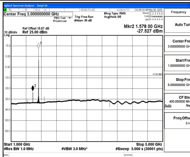
Band4-10MHz-16QAM-20175-1-0-Low-1000-5000--27.53-PASS
