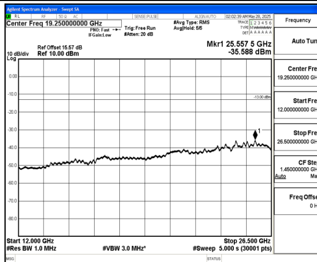
Band4-10MHz-QPSK-20350-1-0-High-12000-26500--35.59-PASS
