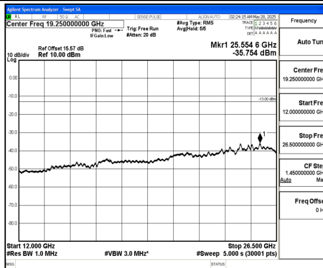
Band4-15MHz-QPSK-20175-1-0-Low-12000-26500--35.75-PASS
