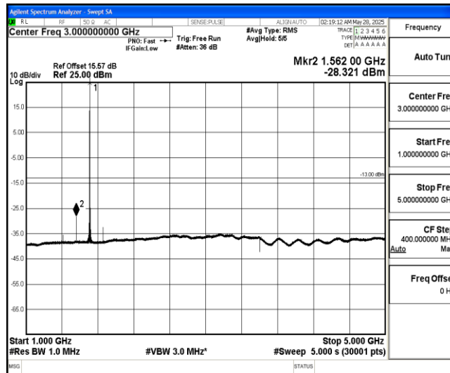
Band4-15MHz-QPSK-20025-1-0-Low-1000-5000--28.32-PASS
