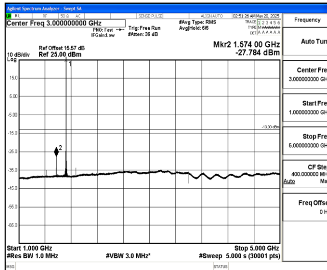
Band4-20MHz-16QAM-20175-1-0-Low-1000-5000--27.78-PASS
