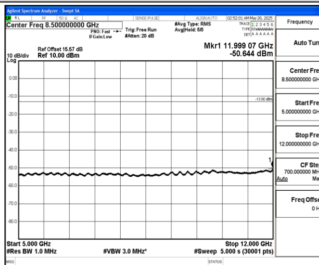
Band4-20MHz-16QAM-20175-1-0-Low-5000-12000--50.64-PASS
