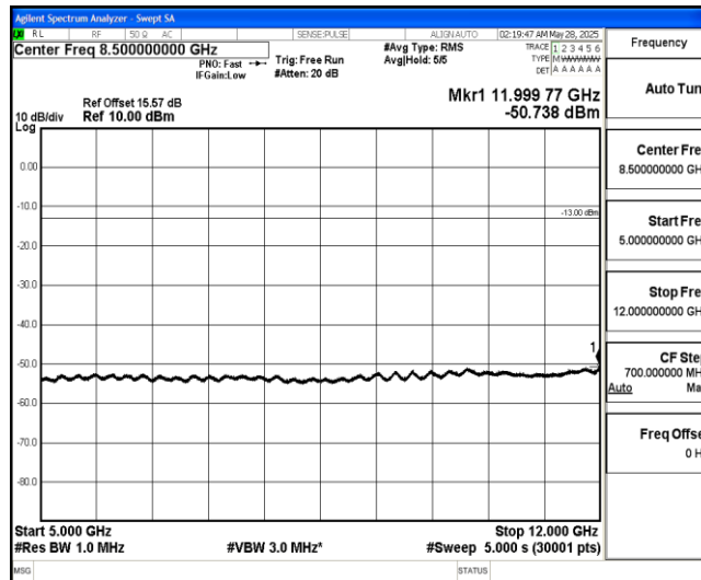
Band4-15MHz-QPSK-20025-1-0-Low-5000-12000--50.74-PASS
