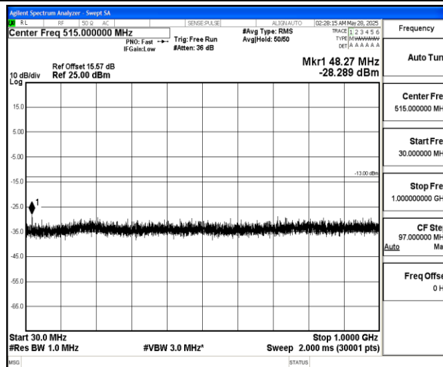
Band4-15MHz-16QAM-20325-1-0-High-30-1000--28.29-PASS
