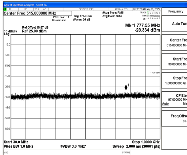
Band4-5MHz-QPSK-20375-1-0-High-30-1000--28.33-PASS
