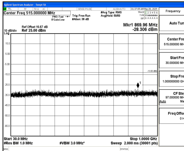
Band4-5MHz-16QAM-20375-1-0-High-30-1000--28.31-PASS
