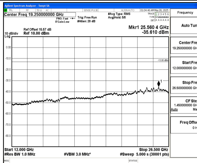
Band4-3MHz-QPSK-20175-1-0-Low-12000-26500--35.61-PASS
