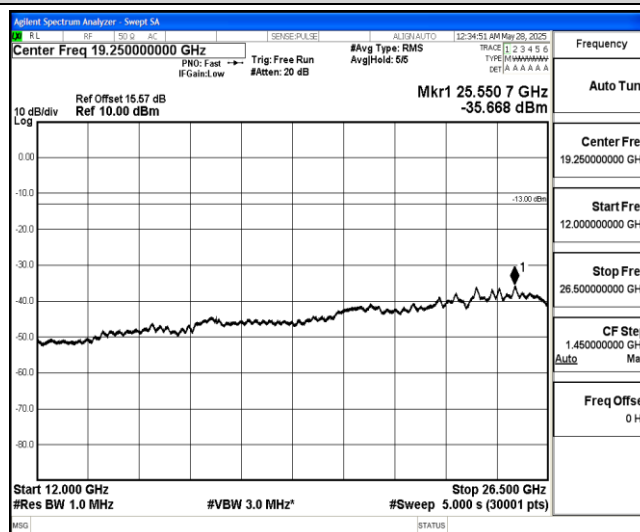
Band4-1.4MHz-16QAM-19957-1-0-Low-12000-26500--35.67-PASS
