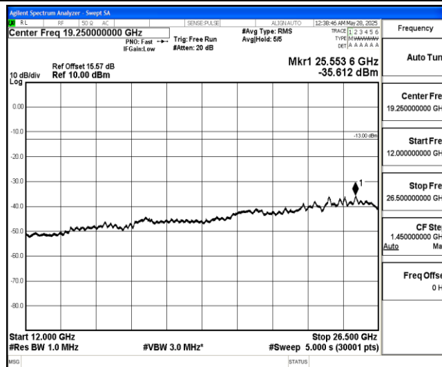
Band4-1.4MHz-16QAM-20175-1-0-Low-12000-26500--35.61-PASS
