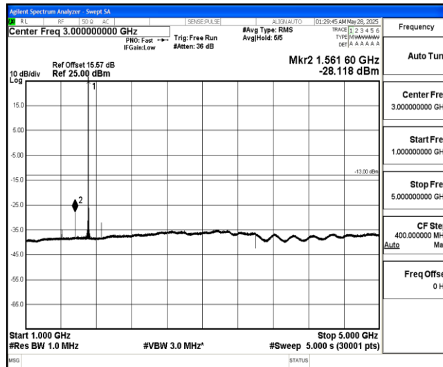
Band4-5MHz-16QAM-19975-1-0-Low-1000-5000--28.12-PASS
