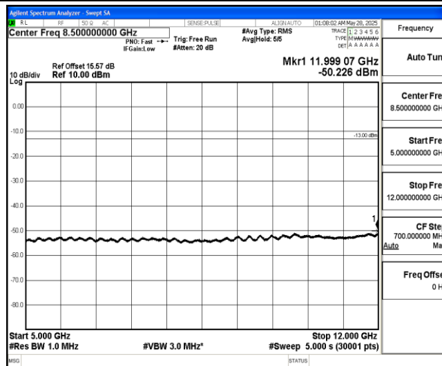
Band4-3MHz-QPSK-20385-1-0-High-5000-12000--50.23-PASS
