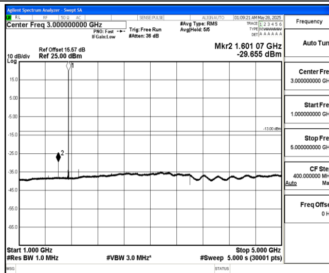
Band4-3MHz-16QAM-20385-1-0-High-1000-5000--29.66-PASS
