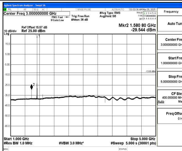
Band4-3MHz-QPSK-20175-1-0-Low-1000-5000--29.54-PASS
