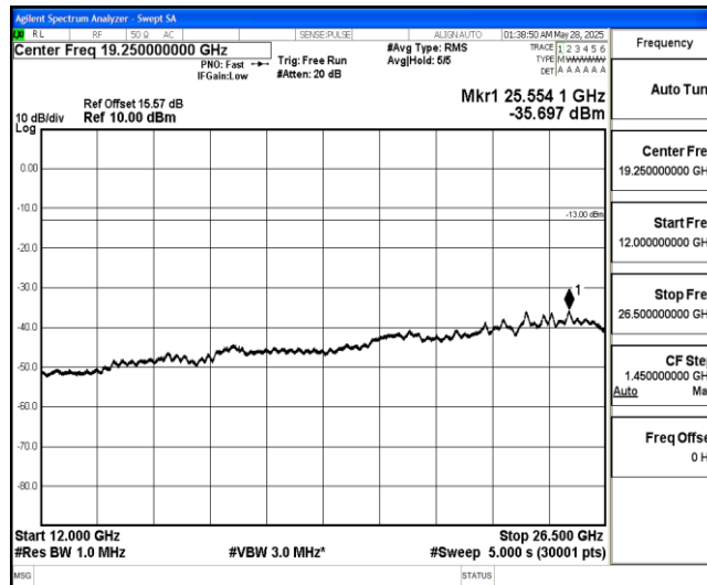
Band4-5MHz-16QAM-20375-1-0-High-12000-26500--35.7-PASS
