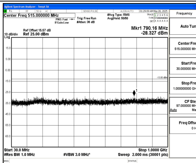
Band4-5MHz-16QAM-19975-1-0-Low-30-1000--28.33-PASS
