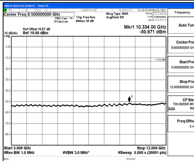
Band4-5MHz-QPSK-19975-1-0-Low-5000-12000--50.67-PASS
