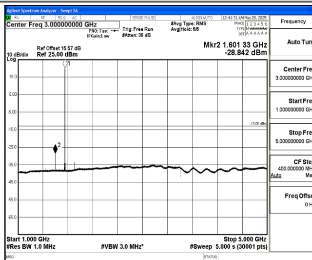
Band4-1.4MHz-16QAM-20393-1-0-High-1000-5000--28.84-PASS
