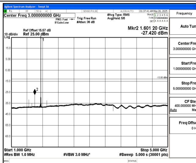
Band4-5MHz-16QAM-20375-1-0-High-1000-5000--27.42-PASS
