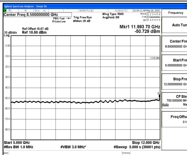
Band4-3MHz-QPSK-20175-1-0-Low-5000-12000--50.73-PASS
