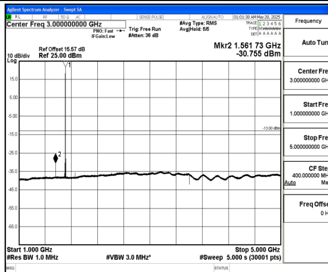
Band4-3MHz-16QAM-19965-1-0-Low-1000-5000--30.76-PASS
