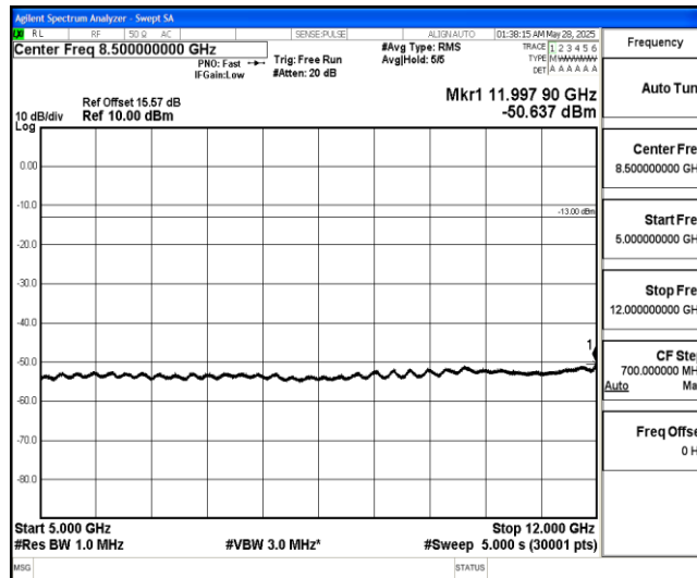
Band4-5MHz-16QAM-20375-1-0-High-5000-12000--50.64-PASS
