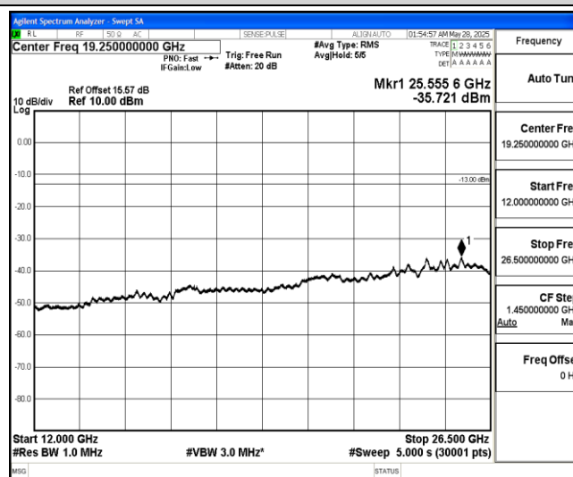
Band4-10MHz-QPSK-20000-1-0-Low-12000-26500--35.72-PASS
