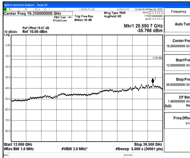
Band4-3MHz-16QAM-20175-1-0-Low-12000-26500--35.77-PASS
