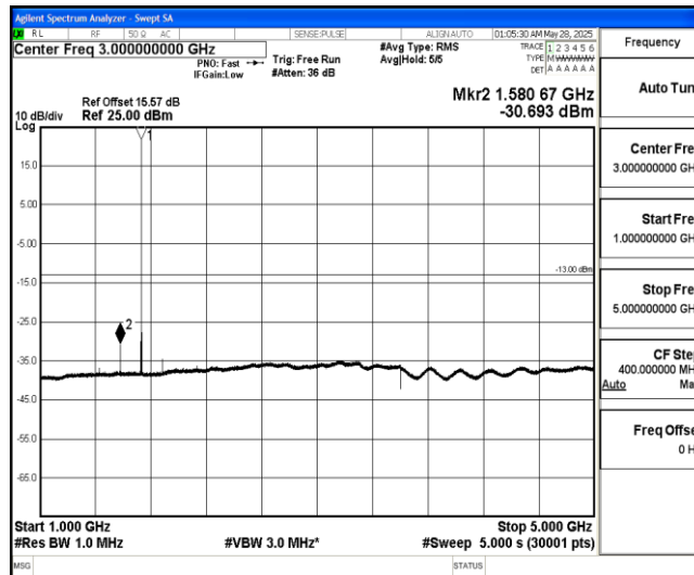
Band4-3MHz-16QAM-20175-1-0-Low-1000-5000--30.69-PASS
