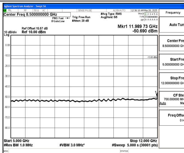
Band4-1.4MHz-QPSK-20175-1-0-Low-5000-12000--50.69-PASS
