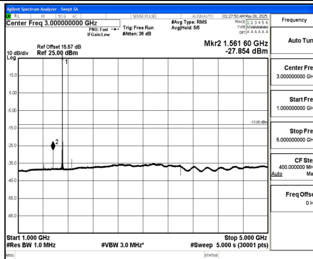
Band4-5MHz-QPSK-19975-1-0-Low-1000-5000--27.85-PASS
