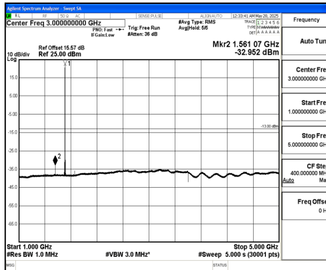
Band4-1.4MHz-16QAM-19957-1-0-Low-1000-5000--32.95-PASS
