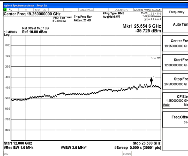
Band4-1.4MHz-QPSK-20175-1-0-Low-12000-26500--35.73-PASS
