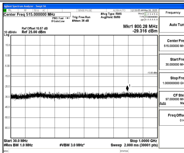
Band4-1.4MHz-16QAM-19957-1-0-Low-30-1000--29.32-PASS
