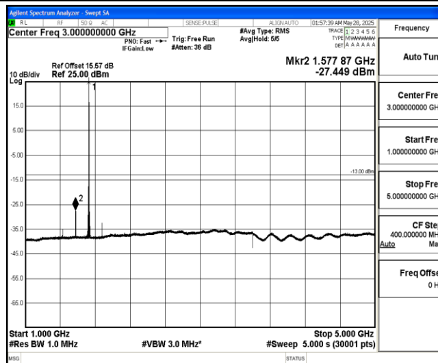
Band4-10MHz-QPSK-20175-1-0-Low-1000-5000--27.45-PASS
