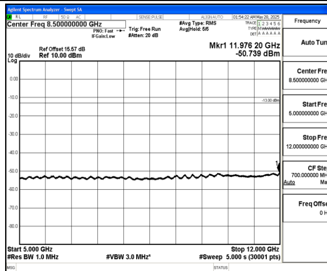
Band4-10MHz-QPSK-20000-1-0-Low-5000-12000--50.74-PASS
