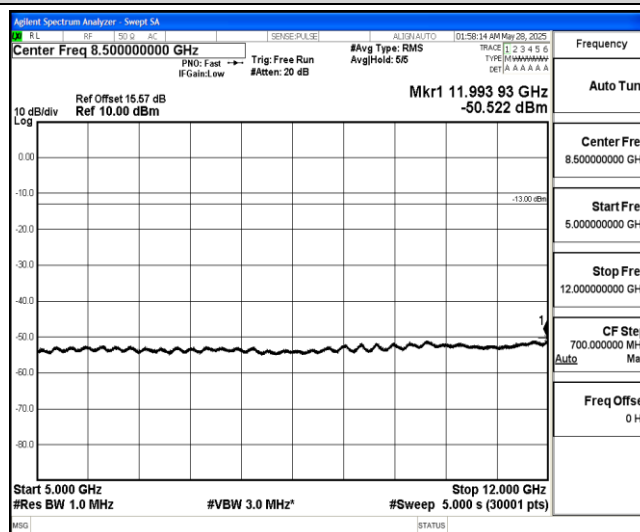
Band4-10MHz-QPSK-20175-1-0-Low-5000-12000--50.52-PASS
