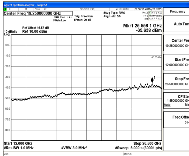
Band4-3MHz-QPSK-20385-1-0-High-12000-26500--35.64-PASS
