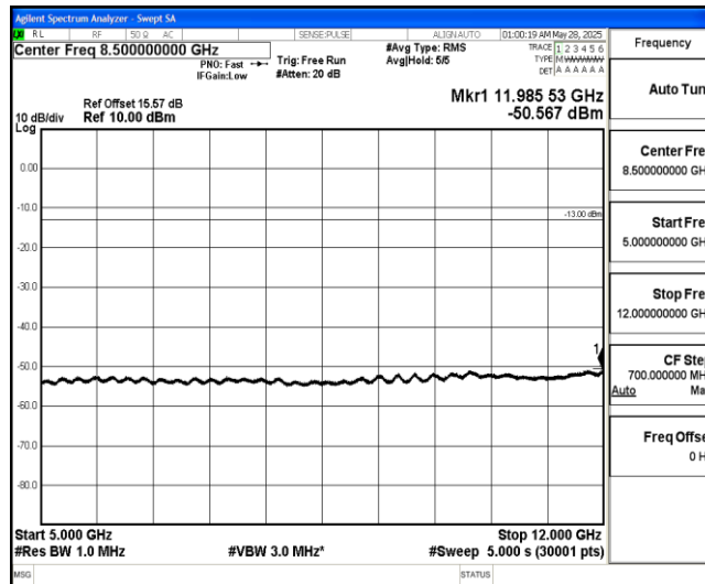
Band4-3MHz-QPSK-19965-1-0-Low-5000-12000--50.57-PASS
