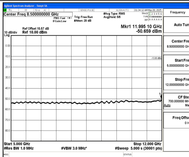
Band4-5MHz-16QAM-20175-1-0-Low-5000-12000--50.66-PASS
