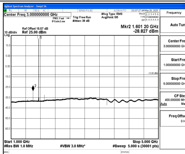
Band4-3MHz-QPSK-20385-1-0-High-1000-5000--28.83-PASS
