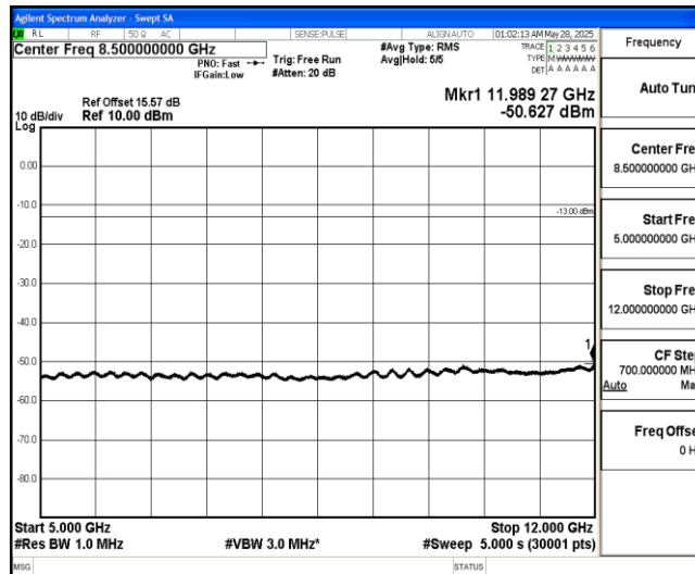
Band4-3MHz-16QAM-19965-1-0-Low-5000-12000--50.63-PASS
