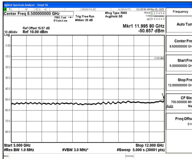
Band4-3MHz-16QAM-20385-1-0-High-5000-12000--50.66-PASS
