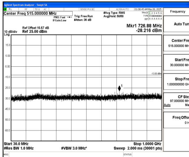
Band4-3MHz-16QAM-20385-1-0-High-30-1000--28.22-PASS
