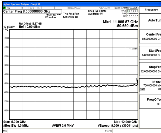
Band4-1.4MHz-16QAM-19957-1-0-Low-5000-12000--50.65-PASS
