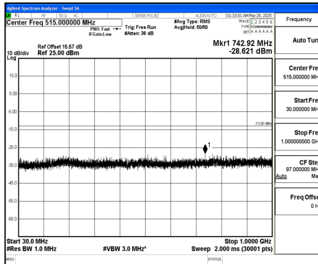
Band4-5MHz-16QAM-20175-1-0-Low-30-1000--28.62-PASS
