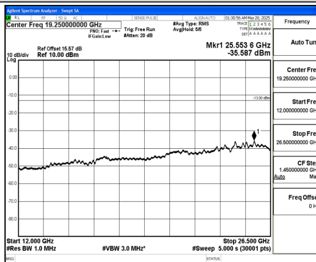
Band4-5MHz-16QAM-19975-1-0-Low-12000-26500--35.59-PASS
