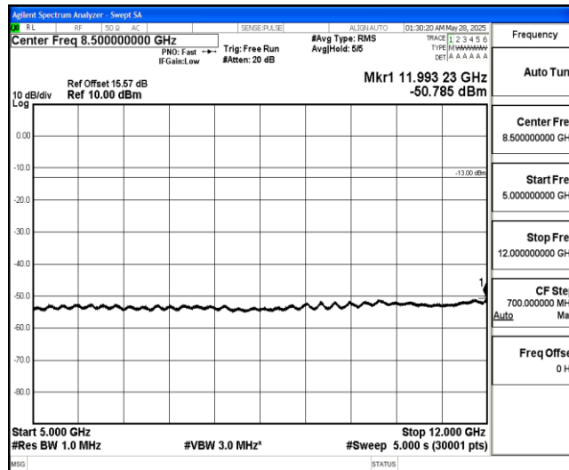
Band4-5MHz-16QAM-19975-1-0-Low-5000-12000--50.79-PASS
