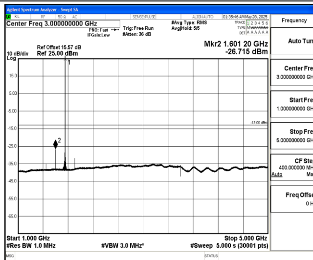
Band4-5MHz-QPSK-20375-1-0-High-1000-5000--26.72-PASS
