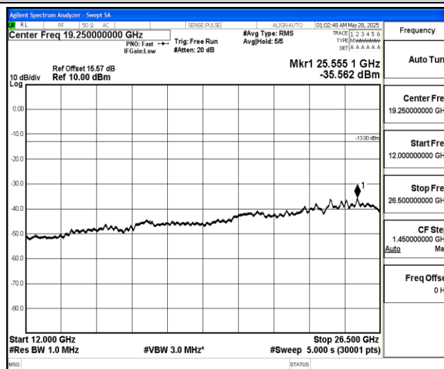
Band4-3MHz-16QAM-19965-1-0-Low-12000-26500--35.56-PASS
