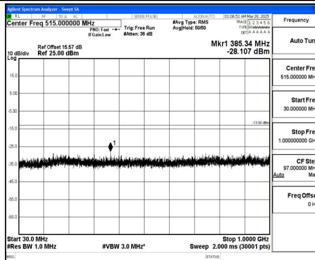
Band4-3MHz-QPSK-20385-1-0-High-30-1000--28.11-PASS
