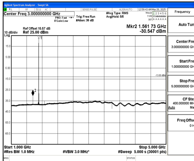
Band4-3MHz-QPSK-19965-1-0-Low-1000-5000--30.55-PASS
