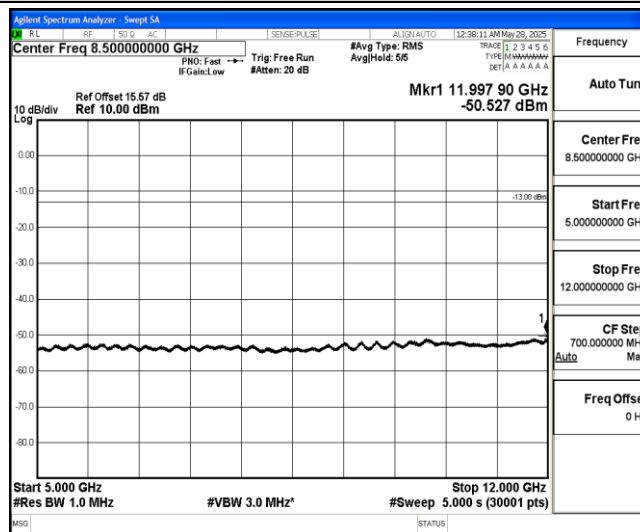
Band4-1.4MHz-16QAM-20175-1-0-Low-5000-12000--50.53-PASS
