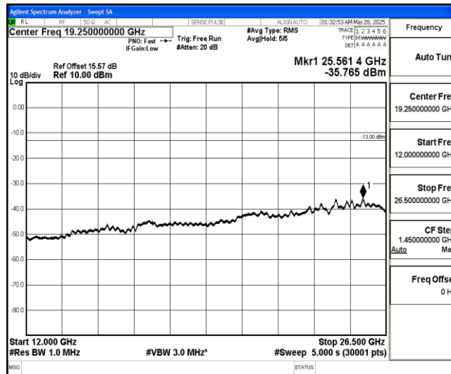
Band4-5MHz-QPSK-20175-1-0-Low-12000-26500--35.77-PASS
