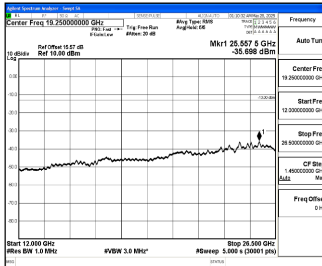
Band4-3MHz-16QAM-20385-1-0-High-12000-26500--35.7-PASS
