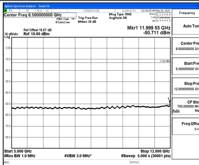
Band4-3MHz-16QAM-20175-1-0-Low-5000-12000--50.71-PASS
