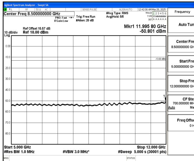
Band4-1.4MHz-16QAM-20393-1-0-High-5000-12000--50.8-PASS
