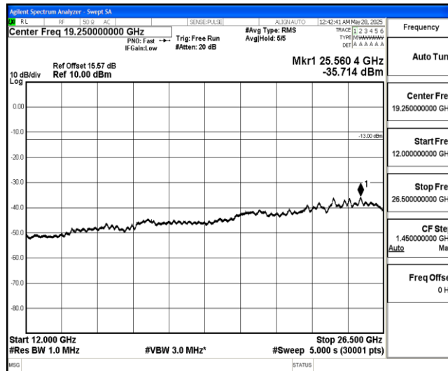
Band4-1.4MHz-16QAM-20393-1-0-High-12000-26500--35.71-PASS
