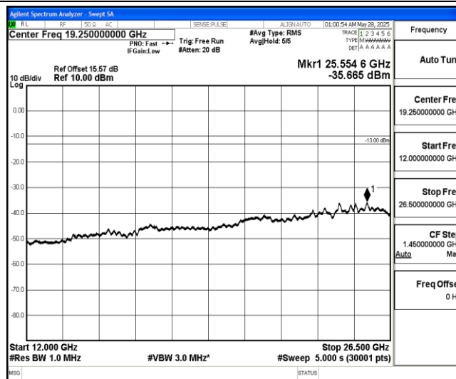
Band4-3MHz-QPSK-19965-1-0-Low-12000-26500--35.67-PASS
