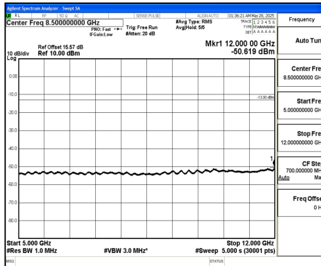
Band4-5MHz-QPSK-20375-1-0-High-5000-12000--50.62-PASS
