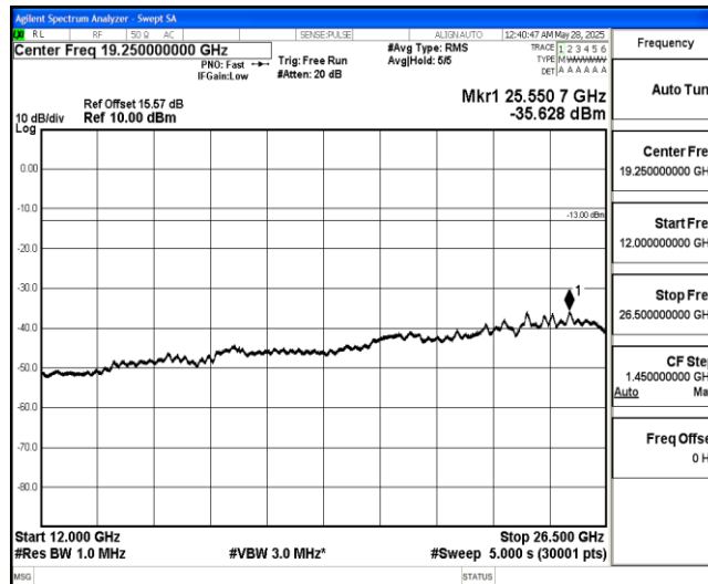
Band4-1.4MHz-QPSK-20393-1-0-High-12000-26500--35.63-PASS
