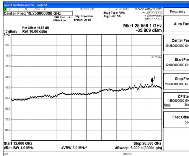
Band4-5MHz-QPSK-20375-1-0-High-12000-26500--35.81-PASS
