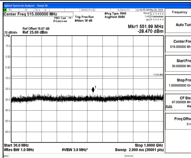
Band4-1.4MHz-16QAM-20393-1-0-High-30-1000--28.47-PASS
