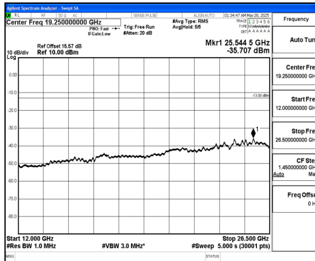
Band4-5MHz-16QAM-20175-1-0-Low-12000-26500--35.71-PASS
