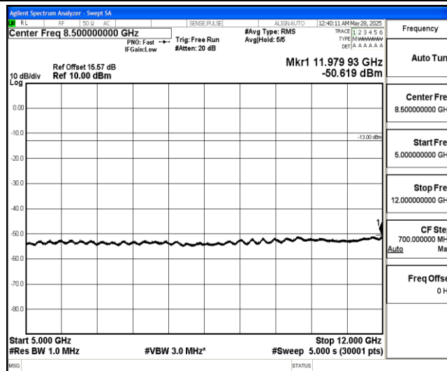
Band4-1.4MHz-QPSK-20393-1-0-High-5000-12000--50.62-PASS
