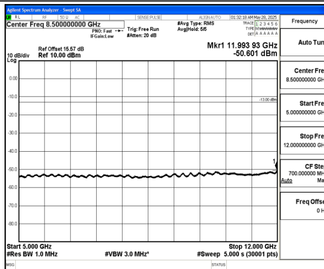
Band4-5MHz-QPSK-20175-1-0-Low-5000-12000--50.6-PASS
