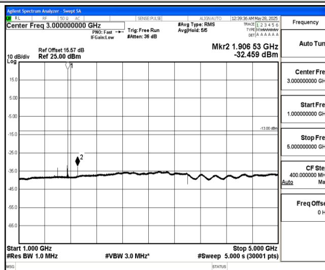
Band4-1.4MHz-QPSK-20393-1-0-High-1000-5000--32.46-PASS
