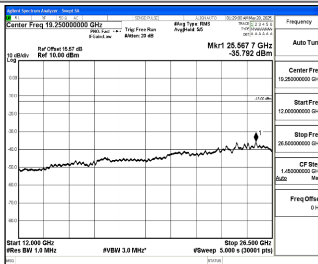
Band4-5MHz-QPSK-19975-1-0-Low-12000-26500--35.79-PASS
