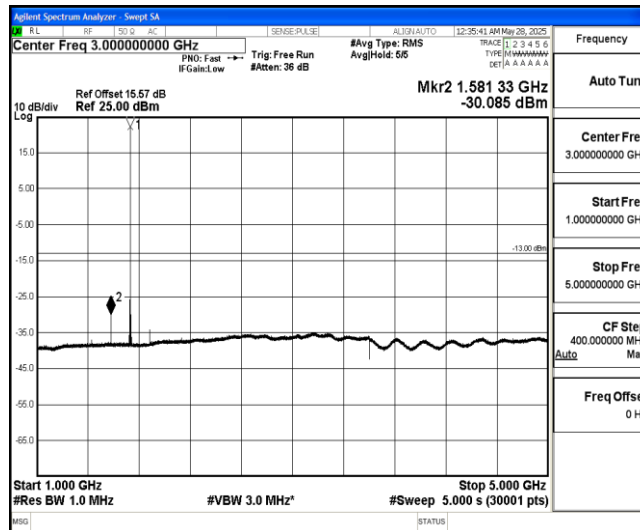
Band4-1.4MHz-QPSK-20175-1-0-Low-1000-5000--30.09-PASS
