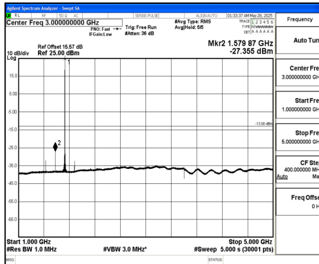
Band4-5MHz-16QAM-20175-1-0-Low-1000-5000--27.36-PASS
