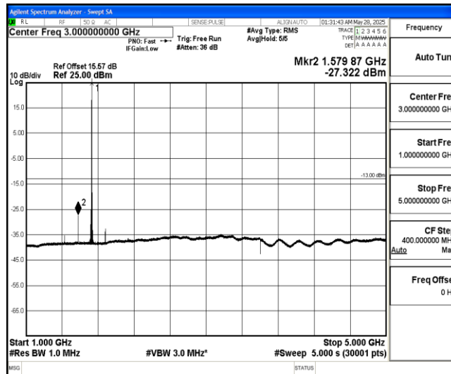
Band4-5MHz-QPSK-20175-1-0-Low-1000-5000--27.32-PASS
