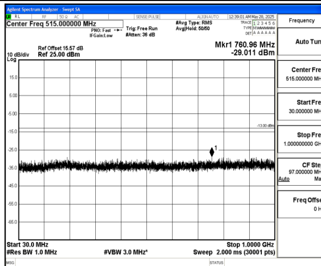
Band4-1.4MHz-QPSK-20393-1-0-High-30-1000--29.01-PASS
