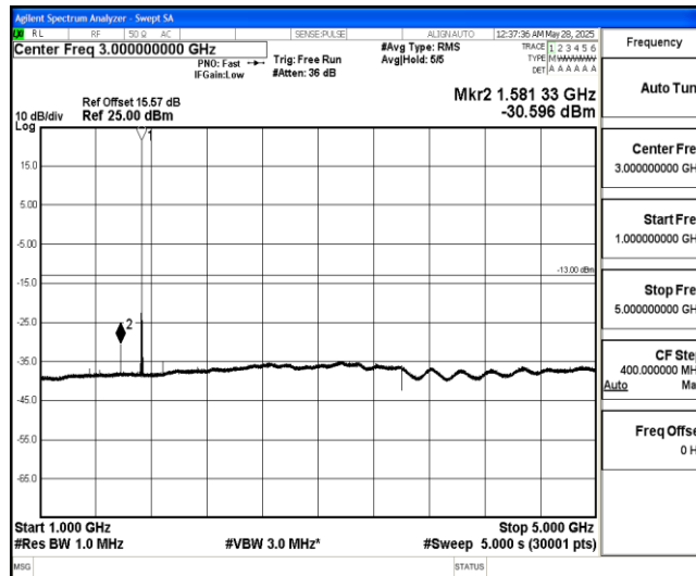
Band4-1.4MHz-16QAM-20175-1-0-Low-1000-5000--30.6-PASS
