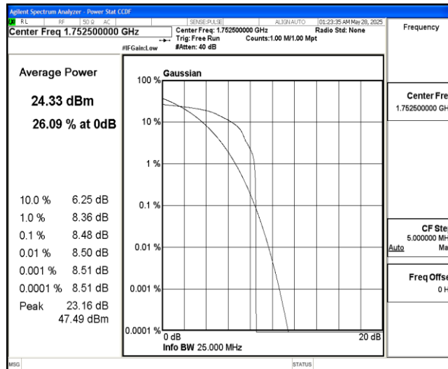
Band4-5MHz-16QAM-20375-1-0-High-8.48-&lt;=13-PASS
