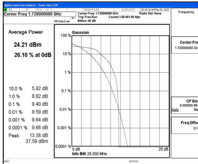
Band4-20MHz-QPSK-20050-6-0-Low-9.40-&lt;=13-PASS
