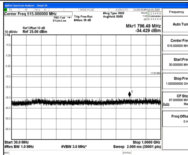
Band2-1.4MHz-QPSK-19193-1-0-High-30-1000--34.43-PASS
