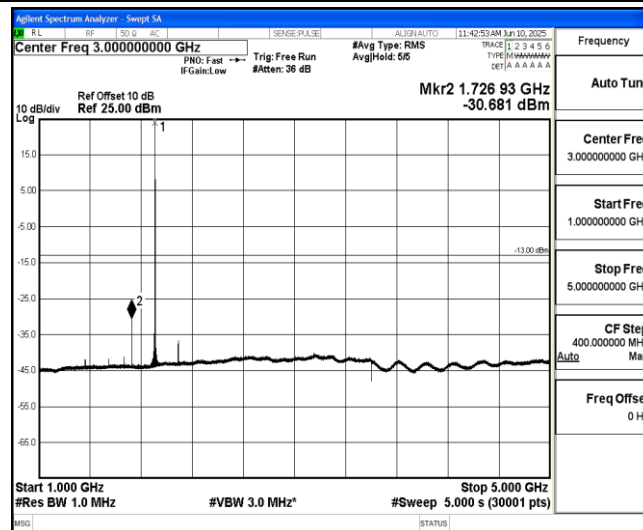
Band2-5MHz-QPSK-19175-1-0-High-1000-5000--30.68-PASS
