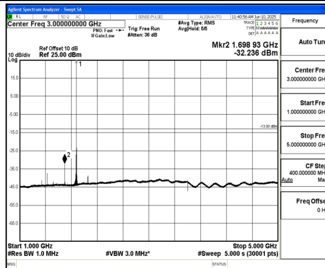
Band2-5MHz-16QAM-18900-1-0-Low-1000-5000--32.24-PASS
