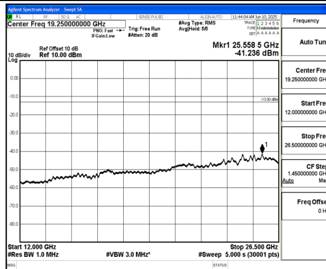
Band2-5MHz-QPSK-19175-1-0-High-12000-26500--41.24-PASS
