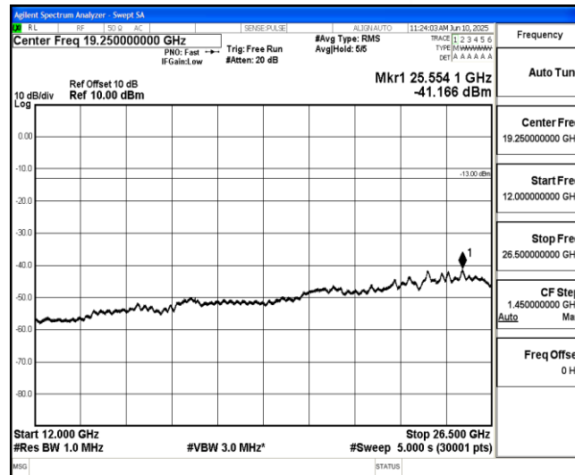
Band2-3MHz-16QAM-19185-1-0-High-12000-26500--41.17-PASS
