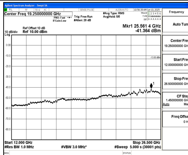
Band2-1.4MHz-QPSK-18607-1-0-Low-12000-26500--41.36-PASS
