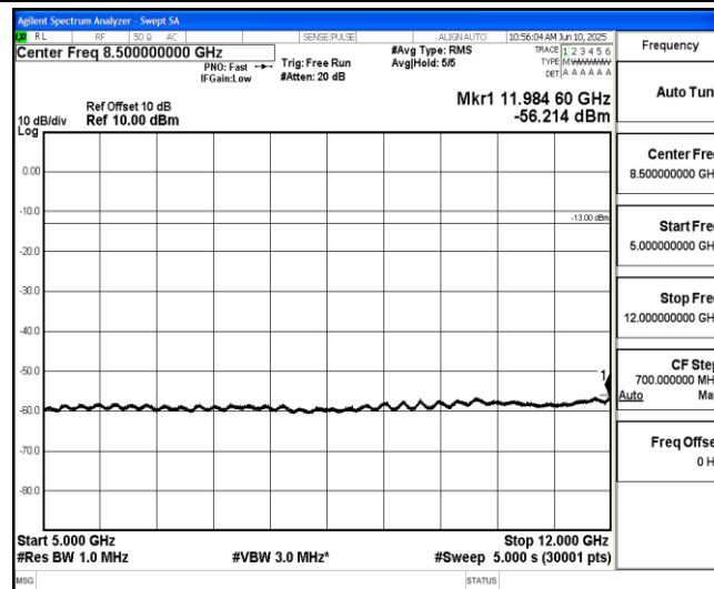
Band2-1.4MHz-QPSK-18607-1-0-Low-5000-12000--56.21-PASS
