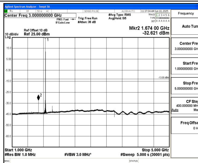
Band2-5MHz-16QAM-18625-1-0-Low-1000-5000--32.62-PASS
