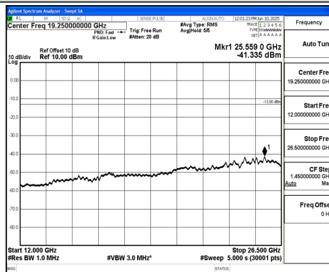
Band2-10MHz-QPSK-18900-1-0-Low-12000-26500--41.34-PASS
