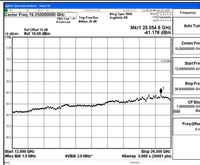
Band2-1.4MHz-16QAM-19193-1-0-High-12000-26500--41.18-PASS
