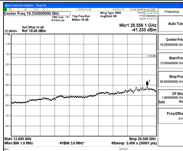
Band2-3MHz-16QAM-18615-1-0-Low-12000-26500--41.23-PASS
