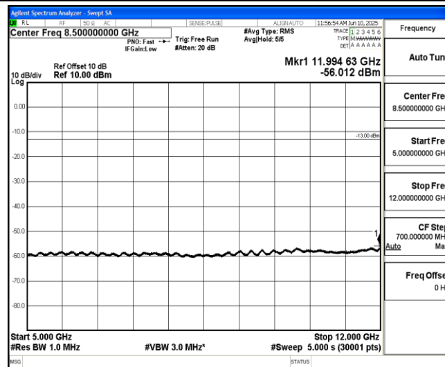
Band2-10MHz-QPSK-18650-1-0-Low-5000-12000--56.01-PASS
