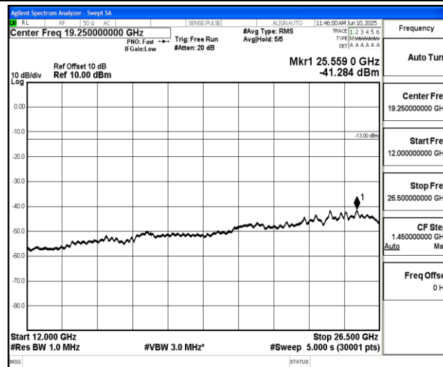
Band2-5MHz-16QAM-19175-1-0-High-12000-26500--41.28-PASS
