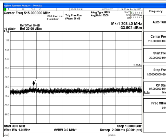
Band2-3MHz-16QAM-18900-1-0-Low-30-1000--33.9-PASS
