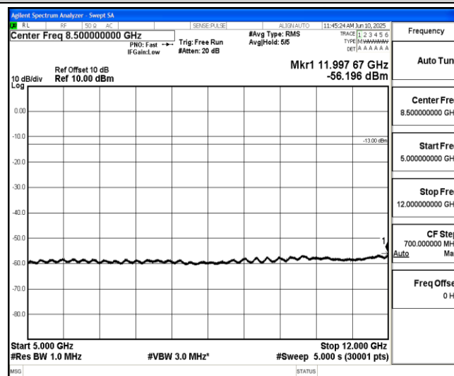
Band2-5MHz-16QAM-19175-1-0-High-5000-12000--56.2-PASS
