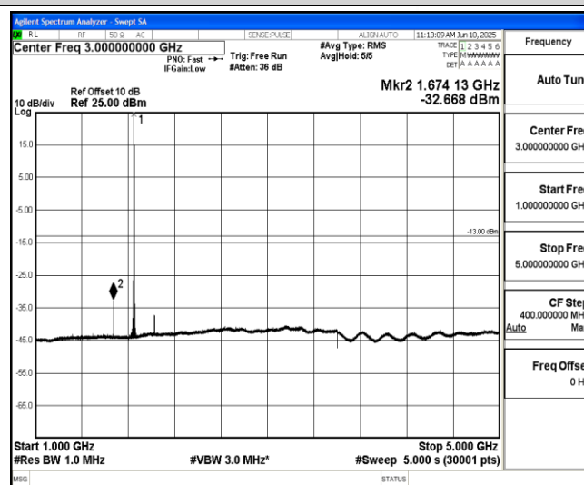
Band2-3MHz-QPSK-18615-1-0-Low-1000-5000--32.67-PASS
