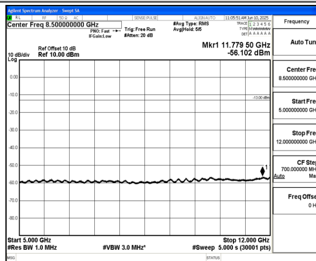
Band2-1.4MHz-16QAM-19193-1-0-High-5000-12000--56.1-PASS
