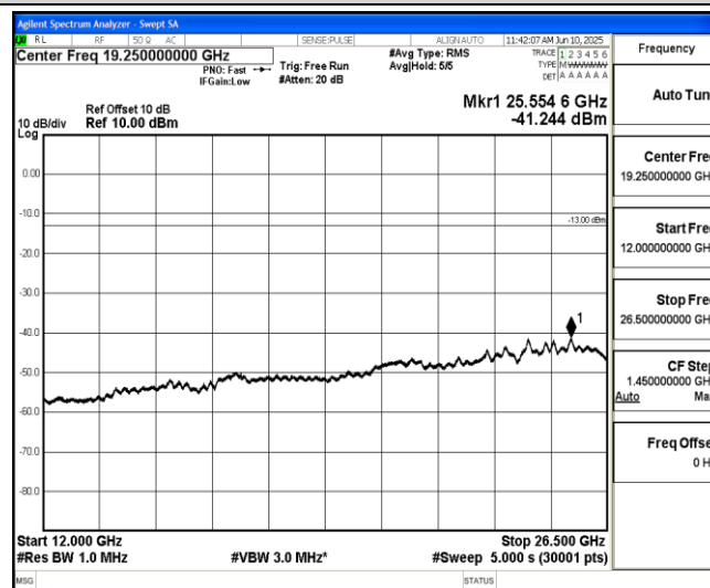
Band2-5MHz-16QAM-18900-1-0-Low-12000-26500--41.24-PASS
