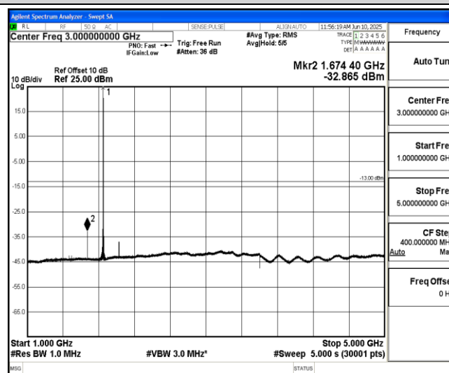
Band2-10MHz-QPSK-18650-1-0-Low-1000-5000--32.87-PASS
