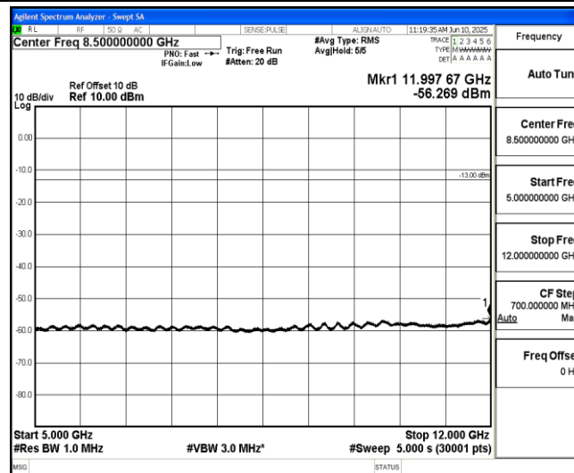
Band2-3MHz-16QAM-18900-1-0-Low-5000-12000--56.27-PASS
