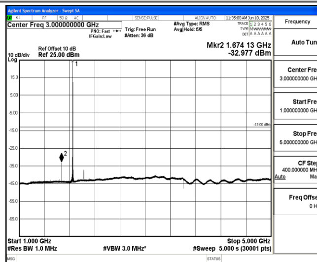
Band2-5MHz-QPSK-18625-1-0-Low-1000-5000--32.98-PASS
