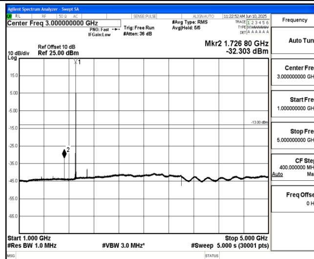
Band2-3MHz-16QAM-19185-1-0-High-1000-5000--32.3-PASS
