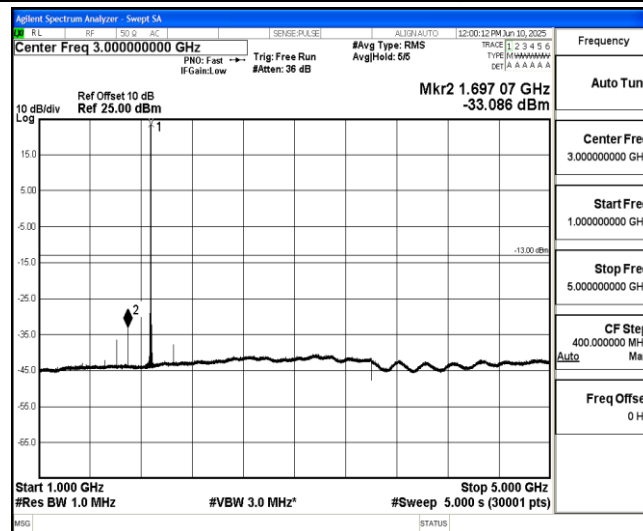
Band2-10MHz-QPSK-18900-1-0-Low-1000-5000--33.09-PASS
