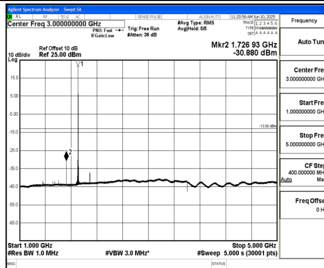
Band2-3MHz-QPSK-19185-1-0-High-1000-5000--30.88-PASS
