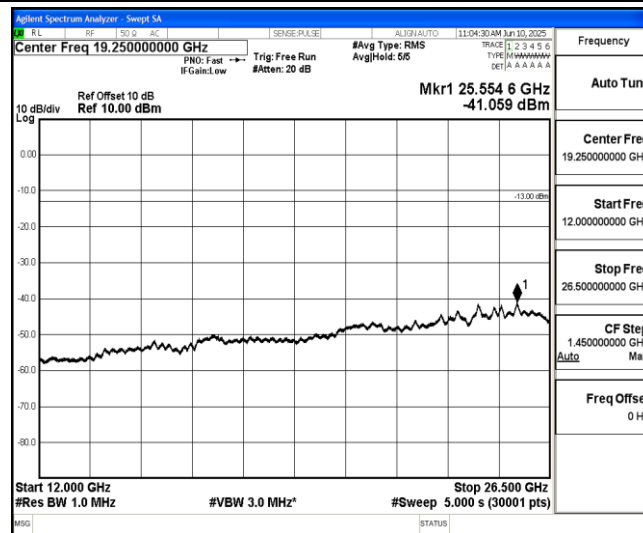
Band2-1.4MHz-QPSK-19193-1-0-High-12000-26500--41.06-PASS
