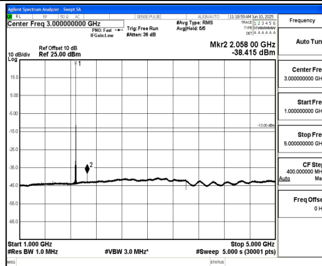
Band2-3MHz-16QAM-18900-1-0-Low-1000-5000--38.42-PASS
