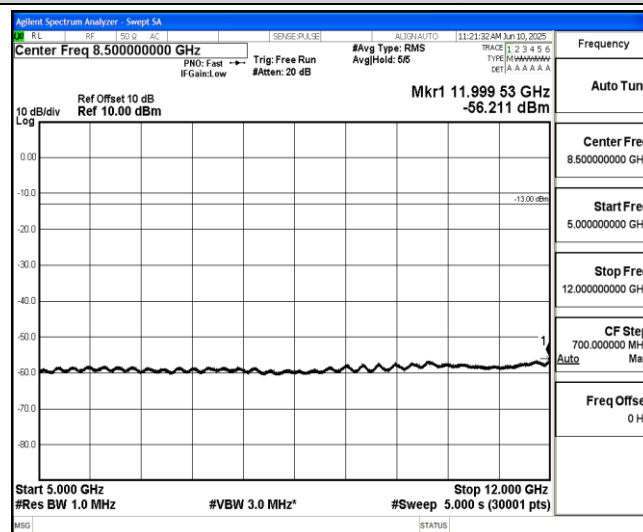
Band2-3MHz-QPSK-19185-1-0-High-5000-12000--56.21-PASS
