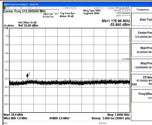
Band2-5MHz-QPSK-19175-1-0-High-30-1000--33.84-PASS
