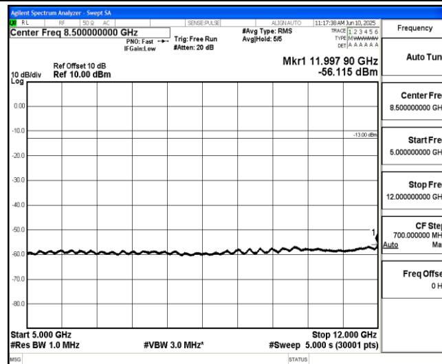
Band2-3MHz-QPSK-18900-1-0-Low-5000-12000--56.12-PASS
