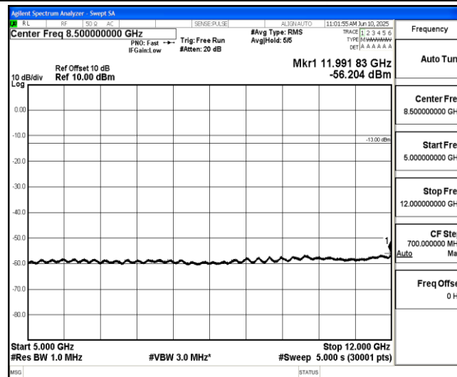
Band2-1.4MHz-16QAM-18900-1-0-Low-5000-12000--56.2-PASS
