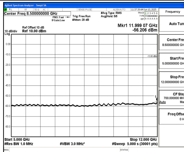
Band2-5MHz-16QAM-18625-1-0-Low-5000-12000--56.21-PASS
