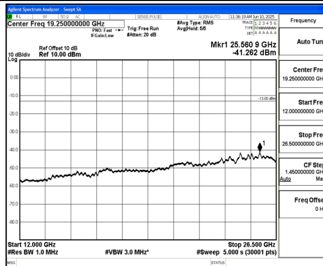
Band2-5MHz-QPSK-18625-1-0-Low-12000-26500--41.26-PASS
