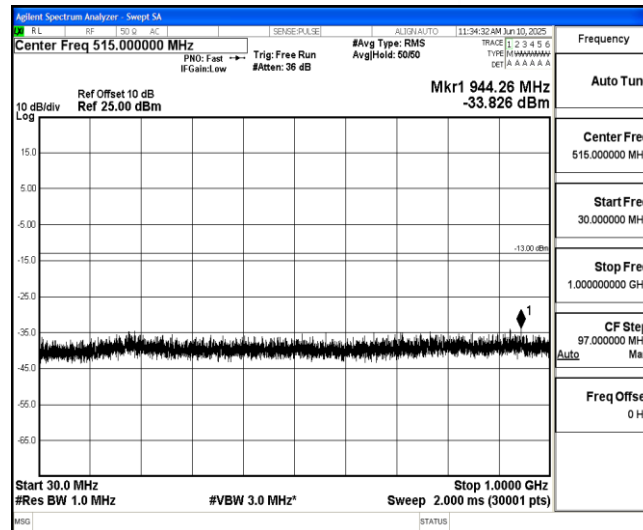
Band2-5MHz-QPSK-18625-1-0-Low-30-1000--33.83-PASS
