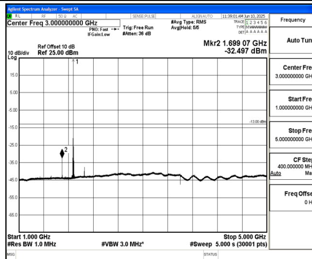
Band2-5MHz-QPSK-18900-1-0-Low-1000-5000--32.5-PASS
