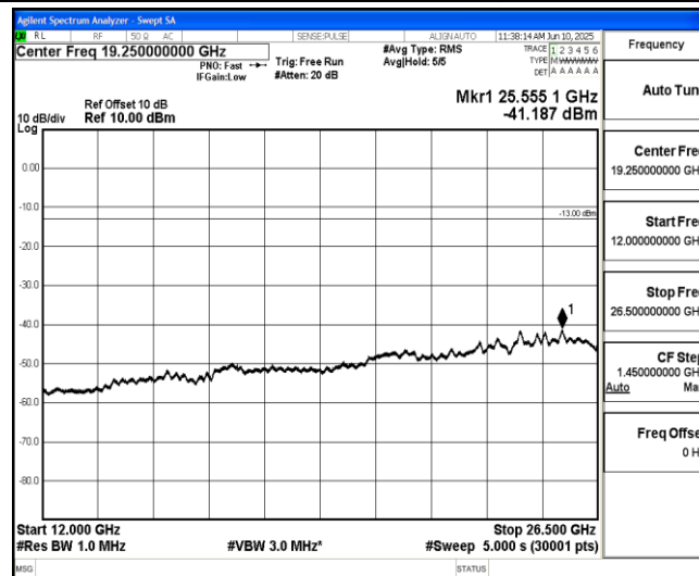
Band2-5MHz-16QAM-18625-1-0-Low-12000-26500--41.19-PASS
