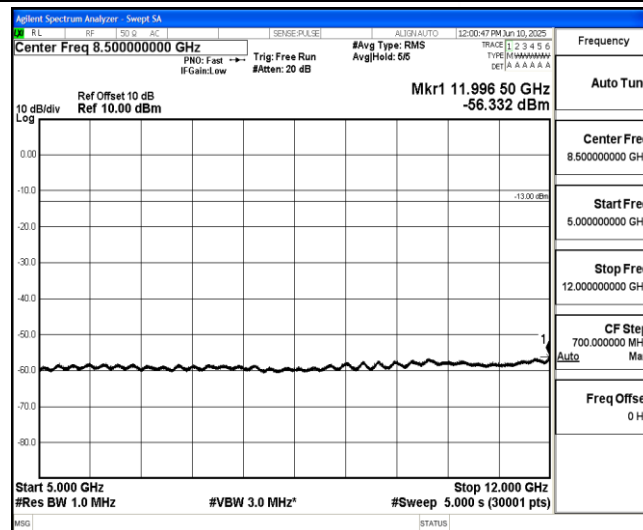
Band2-10MHz-QPSK-18900-1-0-Low-5000-12000--56.33-PASS
