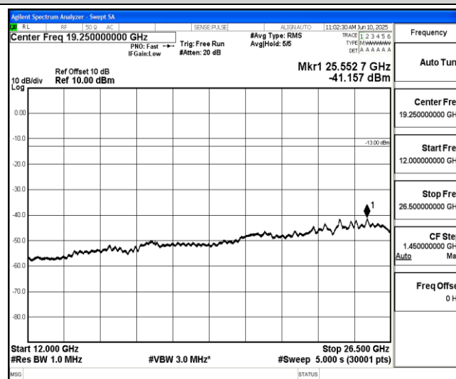
Band2-1.4MHz-16QAM-18900-1-0-Low-12000-26500--41.16-PASS
