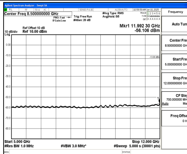
Band2-1.4MHz-QPSK-18900-1-0-Low-5000-12000--56.11-PASS
