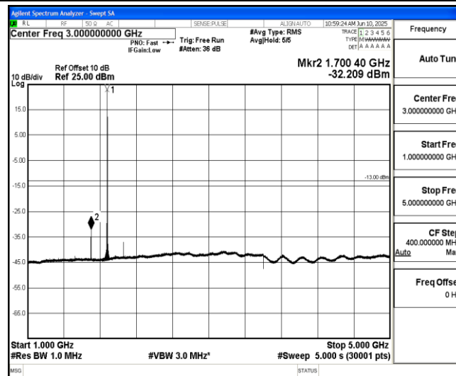
Band2-1.4MHz-QPSK-18900-1-0-Low-1000-5000--32.21-PASS
