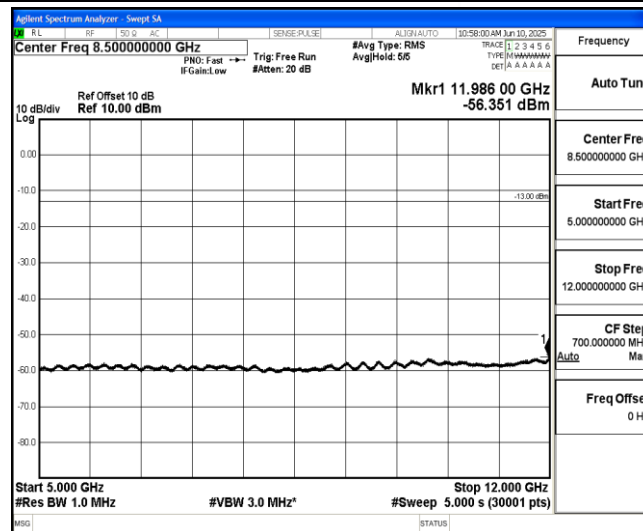
Band2-1.4MHz-16QAM-18607-1-0-Low-5000-12000--56.35-PASS
