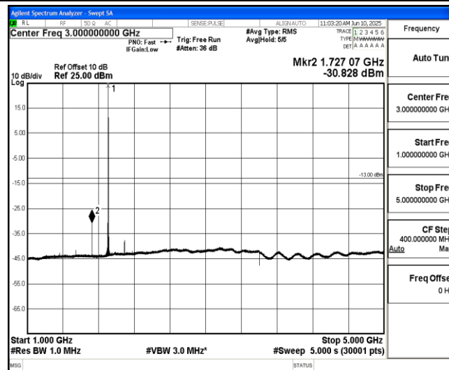
Band2-1.4MHz-QPSK-19193-1-0-High-1000-5000--30.83-PASS
