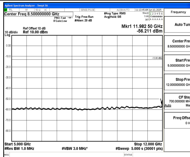
Band2-3MHz-QPSK-18615-1-0-Low-5000-12000--56.21-PASS
