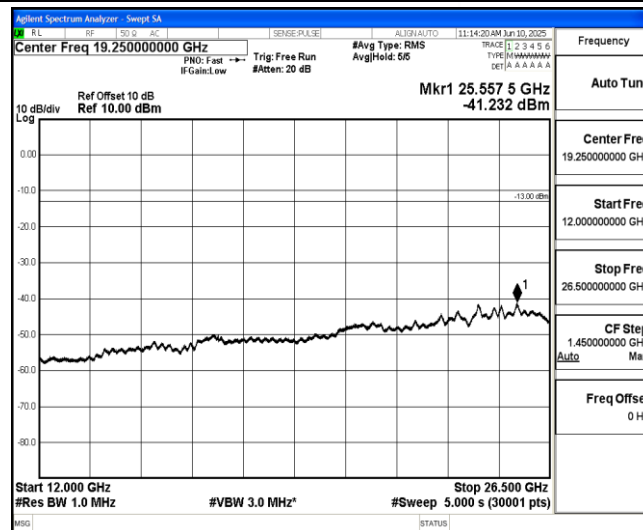
Band2-3MHz-QPSK-18615-1-0-Low-12000-26500--41.23-PASS
