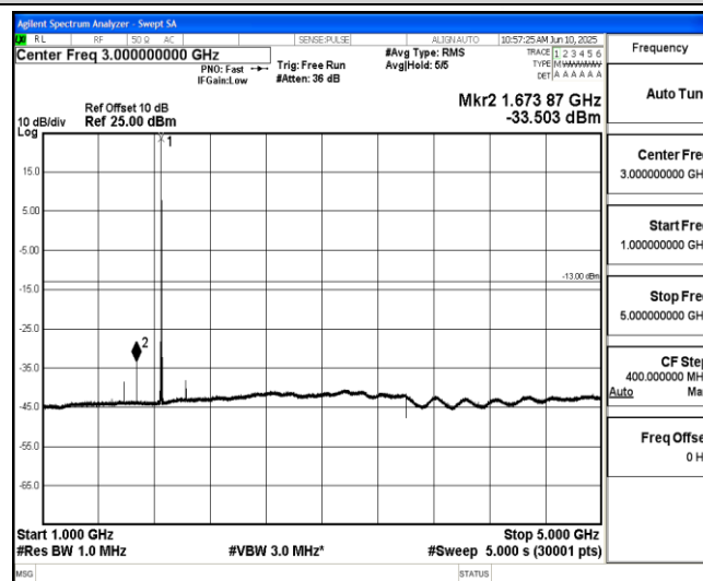
Band2-1.4MHz-16QAM-18607-1-0-Low-1000-5000--33.5-PASS
