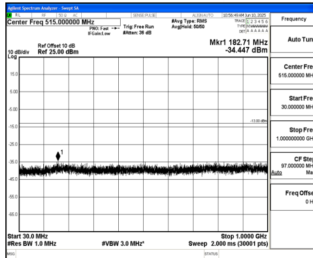
Band2-1.4MHz-16QAM-18607-1-0-Low-30-1000--34.45-PASS
