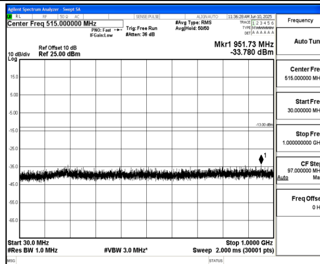
Band2-5MHz-16QAM-18625-1-0-Low-30-1000--33.78-PASS
