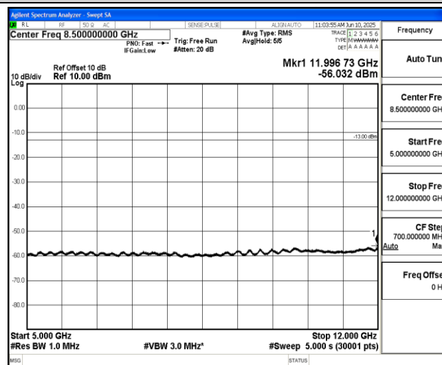
Band2-1.4MHz-QPSK-19193-1-0-High-5000-12000--56.03-PASS
