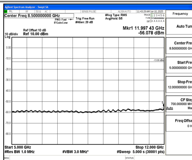
Band2-5MHz-QPSK-19175-1-0-High-5000-12000--56.08-PASS
