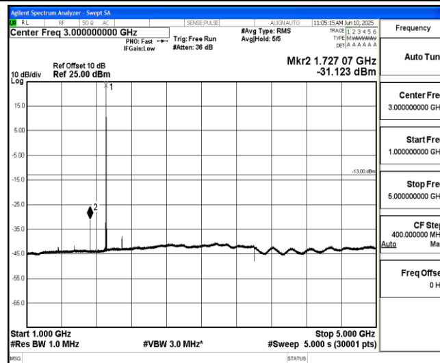
Band2-1.4MHz-16QAM-19193-1-0-High-1000-5000--31.12-PASS
