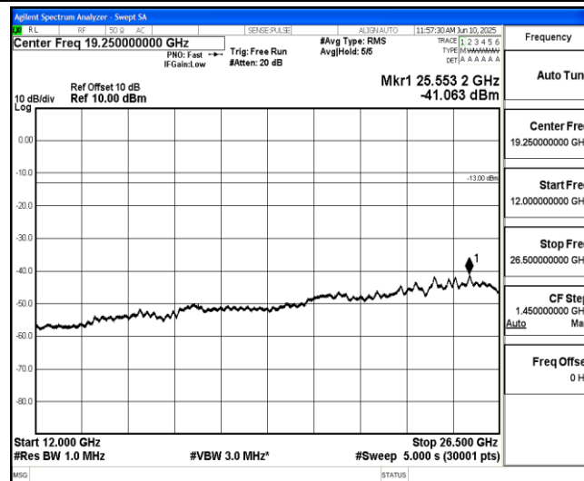
Band2-10MHz-QPSK-18650-1-0-Low-12000-26500--41.06-PASS
