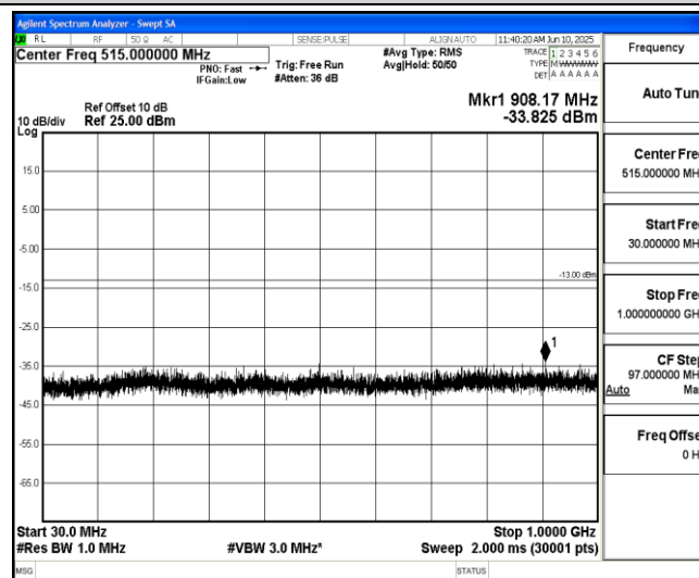
Band2-5MHz-16QAM-18900-1-0-Low-30-1000--33.83-PASS
