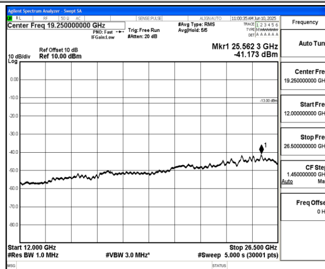
Band2-1.4MHz-QPSK-18900-1-0-Low-12000-26500--41.17-PASS
