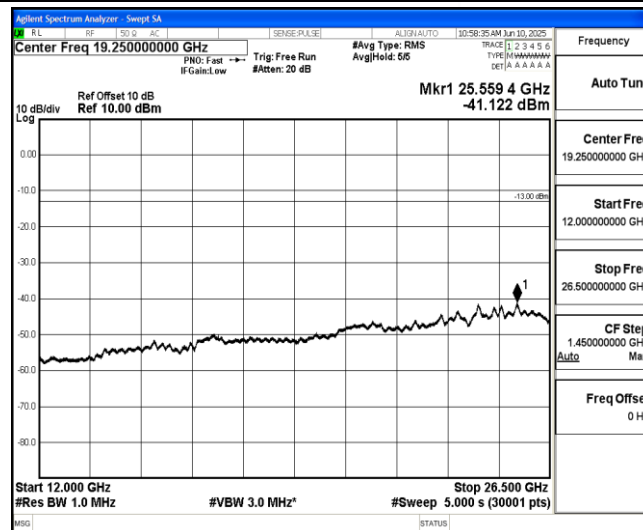
Band2-1.4MHz-16QAM-18607-1-0-Low-12000-26500--41.12-PASS
