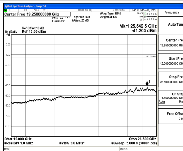
Band2-5MHz-QPSK-18900-1-0-Low-12000-26500--41.2-PASS
