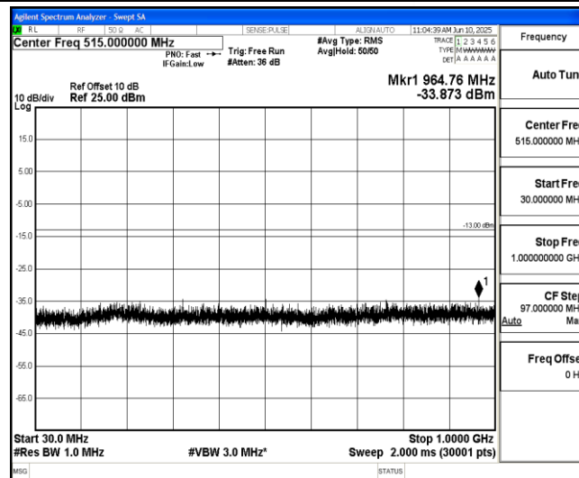
Band2-1.4MHz-16QAM-19193-1-0-High-30-1000--33.87-PASS
