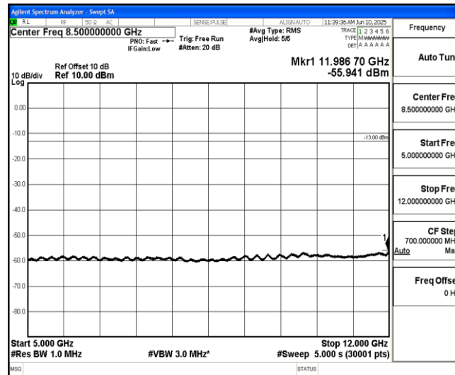
Band2-5MHz-QPSK-18900-1-0-Low-5000-12000--55.94-PASS
