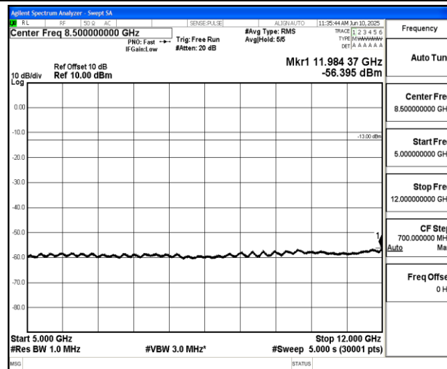
Band2-5MHz-QPSK-18625-1-0-Low-5000-12000--56.4-PASS
