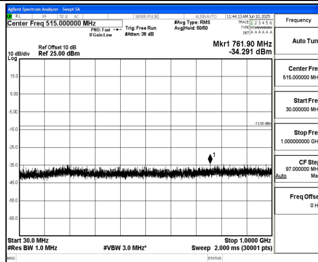
Band2-5MHz-16QAM-19175-1-0-High-30-1000--34.29-PASS
