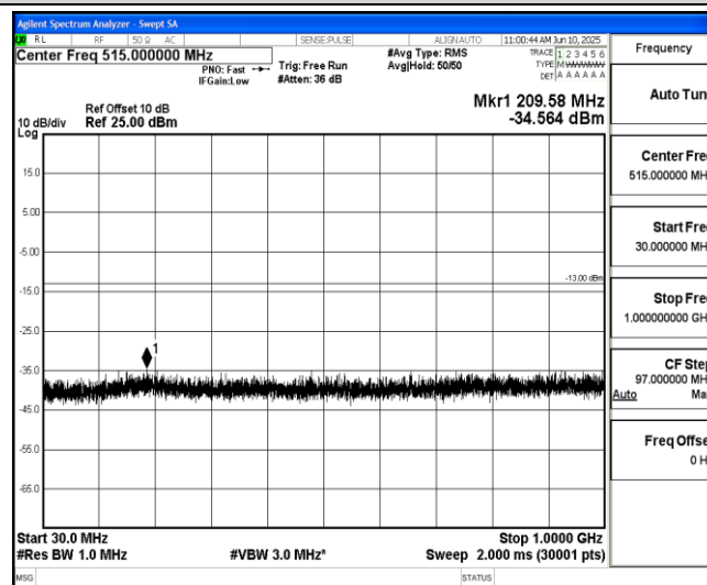
Band2-1.4MHz-16QAM-18900-1-0-Low-30-1000--34.56-PASS
