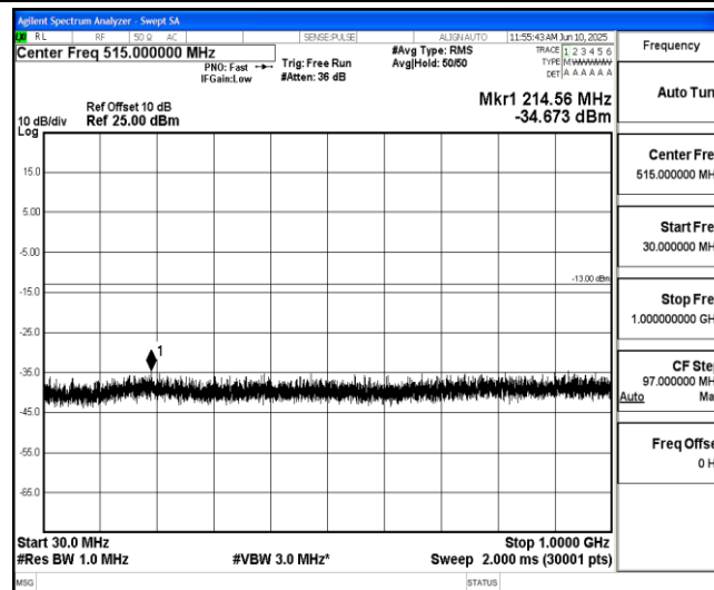
Band2-10MHz-QPSK-18650-1-0-Low-30-1000--34.67-PASS
