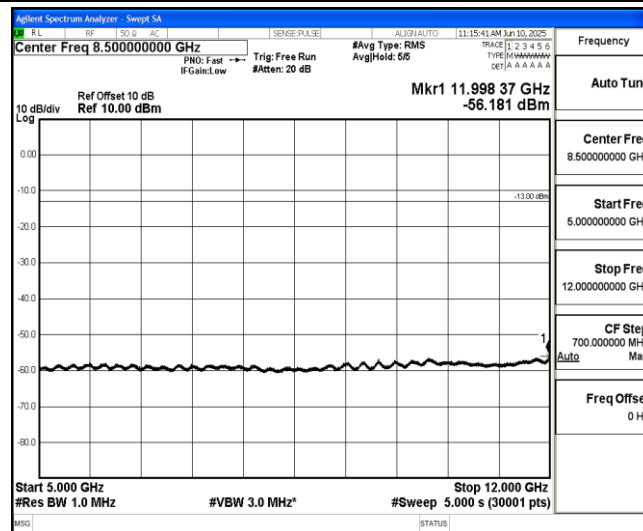
Band2-3MHz-16QAM-18615-1-0-Low-5000-12000--56.18-PASS
