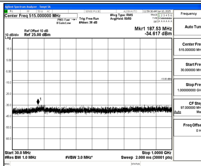
Band2-10MHz-QPSK-18900-1-0-Low-30-1000--34.62-PASS
