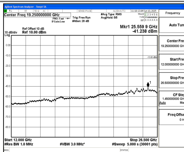
Band2-3MHz-QPSK-18900-1-0-Low-12000-26500--41.24-PASS
