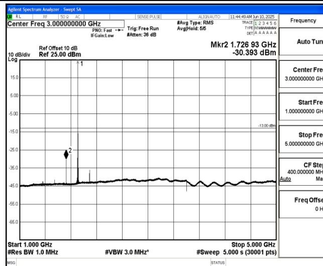
Band2-5MHz-16QAM-19175-1-0-High-1000-5000--30.39-PASS
