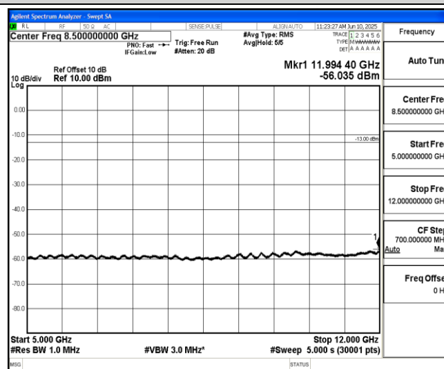
Band2-3MHz-16QAM-19185-1-0-High-5000-12000--56.04-PASS
