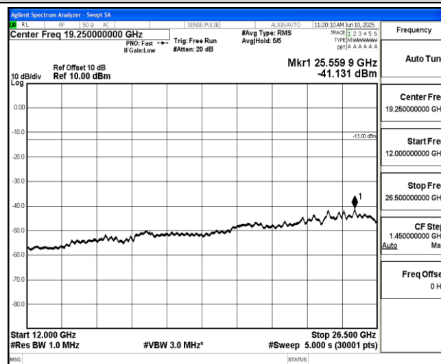
Band2-3MHz-16QAM-18900-1-0-Low-12000-26500--41.13-PASS
