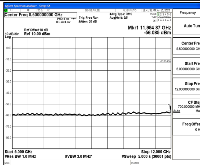
Band2-5MHz-16QAM-18900-1-0-Low-5000-12000--56.09-PASS
