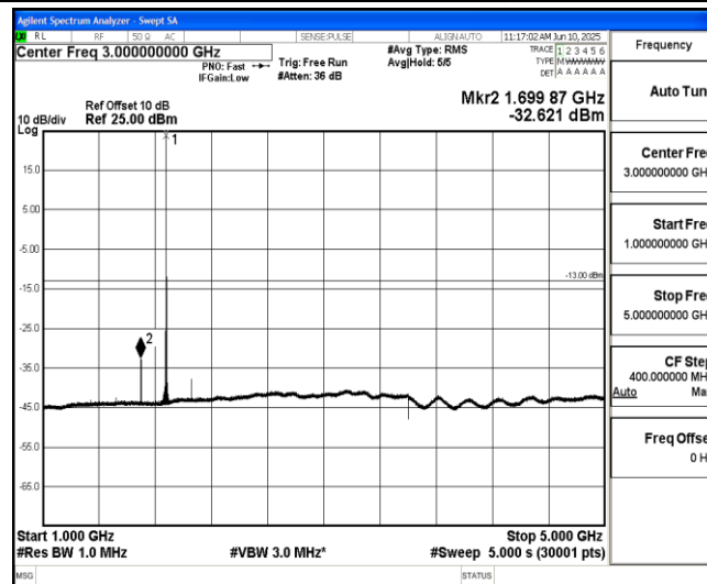
Band2-3MHz-QPSK-18900-1-0-Low-1000-5000--32.62-PASS
