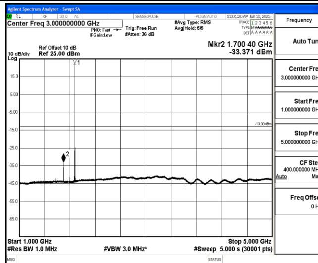
Band2-1.4MHz-16QAM-18900-1-0-Low-1000-5000--33.37-PASS
