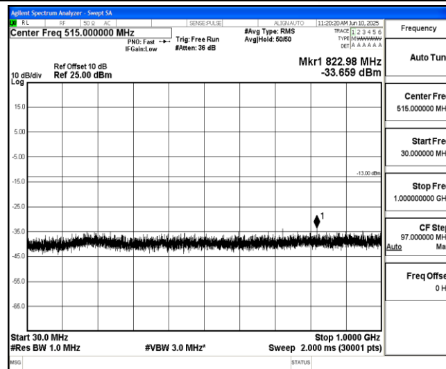
Band2-3MHz-QPSK-19185-1-0-High-30-1000--33.66-PASS
