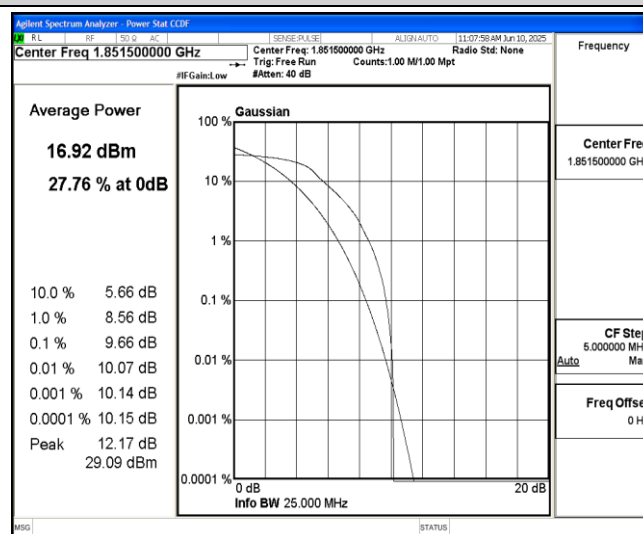
Band2-3MHz-16QAM-18615-6-0-Low-9.66-&lt;=13-PASS
