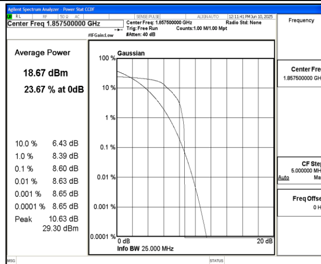
Band2-15MHz-QPSK-18675-1-0-Low-8.60-&lt;=13-PASS
