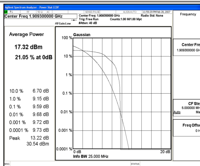
Band2-1.4MHz-QPSK-19193-1-0-High-9.59-&lt;=13-PASS
