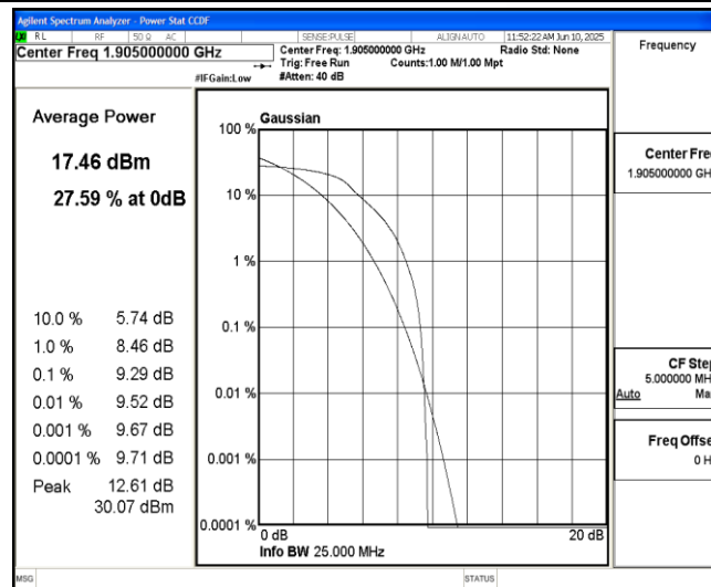
Band2-10MHz-16QAM-19150-6-0-High-9.29-&lt;=13-PASS
