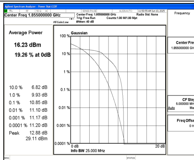
Band2-10MHz-QPSK-18650-6-0-Low-10.85-&lt;=13-PASS
