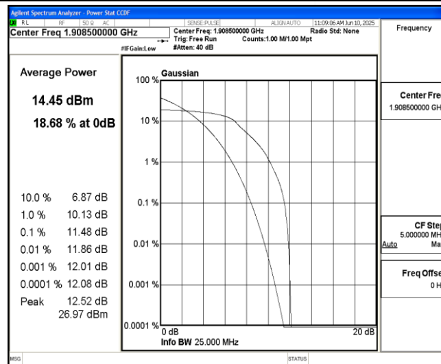
Band2-3MHz-QPSK-19185-6-0-High-11.48-&lt;=13-PASS
