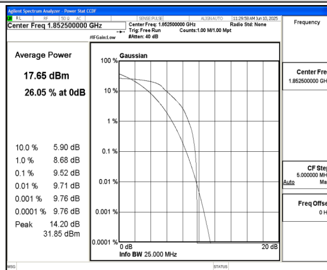
Band2-5MHz-16QAM-18625-6-0-Low-9.52-&lt;=13-PASS
