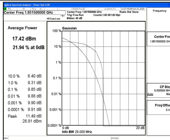
Band2-3MHz-16QAM-18615-1-0-Low-9.85-&lt;=13-PASS
