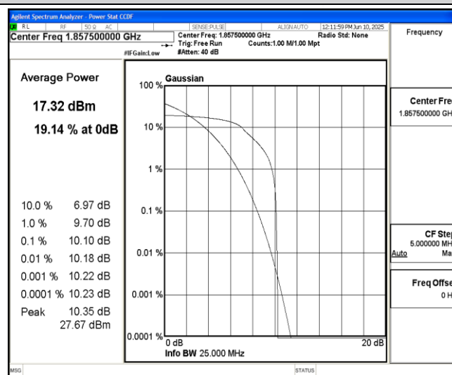
Band2-15MHz-QPSK-18675-6-0-Low-10.10-&lt;=13-PASS
