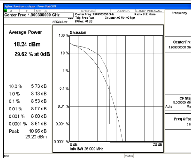
Band2-1.4MHz-16QAM-19193-1-0-High-8.53-&lt;=13-PASS
