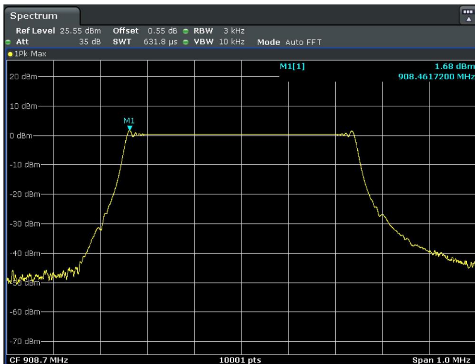
Figure 12. Antenna-Port Conducted Measurements, Maximum Peak Power Spectral Density: Mid Channel, 908.7 MHz Plot
