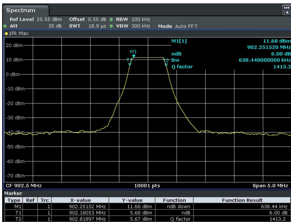
Figure 2. Antenna-Port Conducted Measurements, 6dB DTS Bandwidth: Low Channel, 902.5 MHz Plot
