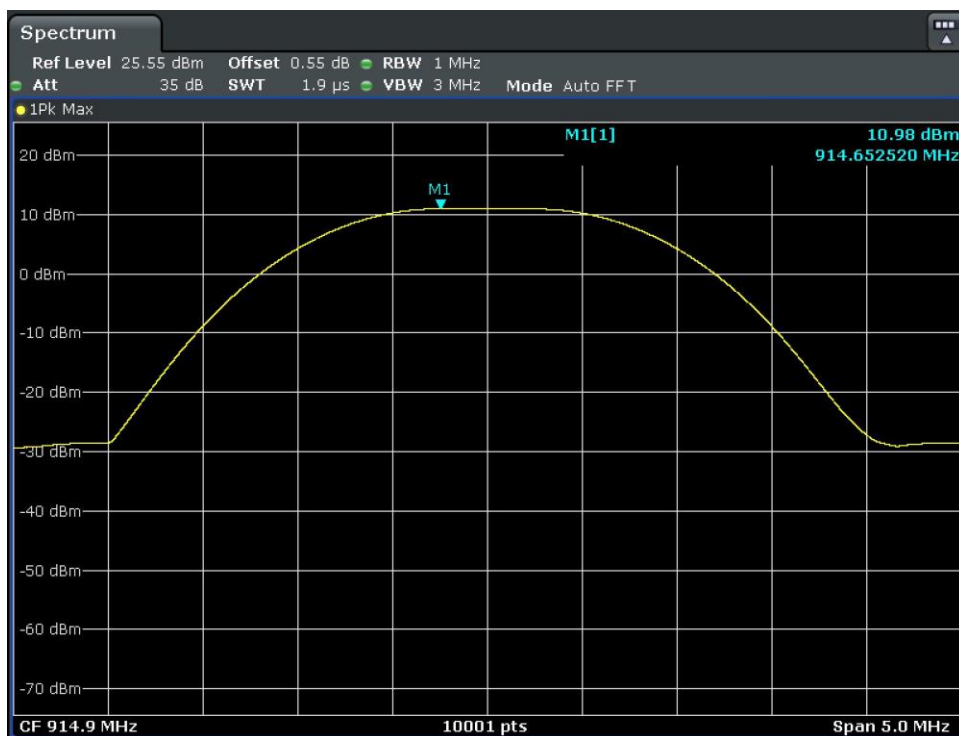
Figure 10. Antenna-Port Conducted Measurements, Maximum Peak Conducted Output Power: High Channel, 914.9 MHz Plot
