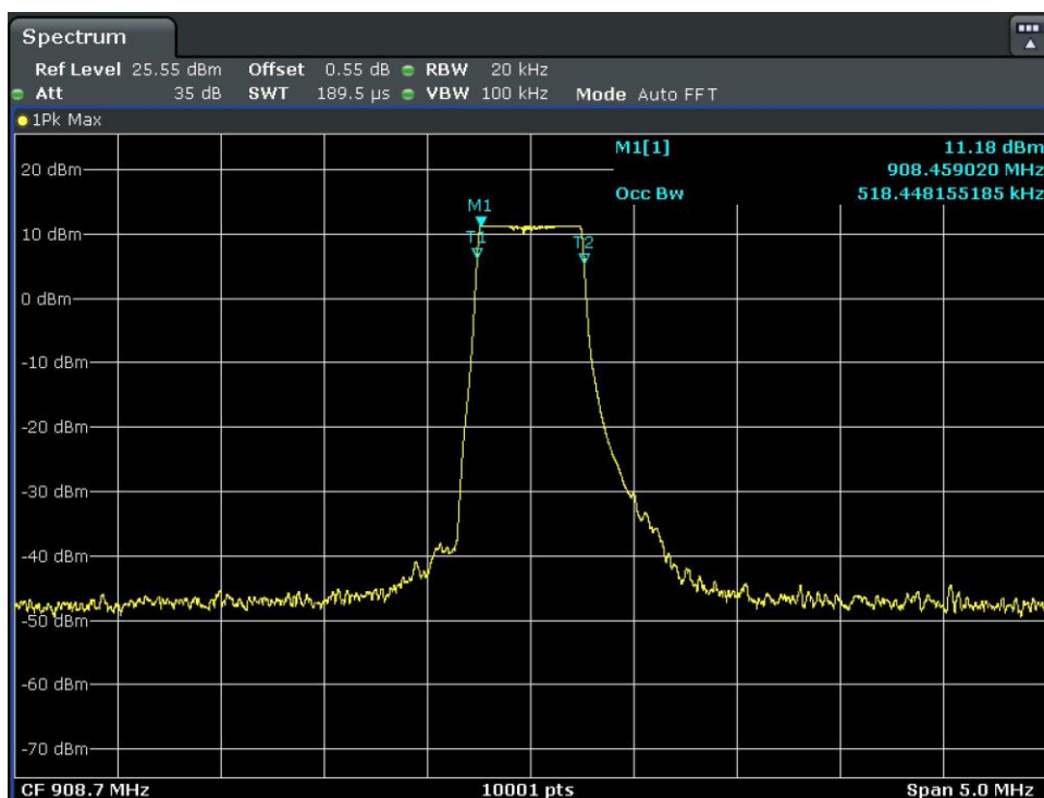
Figure 6. Antenna-Port Conducted Measurements, 99% OBW: Mid Channel, 908.7 MHz Plot
