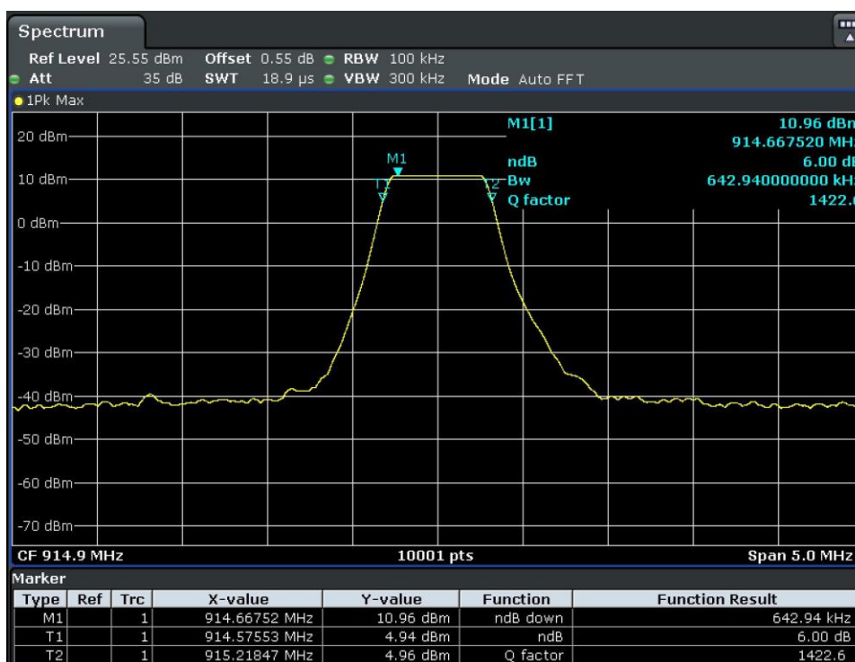
Figure 4. Antenna-Port Conducted Measurements, 6dB DTS Bandwidth: High Channel, 914.9 MHz Plot
