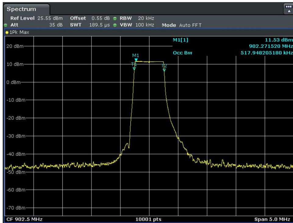
Figure 5. Antenna-Port Conducted Measurements, 99% OBW: Low Channel, 902.5 MHz Plot
