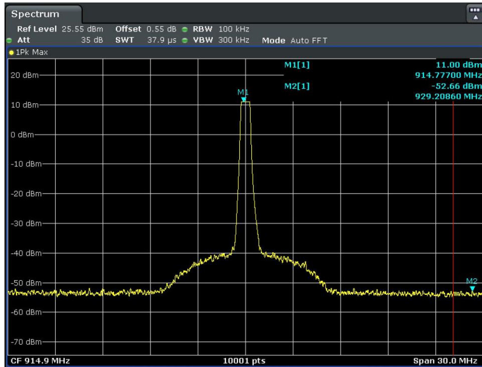
Figure 21. Antenna-Port Conducted Measurements, Upper Band Edge: High Channel, 914.9 MHz Plot
