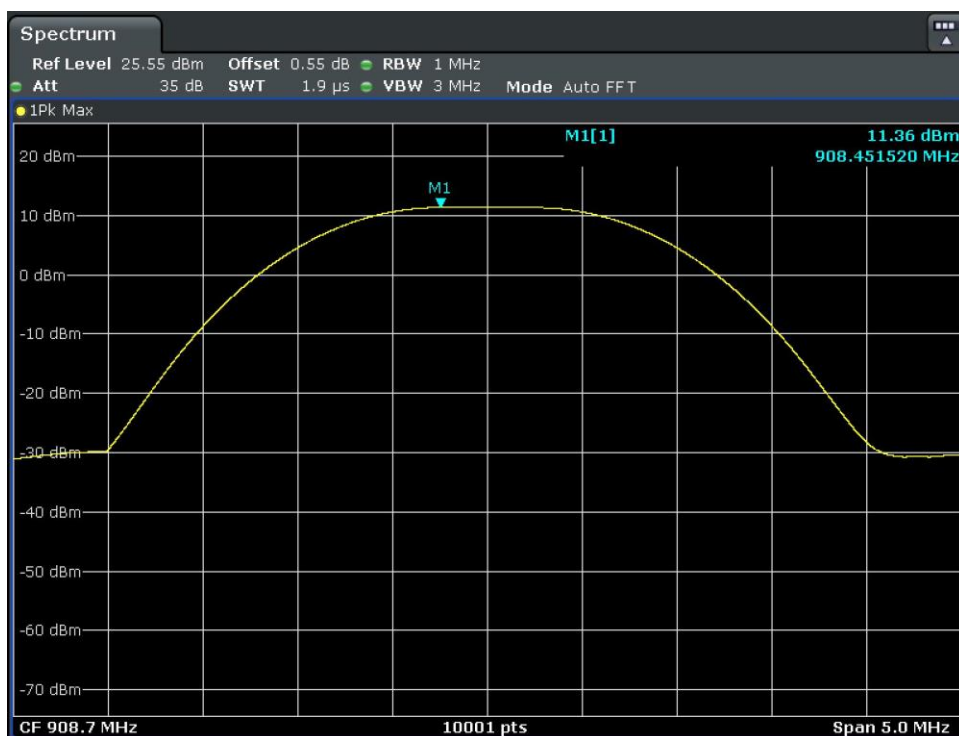
Figure 9. Antenna-Port Conducted Measurements, Maximum Peak Conducted Output Power: Mid Channel, 908.7 MHz Plot
