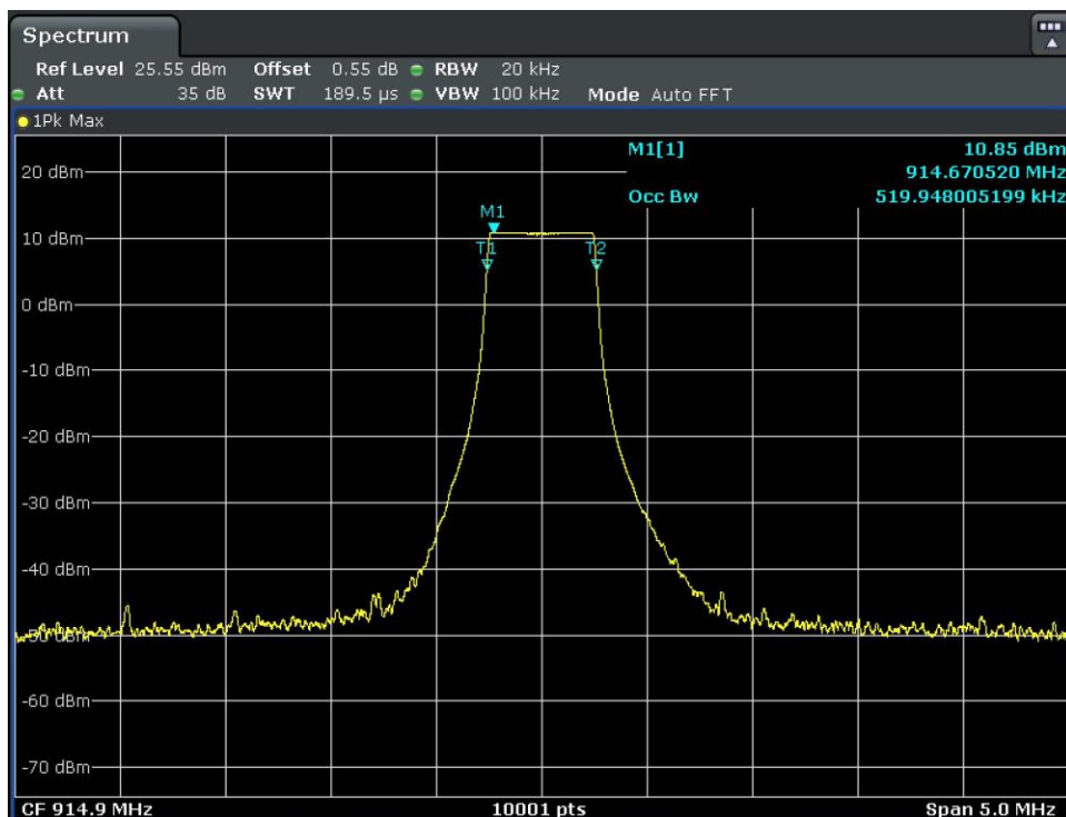
Figure 7. Antenna-Port Conducted Measurements, 99% OBW: High Channel, 914.9 MHz Plot
