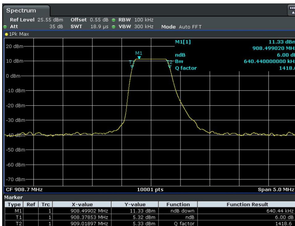
Figure 3. Antenna-Port Conducted Measurements, 6dB DTS Bandwidth: Mid Channel, 908.7 MHz Plot
