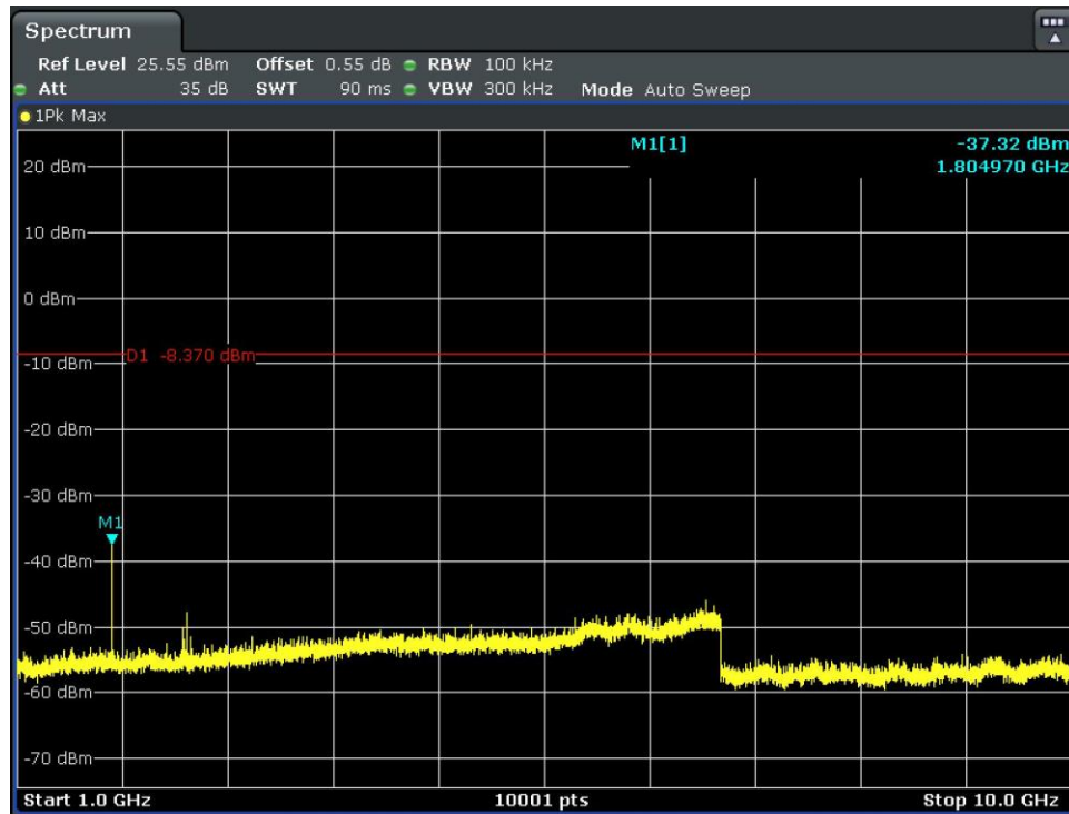
Figure 15. Antenna-Port Conducted Measurements, Conducted Spurious Emissions: Low Channel, 902.5 MHz Plot
