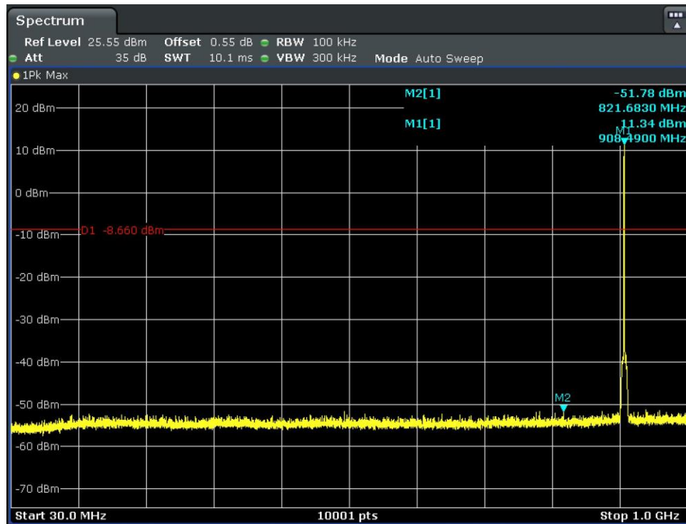
Figure 16. Antenna-Port Conducted Measurements, Conducted Spurious Emissions: Mid Channel, 908.7 MHz Plot
