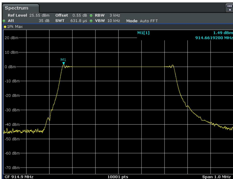
Figure 13. Antenna-Port Conducted Measurements, Maximum Peak Power Spectral Density: High Channel, 914.9 MHz Plot
