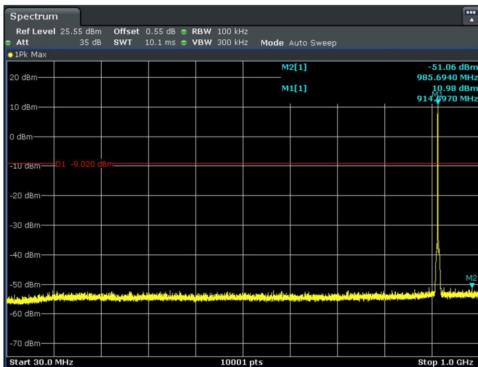
Figure 18. Antenna-Port Conducted Measurements, Conducted Spurious Emissions: High Channel, 914.9 MHz Plot
