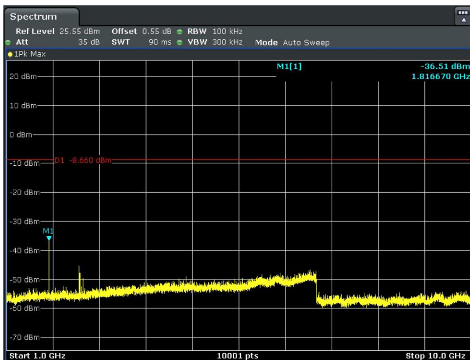
Figure 17. Antenna-Port Conducted Measurements, Conducted Spurious Emissions: Mid Channel, 908.7 MHz Plot
