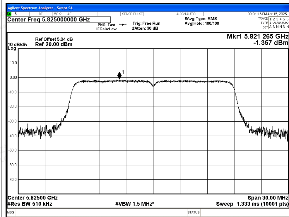
PSD NVNT n20 5825MHz Ant
