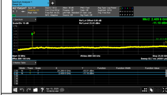
30.0 MHz - 25000.0 MHz IEEE 802.11n Channel 1 20MHz Antenna 0
