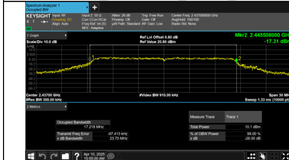
IEEE 802.11g Channel 6 20MHz Antenna 0
