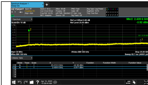
30.0 MHz - 25000.0 MHz IEEE 802.11b Channel 6 20MHz Antenna 0
