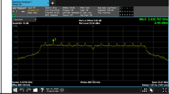
In-Band Reference Level IEEE 802.11g Channel 6 20MHz Antenna 0
