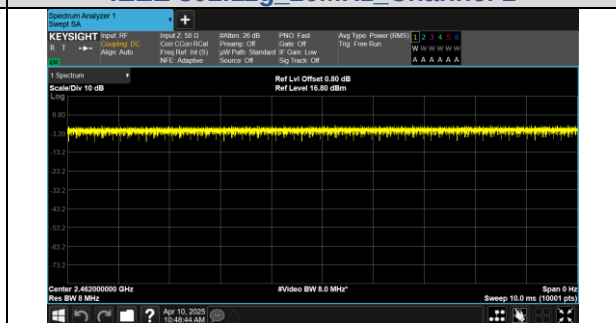
IEEE 802.11g 20MHz Channel 11
