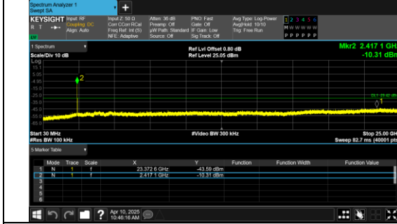
30.0 MHz - 25000.0 MHz IEEE 802.11g Channel 1 20MHz Antenna 0
