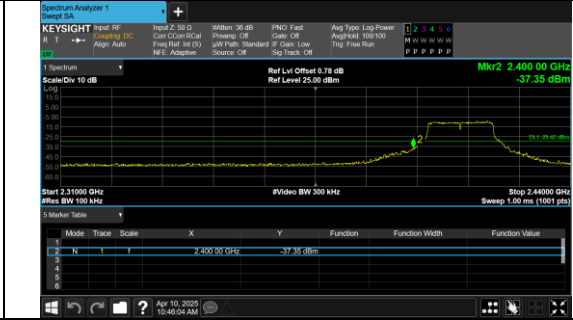
Out Of Band Emission IEEE 802.11g Channel 1 20MHz Antenna 0
