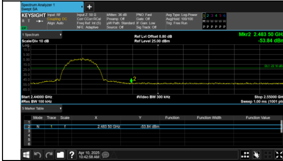
Out Of Band Emission IEEE 802.11b Channel 11 20MHz Antenna 0
