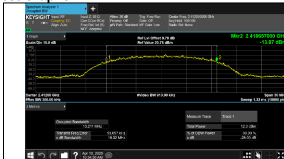
IEEE 802.11b Channel 1 20MHz Antenna 0
