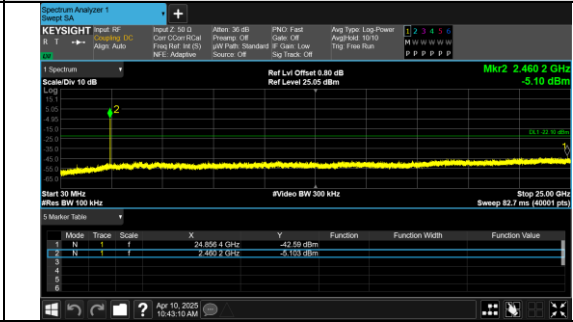
30.0 MHz - 25000.0 MHz IEEE 802.11b Channel 11 20MHz Antenna 0
