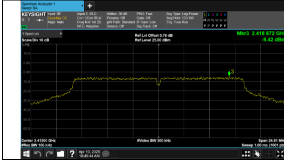
In-Band Reference Level IEEE 802.11g Channel 1 20MHz Antenna 0
