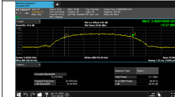
IEEE 802.11b Channel 11 20MHz Antenna 0
