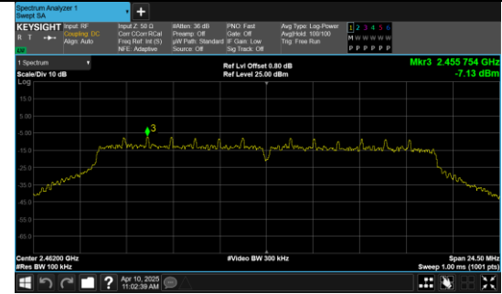
In-Band Reference Level IEEE 802.11n_Channel 11_20MHz_Antenna 0
