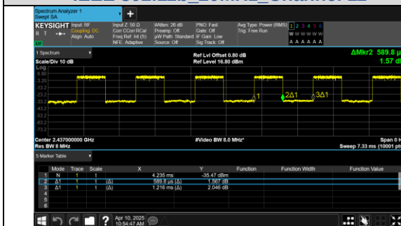
IEEE 802.11g 20MHz Channel 6
