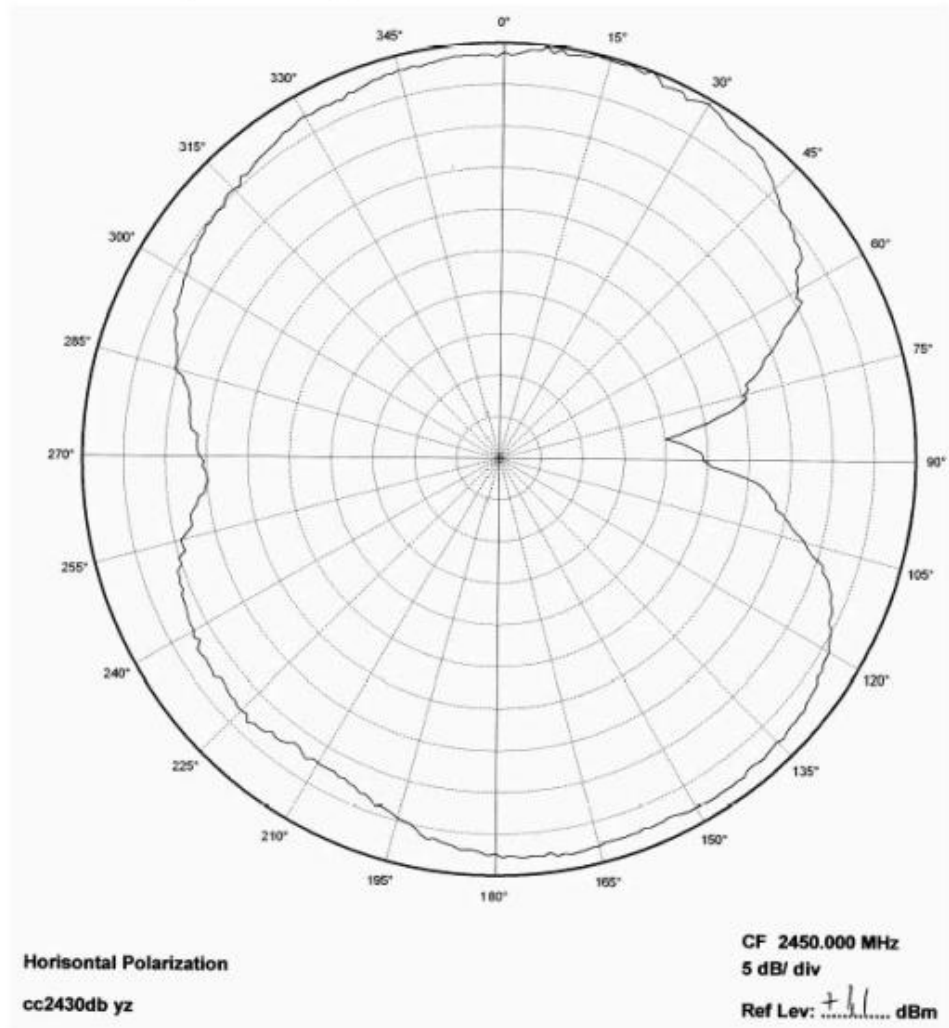
YZ Plane—Horizontal Polarization
