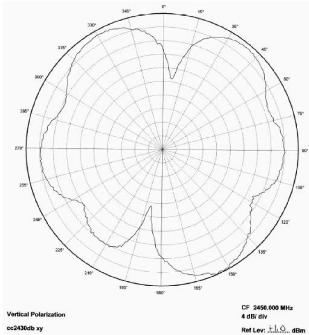
XY Plane-Vertical Polarization
