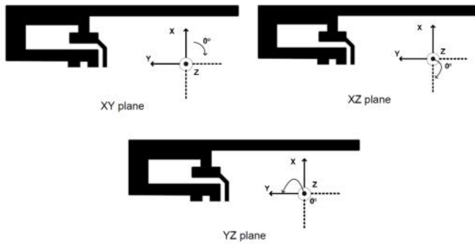
Figure 2-1. Relating Antenna to Radiation Patterns
