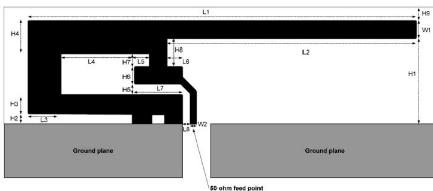
Figure 1-1. IFA Dimensions
