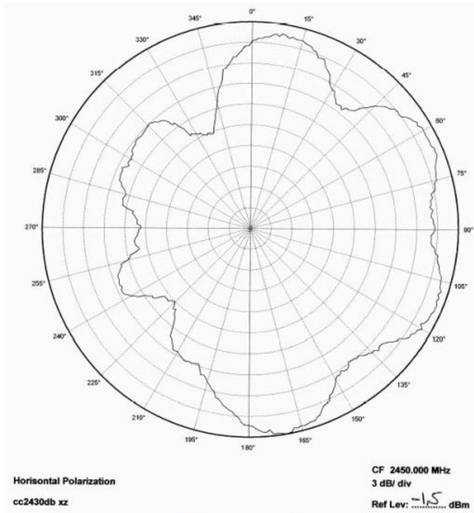
XZ Plane—Horizontal Polarization
