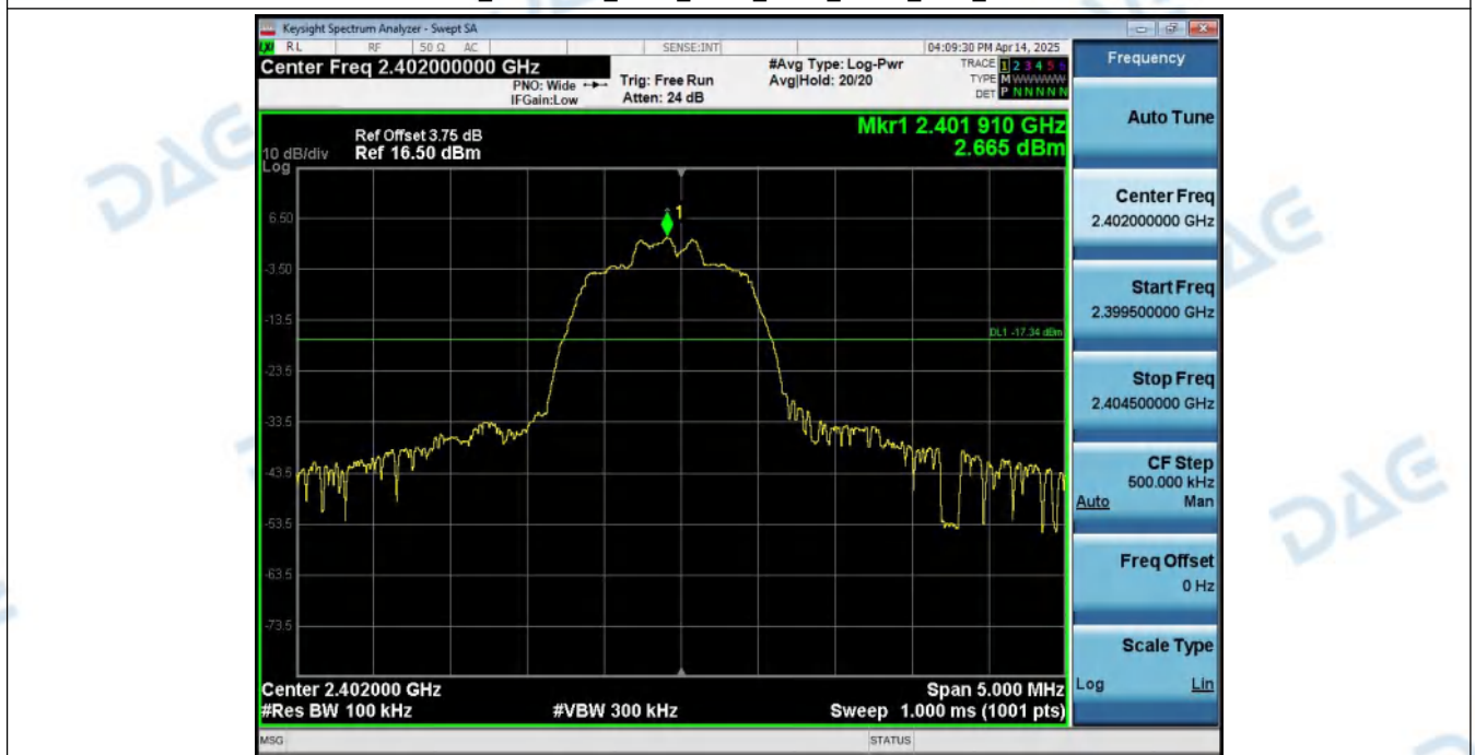
2_Bandedge_NVNT_ANT1_2-DH5_2402_00
