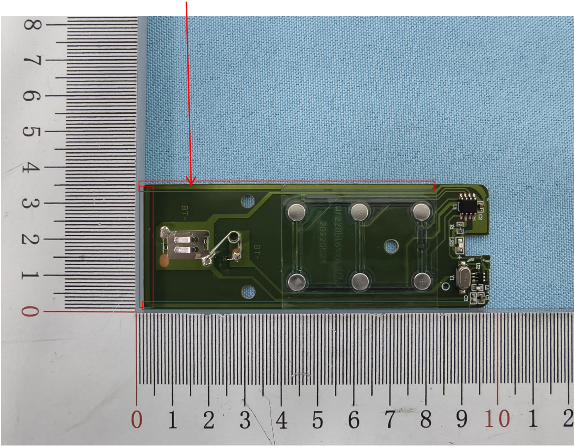
Antenna Photo & Length (cm)
