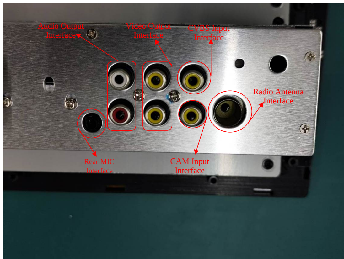
Rear Interface
