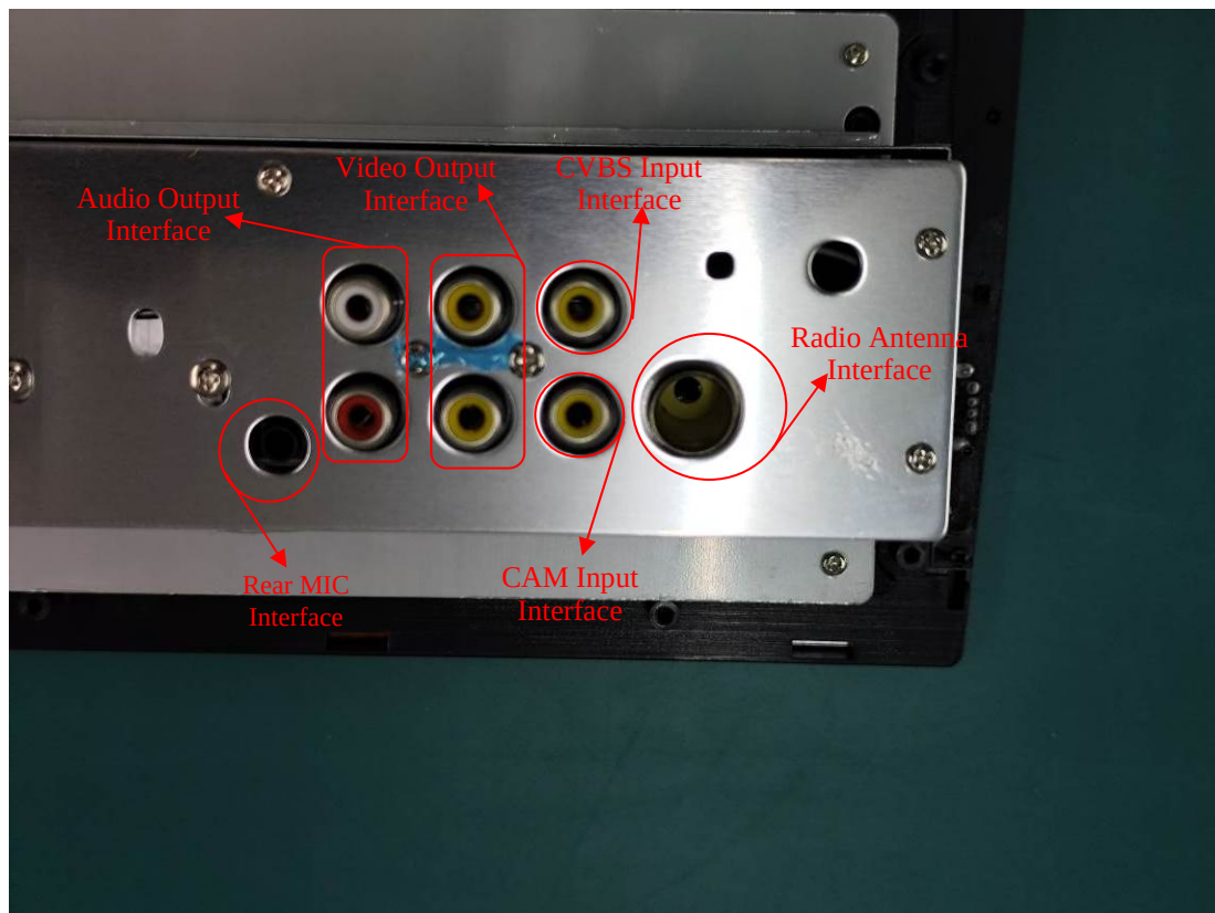
Rear Interface
