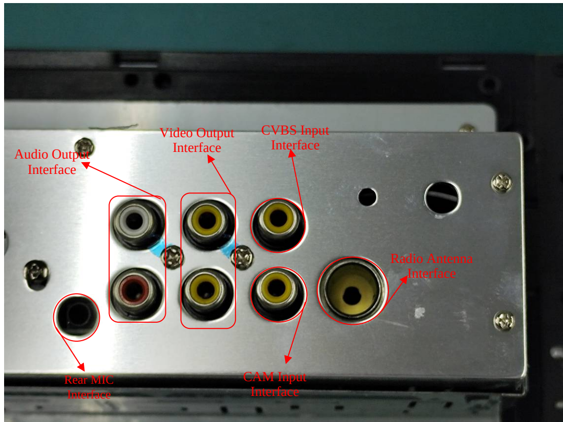
Rear Interface
