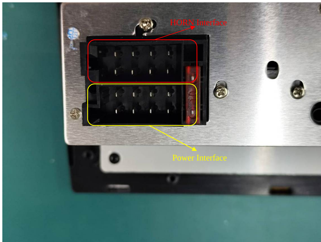
Rear Interface
