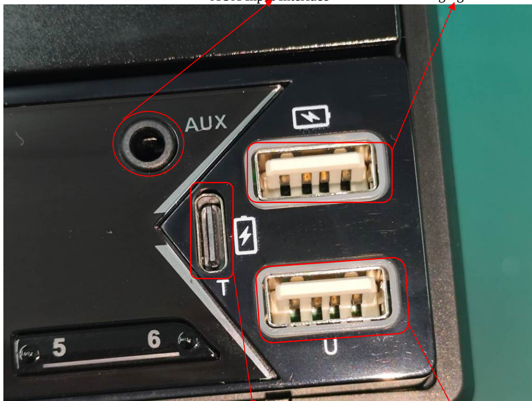
TYPE-C Charging Interface
