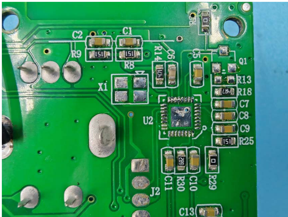
Reserved Antenna (not linked to any RF chip)
