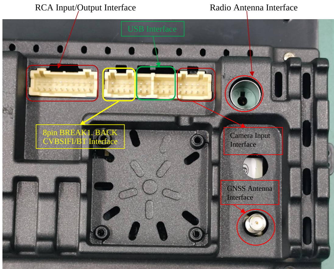
GNSS Antenna
