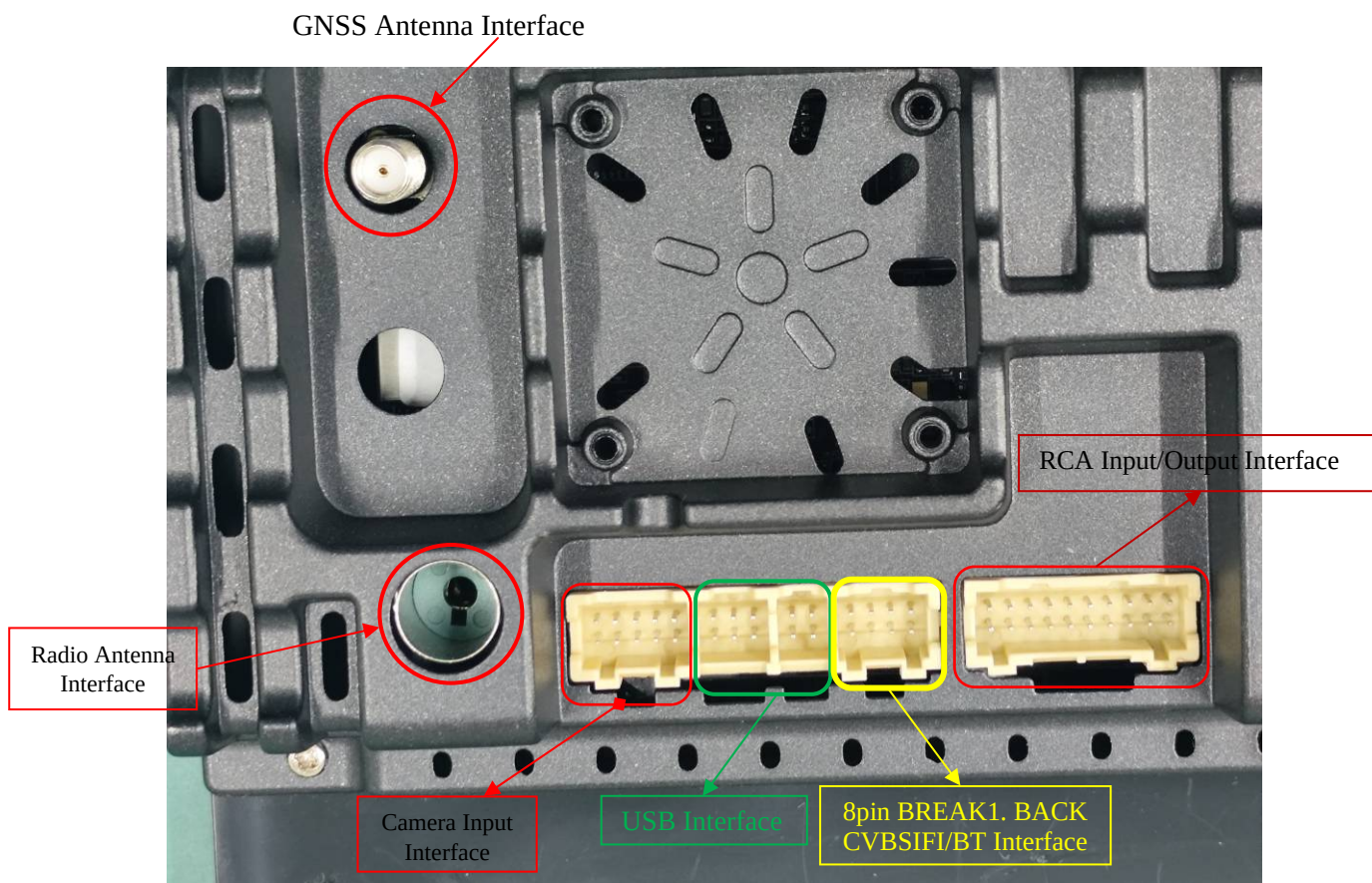
GNSS Antenna
