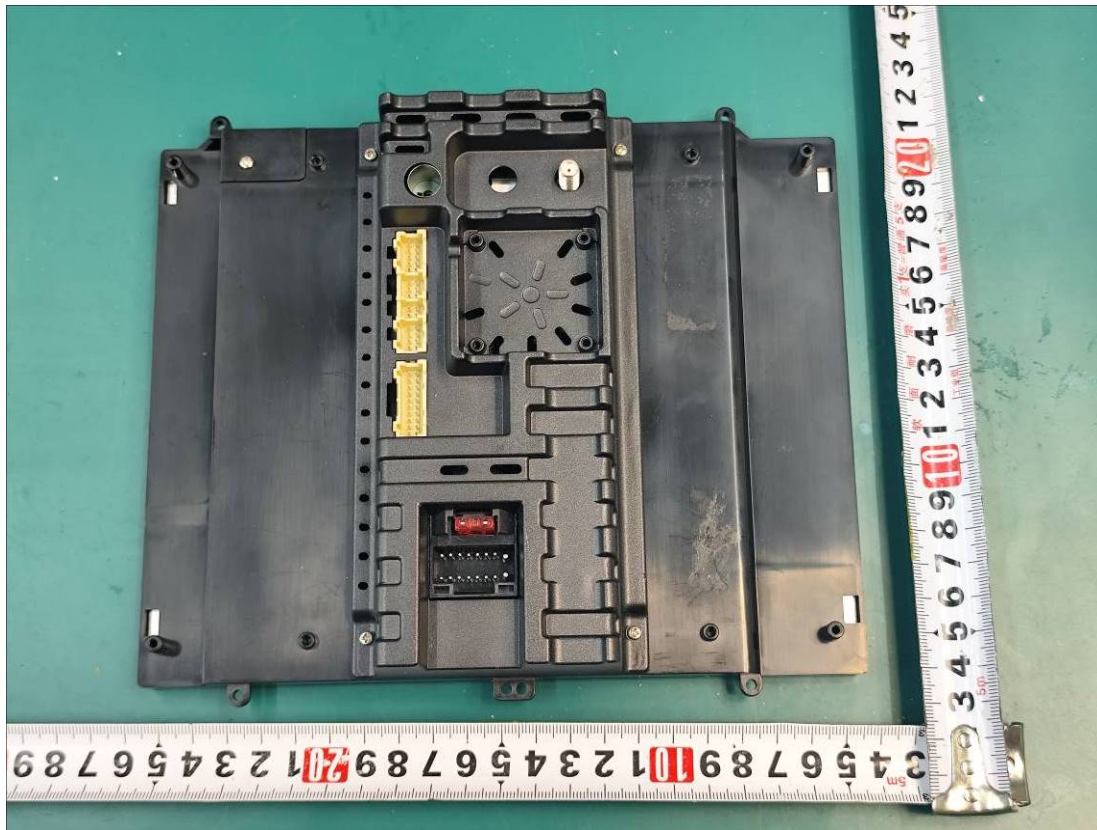
CAN Interface
