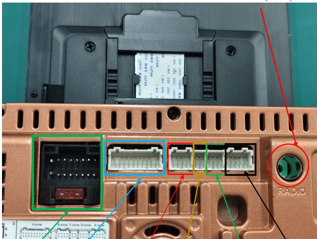
CAN-BUS Interface
