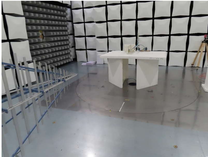
Test setup semi anechoic chamber 30 MHz - 1 GHz
