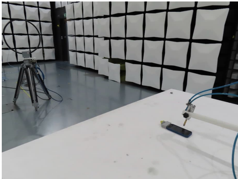
Test setup semi anechoic chamber <30 MHz
