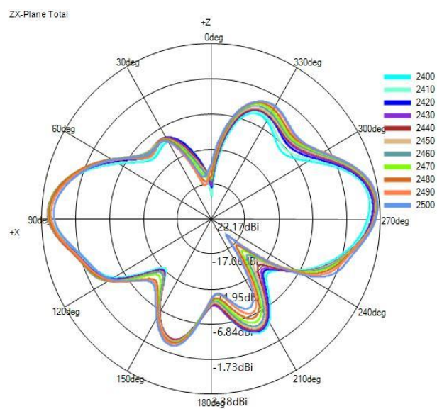
(1) X-Z Plane(unit:dBi):
