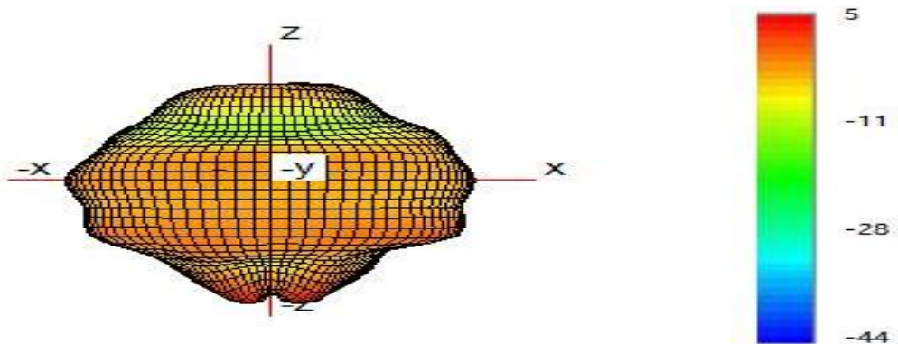
(4) Typical Free Space 3D Radiation Pattern at 5000MHz(unit:dBi):
