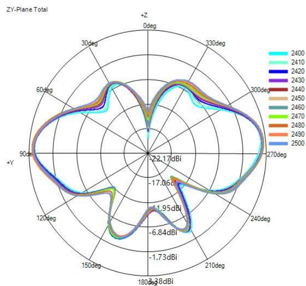
(2) Y-Z Plane(unit:dBi):
