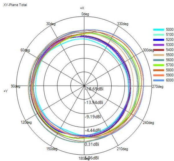
(3) X-Y Plane(unit:dBi):
