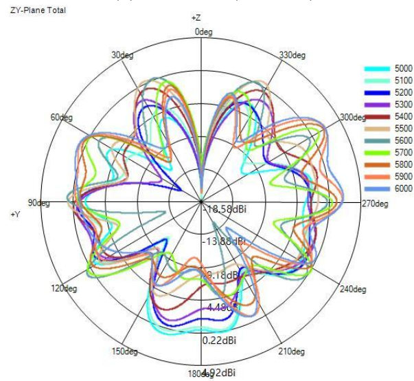
(2) Y-Z Plane(unit:dBi):
