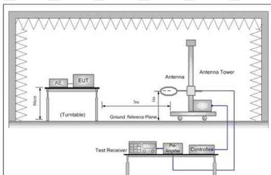
Figure 1. Below 30MHz
