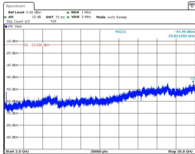
Band5-1.4MHz-QPSK-20407-1RB#0-Range1:30~1000MHz
