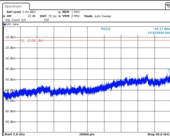
Band2-20MHz-16QAM-19100-1RB#0-Range1:30~1000MHz
