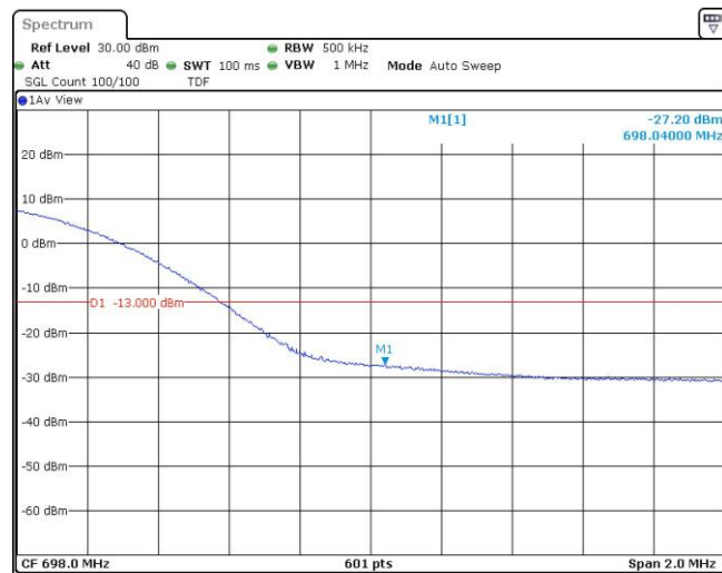
Band71-20MHz-16QAM-133222-1RB#0
