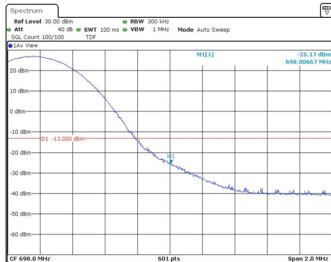
Band71-15MHz-16QAM-133397-75RB#0
