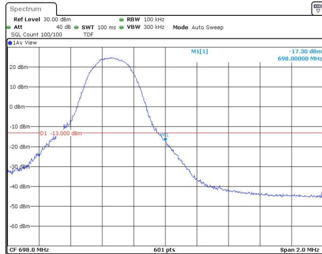
Band71-5MHz-16QAM-133447-25RB#0
