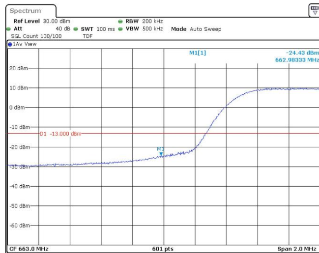
Band71-10MHz-16QAM-133422-1RB#0
