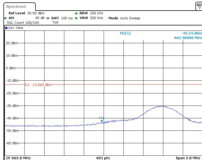
Band71-10MHz-16QAM-133172-50RB#0
