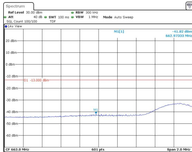
Band71-15MHz-QPSK-133197-75RB#0
