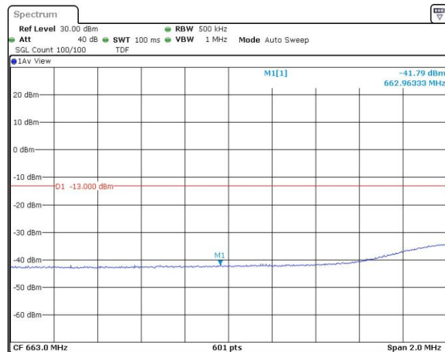
Band71-20MHz-QPSK-133222-100RB#0
