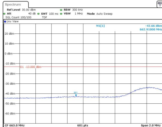
Band71-15MHz-16QAM-133197-75RB#0
