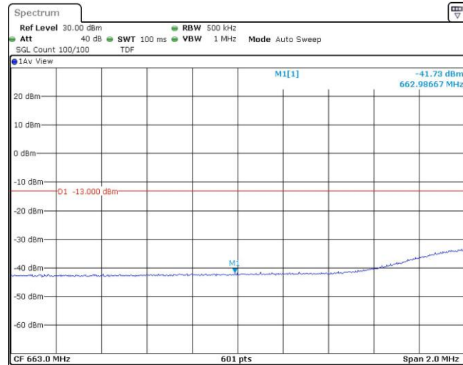
Band71-20MHz-16QAM-133222-100RB#0
