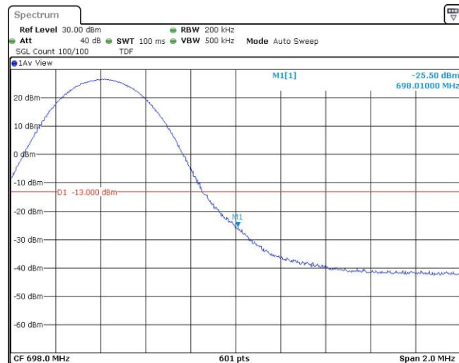
Band71-10MHz-16QAM-133422-50RB#0
