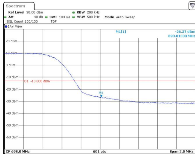
Band71-10MHz-16QAM-133172-1RB#0
