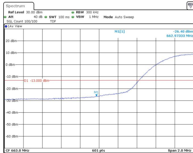
Band71-15MHz-16QAM-133397-1RB#0
