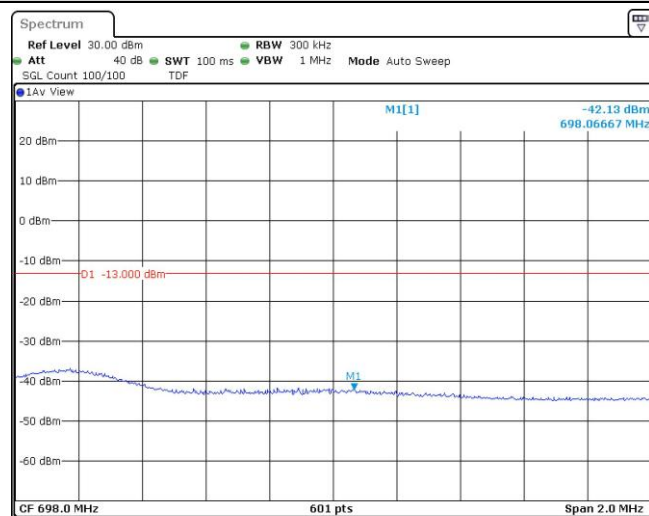
Band71-15MHz-16QAM-133397-1RB#74
