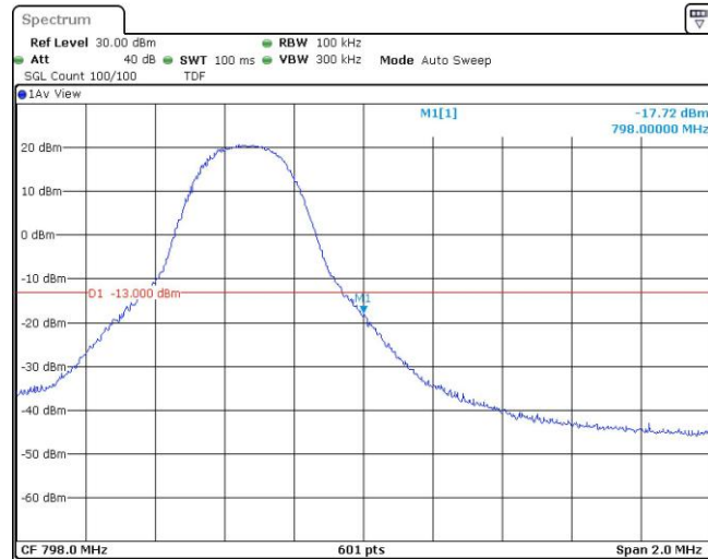
Band14-5MHz-16QAM-23355-25RB#0
