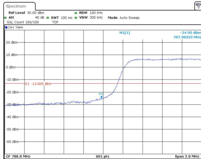
Band14-5MHz-QPSK-23355-1RB#0
