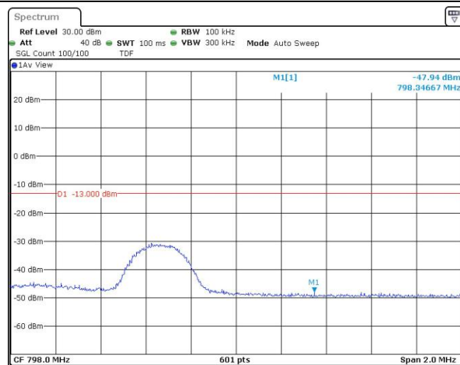
Band14-5MHz-QPSK-23355-1RB#24
