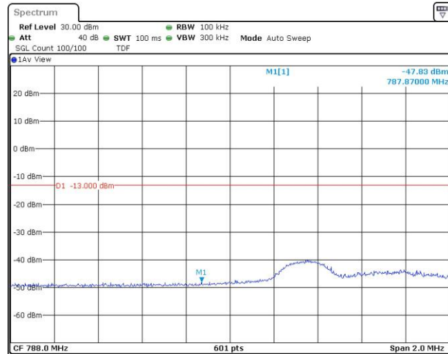
Band14-5MHz-QPSK-23305-25RB#0
