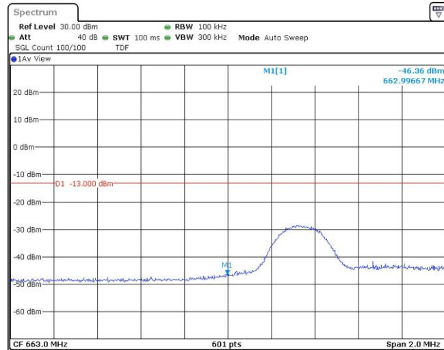
Band71-5MHz-16QAM-133147-25RB#0
