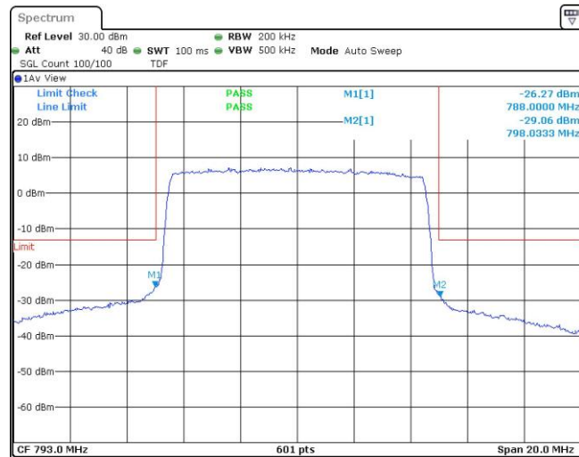
Band14-10MHz-16QAM-23330-1RB#0
