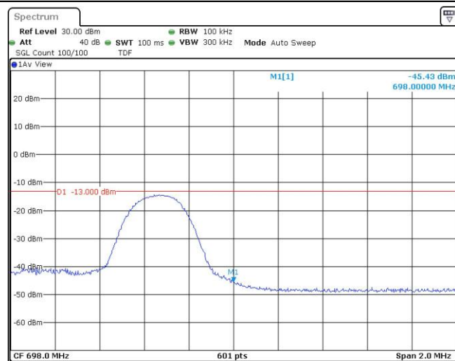
Band71-5MHz-QPSK-133447-1RB#24
