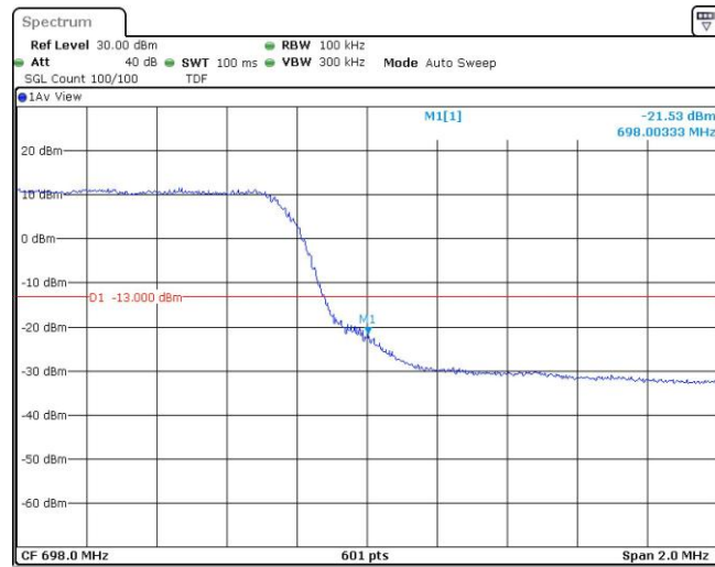
Band71-5MHz-16QAM-133147-1RB#0
