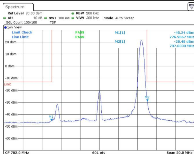
Band13-10MHz-16QAM-23230-50RB#0
