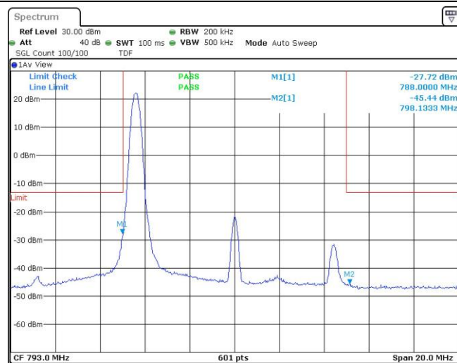
Band14-10MHz-QPSK-23330-1RB#49
