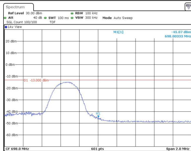
Band71-5MHz-16QAM-133447-1RB#24
