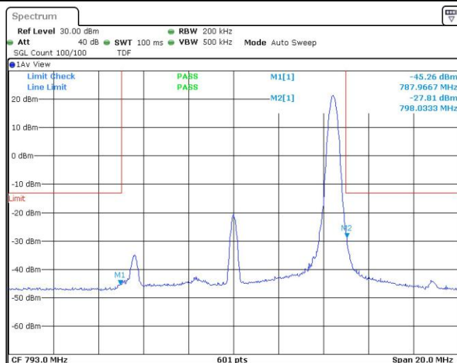
Band14-10MHz-16QAM-23330-50RB#0
