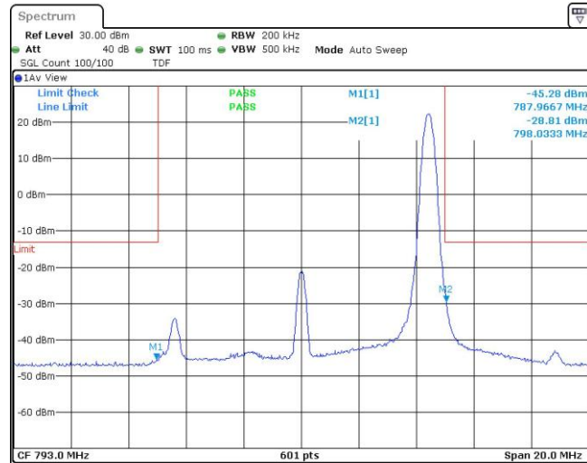
Band14-10MHz-QPSK-23330-50RB#0
