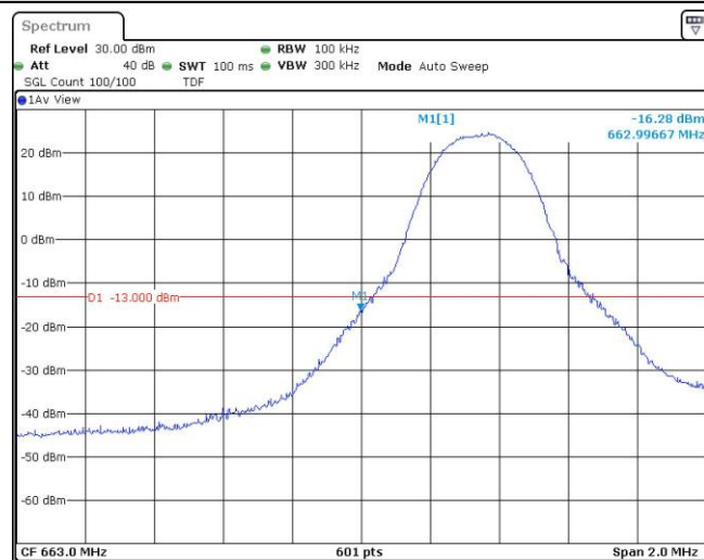
Band71-5MHz-16QAM-133147-1RB#24
