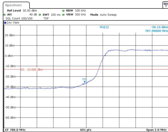
Band14-5MHz-16QAM-23355-1RB#0
