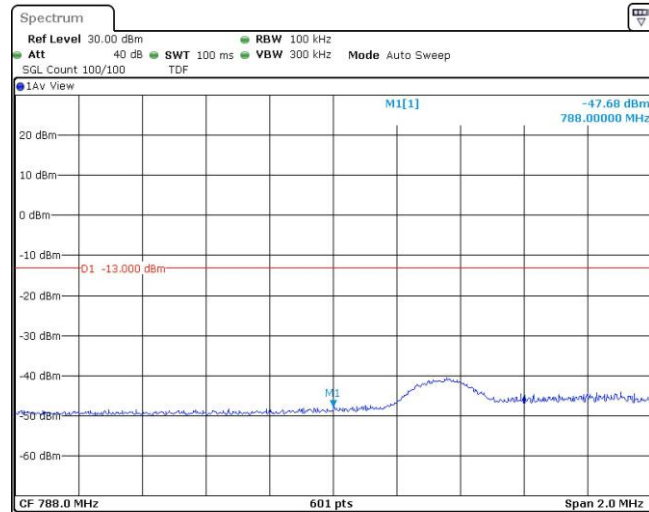
Band14-5MHz-16QAM-23305-25RB#0
