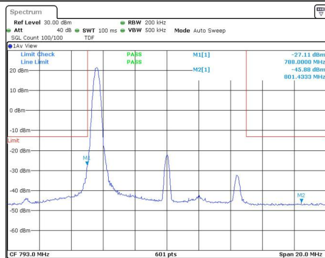
Band14-10MHz-16QAM-23330-1RB#49
