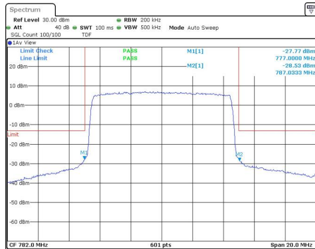
Band13-10MHz-16QAM-23230-1RB#0
