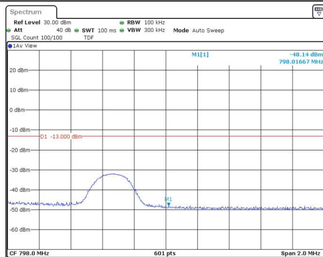
Band14-5MHz-16QAM-23355-1RB#24
