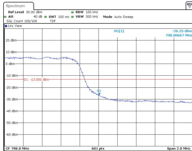
Band14-10MHz-QPSK-23330-1RB#0
