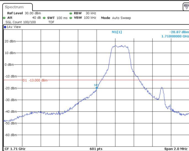
Band66-1.4MHz-QPSK-131979-1RB#5
