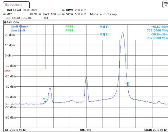
Band13-10MHz-QPSK-23230-50RB#0
