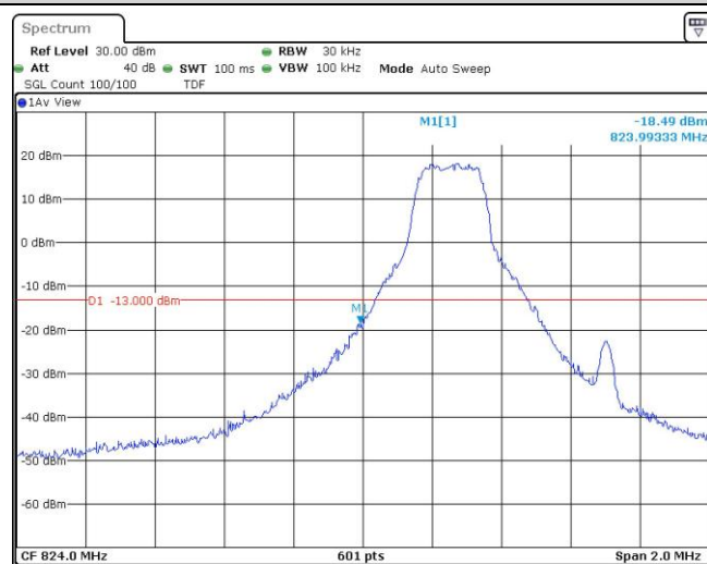
Band5-1.4MHz-QPSK-20407-1RB#5
