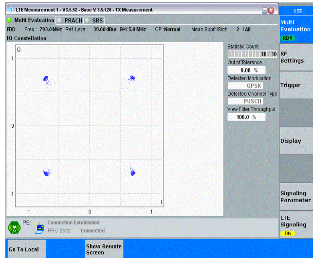
Band14-5MHz-QPSK-23355-25RB#0
