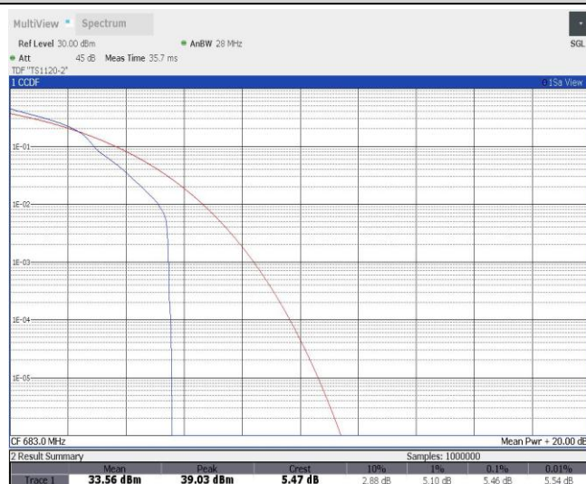
Band71-20MHz-16QAM-133322-100RB#0
