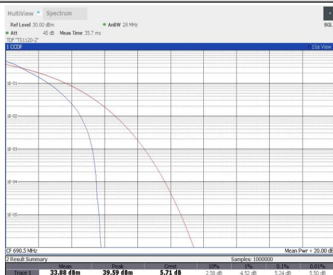
Band71-15MHz-16QAM-133197-1RB#0
