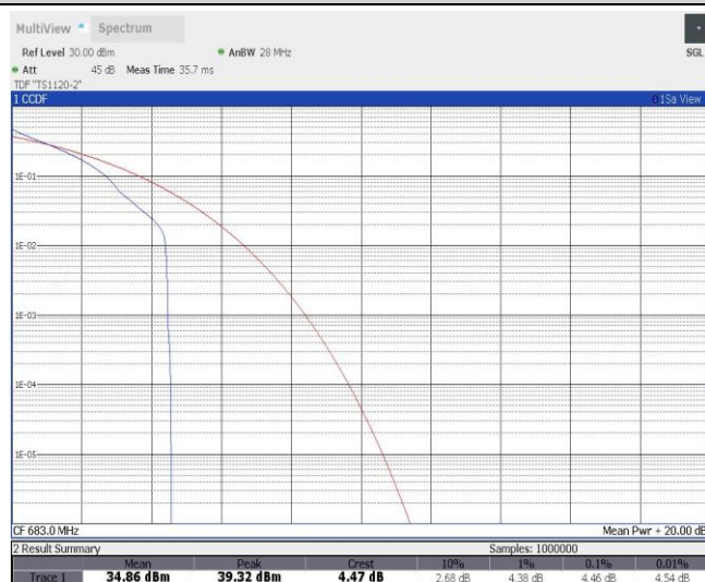
Band71-20MHz-QPSK-133322-100RB#0
